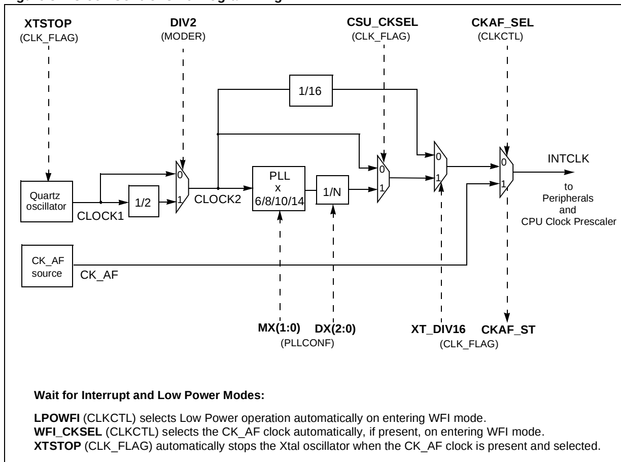
Figure 32. Clock Control Unit Programming
