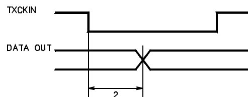
FIG 2: TRANSMISSION WITH EXTERNAL CLOCK 1X MODE
