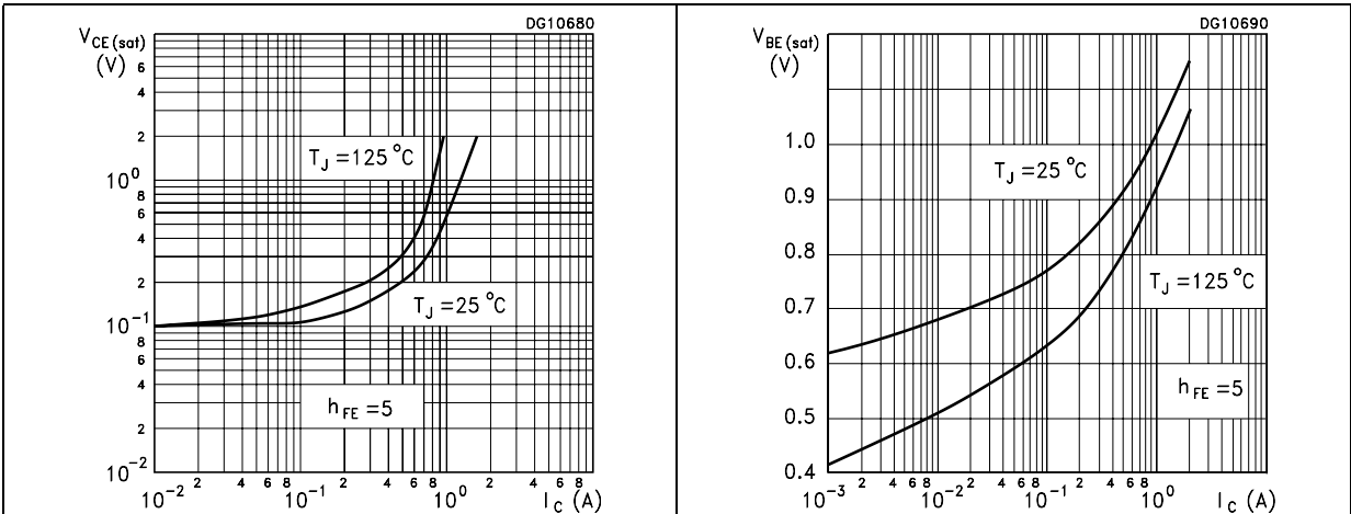
Figure 6. Collector emitter saturation voltage Figure 7. Base emitter saturation voltage
