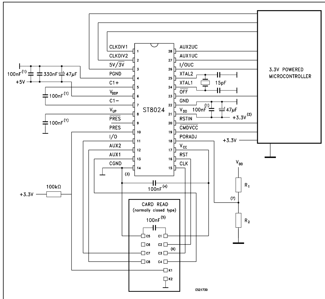
Figure 10. Application diagram
