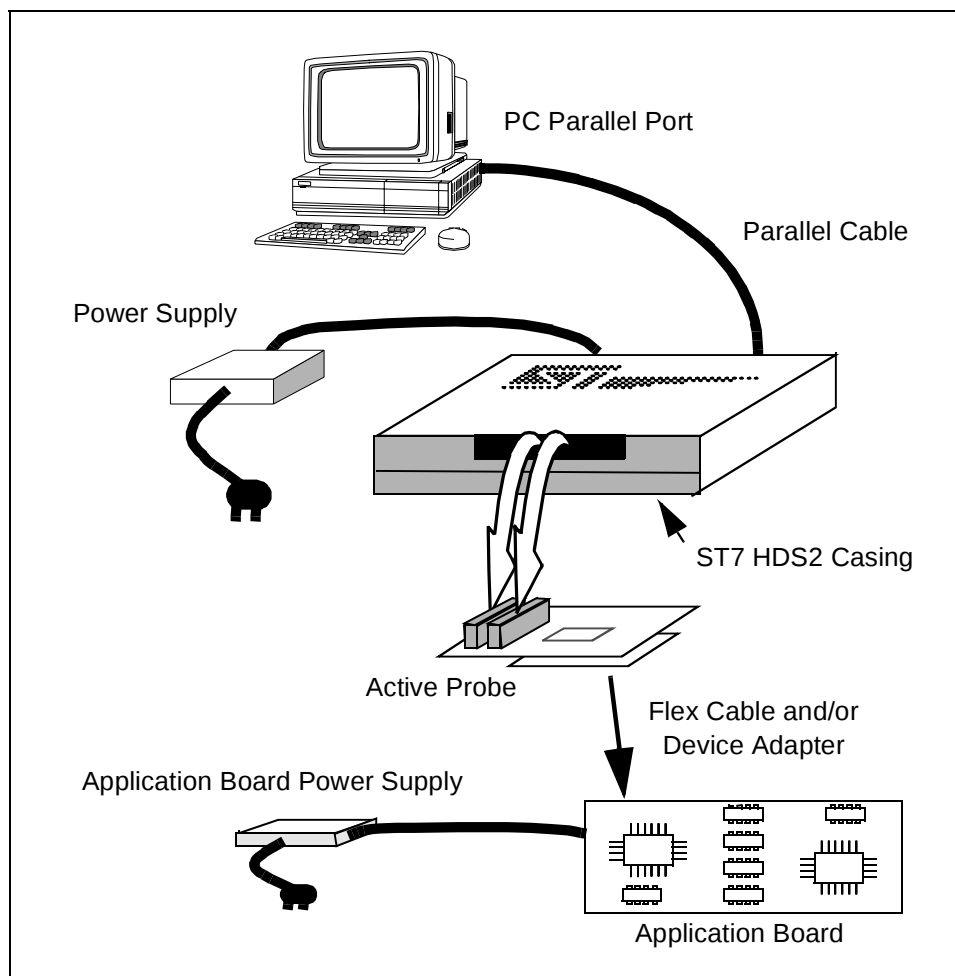
Figure 1: ST7MDTS1-EMU2B general configuration
