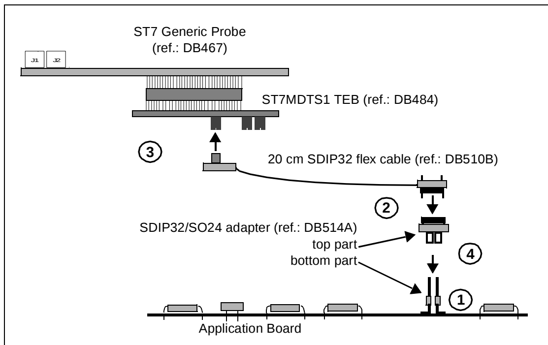
Figure 8: SO24 MCU package connections
