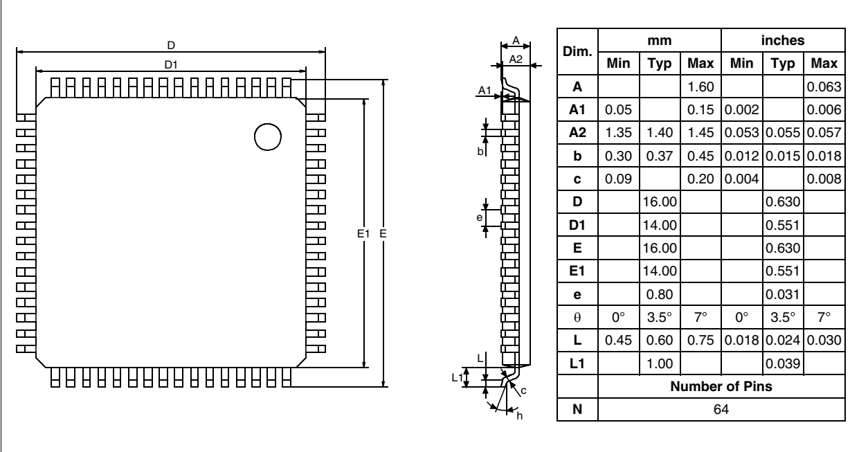
Figure 44. 64-Pin Low Profile Quad Flat Package (14x14)
