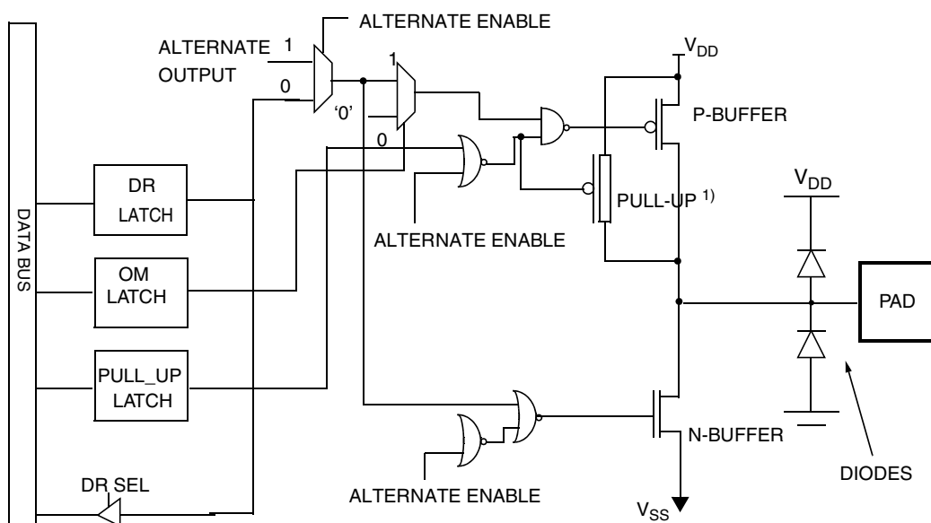
Figure 25. Port B and D Configuration
