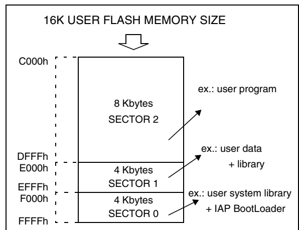
Figure 8. Memory map and sector address
