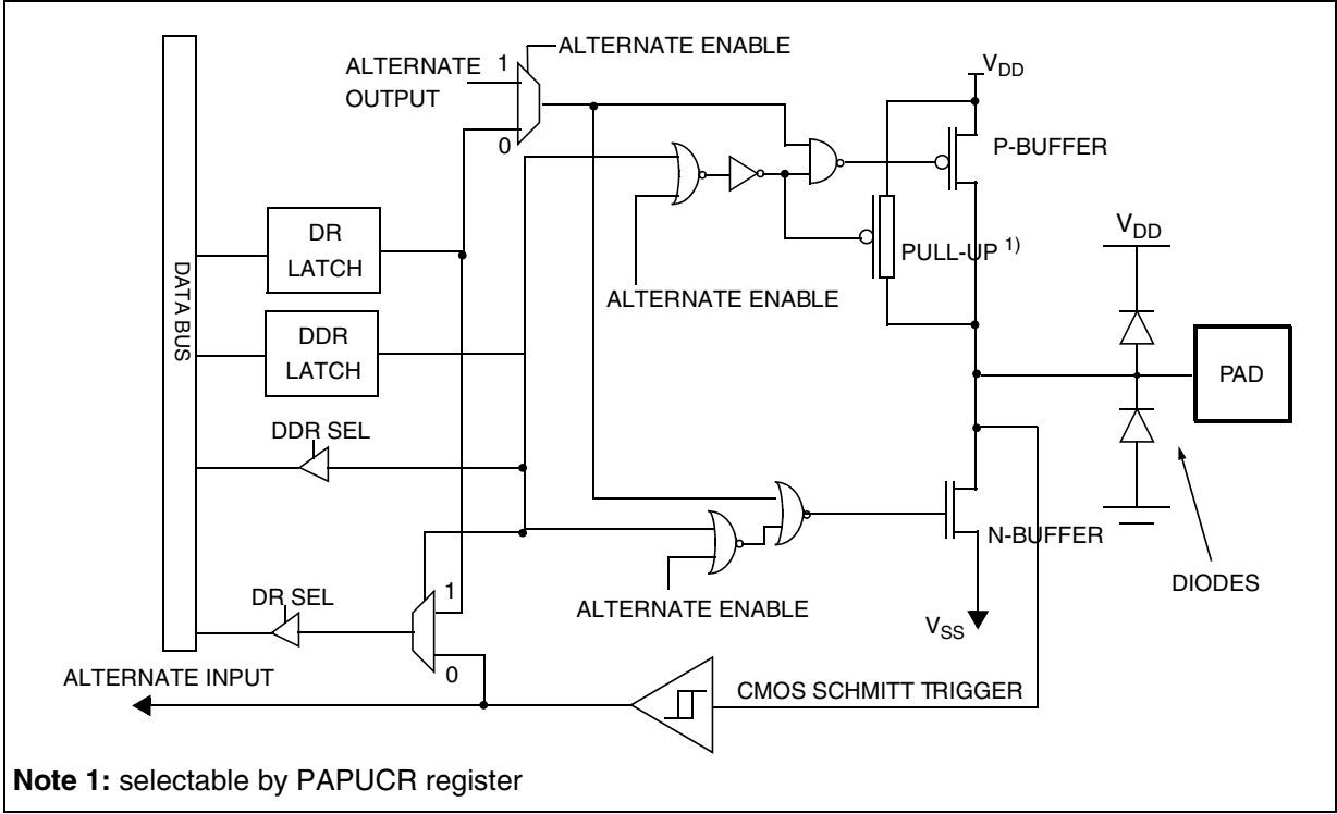
Figure 24. PA6 Configuration
