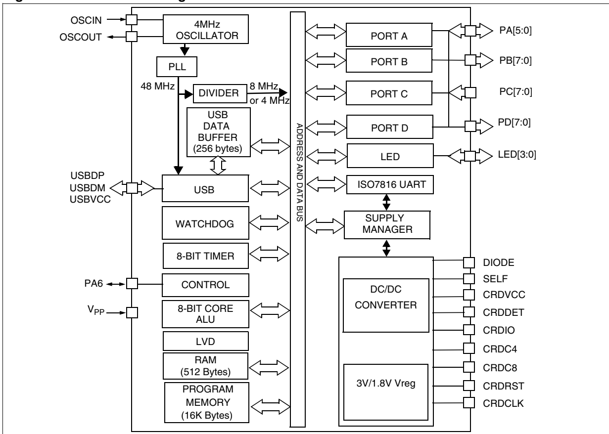
Figure 1. ST7SCR Block Diagram
