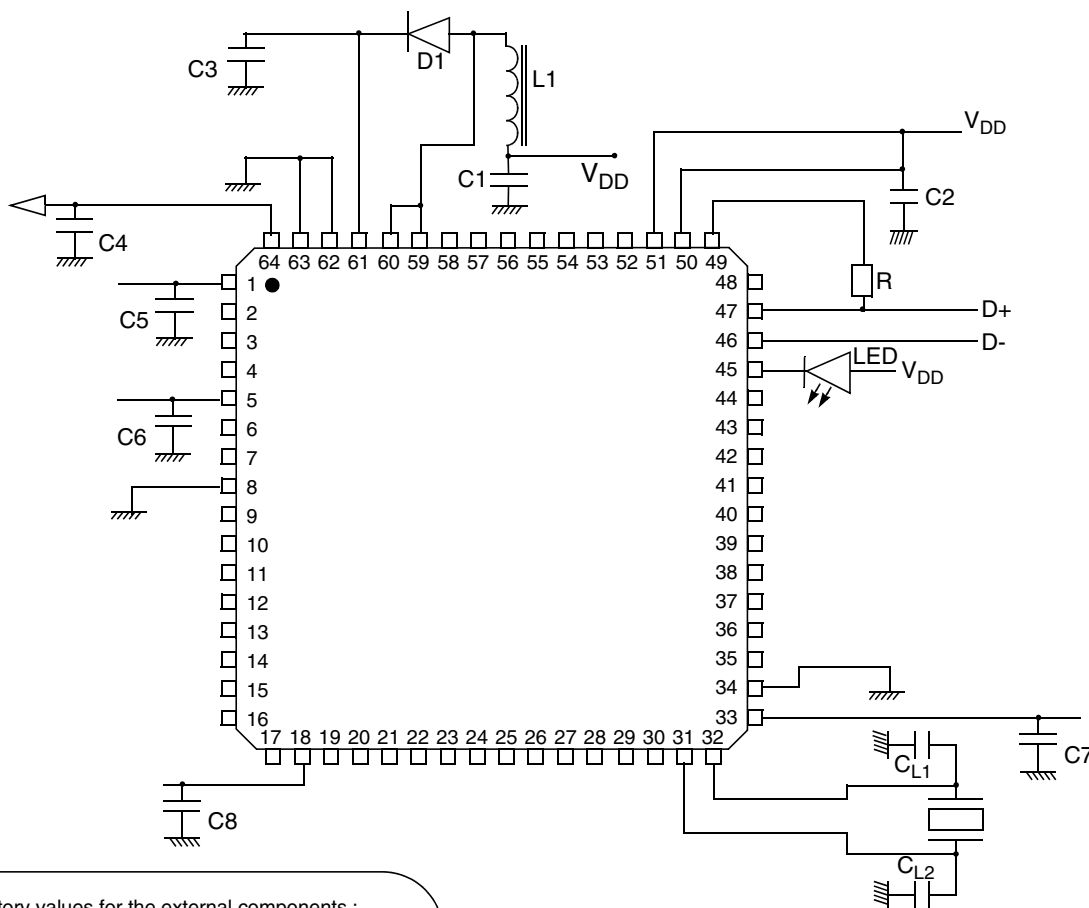
Figure 6. Smartcard Interface Reference Application - 64-Pin LQFP Package
