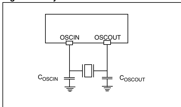
Figure 14. Crystal Resonator
