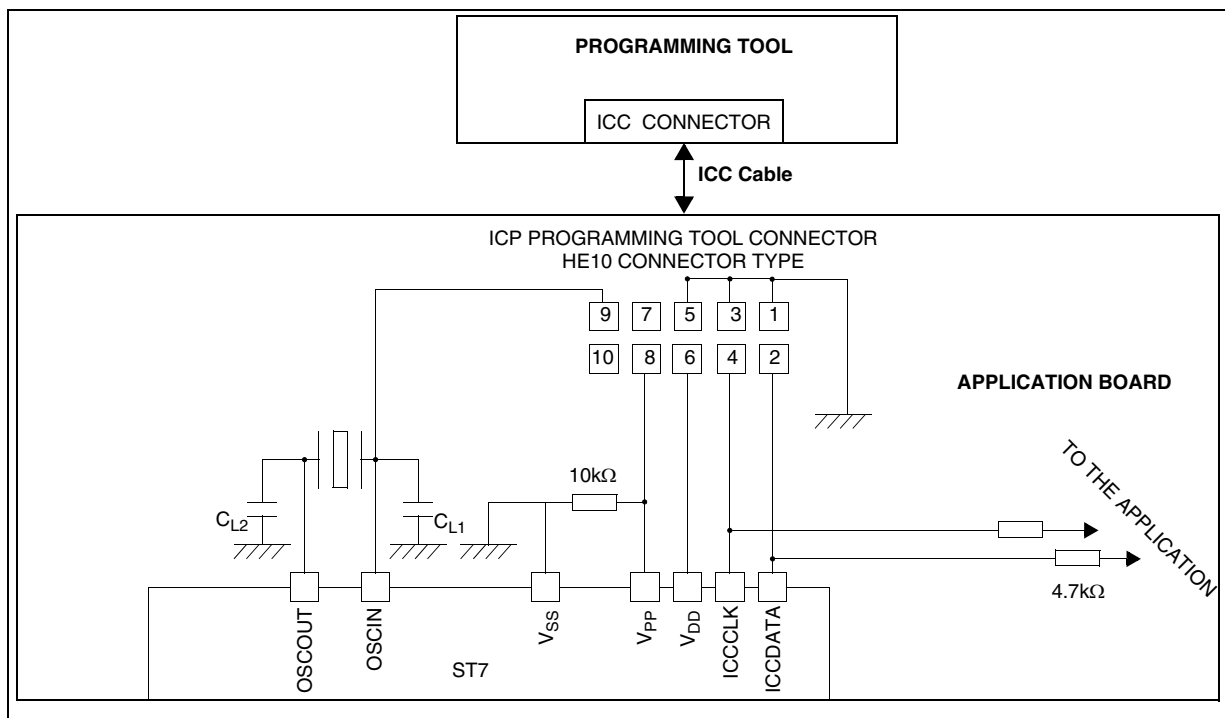
Figure 9. Typical ICP Interface
