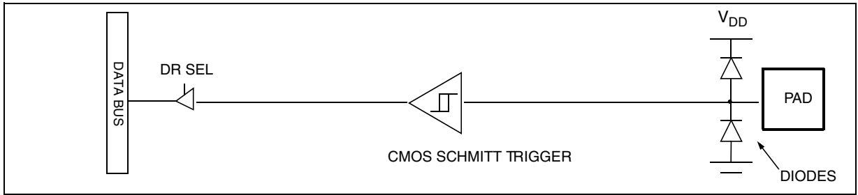
Figure 24. PA6 Configuration
