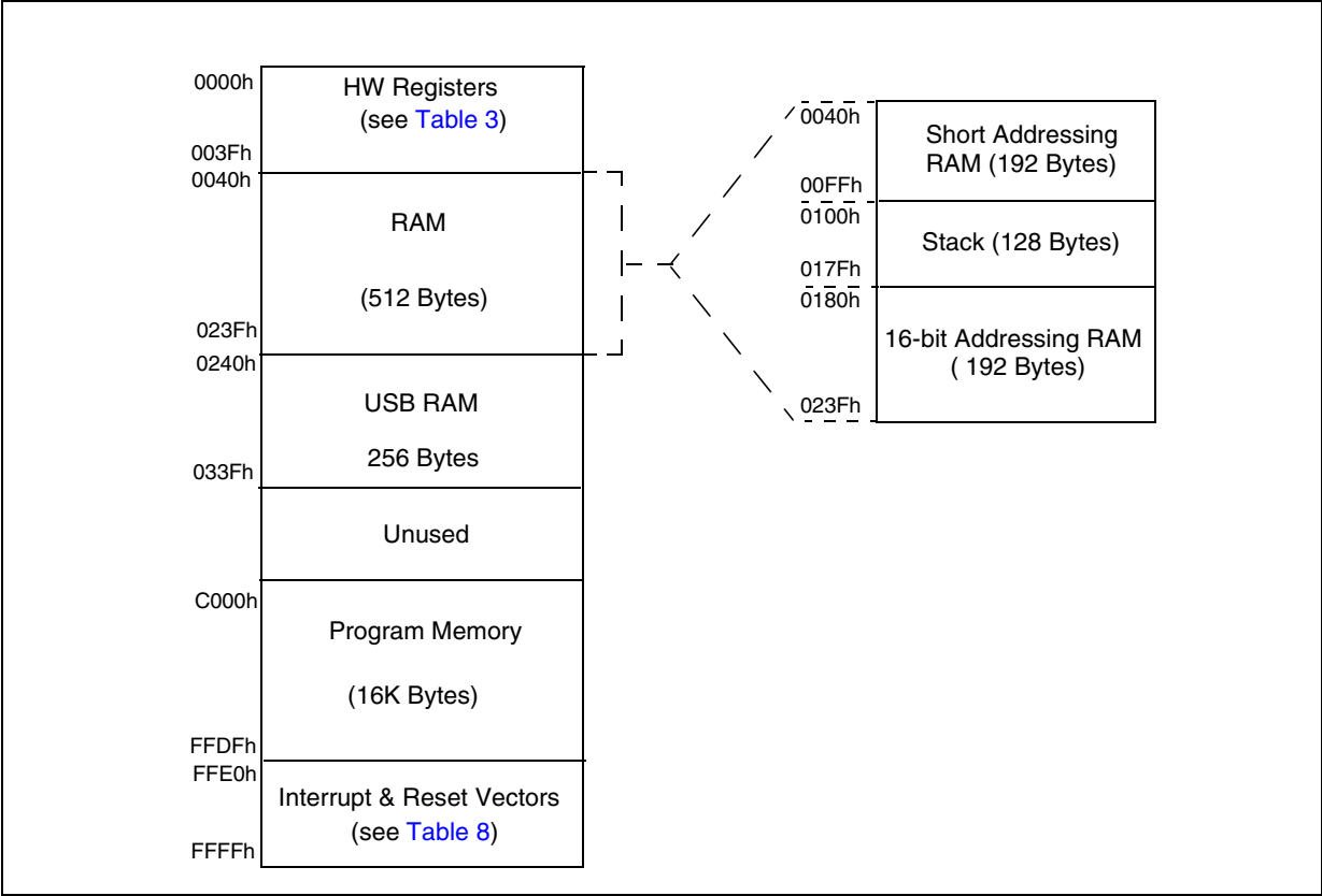
Figure 7. Memory Map
