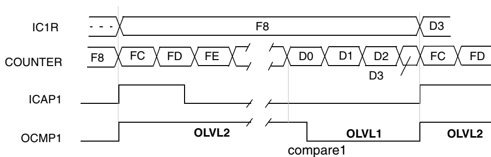
Figure 68. One Pulse Mode Timing Example
