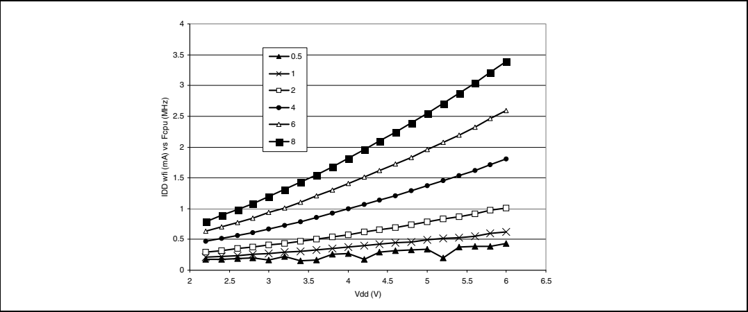
Figure 93. Typical I_{DD} in Wait at f_{CPU} = 8\text{ MHz}
