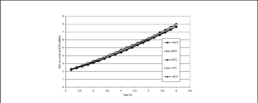
Figure 90. Typical I_{DD} in Run at f_{CPU} = 8\text{ MHz}
