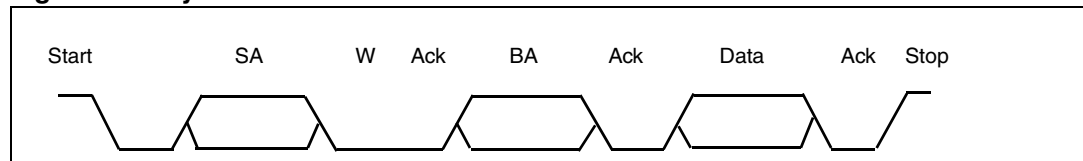
Figure 76. Byte write
