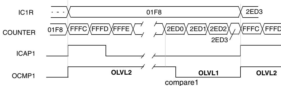
Figure 41. One Pulse Mode Timing Example
