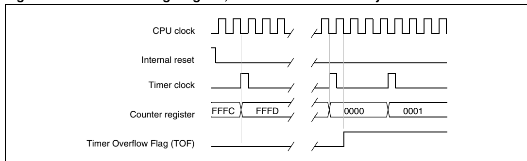
Figure 39. Counter timing diagram, internal clock divided by 4
