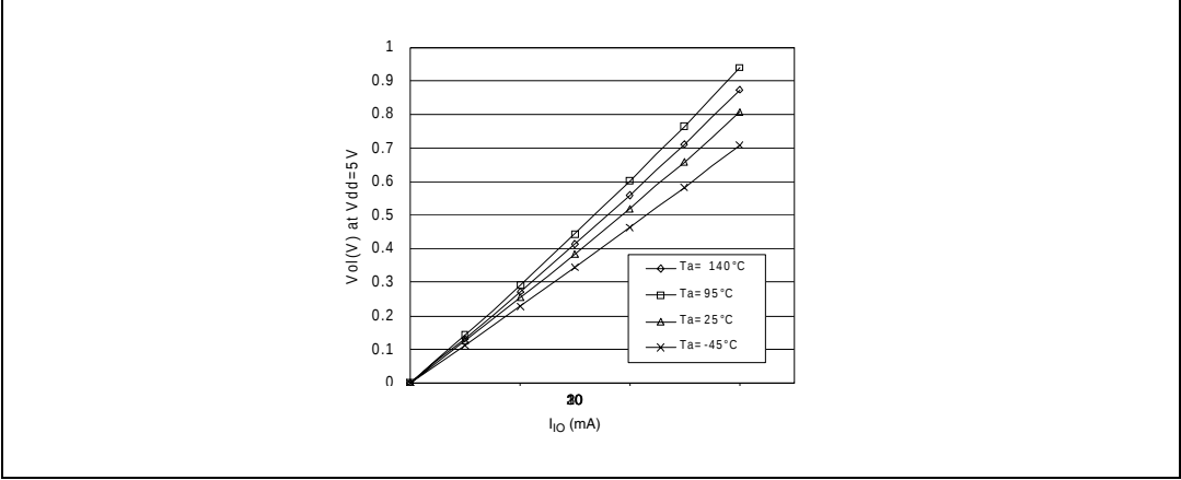
Figure 73. Typical V_{OL} at V_{DD} = 5V (high-sink ports)
