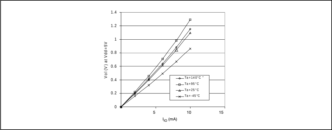
Figure 72. Typical V_{OL} at V_{DD} = 5V (standard ports)
