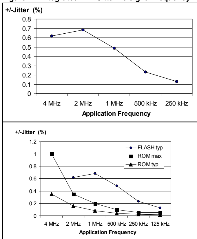
Figure 77. Integrated PLL Jitter vs signal frequency 1
