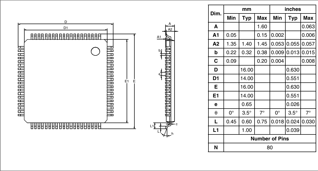
Figure 98. 80-Pin Low Profile Quad Flat Package
