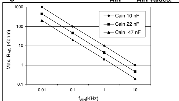
Figure 94. Recommended C_{AIN} & R_{AIN} values. 2)
