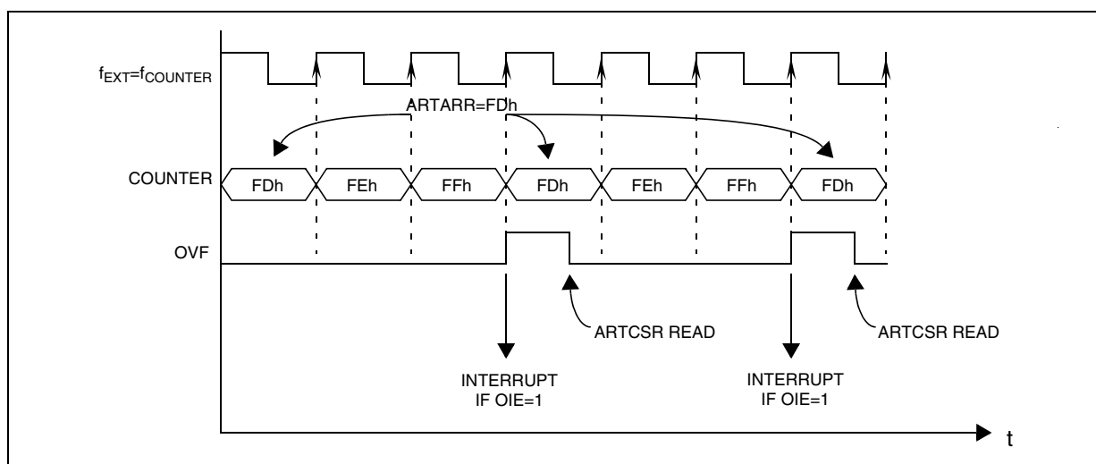
Figure 37. External Event Detector Example (3 counts)
