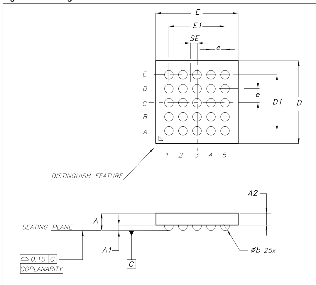
Figure 5. Package dimensions
