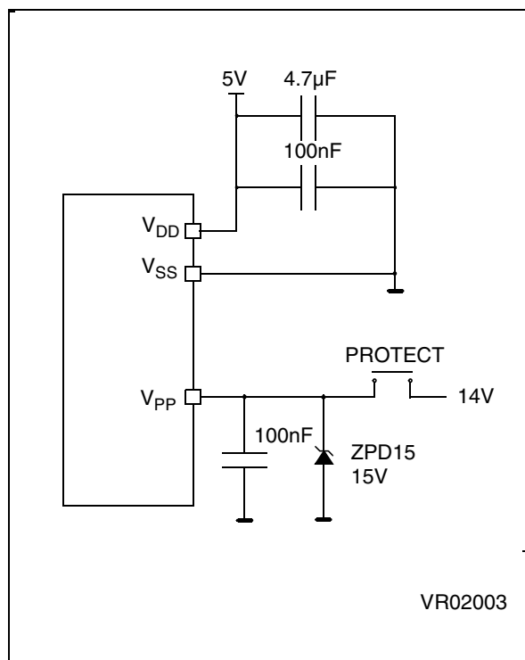
Figure 73. Programming Circuit
