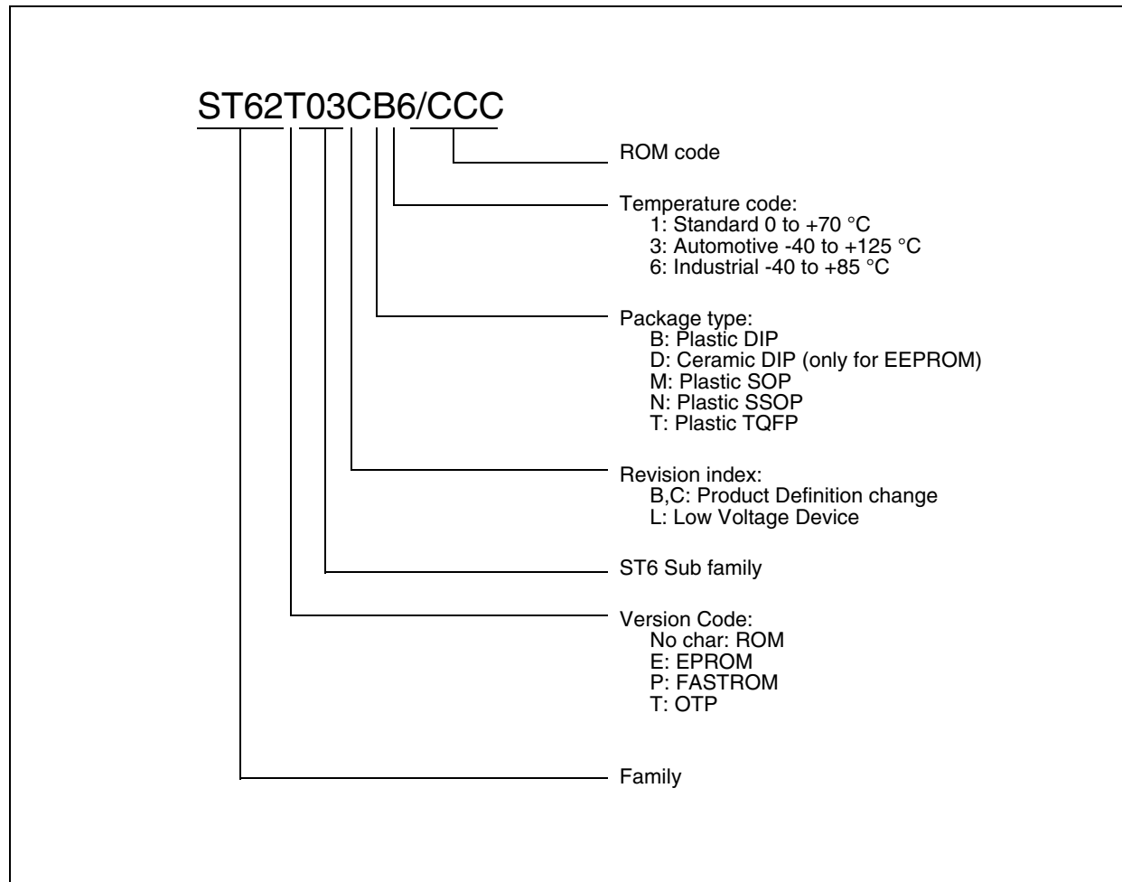
Figure 72. ST6 Factory Coded Device Types
