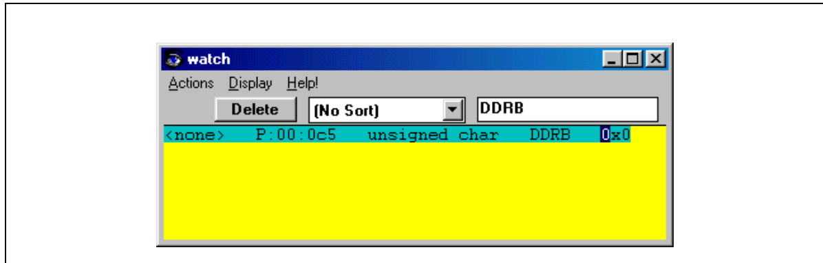
Figure 13: Watch window
