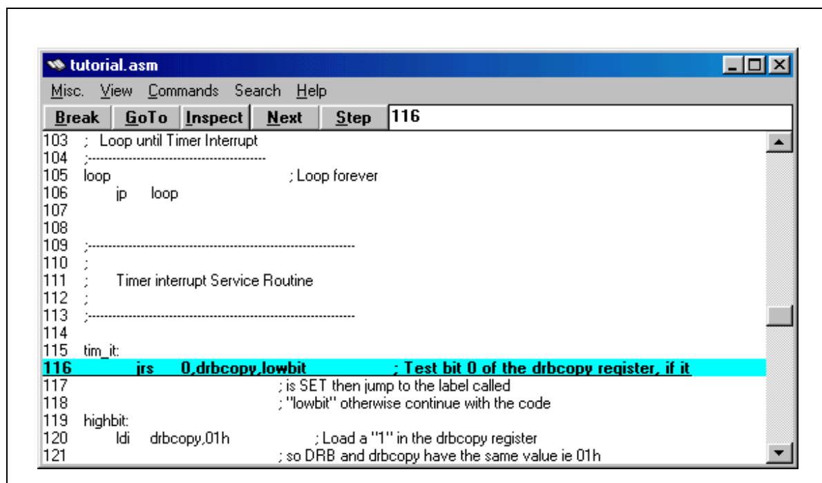
Figure 16: Breakpoint encountered
