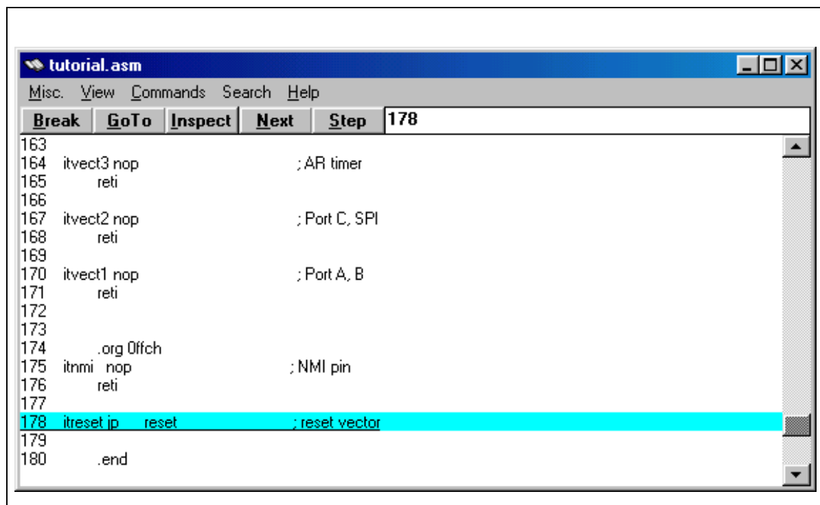
Figure 11: tutorial.asm window
