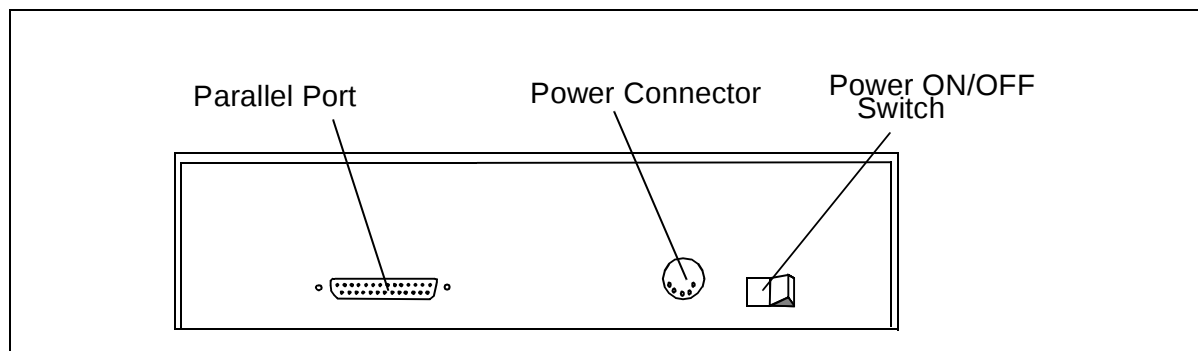
Figure 2: ST62GP-EMU2 Back Panel
