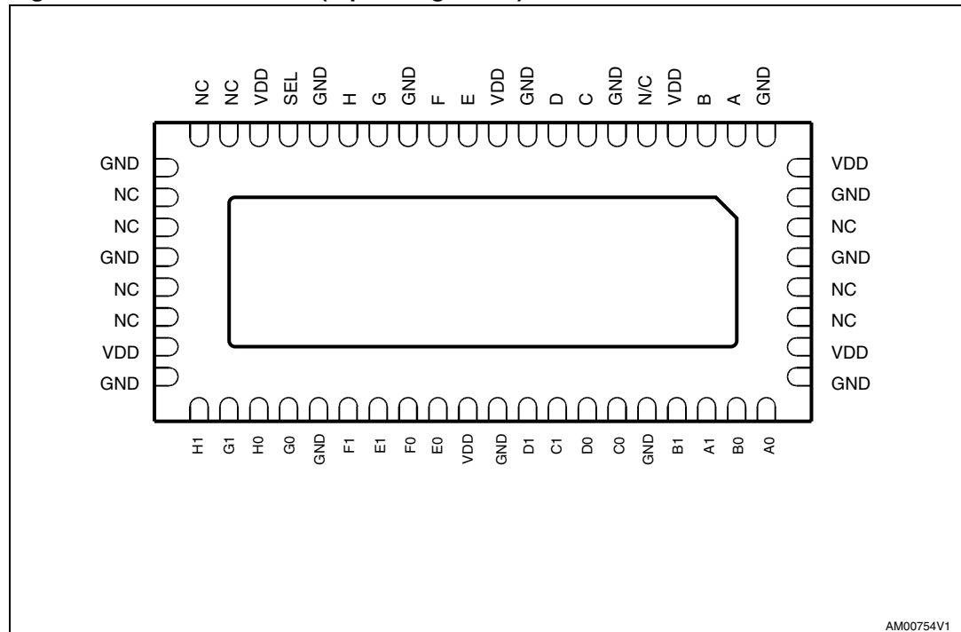
Figure 1. Pin connection (top through view)
