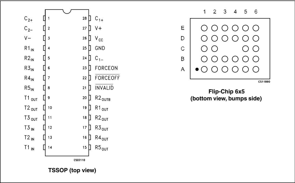
Figure 1. Pin configuration
