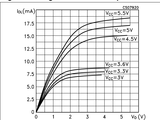
Figure 5. High level receiver output current
