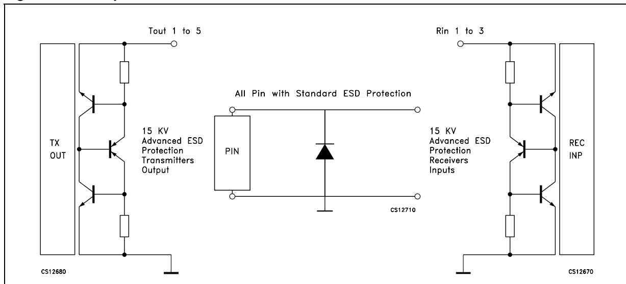
Figure 6. ESD protection
