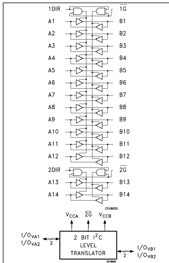
Figure 1: Logic Diagram
