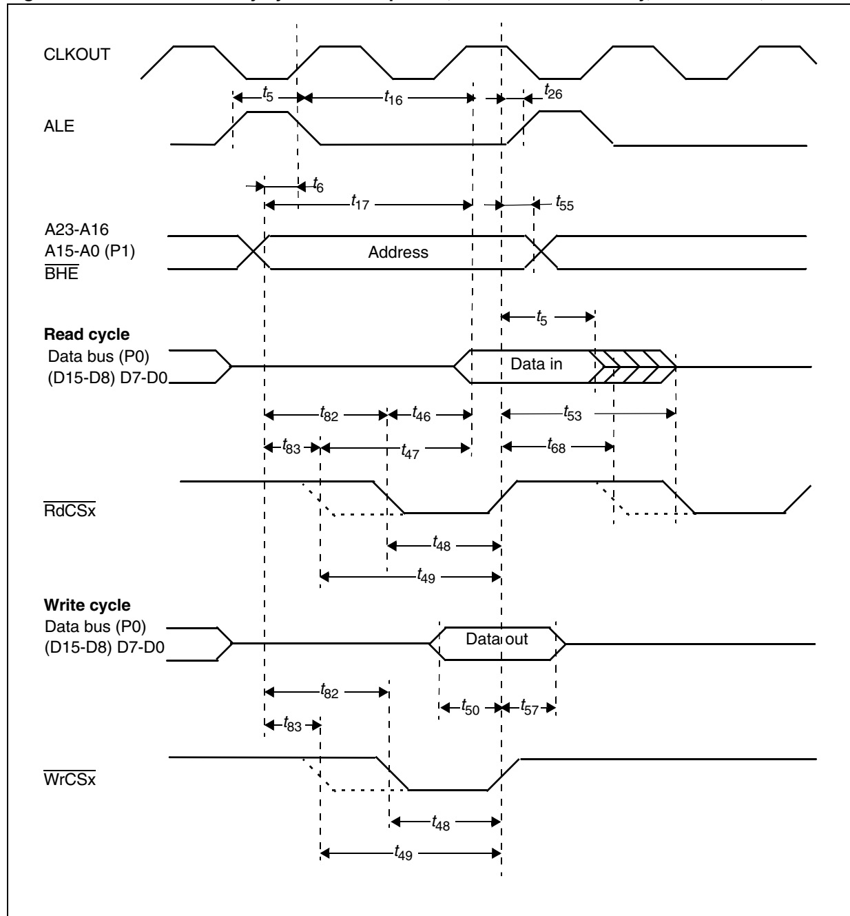
Figure 59. External memory cycle: Demultipl. bus, with/without r/w delay, normal ALE, r/w CS
