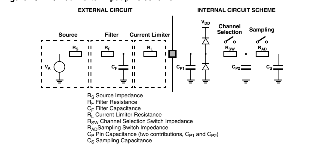
Figure 43. A/D converter input pins scheme
