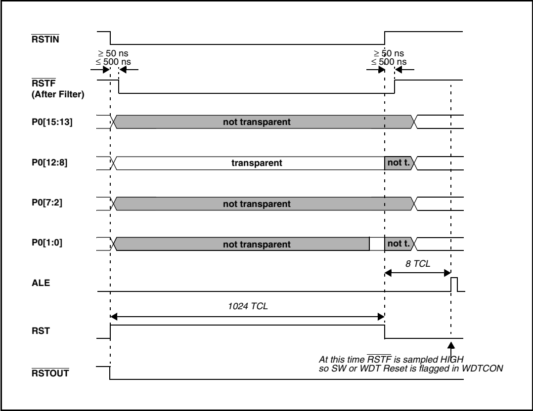
Figure 28. SW / WDT bidirectional RESET ( \overline{EA} = 0 )
