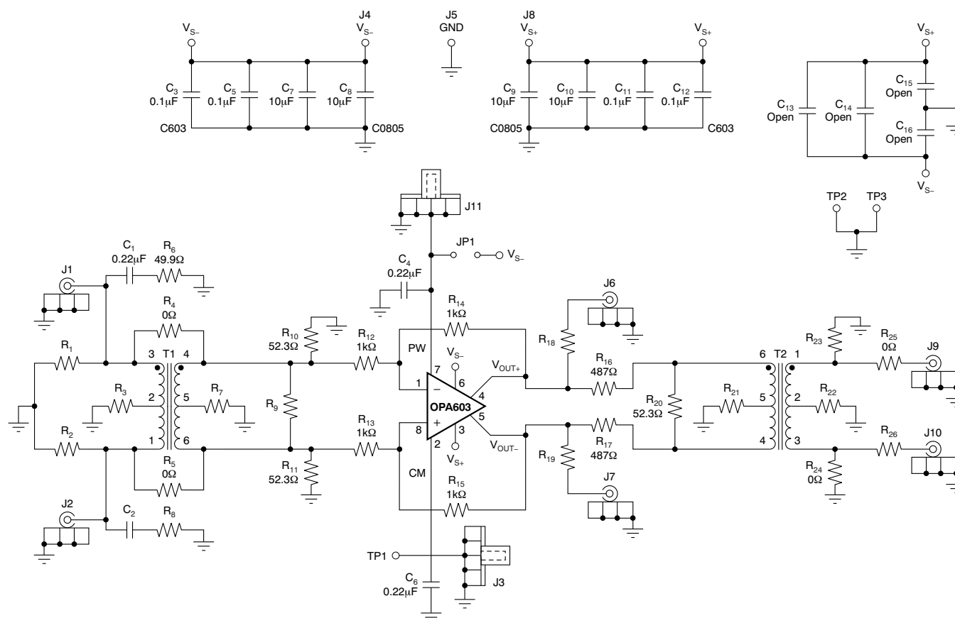
Figure 77. THS4521EVM: Schematic
