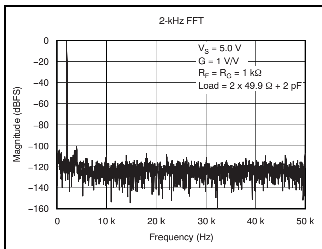
Figure 75. 2-kHz FFT
