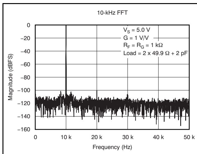
Figure 76. 10-kHz FFT
