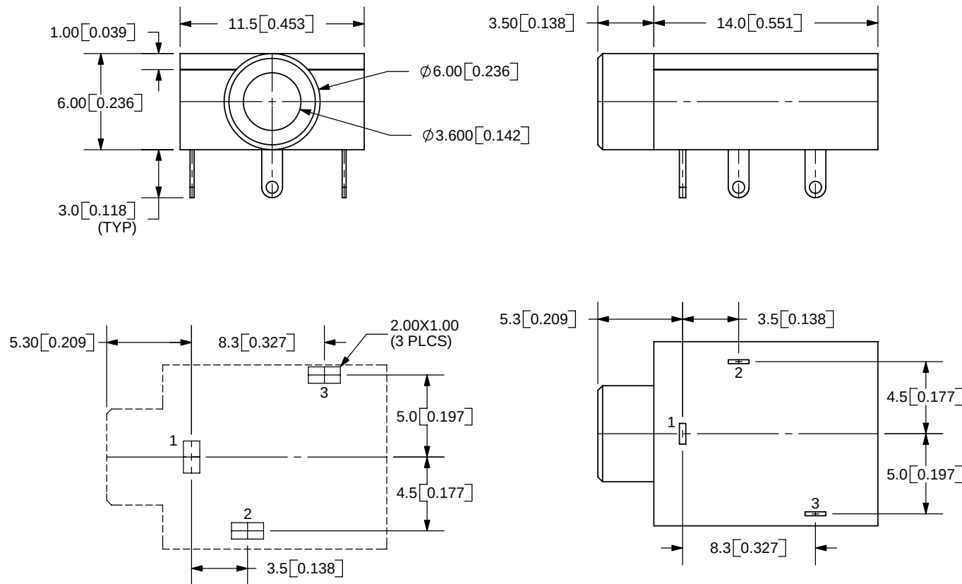
PCB LAYOUT TOP VIEW
