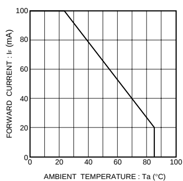
Fig.1 Forward current
