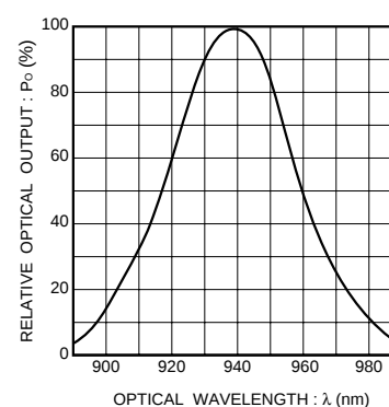
Fig.3 Wavelength
