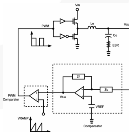
Figure 23. Closed Loop
