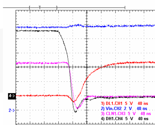
Figure 16. Dead Time with Heavy Load (Fall Edge)
