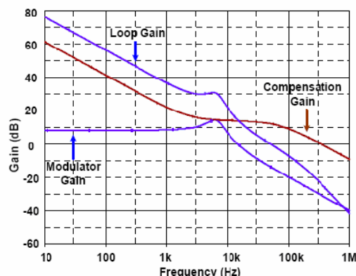
Figure 25. Bode Plot
