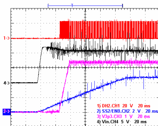
Figure 8. V3p3 Power On with 8A Load
