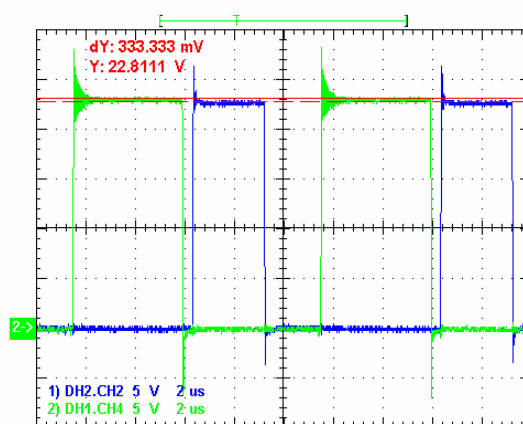
Figure 12. V3p3 & V5p0 Phase Shift with Heavy Load
