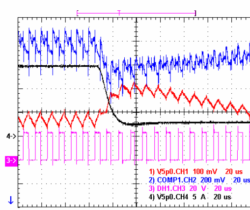
Figure 18. Load Transient Response (Step-Down) 20kΩ/22nF in Compensation Loop
