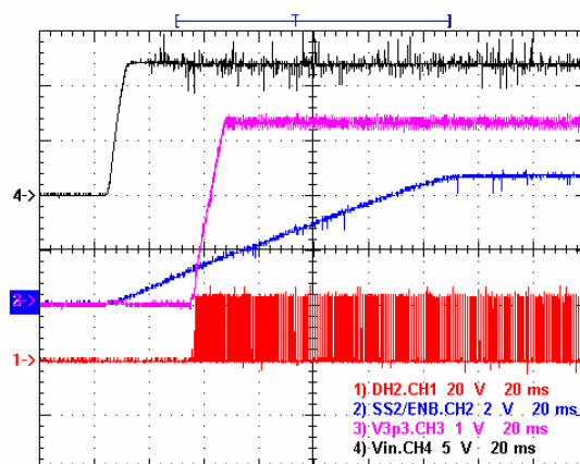
Figure 6. V3p3 Power On with 3A Load
