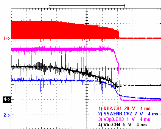
Figure 10. V3p3 Power Off with 8A Load
