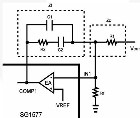
Figure 24. Compensation Loop
