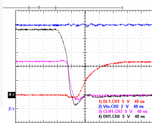
Figure 14. Dead Time with Light Load (Fall Edge)
