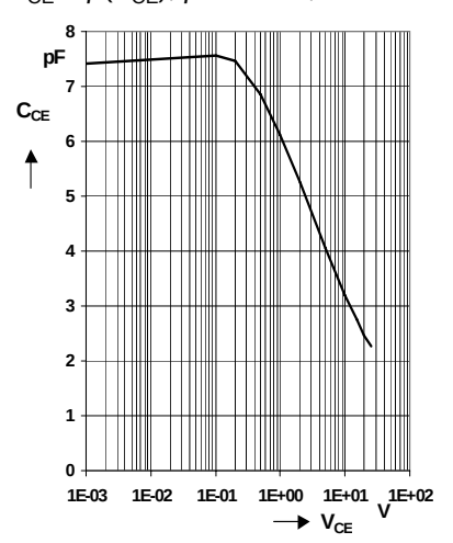
Collector-Emitter Capacitance
