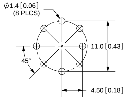
PCB LAYOUT FRONT VIEW
