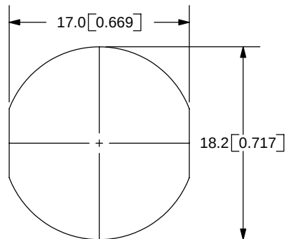
Panel Cutout
