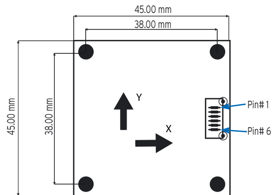
Mechanical dimensions in mm.
