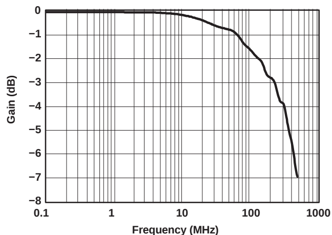
Figure 9. Gain vs Frequency ( V_+ = 5\text{ V} )
