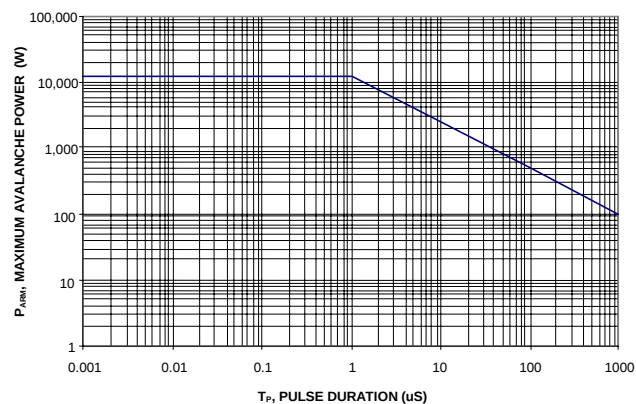
Figure 5: Maximum Avalanche Power Curve, Per Element
