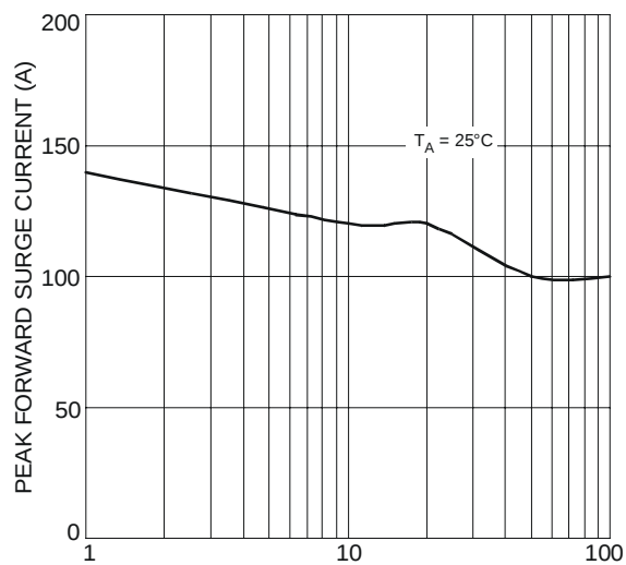
Fig. 7 Maximum Repetitive Surge Current
