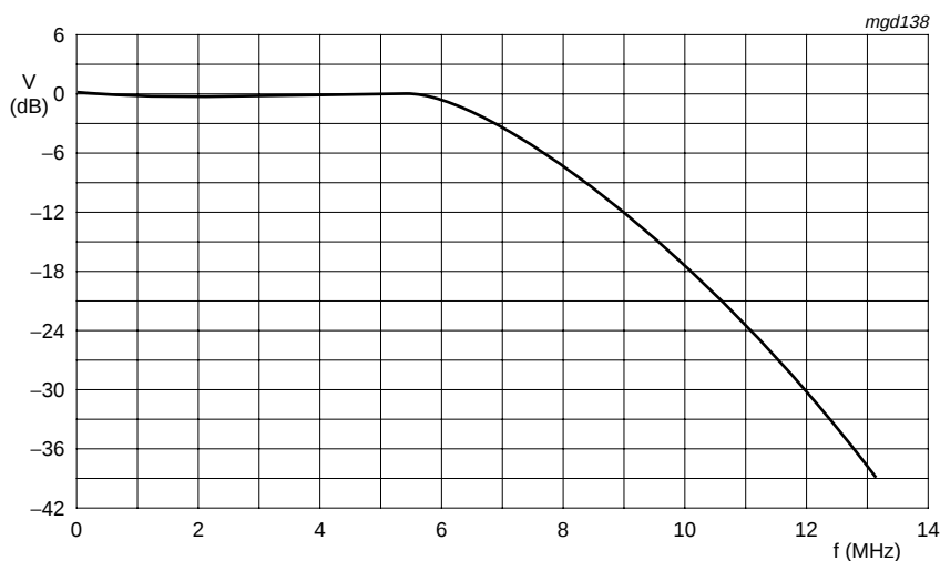
Fig 4. Anti-alias filter
