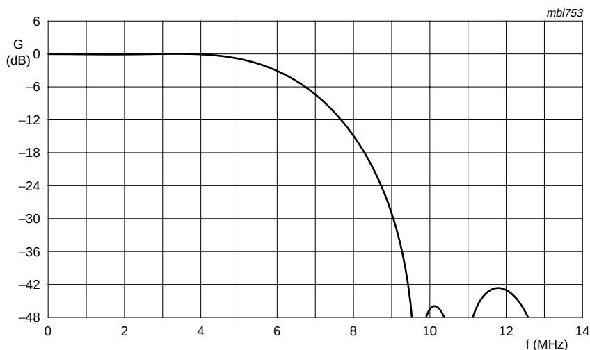
Fig 5. Decimation filter
