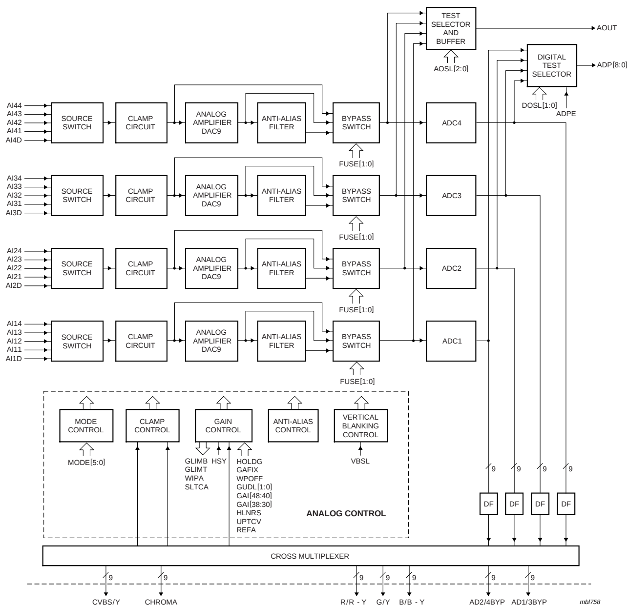
Fig 6. Analog input processing using the SAA7118 as differential front-end with 9-bit ADC
