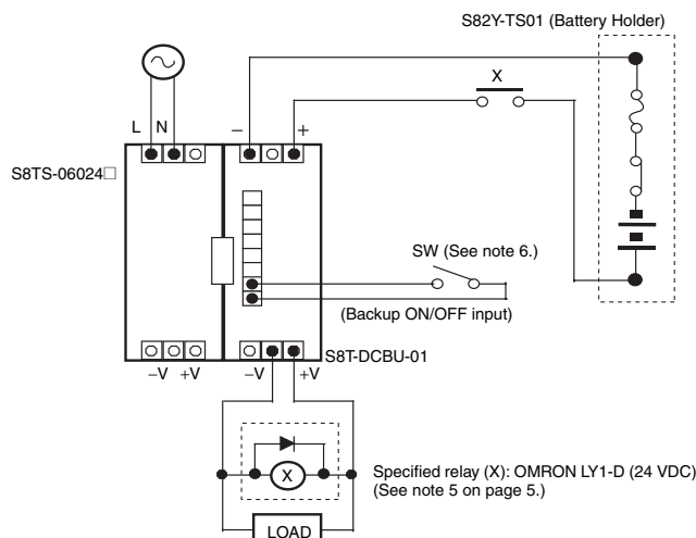
Figure 2 Overdischarge Protection Circuit Using an External Signal
