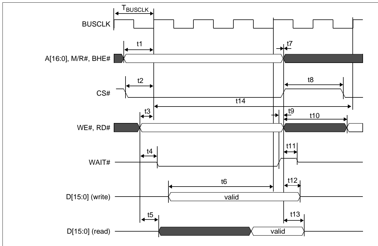
Figure 6-3: Generic #2 Interface Timing
