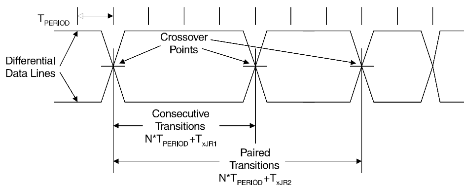
Figure 6-35 Differential Data Jitter
