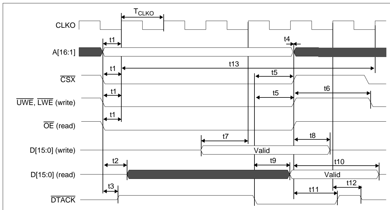
Figure 6-9: Motorola Dragonball Interface Timing with \overline{DTACK}
