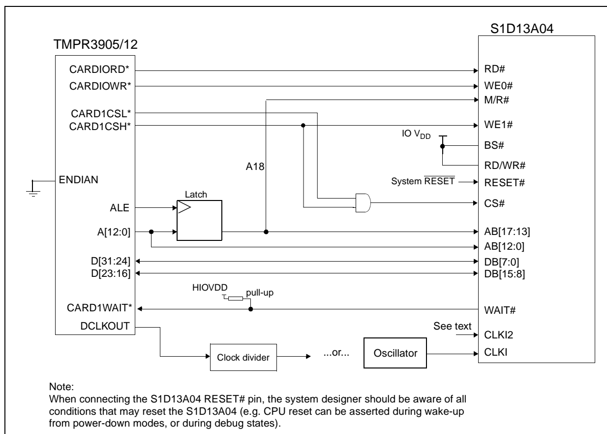
Figure 4-1: S1D13A04 to TMPR3905/12 Direct Connection
