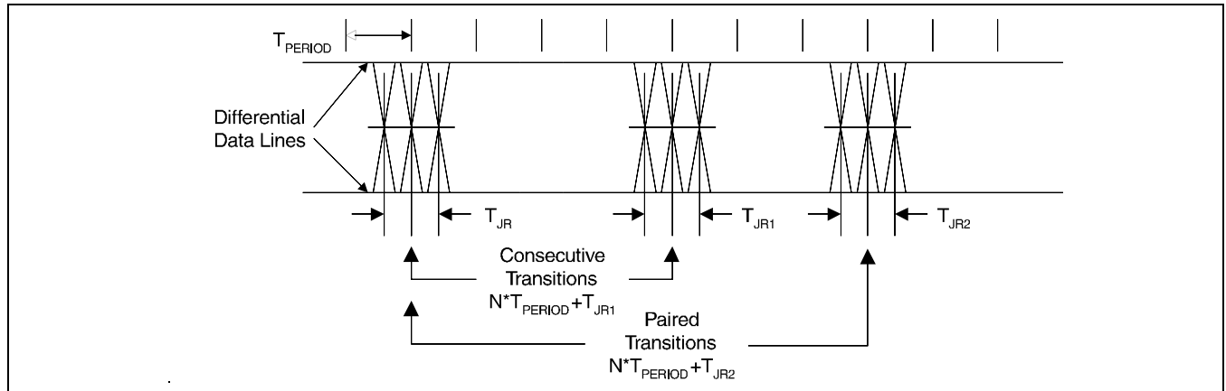
Figure 6-37 Receiver Jitter Tolerance
