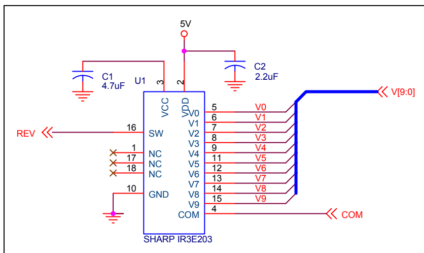
Figure 3-1: Sharp LQ031B1DDxx Gray Scale Voltage (V0-V9) Generation
