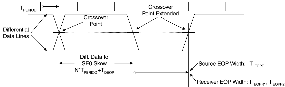
Figure 6-36 Differential to EOP Transition Skew and EOP Width
