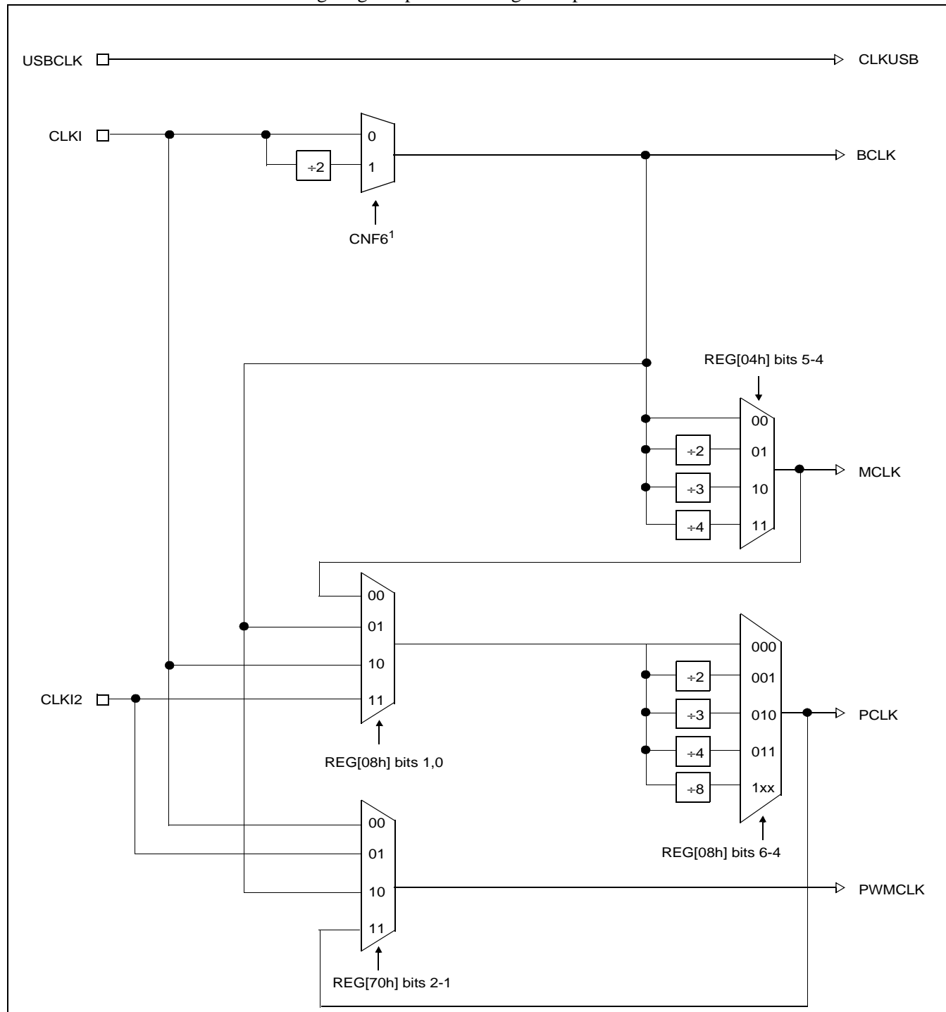
Figure 7-1: Clock Selection
