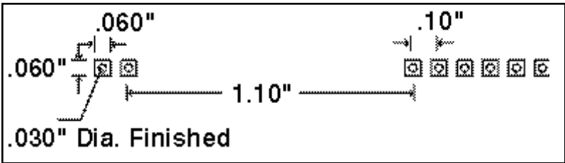
Figure 7: Recommended pad layout
