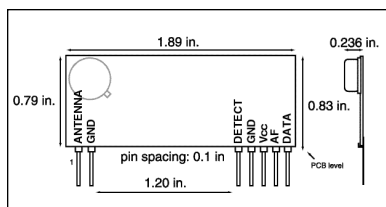
Package Outline
