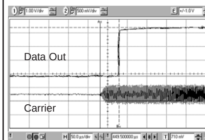
Figure 5: RF in vs. Receiver Response Time
