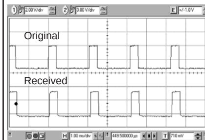
Figure 7: Original vs. Received Data 4,800bps 20% Duty Cycle
