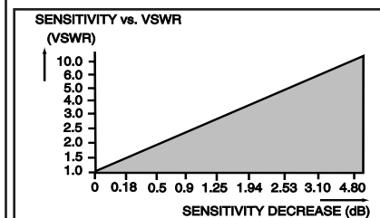
Figure 3: Sensitivity vs. VSWR
