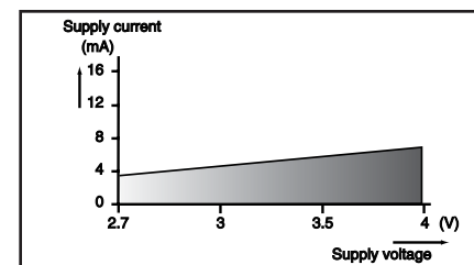
Figure 4: Consumption vs. Supply Voltage
