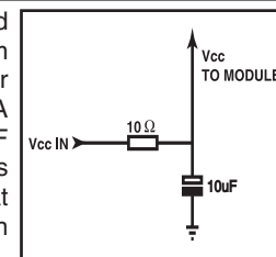
Figure 15: Supply Filter
