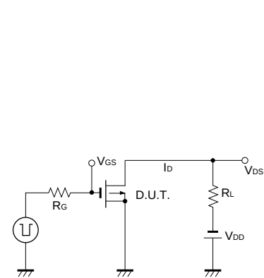
Fig.10 Switching Time Test Circuit
