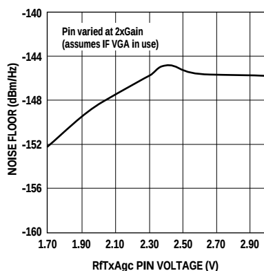
Figure 14. CDMA Driver RX Band Noise Floor vs. V(RfTxAgc).
