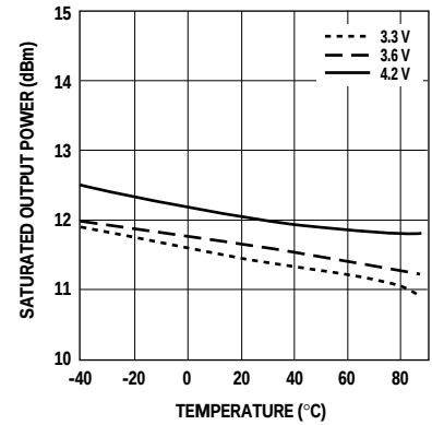
Figure 21. AMPS Driver Output 3 dB Compression Power vs. Temperature and VccBat.
