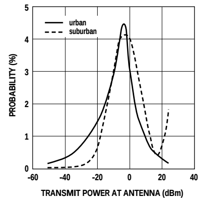
Figure 34. Probability Distribution of Mobile Transmit Power.
