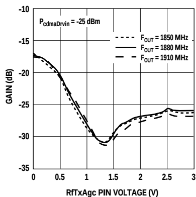
Figure 10. CDMA Driver Isolation (Output 2 to Output 1) vs. V(RfTxAgc) and Frequency.
