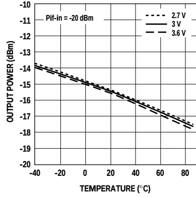
Figure 2. CDMA Upconverter Output Power vs. Temperature and Vcc.
