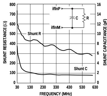
Figure 30. IF Input Port Equivalent Circuit (AMPS Mode) vs. Frequency.
