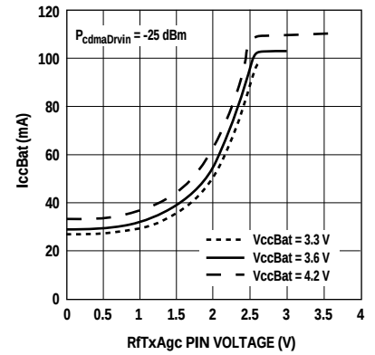
Figure 6. CDMA Driver IccBat vs. V(RfTxAgc) and VccBat.
