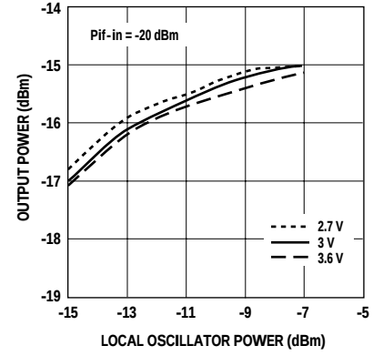
Figure 3. CDMA Upconverter Output Power vs. LO Power and Vcc.
