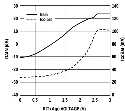
Figure 35. HPMX-7201 RF VGA Gain and Supply Current Consumption vs. RfTxAgc Voltage.
