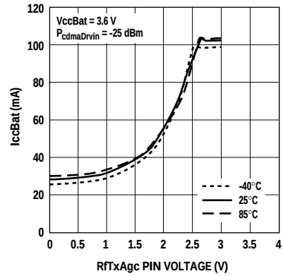
Figure 7. CDMA Driver IccBat vs. V(RfTxAgc) and Temperature.
