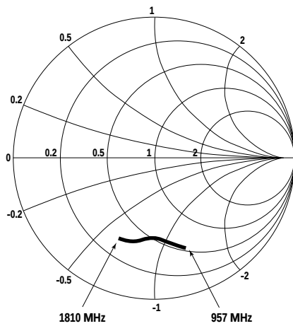
Figure 22. LO Port Input Impedance vs. Frequency.
