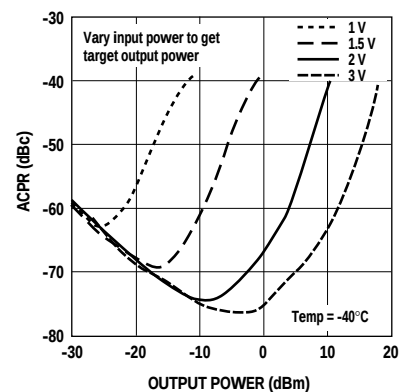
Figure 12. CDMA Driver ACPR vs. Output Power and V(RfTxAgc).
