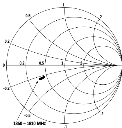
Figure 26. cdmaDrvOut Output Impedance vs. Frequency.
