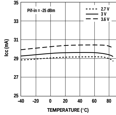
Figure 1. CDMA Upconverter Icc vs. Vcc and Temperature.
