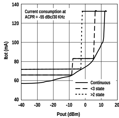
Figure 36. HPMX-7201 Total Current Consumption vs. Output Power and Control Method.
