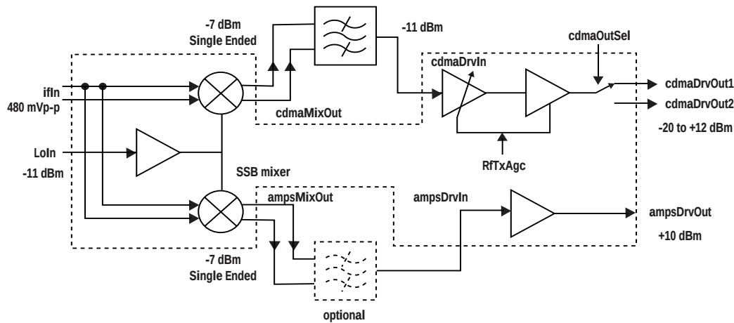
Figure 33. Expected Power and Voltage Levels.
