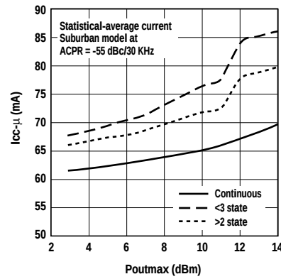
Figure 37. HPMX-7201 Statistical-Average Current Consumption vs. Desired Maximum Output Power.
