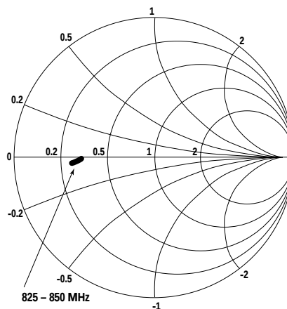
Figure 27. ampsDrvIn Input Impedance vs. Frequency.
