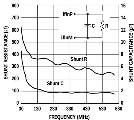
Figure 29. IF Input Port Equivalent Circuit (CDMA Mode) vs. Frequency.
