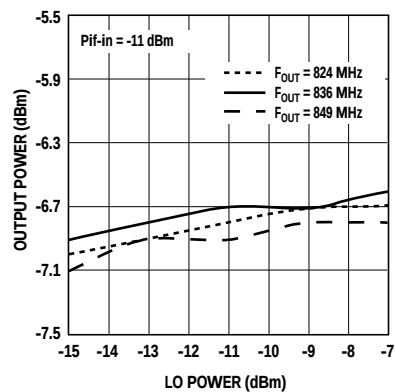
Figure 17. AMPS Upconverter Output Power vs. LO Power and Frequency.
