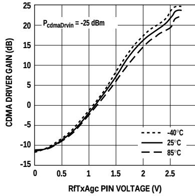
Figure 8. CDMA Driver Gain vs. V(RfTxAgc) and Temperature.
