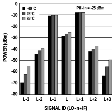
Figure 5. CDMA Upconverter Output Spectrum vs. Temperature.
