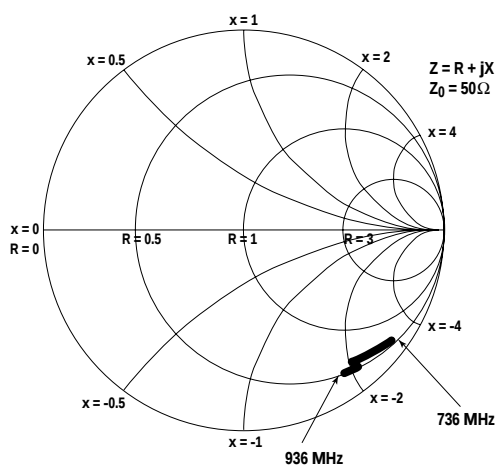
Figure 24. ampsMixOut Output Impedance vs. Frequency.
