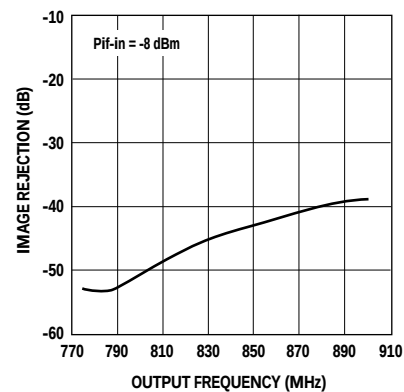
Figure 18. AMPS Upconverter Image Rejection vs. Output Frequency.
