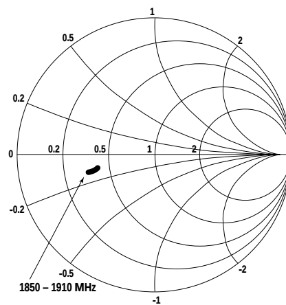
Figure 25. cdmaDrvIn Input Impedance vs. Frequency.
