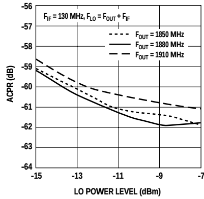
Figure 4. CDMA Upconverter ACPR vs. LO Power and Frequency.
