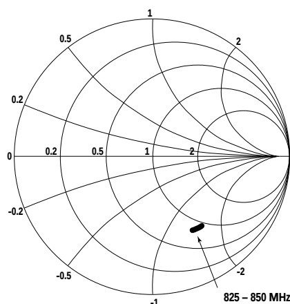
Figure 28. ampsDrvOut Output Impedance vs. Frequency.
