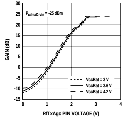
Figure 9. CDMA Driver Gain vs. V(RfTxAgc) and VccBat.
