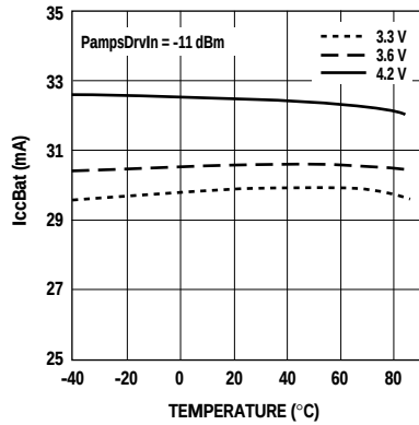
Figure 19. AMPS Driver IccBat vs. Temperature and VccBat.
