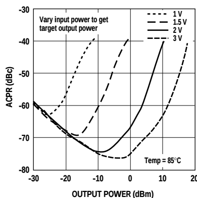
Figure 13. CDMA Driver ACPR vs. Output Power and V(RfTxAgc).
