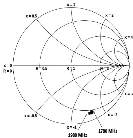
Figure 23. cdmaMixOut Output Impedance vs. Frequency.
