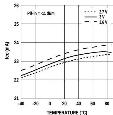
Figure 15. AMPS Upconverter Icc vs. Temperature and Vcc.
