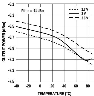
Figure 16. AMPS Upconverter Output Power vs. Temperature and Vcc.
