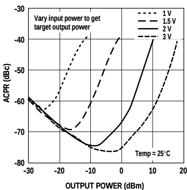
Figure 11. CDMA Driver ACPR vs. Output Power and V(RfTxAgc).
