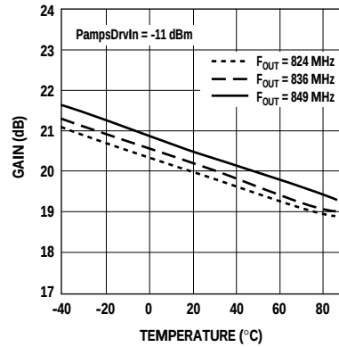
Figure 20. AMPS Driver Gain vs. Temperature and Frequency.
