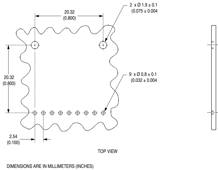
Figure 6. Recommended Board Layout Pattern
