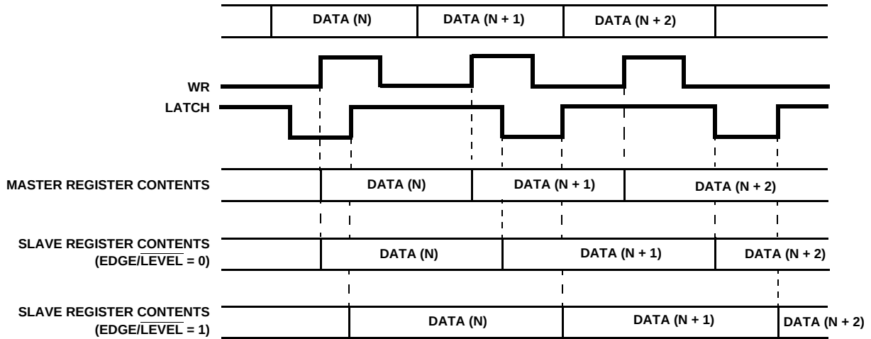
FIGURE 4. PARALLEL PROGRAMMING MODE OPERATION ( \text{SER}/\overline{\text{PAR}} = 0 )
