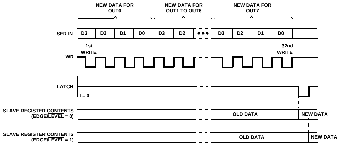
FIGURE 5. SERIAL PROGRAMMING MODE OPERATION ( \text{SER}/\overline{\text{PAR}} = 1 )
