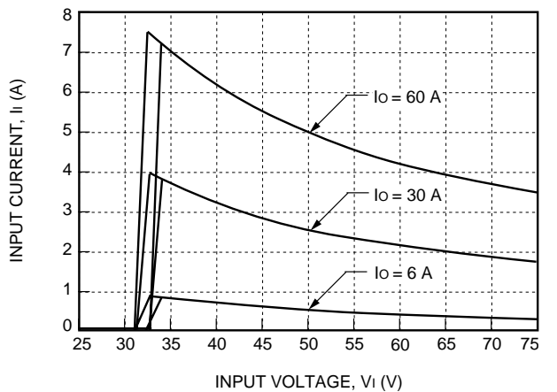
Figure 2. Typical FW300F1 Input Characteristics at Room Temperature
