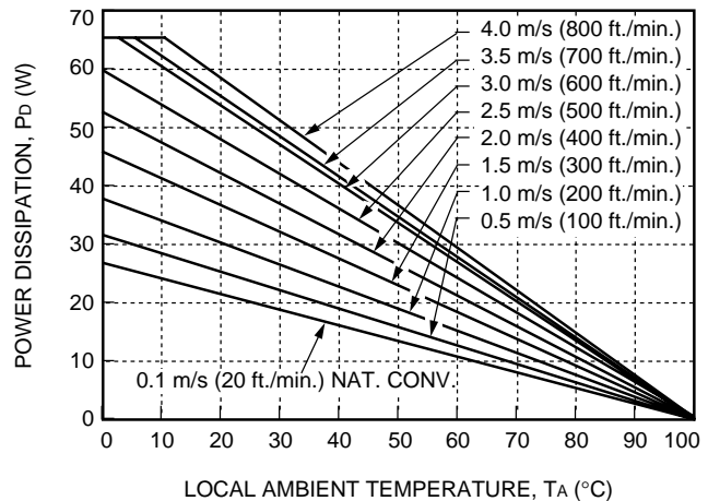
Figure 25. Convection Power Derating with No Heat Sink; Airflow Along Width (Transverse)
