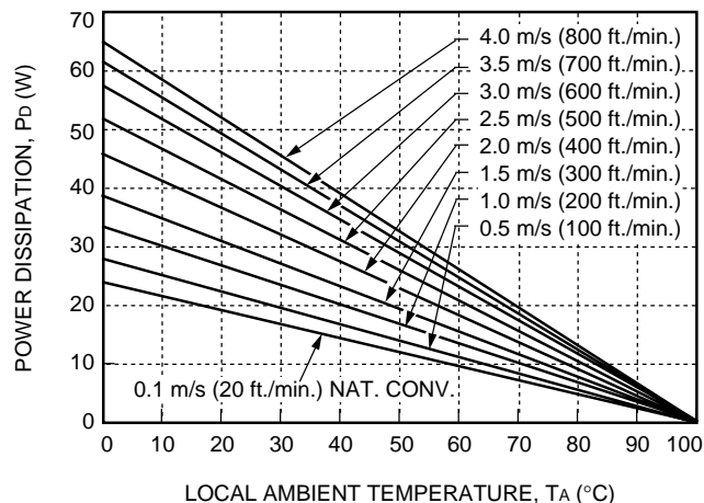
Figure 26. Convection Power Derating with No Heat Sink; Airflow Along Length (Longitudinal)
