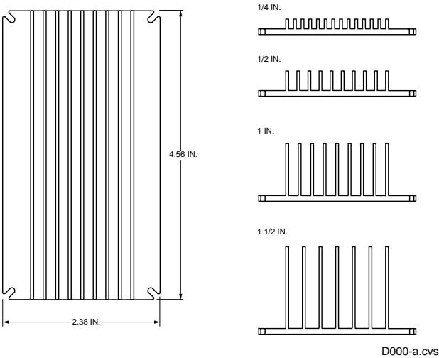
Figure 31. Longitudinal Heat Sink
