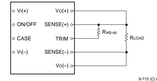
Figure 21. Circuit Configuration to Increase Output Voltage
