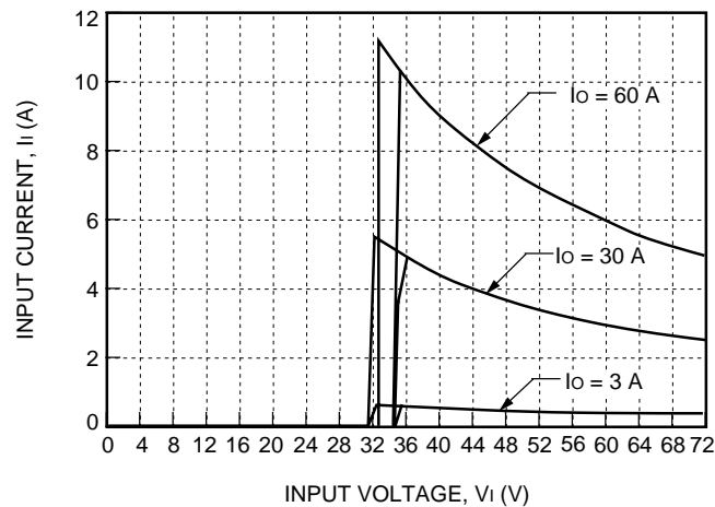
Figure 2. Typical FW300A1 Input Characteristics at Room Temperature
