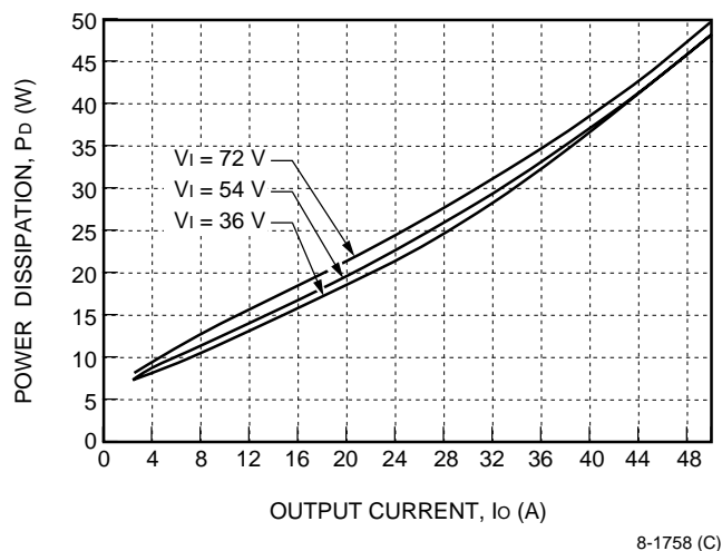
Figure 29. FW250A1 Power Dissipation vs. Output Current at 25 °C
