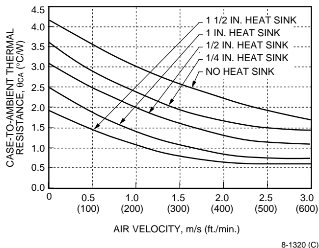
Figure 28. Case-to-Ambient Thermal Resistance Curves; Longitudinal Orientation
