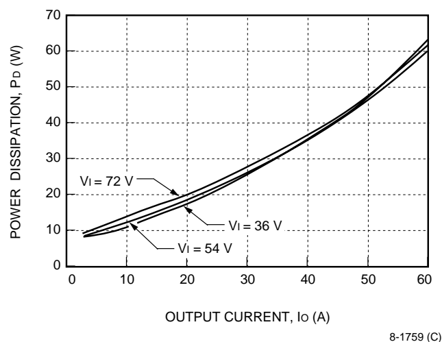
Figure 30. FW300A1 Power Dissipation vs. Output Current at 25 °C
