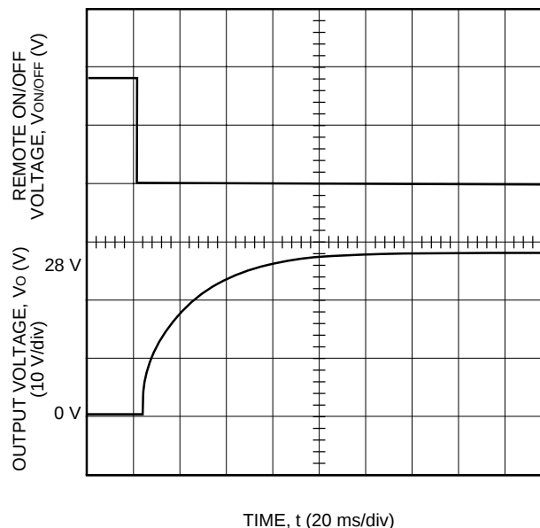
Figure 7. Typical FC250R Start-Up Transient at Room Temperature, 28 V Input, and Full Load
