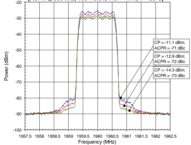
RF2484 Output Channel Power vs I, Q Input Voltage Level (Vcc = 5.0V, Vref = 4.1V, T = 25°C, CDMA/W-CDMA Mod.)
