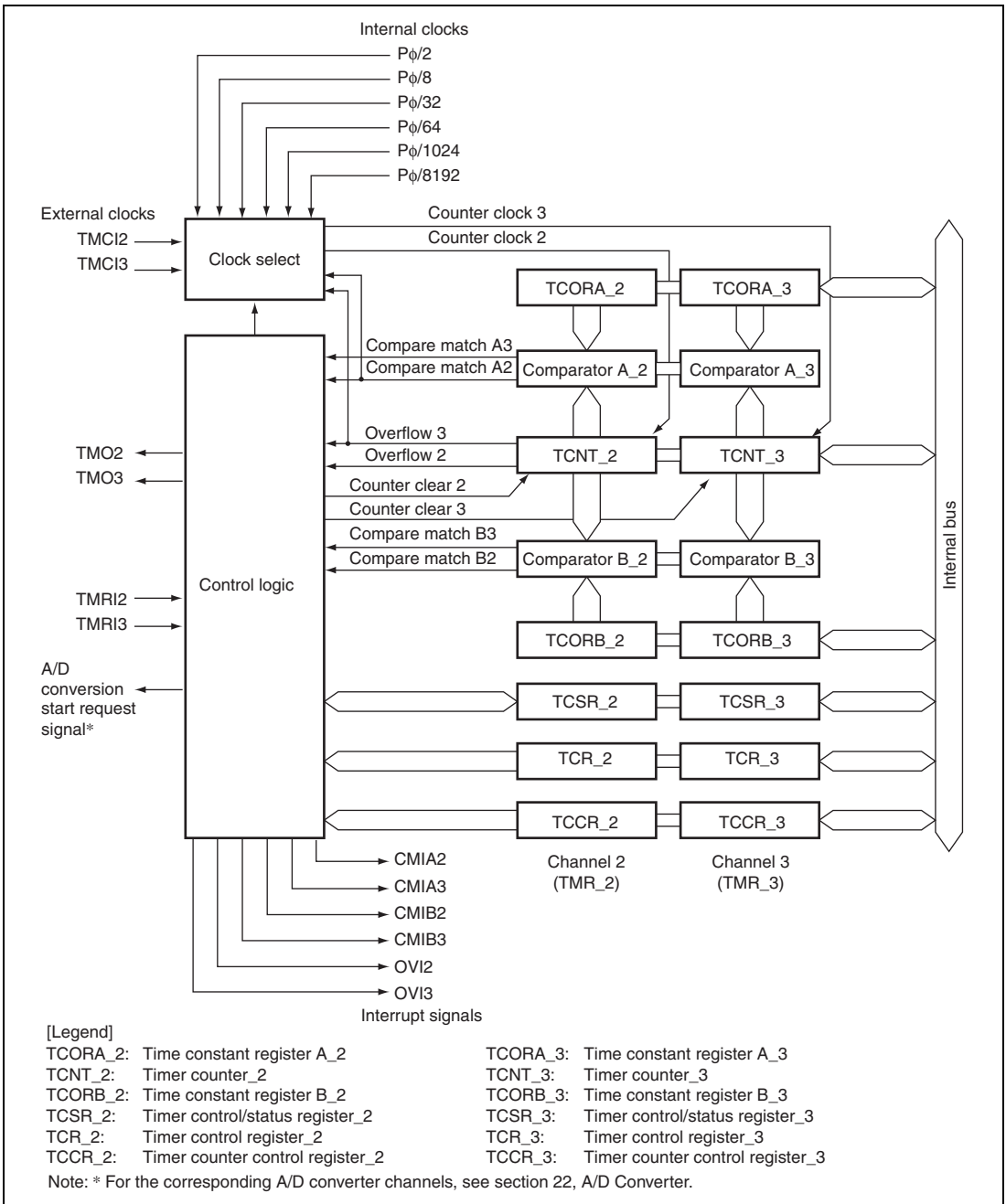
Figure 16.2 Block Diagram of 8-Bit Timer Module (Unit 1)
