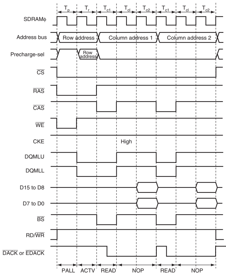
Figure 9.84 Output Timing Example of \overline{DACK} and \overline{EDACK} when DDS = 1 or EDDS = 1 (Read, CAS Latency = 2)
