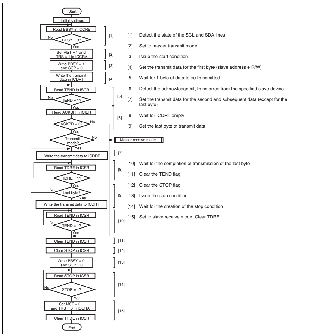
Figure 21.14 Sample Flowchart of Master Transmit Mode
