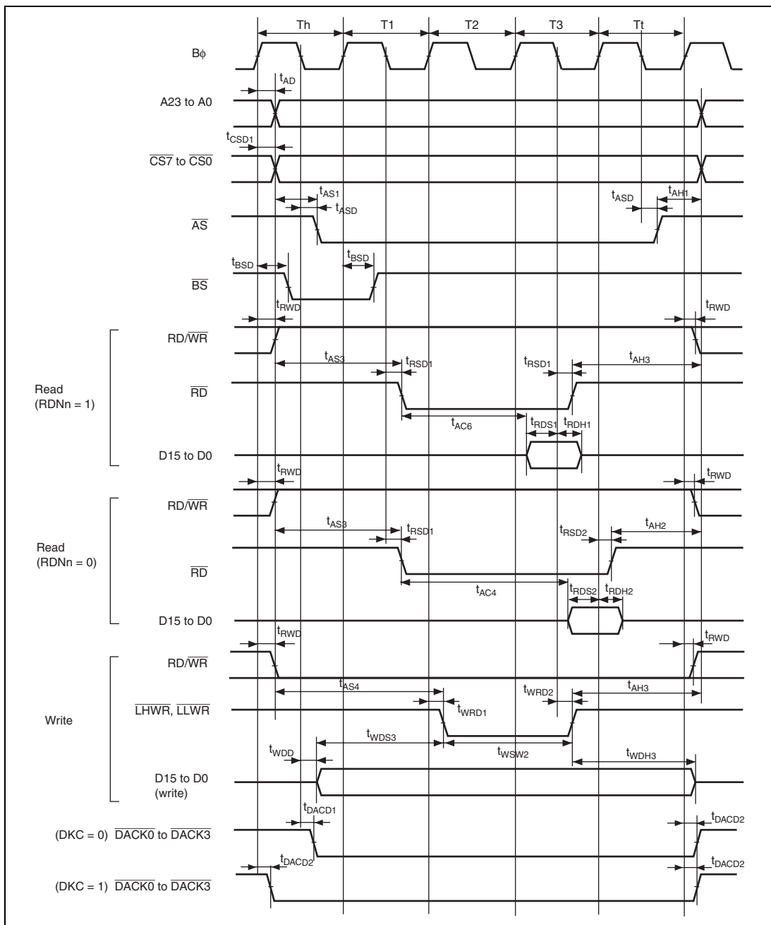
Figure 30.12 Basic Bus Timing: Three-State Access (CS Assertion Period Extended)
