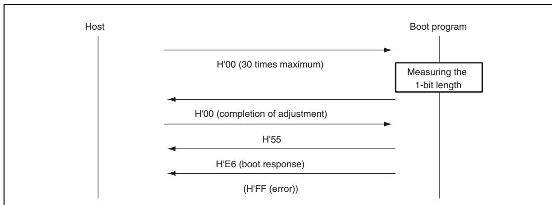
Figure 25.24 Bit-Rate-Adjustment Sequence
