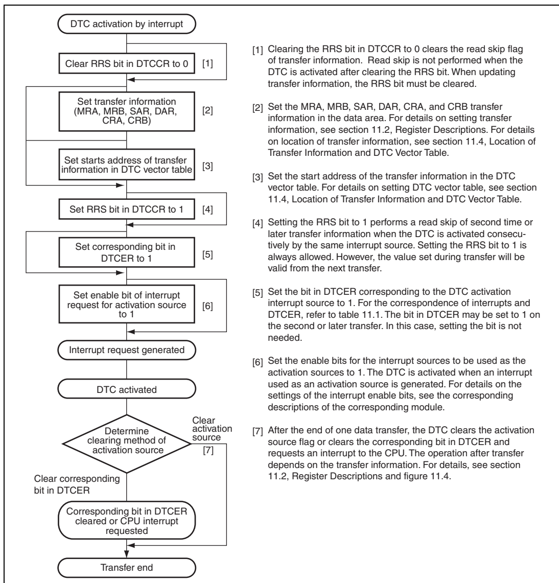
Figure 11.15 DTC with Interrupt Activation
