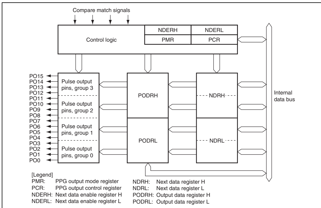
Figure 14.1 Block Diagram of PPG (Unit 0)
