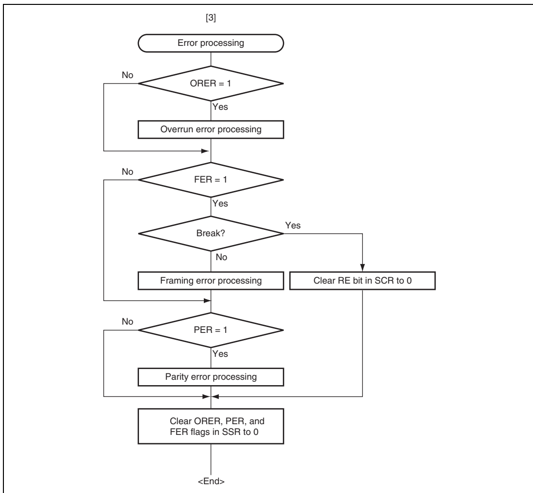
Figure 17.12 Sample Serial Reception Flowchart (2)
