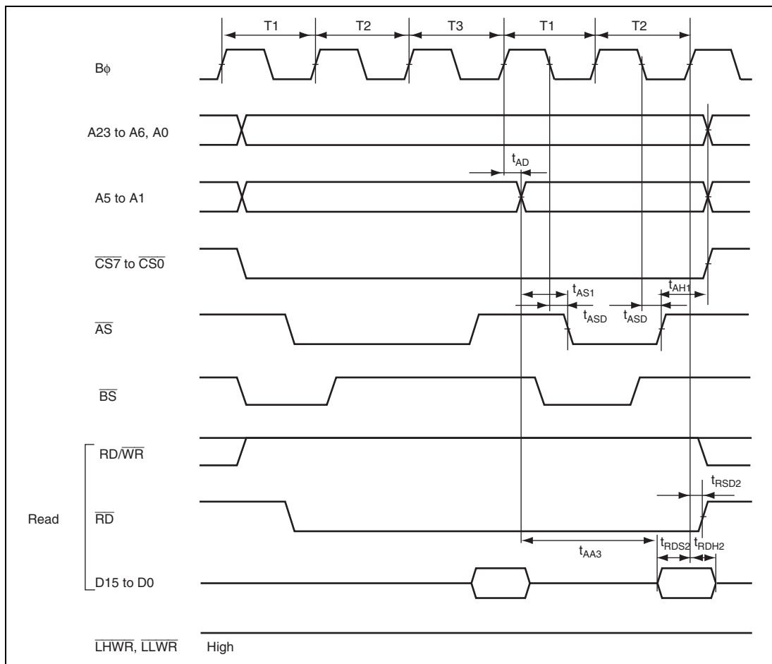
Figure 27.16 Burst ROM Access Timing: Two-State Burst Access
