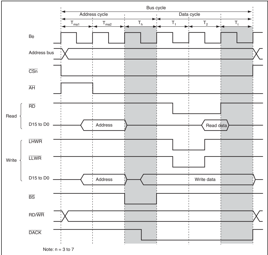
Figure 9.34 Chip Select ( \overline{\text{CS}} ) Assertion Period Extension Timing in Data Cycle
