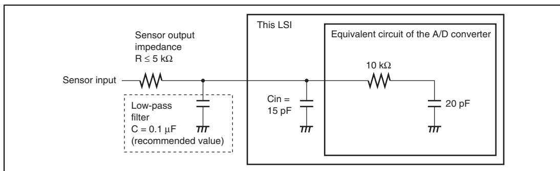
Figure 19.12 Example of Analog Input Circuit
