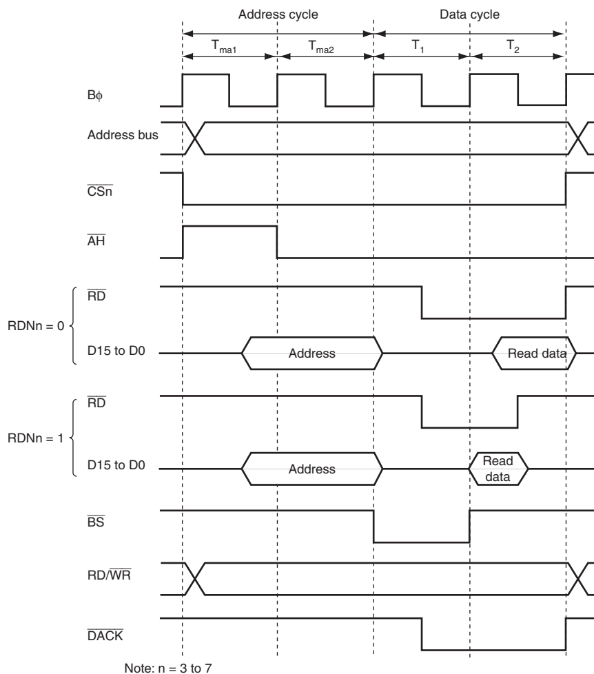
Figure 9.33 Read Strobe Timing
