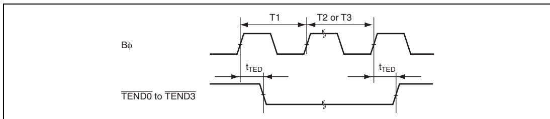
Figure 27.22 DMAC ( \overline{TEND} ) Output Timing
