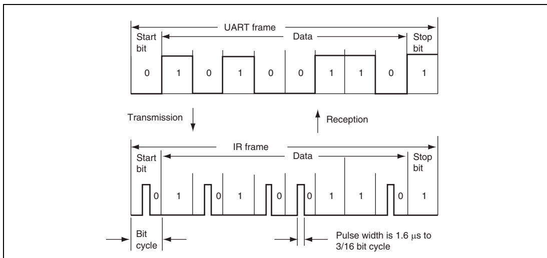
Figure 17.37 IrDA Transmission and Reception
