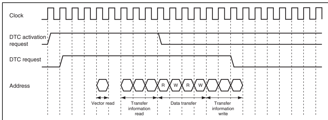
Figure 11.12 DTC Operation Timing (Example of Short Address Mode in Block Transfer Mode with Block Size of 2)
