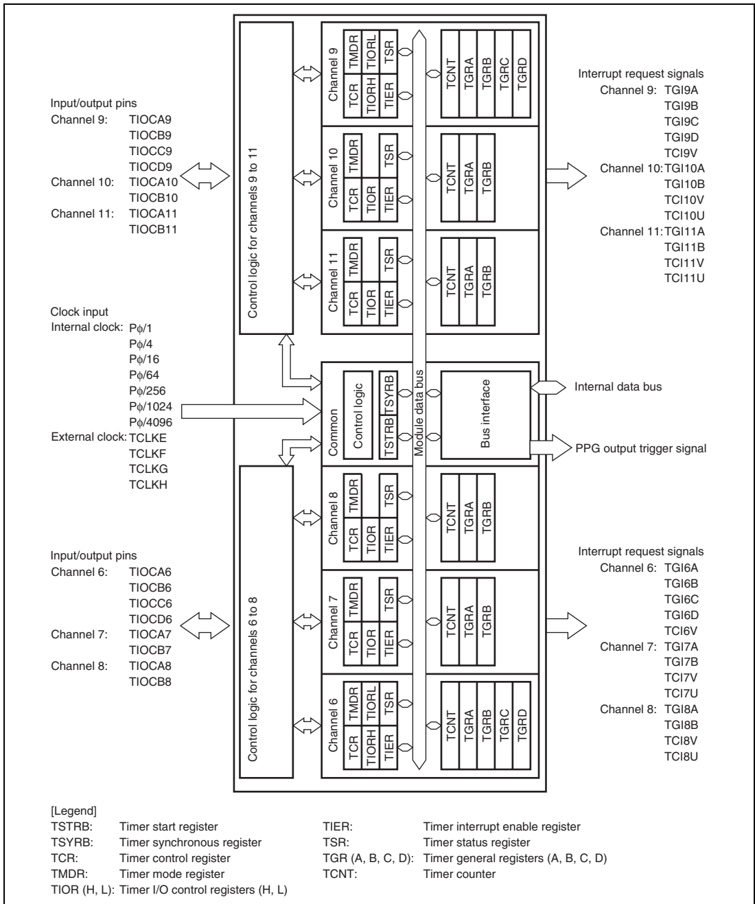
Figure 13.2 Block Diagram of TPU (Unit 1)
