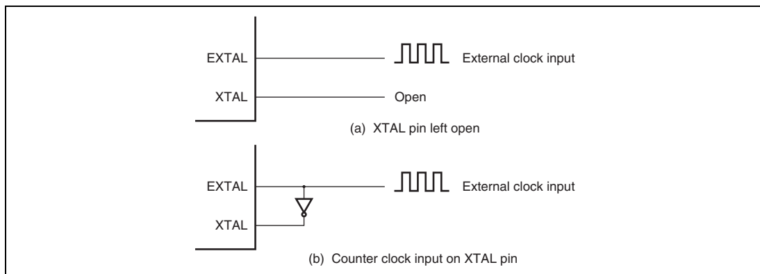
Figure 24.4 External Clock Input (Examples)
