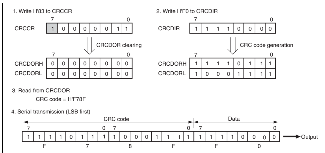
Figure 17.44 LSB-First Data Transmission
