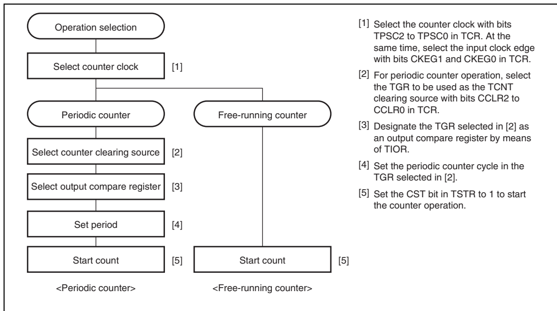
Figure 13.3 Example of Counter Operation Setting Procedure
