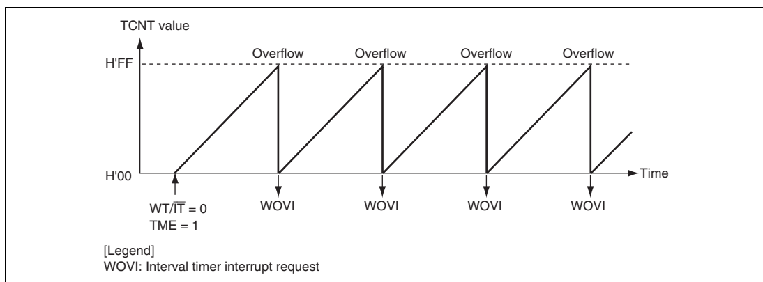
Figure 16.3 Operation in Interval Timer Mode
