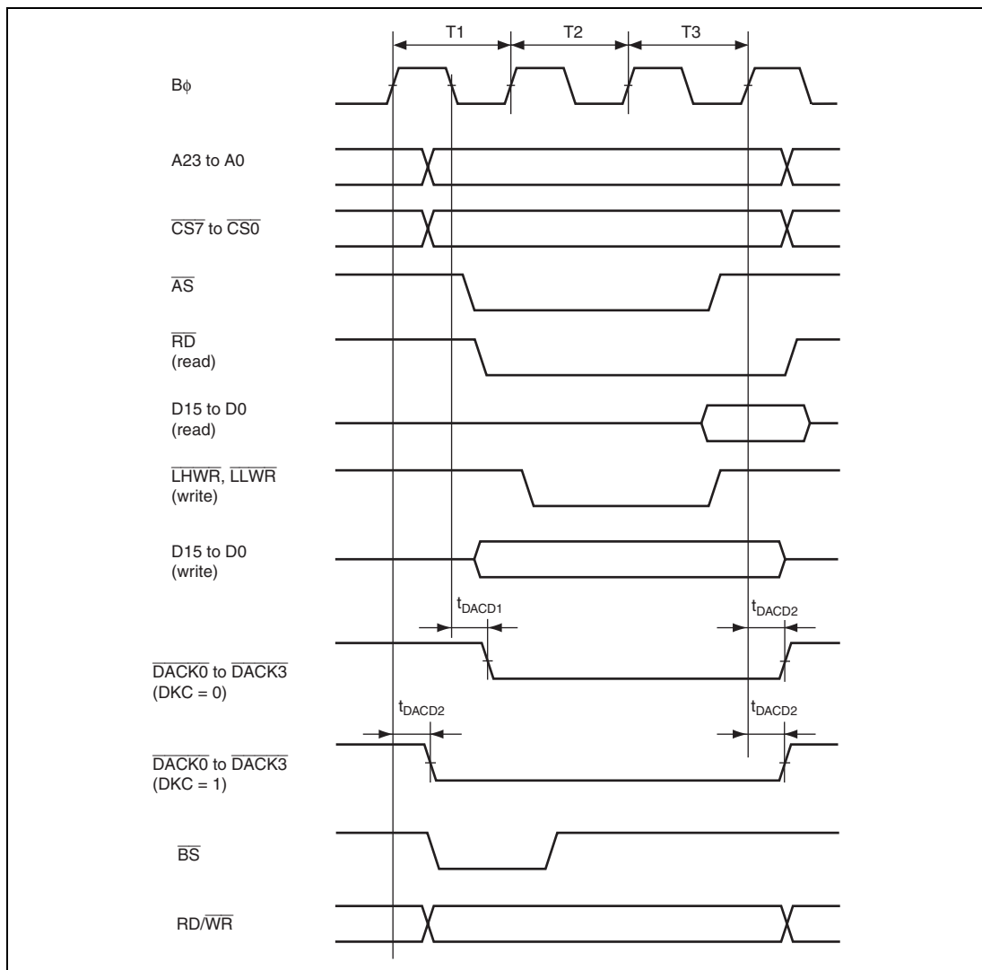
Figure 27.24 DMAC Single-Address Transfer Timing: Three-State Access
