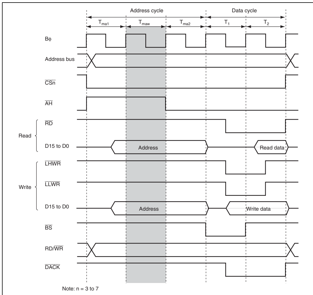
Figure 9.32 Access Timing of 3 Address Cycles (ADDEX = 1)
