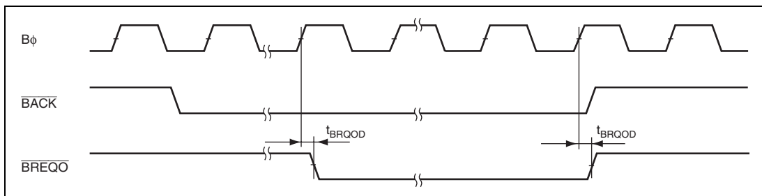
Figure 27.20 External Bus Request Output Timing
