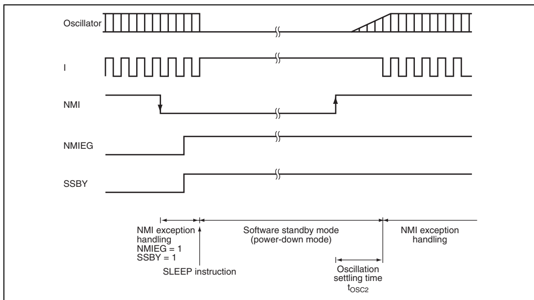
Figure 25.2 Software Standby Mode Application Example
