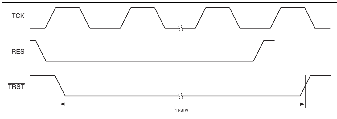
Figure 27.38 Boundary Scan \overline{TRST} Timing
