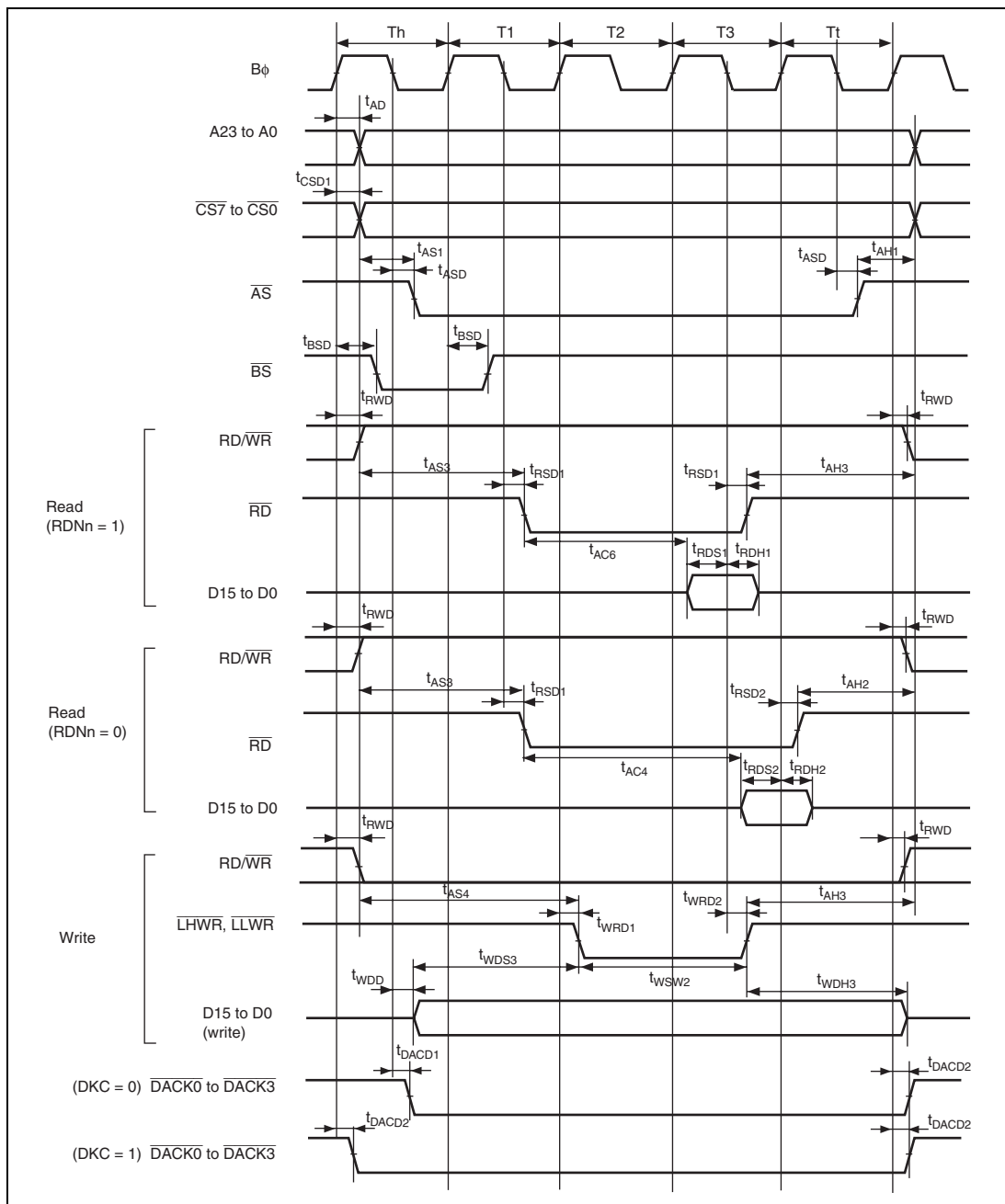
Figure 27.12 Basic Bus Timing: Three-State Access ( \overline{\text{CS}} Assertion Period Extended)
