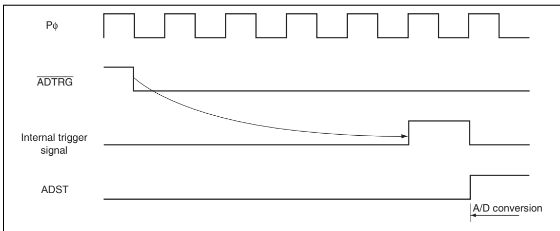
Figure 19.8 External Trigger Input Timing when Multiple Units Start Simultaneously ( \text{TRSG1} , \text{TRGS0} , and \text{EXTRGS} = \text{B}'111 )
