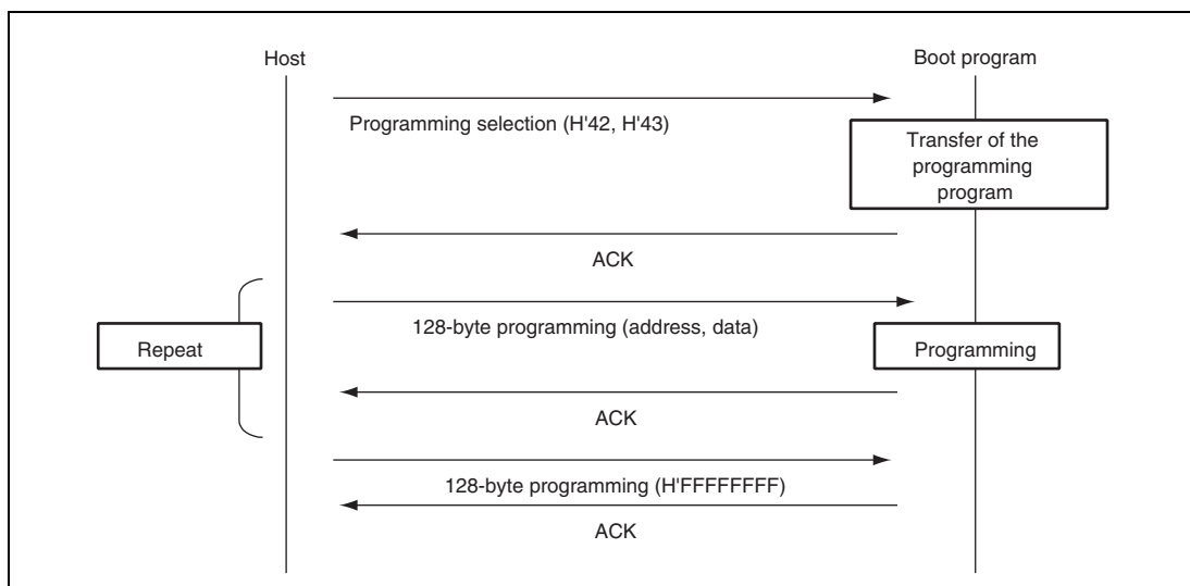
Figure 22.25 Programming Sequence
