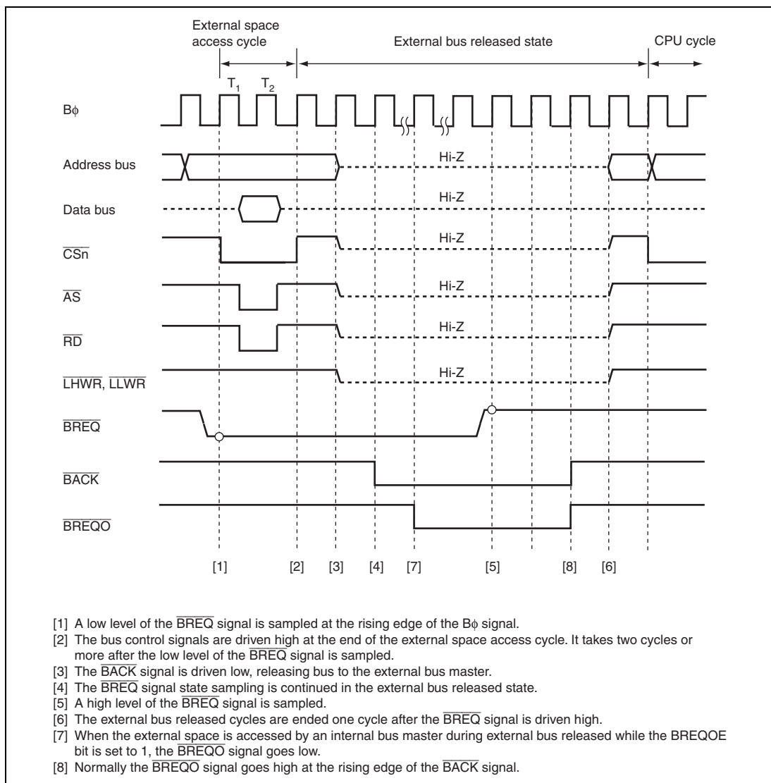
Figure 9.43 Bus Released State Transition Timing
