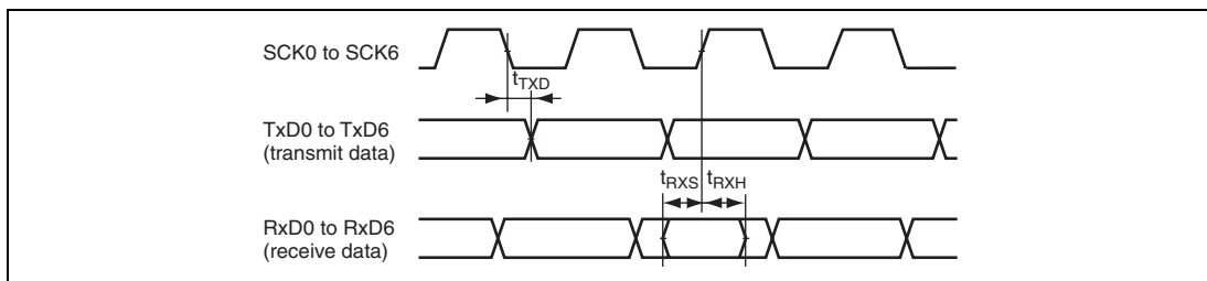
Figure 27.34 SCI Input/Output Timing: Clocked Synchronous Mode
