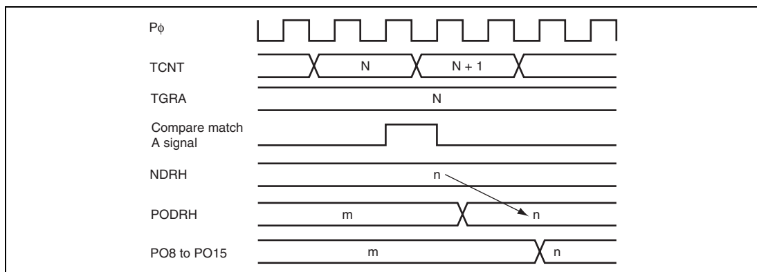
Figure 14.4 Timing of Transfer and Output of NDR Contents (Example)
