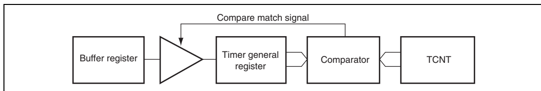
Figure 13.13 Compare Match Buffer Operation
