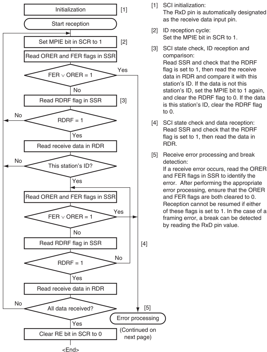
Figure 17.16 Sample Multiprocessor Serial Reception Flowchart (1)
