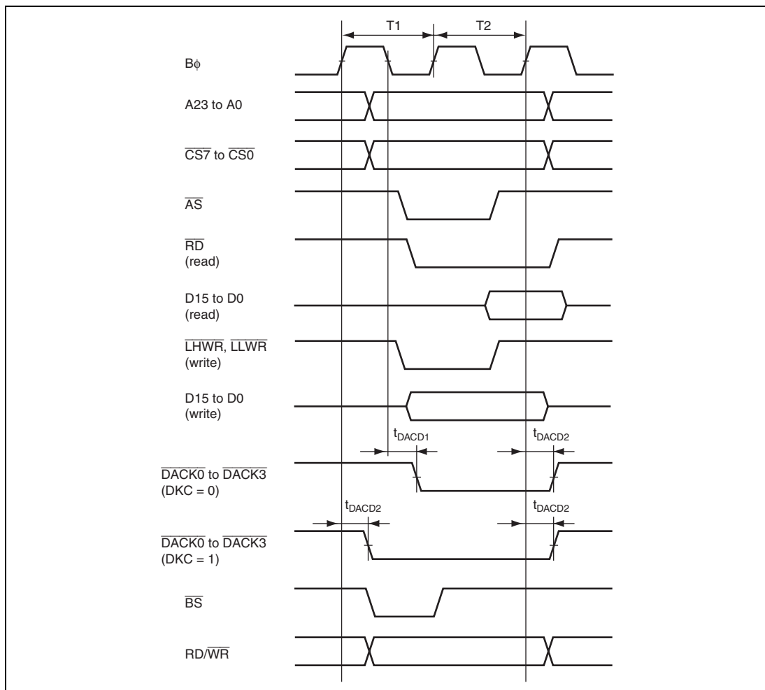
Figure 27.23 DMAC Single-Address Transfer Timing: Two-State Access
