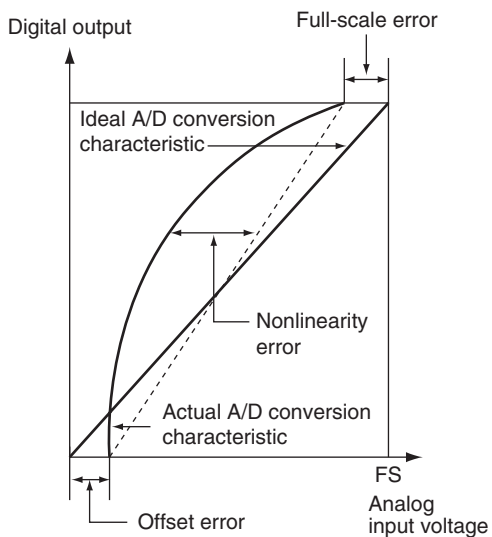
Figure 19.10 A/D Conversion Accuracy Definitions
