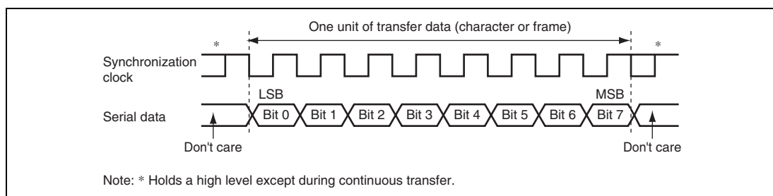
Figure 17.17 Data Format in Clock Synchronous Communication (LSB-First)
