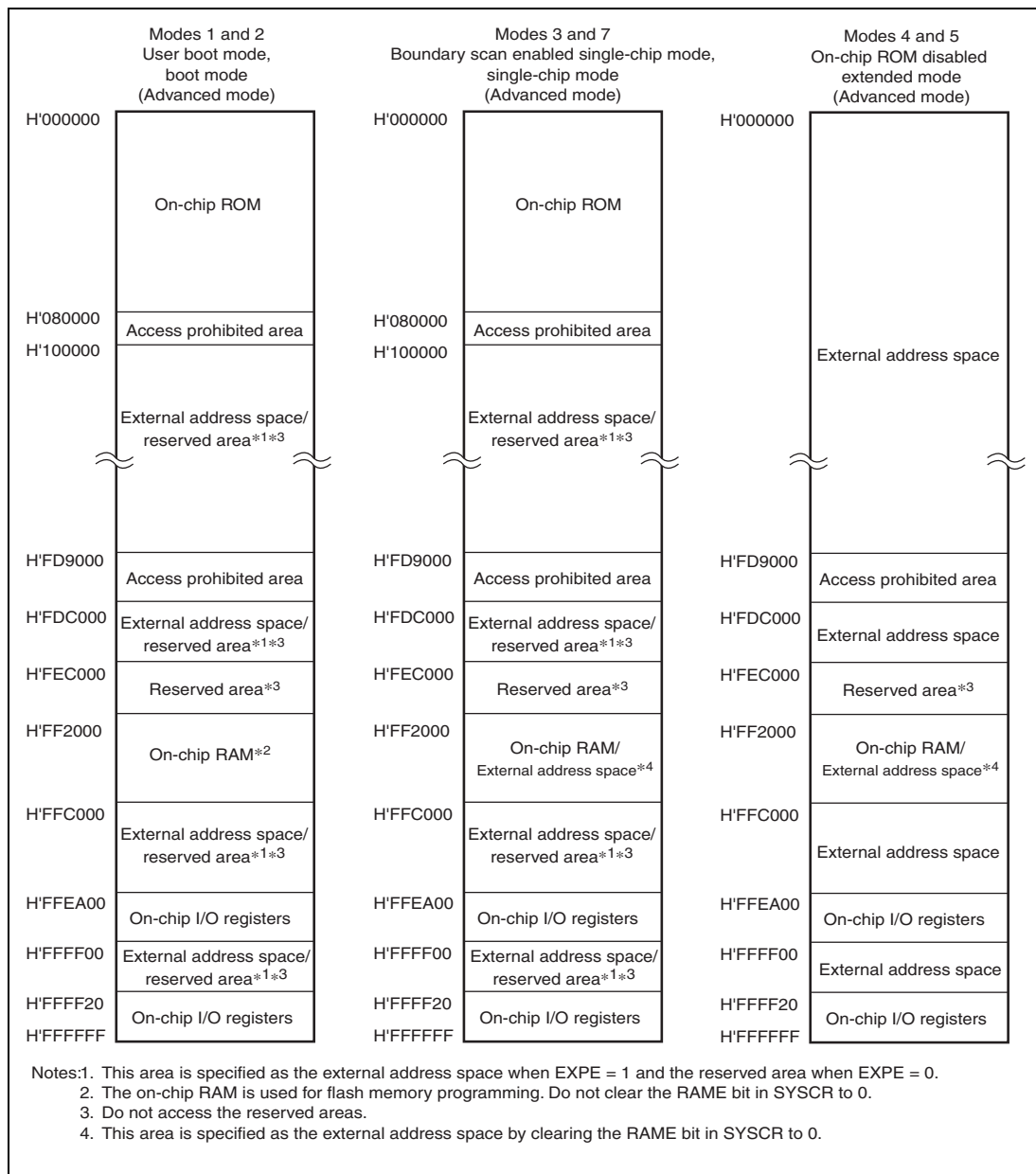
Figure 3.2 Address Map in Each Operating Mode of H8SX/1634 and H8SX/1634L (1)
