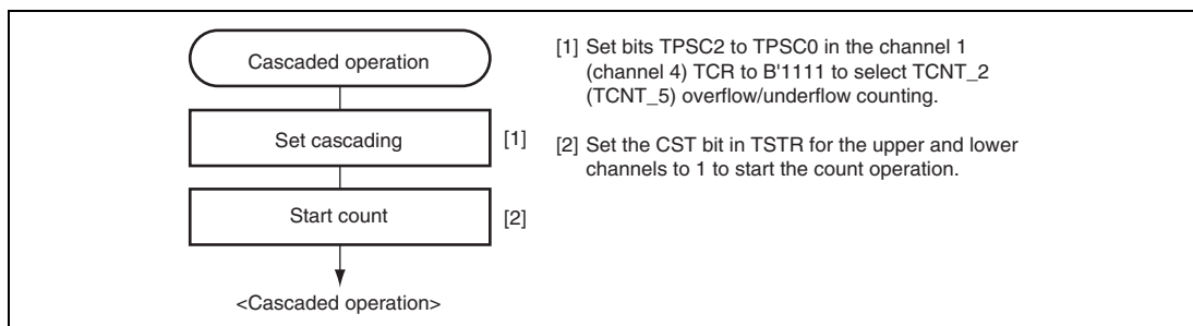
Figure 13.18 Cascaded Operation Setting Procedure
