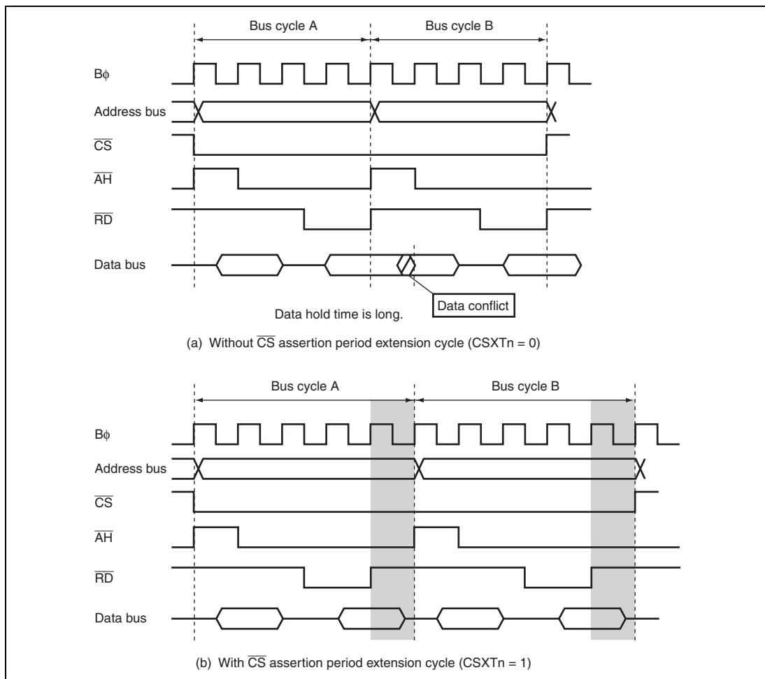
Figure 9.35 Consecutive Read Accesses to Same Area (Address/Data Multiplexed I/O Space)
