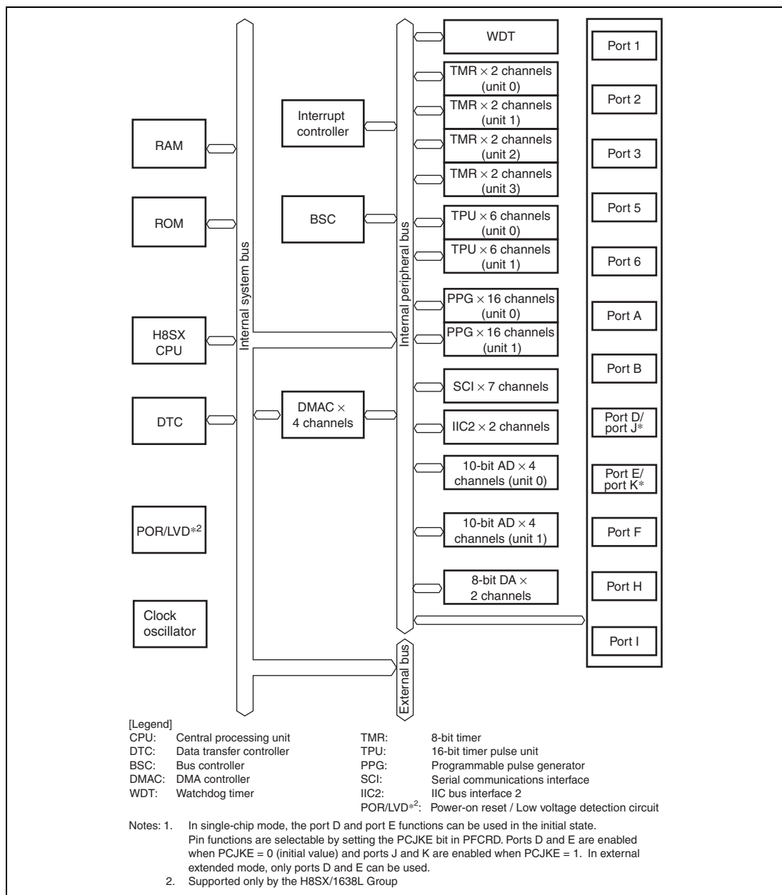
Figure 1.2 Block Diagram
