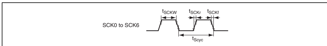
Figure 27.33 SCK Clock Input Timing
