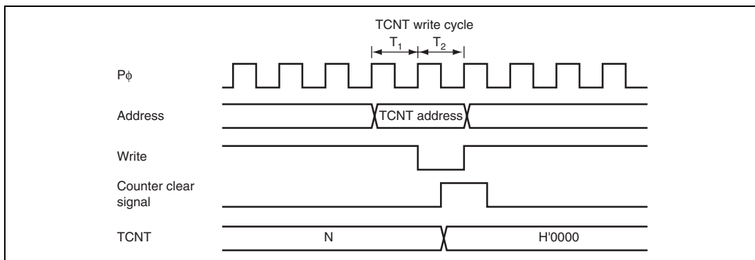
Figure 13.47 Conflict between TCNT Write and Clear Operations
