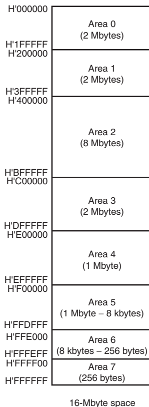
Figure 9.7 Address Space Area Division
