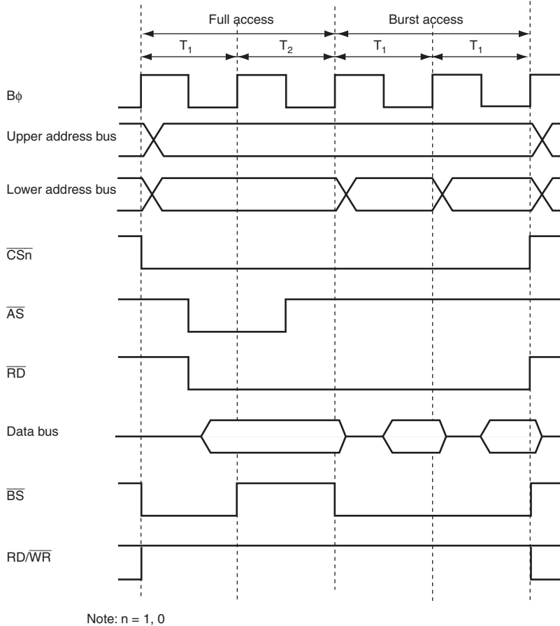
Figure 9.29 Example of Burst ROM Access Timing ( ASTn = 0 , One Burst Cycle)
