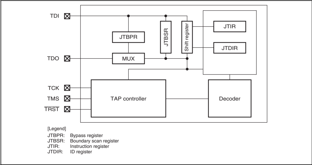
Figure 23.1 Block Diagram of Boundary Scan Function
