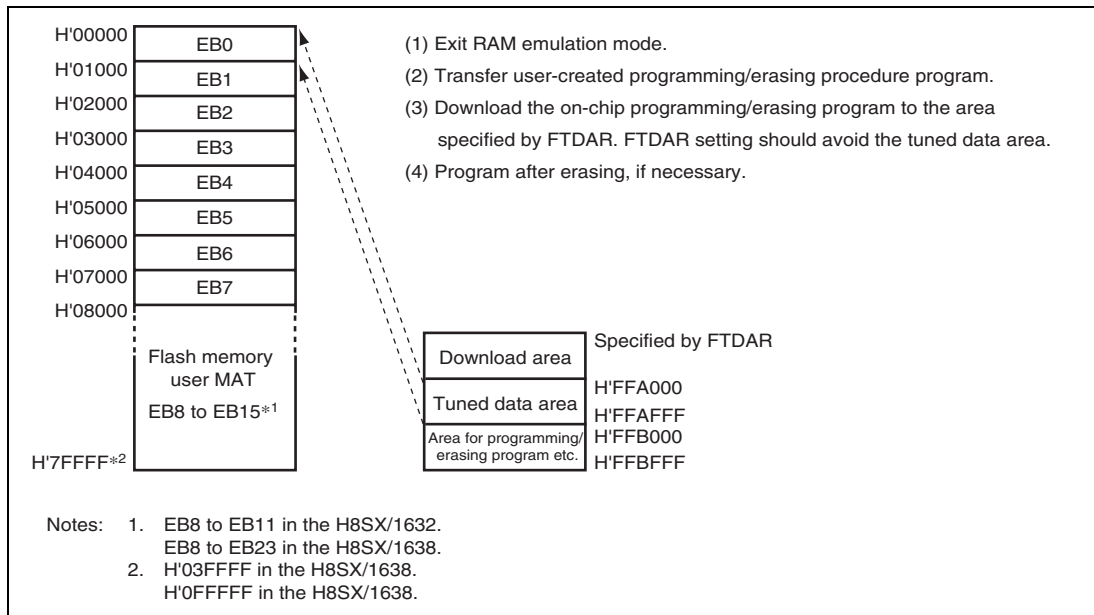
Figure 22.19 Programming Tuned Data (H8SX/1634)
