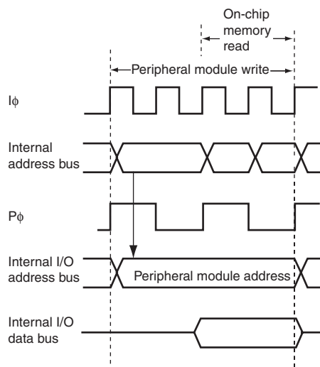
Figure 9.45 Example of Timing when Peripheral Module Write Data Buffer Function is Used
