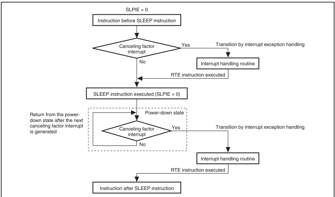
Figure 25.11 When Canceling Factor Interrupt is Generated before SLEEP Instruction Execution (Sleep Instruction Exception Handling Not Initiated)
