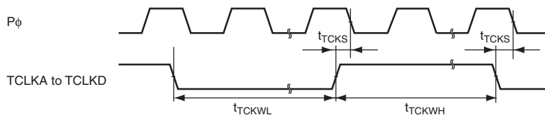
Figure 27.27 TPU Clock Input Timing
