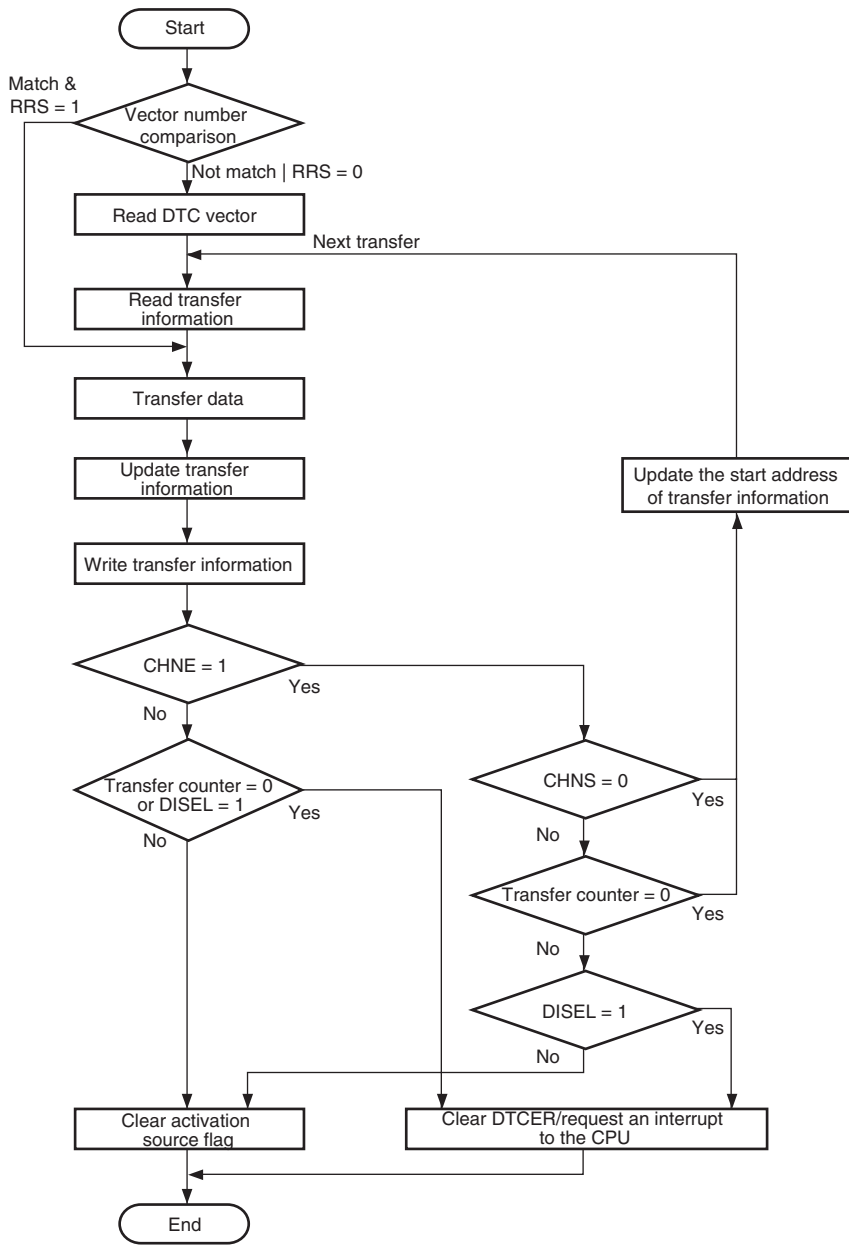
Figure 11.4 Flowchart of DTC Operation
