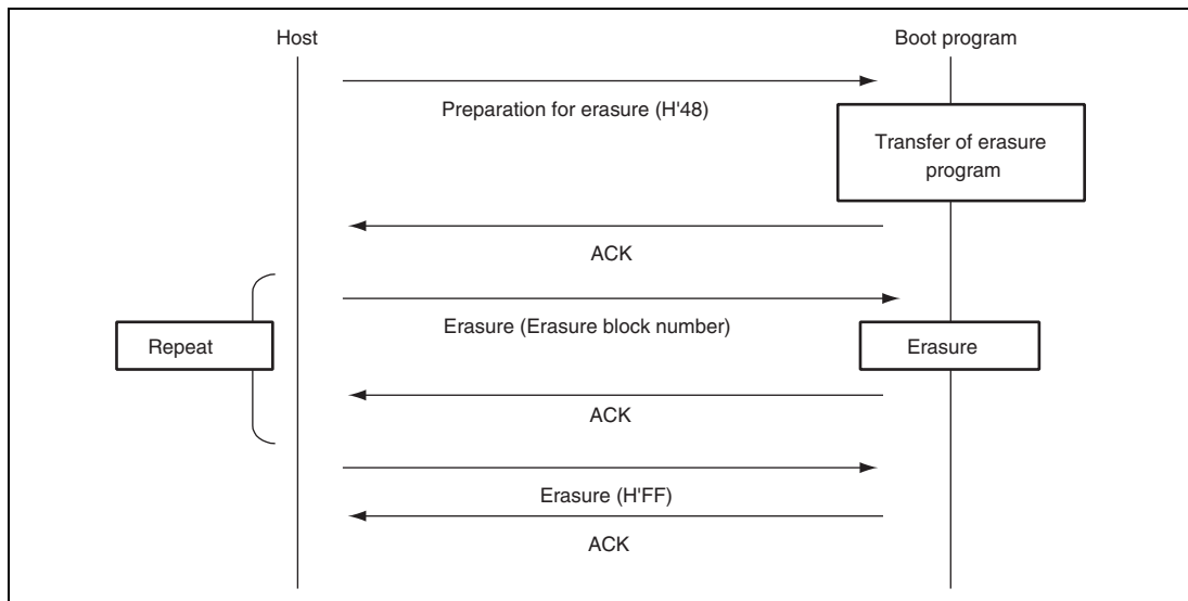
Figure 22.26 Erasure Sequence
