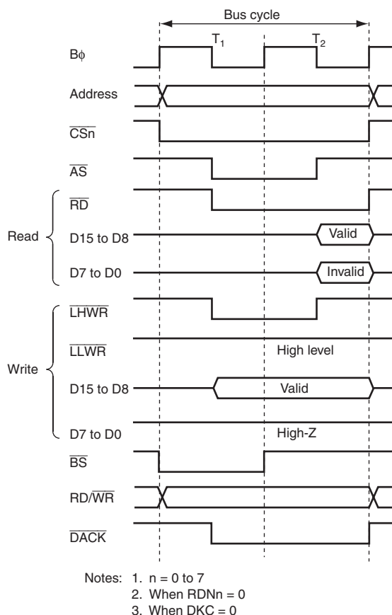
Figure 9.14 16-Bit 2-State Access Space Bus Timing (Byte Access for Even Address)
