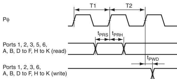
Figure 27.25 I/O Port Input/Output Timing
