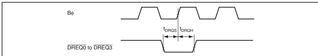
Figure 27.21 DMAC ( \overline{DREQ} ) Input Timing
