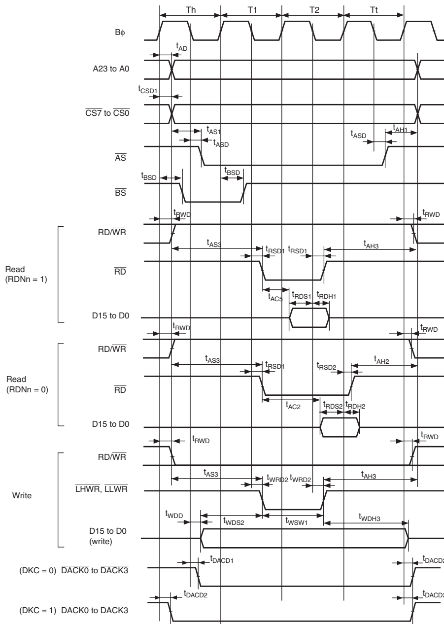
Figure 27.11 Basic Bus Timing: Two-State Access ( \overline{\text{CS}} Assertion Period Extended)
