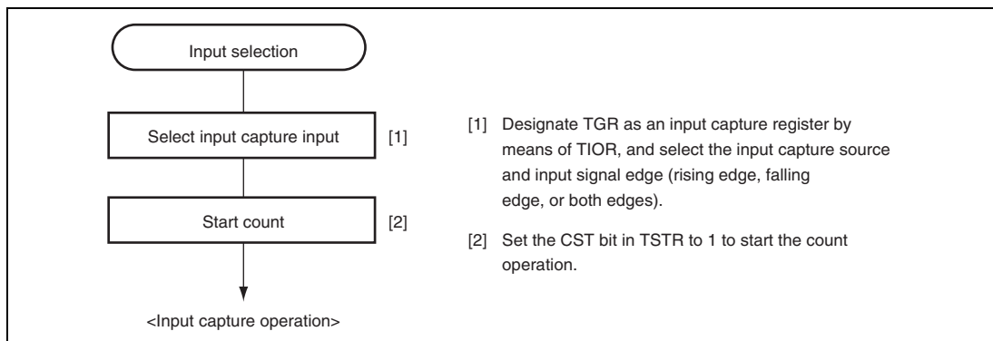
Figure 13.9 Example of Setting Procedure for Input Capture Operation
