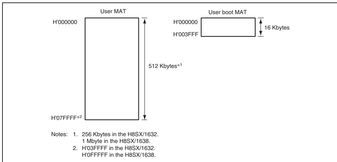
Figure 22.3 Memory MAT Configuration (H8SX/16xx_512K)
