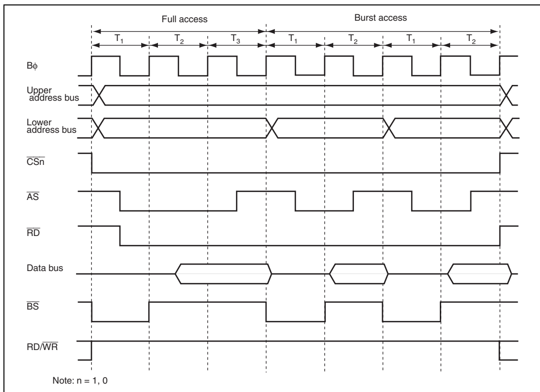
Figure 9.28 Example of Burst ROM Access Timing (AST n = 1, Two Burst Cycles)
