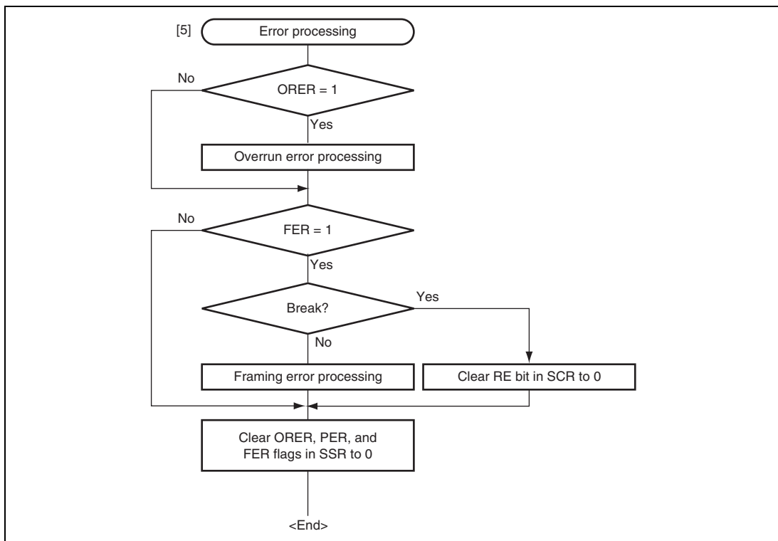
Figure 17.16 Sample Multiprocessor Serial Reception Flowchart (2)
