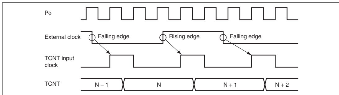
Figure 13.32 Count Timing in External Clock Operation
