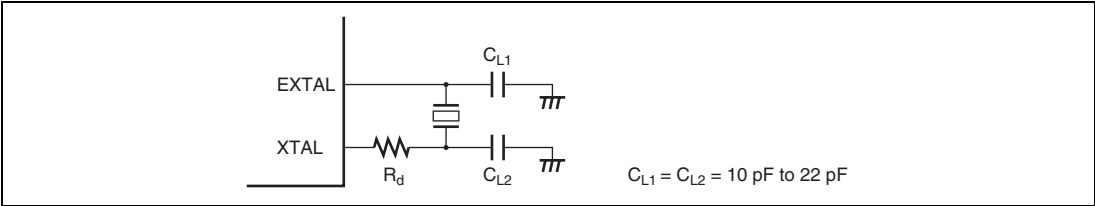
Figure 24.2 Connection of Crystal Resonator (Example)
