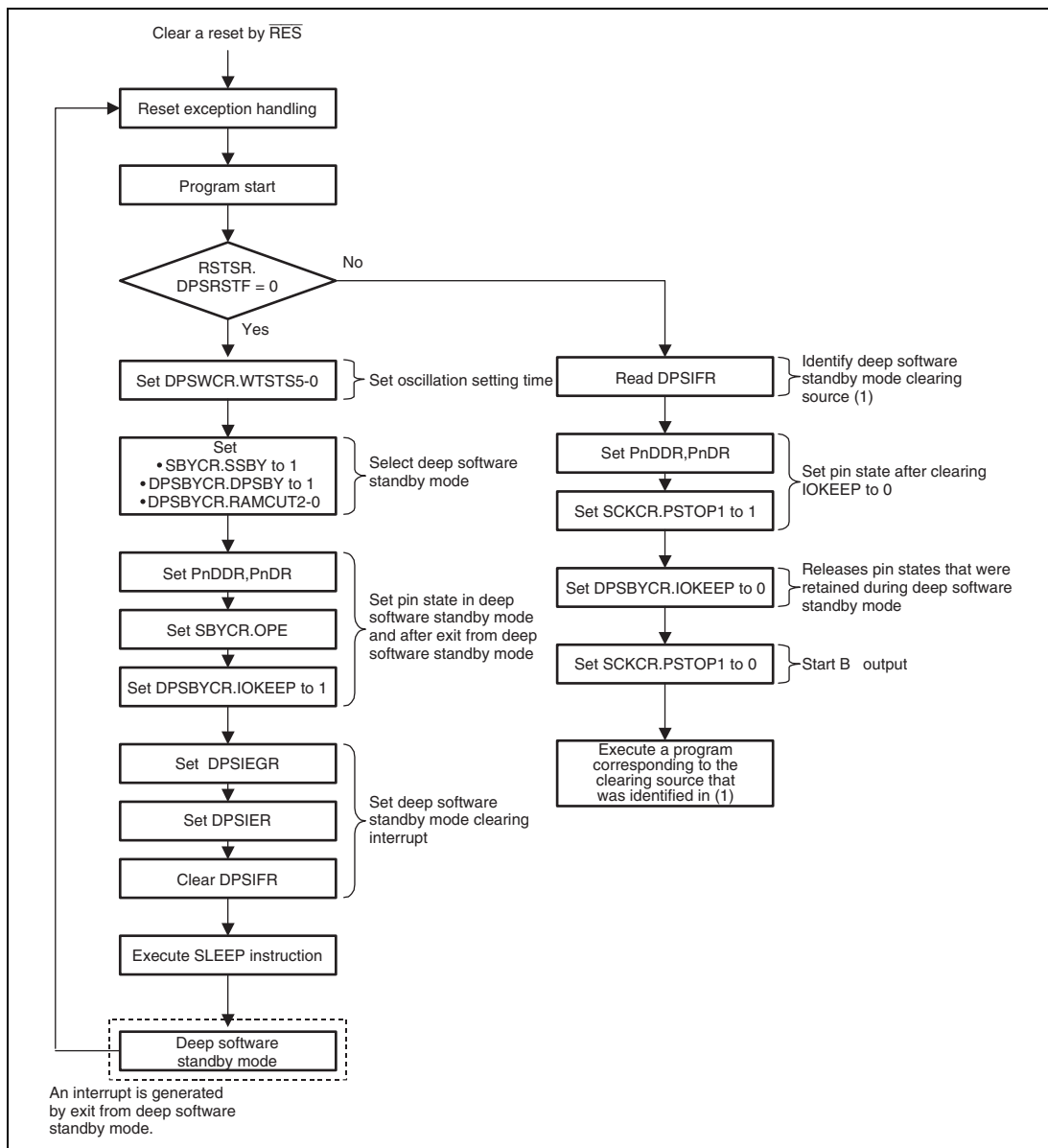
Figure 25.7 Flowchart of Deep Software Standby Mode Operation
