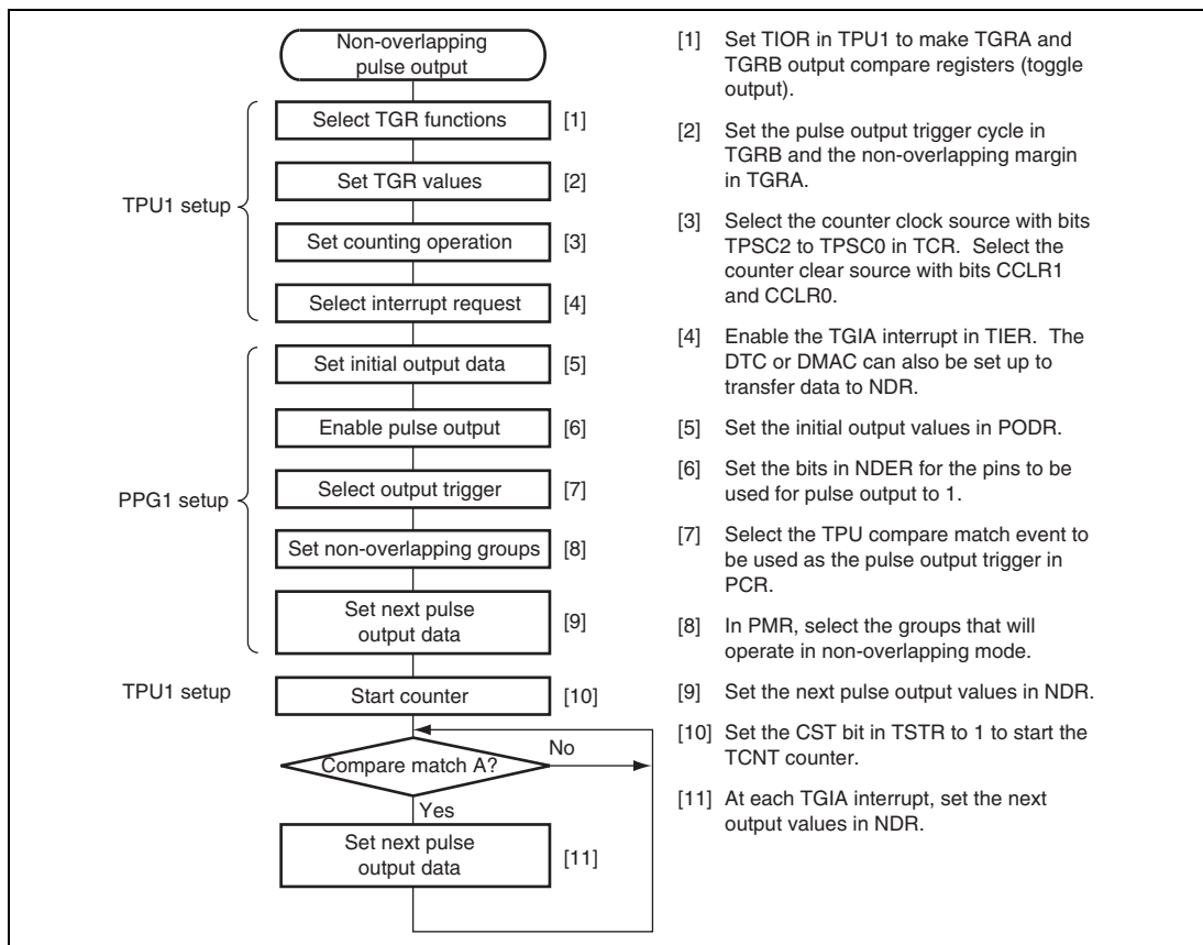
Figure 14.11 Setup Procedure for Non-Overlapping Pulse Output (PPG1)
