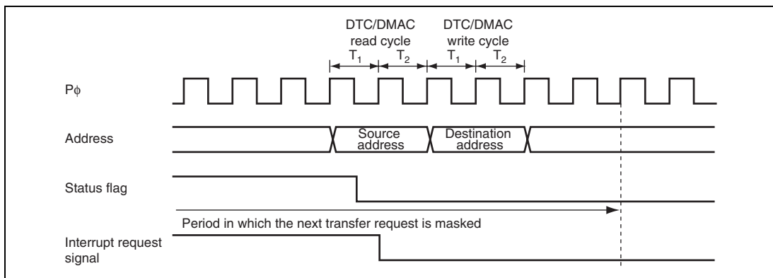
Figure 13.44 Timing for Status Flag Clearing by DTC/DMAC Activation (1)
