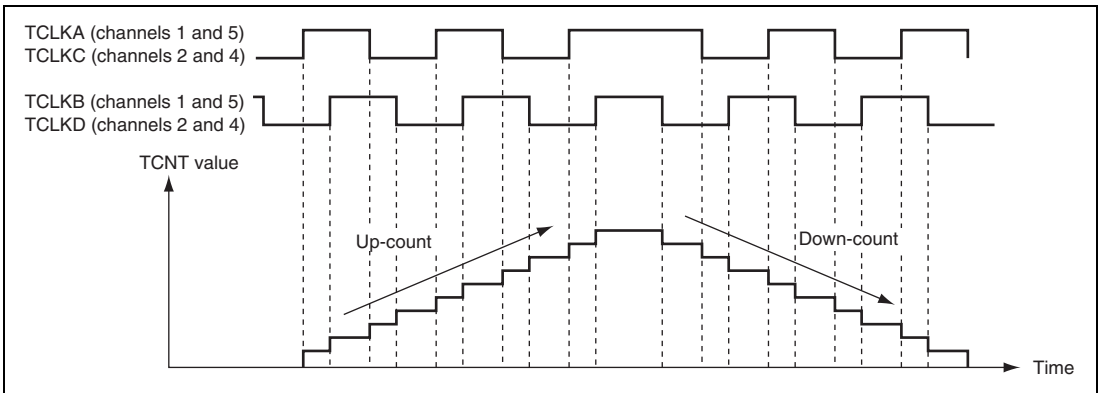
Figure 13.26 Example of Phase Counting Mode 1 Operation
