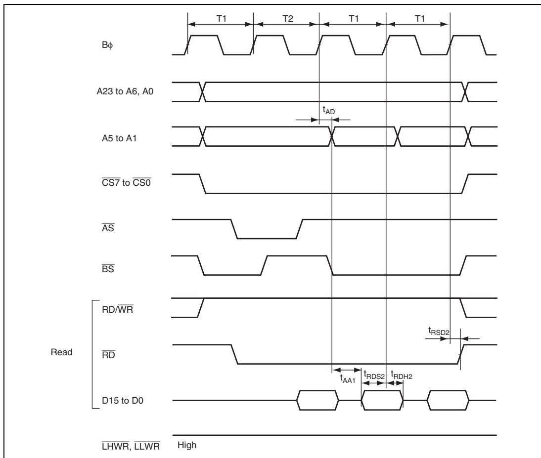
Figure 27.15 Burst ROM Access Timing: One-State Burst Access
