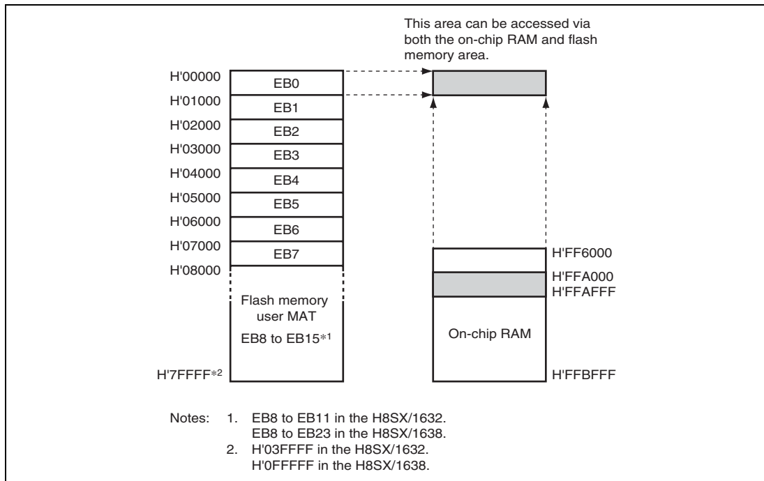
Figure 22.18 Address Map of Overlaid RAM Area (H8SX/1634)
