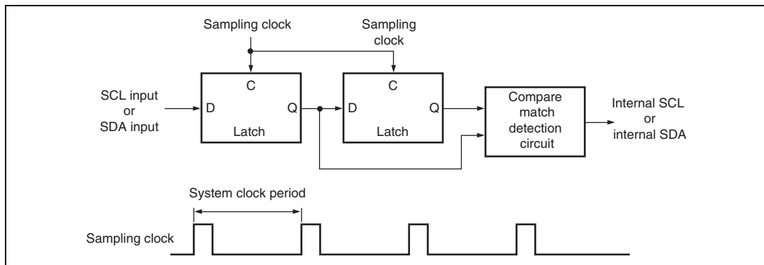
Figure 18.13 Block Diagram of Noise Canceler
