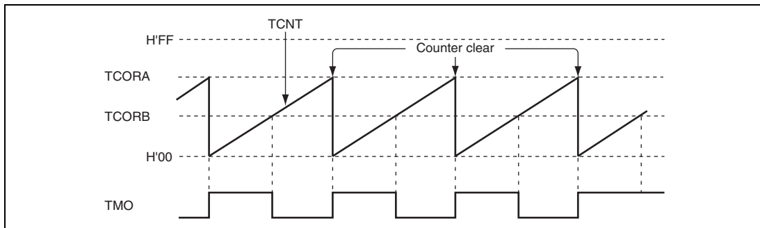
Figure 15.5 Example of Pulse Output
