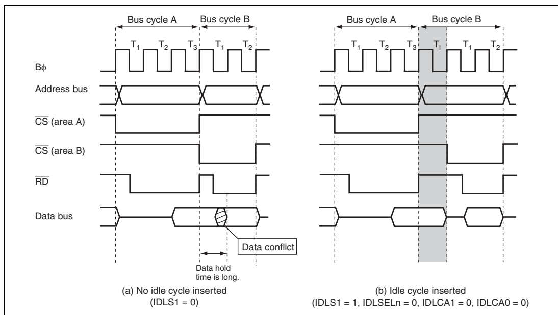
Figure 9.37 Example of Idle Cycle Operation (Consecutive Reads in Different Areas)
