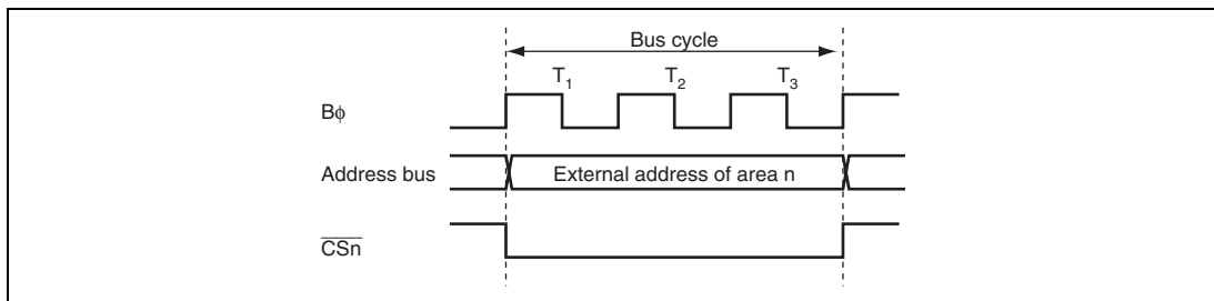
Figure 9.8 \overline{CSn} Signal Output Timing ( n = 0 to 7)
