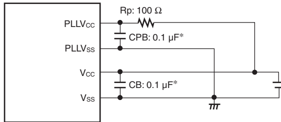
Figure 24.8 Recommended External Circuitry for PLL Circuit
