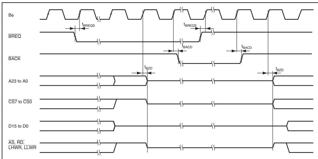
Figure 27.19 External Bus Release Timing
