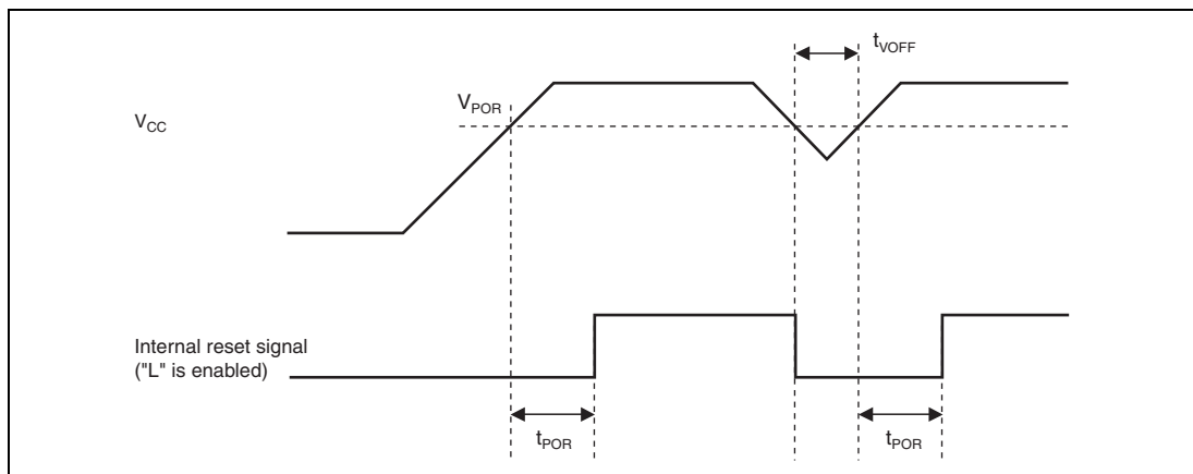
Figure 29.57 Power-on Reset Timing
