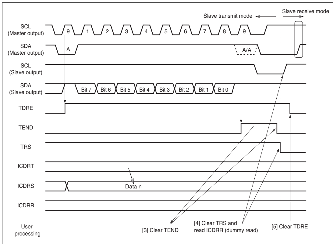
Figure 18.10 Slave Transmit Mode Operation Timing 2
