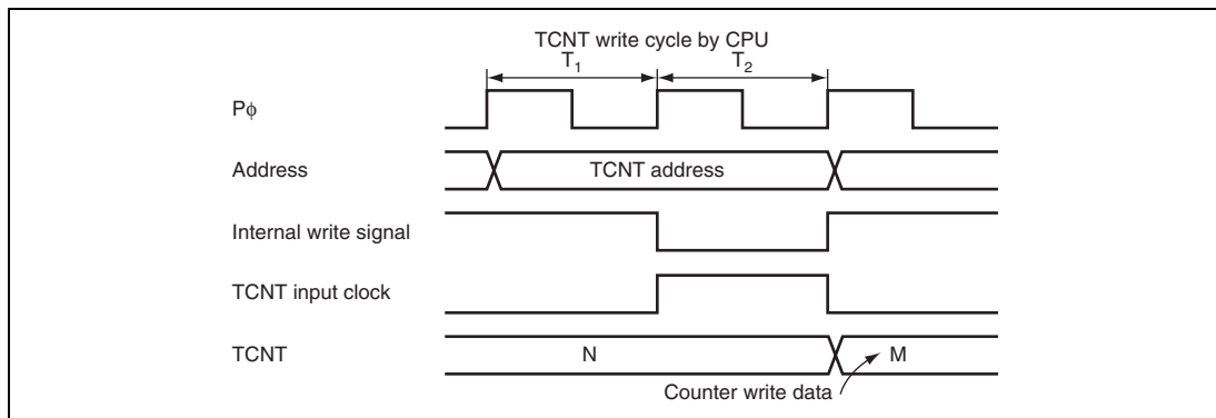
Figure 15.16 Conflict between TCNT Write and Increment
