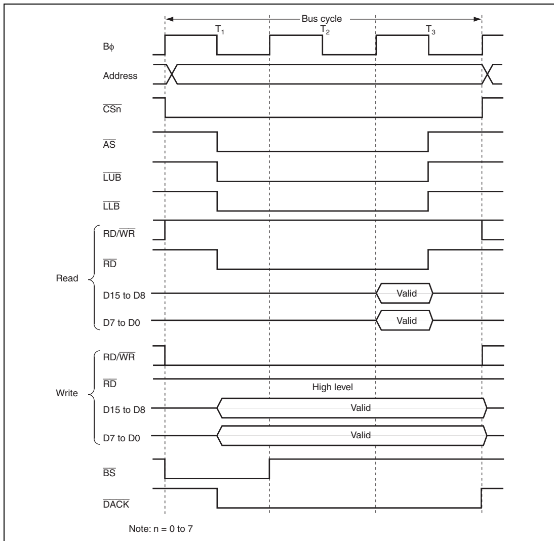
Figure 9.25 16-Bit 3-State Access Space Bus Timing
