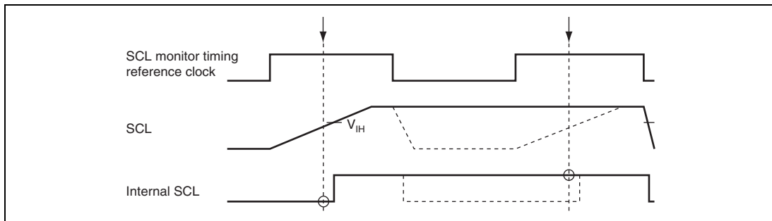
Figure 18.18 Timing of the Bit Synchronous Circuit
