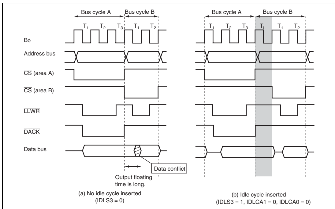
Figure 9.40 Example of Idle Cycle Operation (Write after Single Address Transfer Write)
