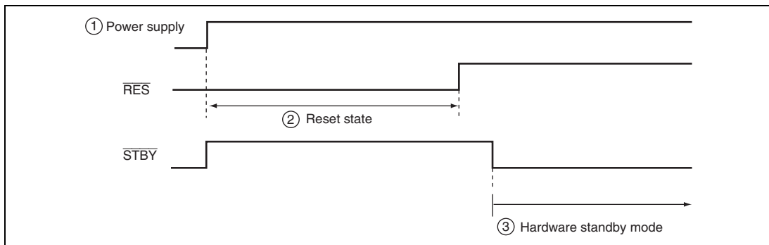
Figure 25.9 Timing Sequence at Power-On
