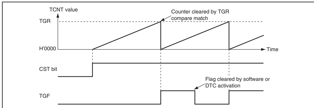
Figure 13.5 Periodic Counter Operation
