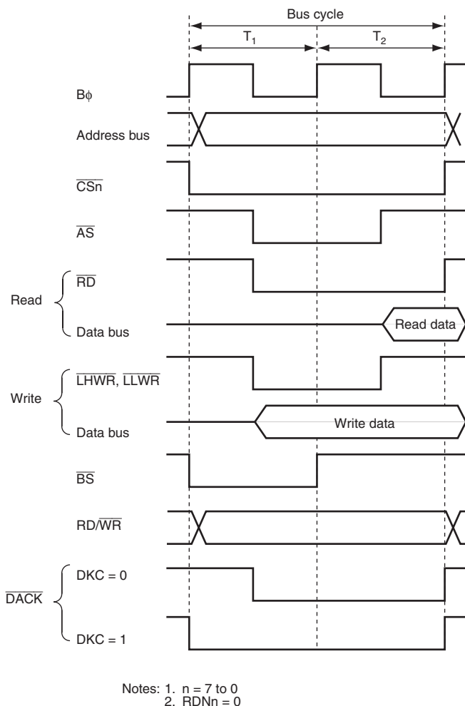
Figure 9.23 \overline{\text{DACK}} Signal Output Timing
