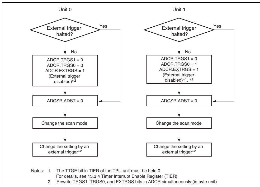
Figure 19.11 Procedure for Changing the Mode When the Setting for Activation by an External Trigger is in Use
