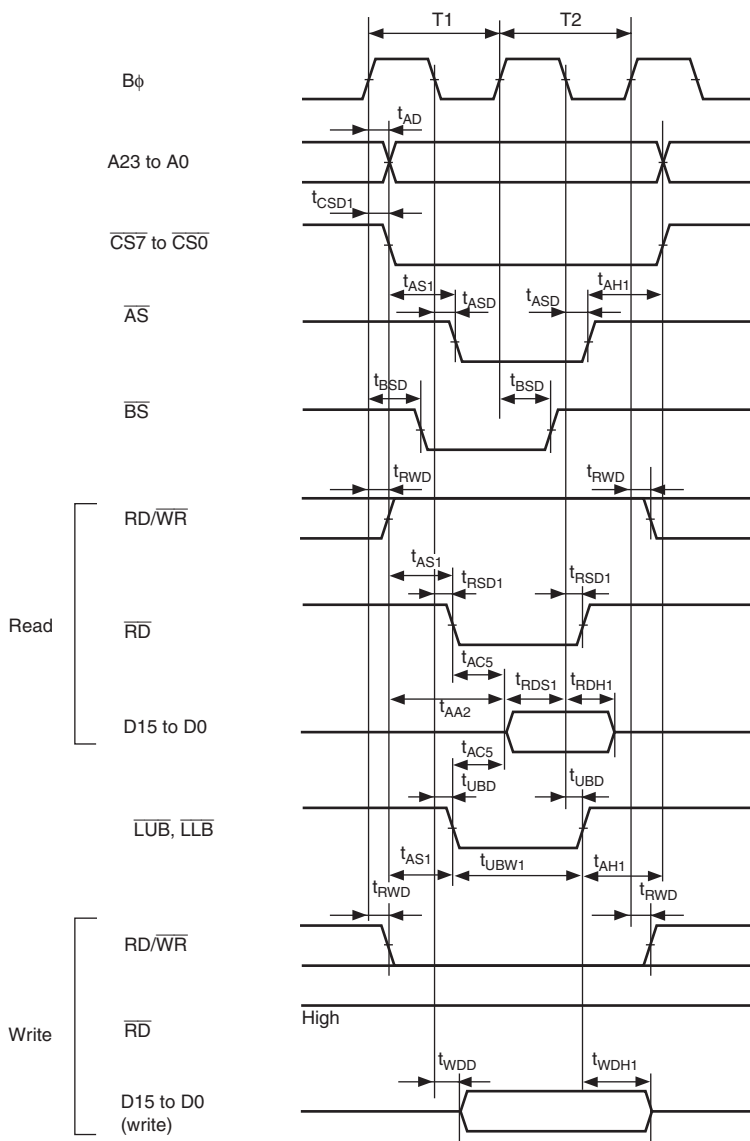
Figure 27.13 Byte Control SRAM: Two-State Read/Write Access
