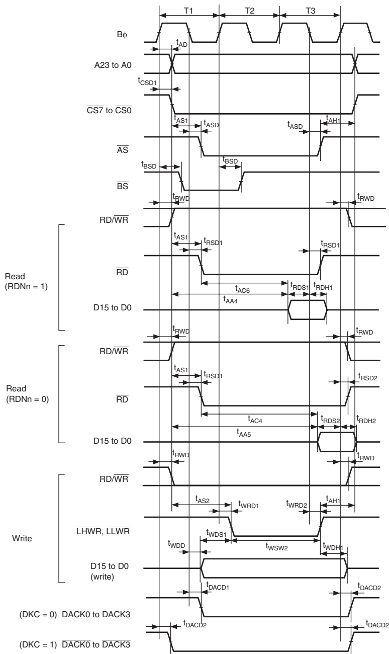
Figure 27.9 Basic Bus Timing: Three-State Access
