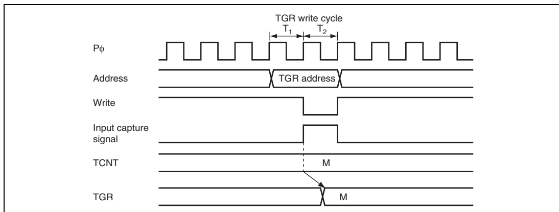
Figure 13.52 Conflict between TGR Write and Input Capture
