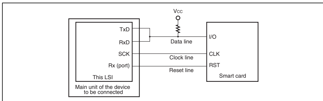
Figure 17.24 Pin Connection for Smart Card Interface
