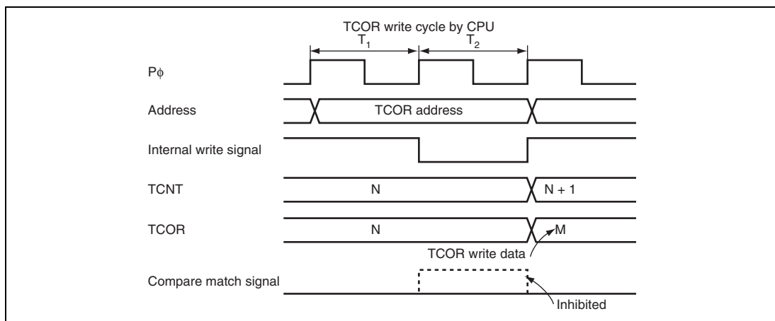
Figure 15.17 Conflict between TCOR Write and Compare Match
