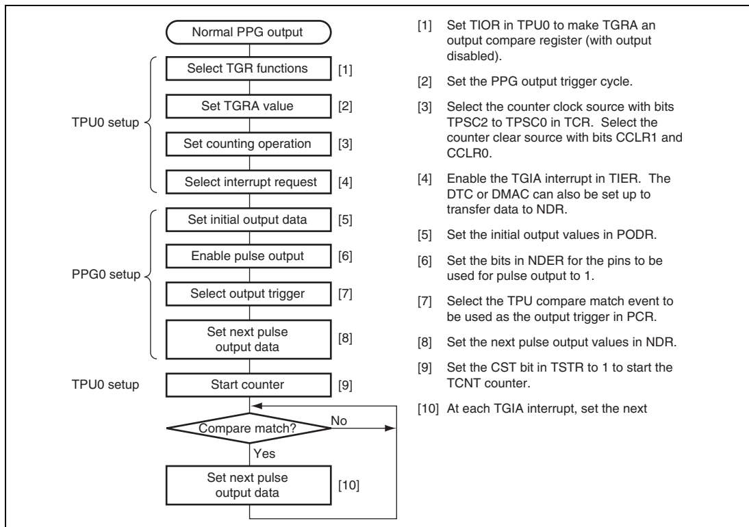
Figure 14.5 Setup Procedure for Normal Pulse Output (PPG0)
