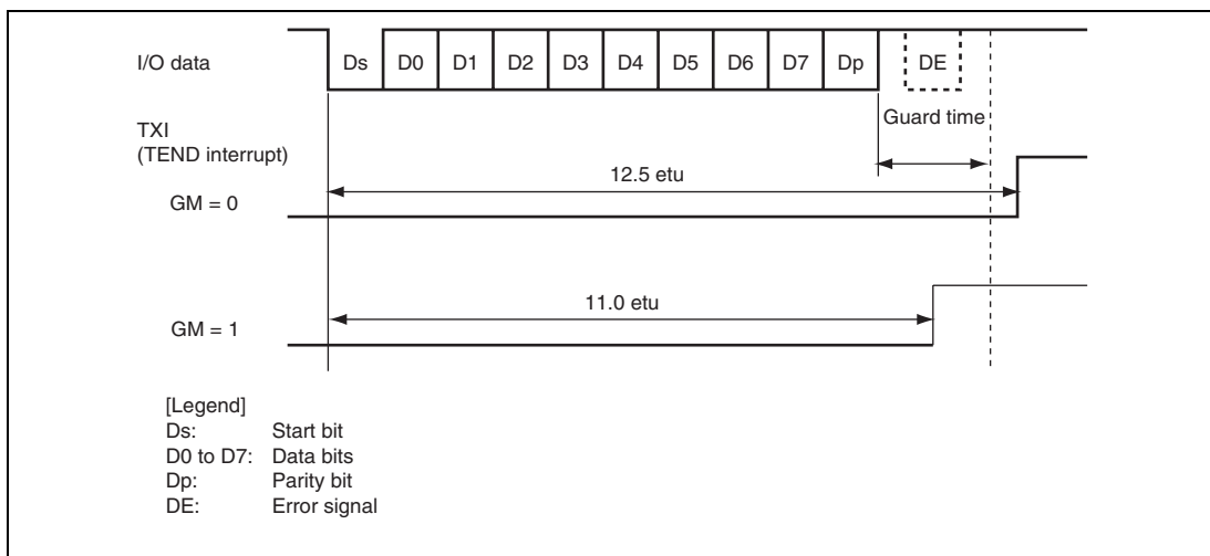
Figure 17.30 TEND Flag Set Timing during Transmission
