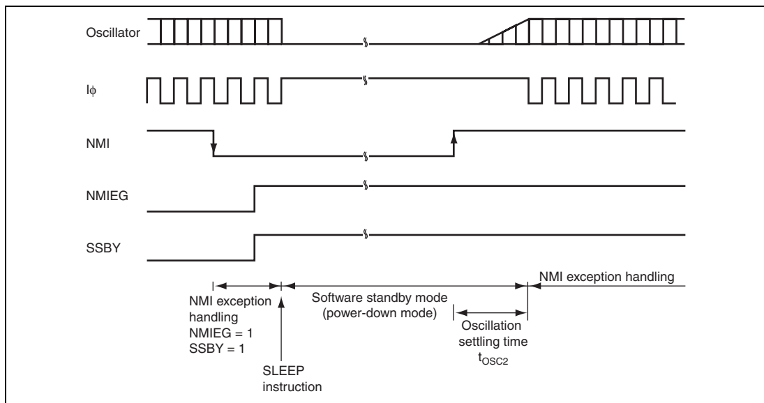
Figure 27.3 Oscillation Settling Timing after Software Standby Mode
