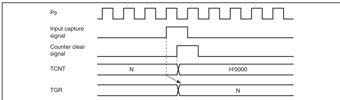
Figure 13.36 Counter Clear Timing (Input Capture)
