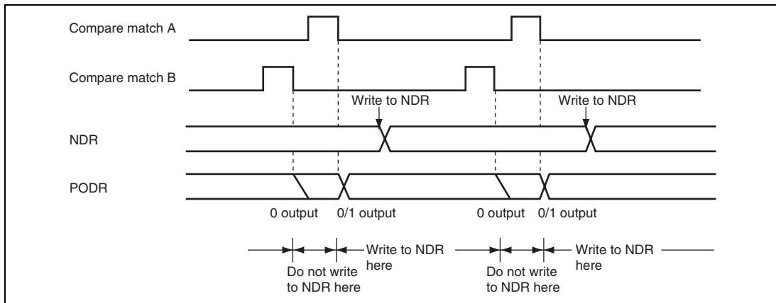
Figure 14.9 Non-Overlapping Operation and NDR Write Timing
