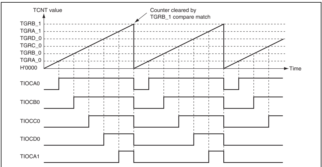
Figure 13.23 Example of PWM Mode Operation (2)
