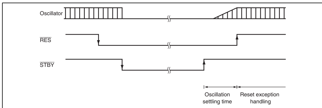
Figure 25.8 Hardware Standby Mode Timing
