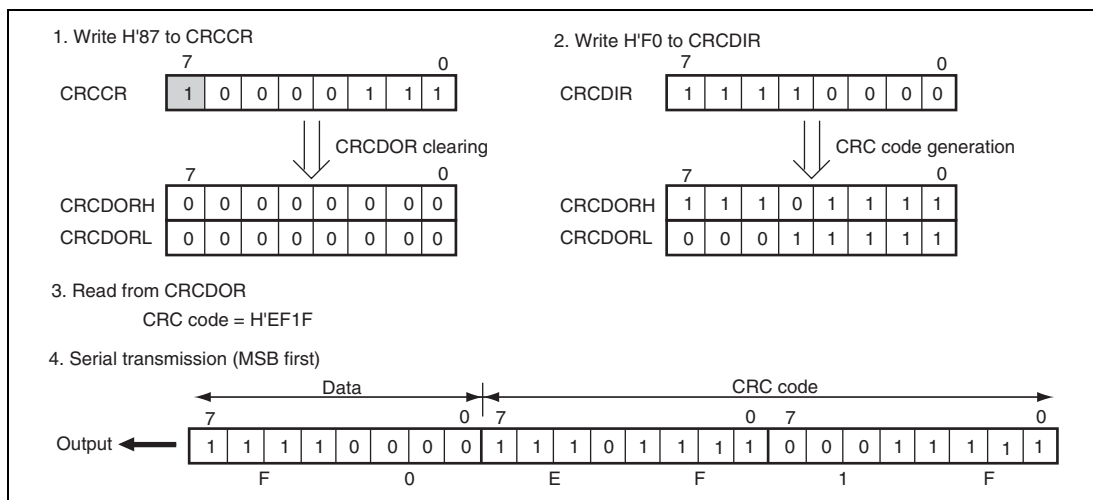
Figure 17.45 MSB-First Data Transmission
