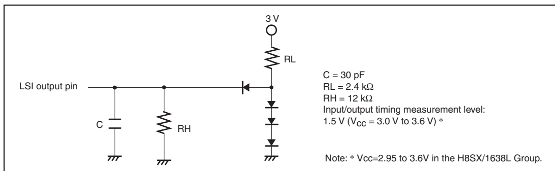
Figure 27.1 Output Load Circuit
