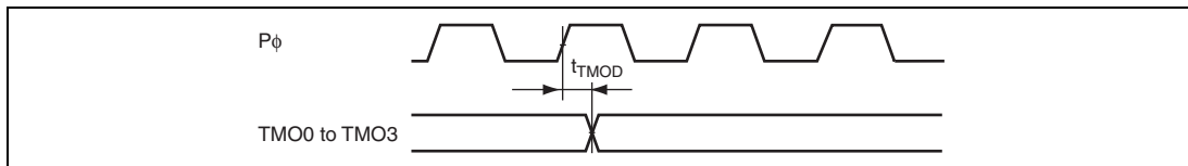
Figure 27.29 8-Bit Timer Output Timing
