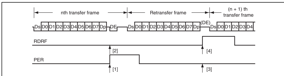
Figure 17.32 Data Re-Transfer Operation in SCI Reception Mode
