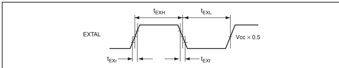
Figure 27.5 External Input Clock Timing
