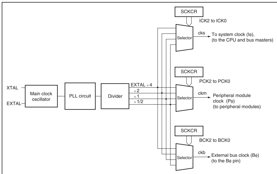
Figure 24.1 Block Diagram of Clock Pulse Generator
