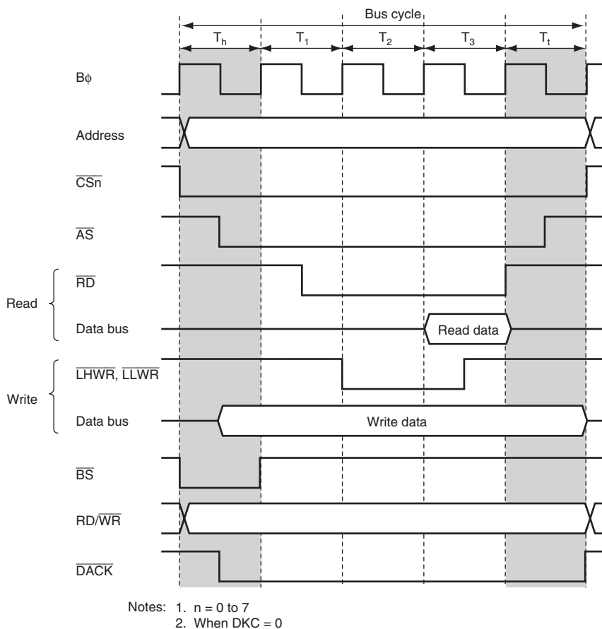
Figure 9.22 Example of Timing when Chip Select Assertion Period is Extended
