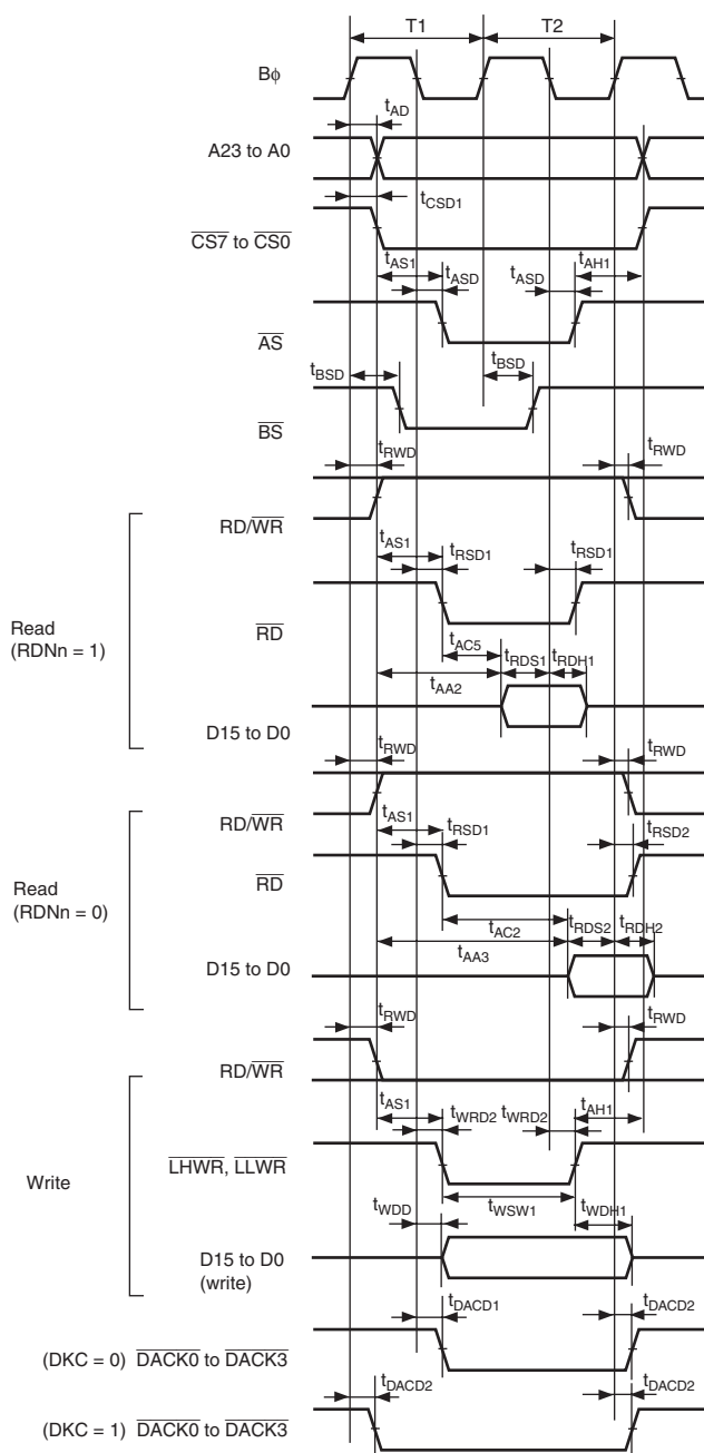
Figure 27.8 Basic Bus Timing: Two-State Access
