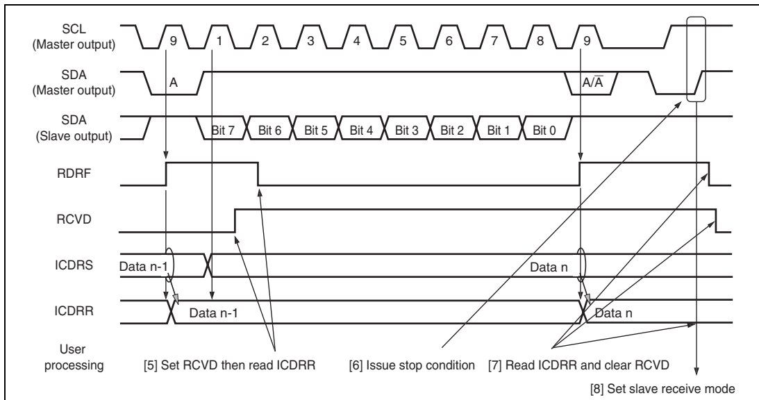
Figure 18.8 Master Receive Mode Operation Timing 2
