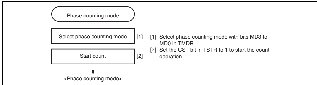
Figure 13.25 Example of Phase Counting Mode Setting Procedure
