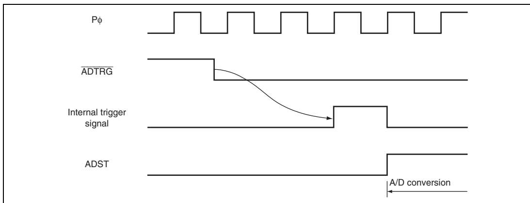
Figure 19.7 External Trigger Input Timing ( \text{TRGS1} , \text{TRGS0} , and \text{EXTRGS} \neq \text{B}'111 )
