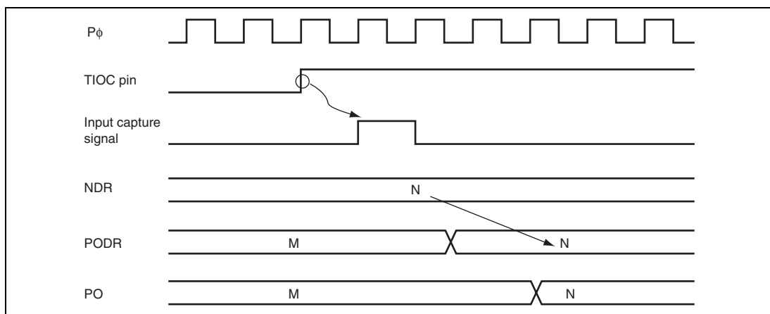
Figure 14.14 Pulse Output Triggered by Input Capture (Example)
