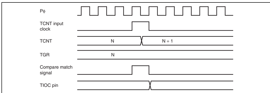
Figure 13.33 Output Compare Output Timing
