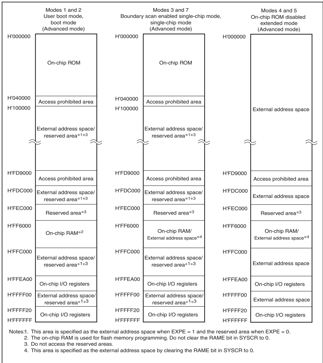
Figure 3.3 Address Map in Each Operating Mode of H8SX/1632 and H8SX/1632L (1)
