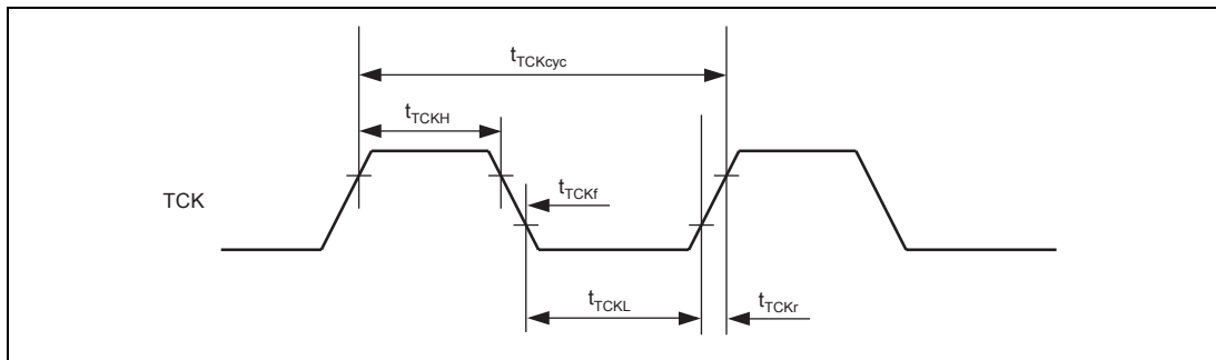
Figure 27.37 Boundary Scan TCK Timing
