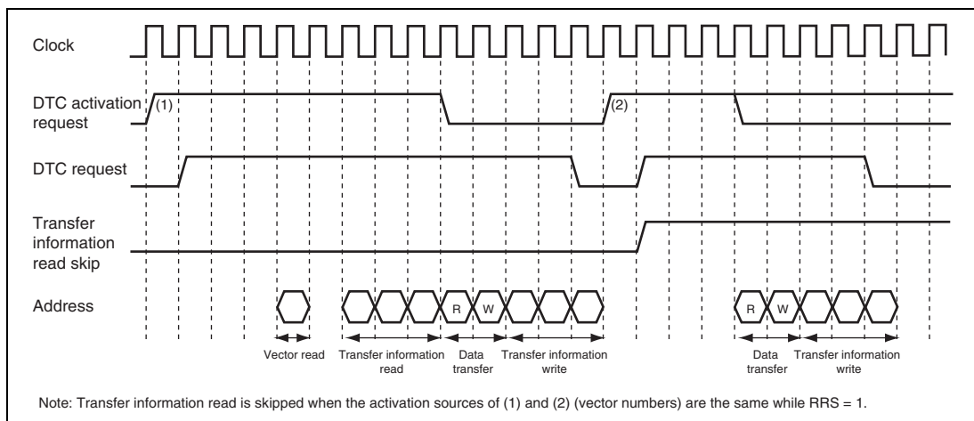
Figure 11.6 Transfer Information Read Skip Timing
