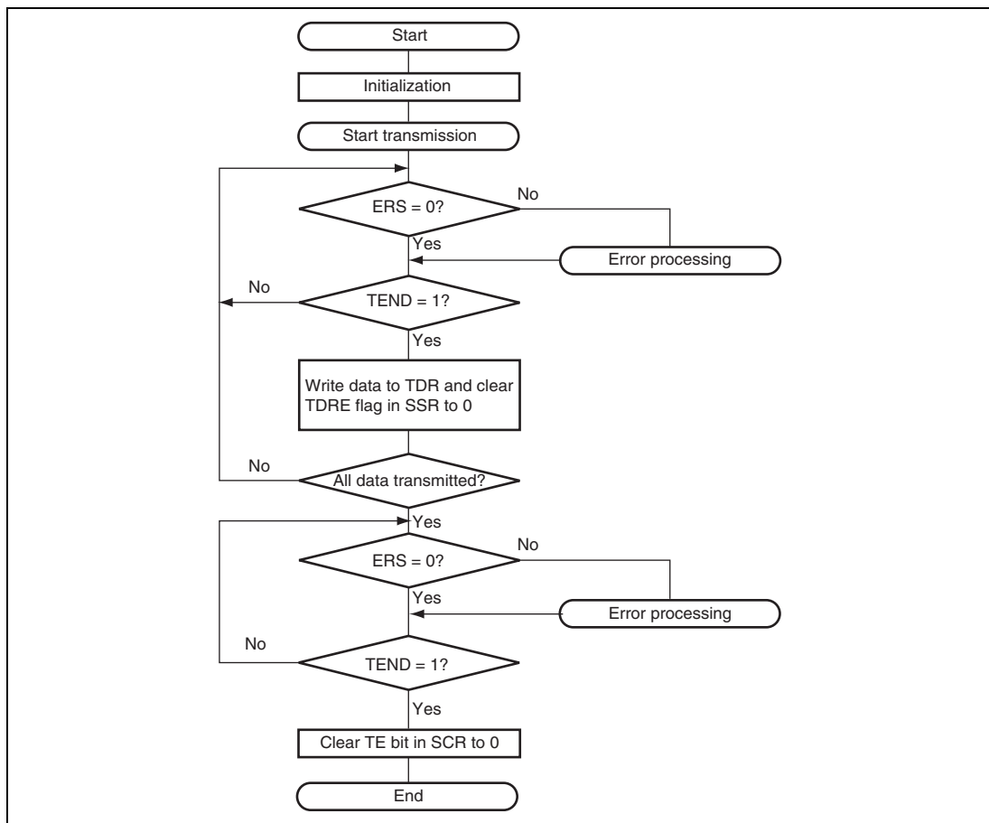
Figure 17.31 Sample Transmission Flowchart
