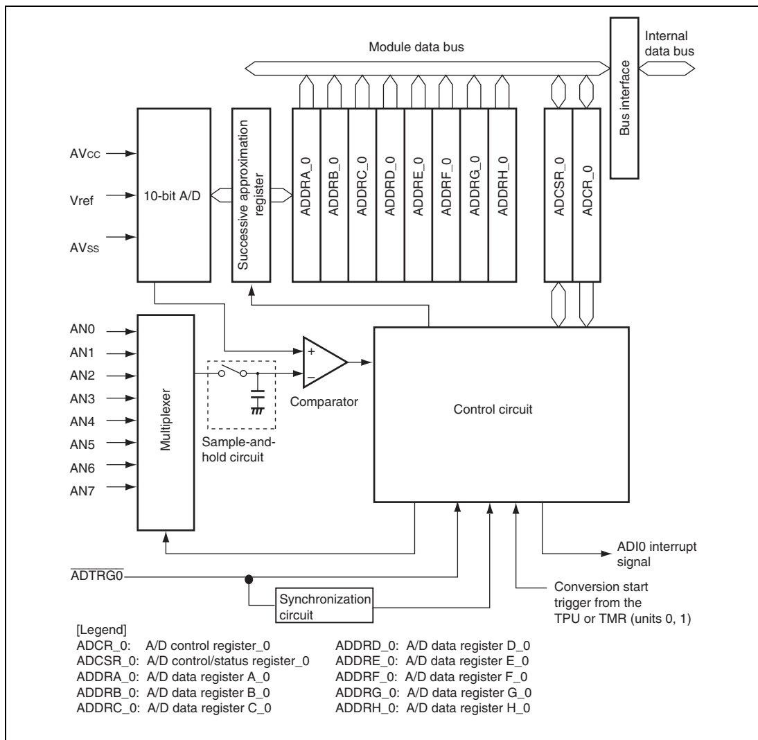
Figure 19.1 Block Diagram of A/D Converter Unit 0 (AD_0)
