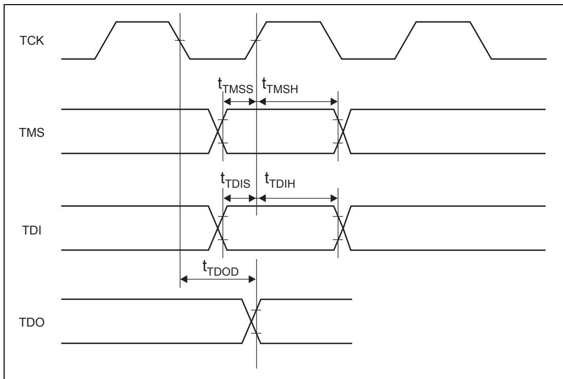
Figure 27.39 Boundary Scan Input/Output Timing
