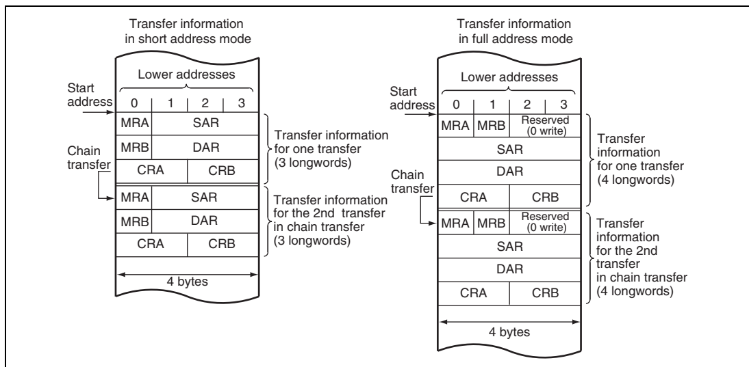
Figure 11.2 Transfer Information on Data Area
