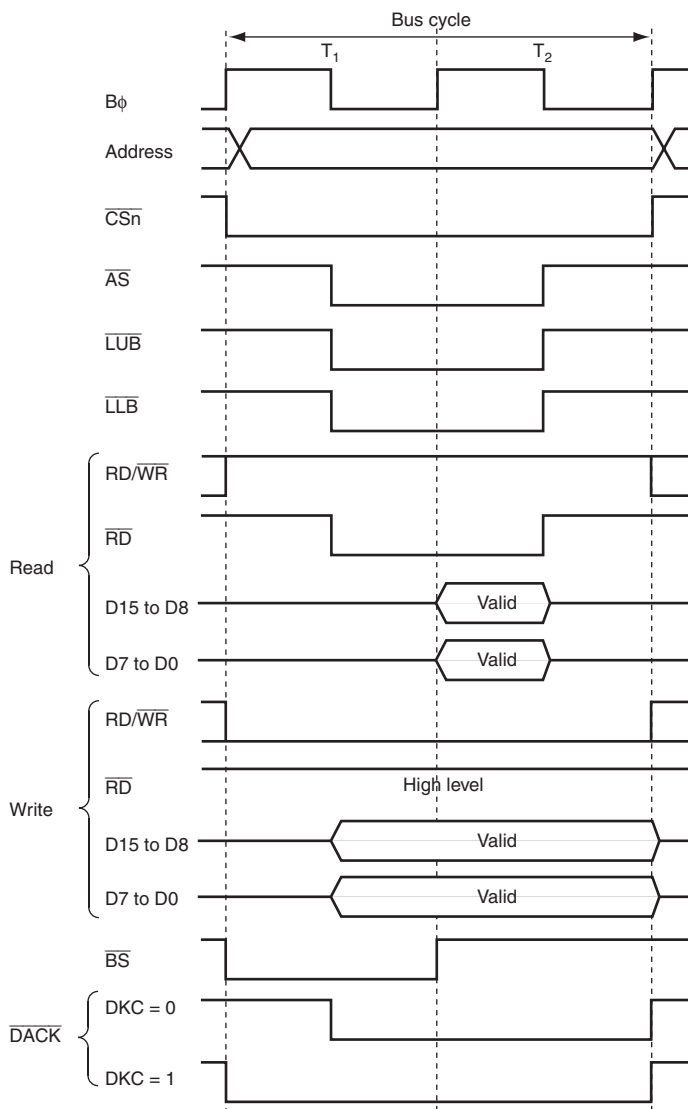
Figure 9.27 \overline{\text{DACK}} Signal Output Timing
