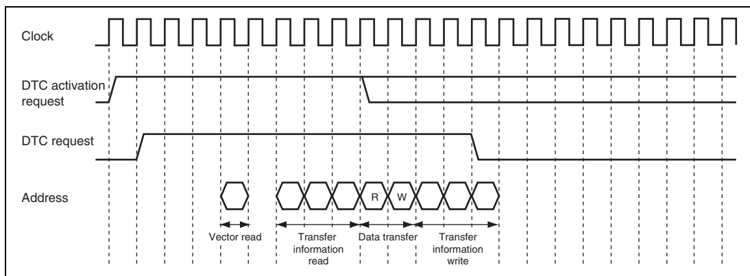
Figure 11.11 DTC Operation Timing (Example of Short Address Mode in Normal Transfer Mode or Repeat Transfer Mode)
