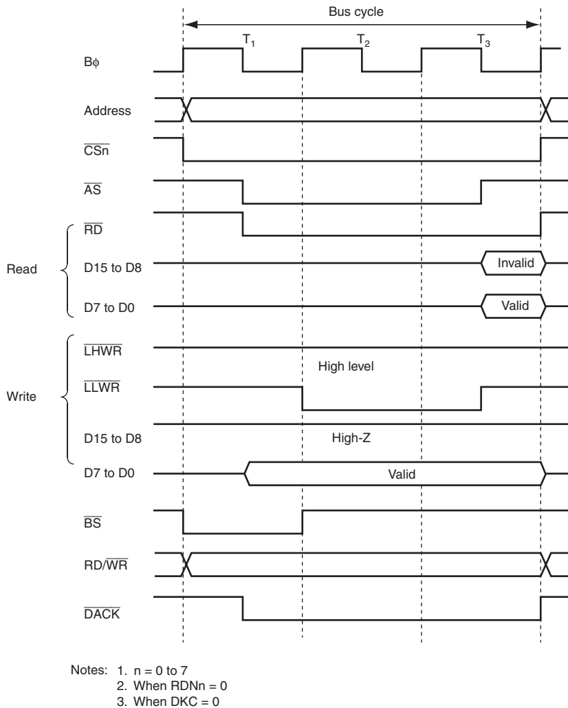
Figure 9.18 16-Bit 3-State Access Space Bus Timing (Word Access for Odd Address)
