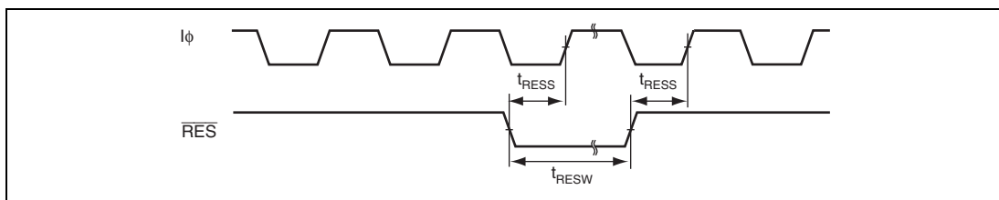
Figure 27.6 Reset Input Timing
