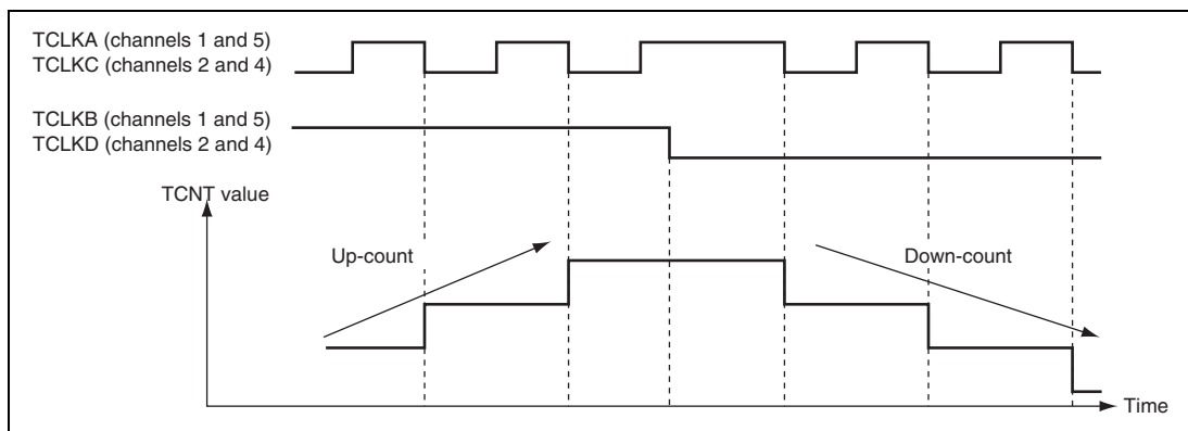
Figure 13.27 Example of Phase Counting Mode 2 Operation
