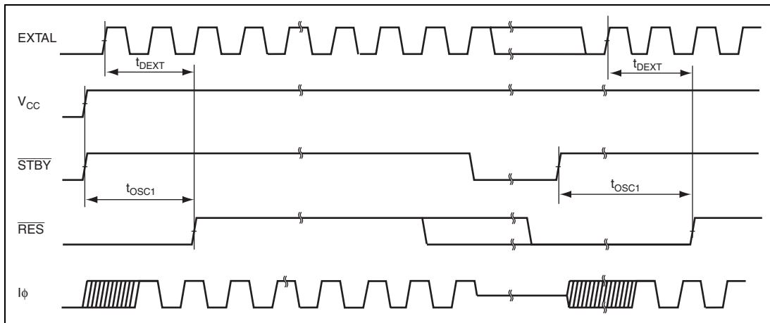
Figure 27.4 Oscillation Settling Timing
