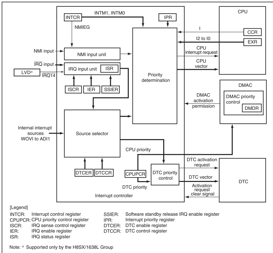
Figure 7.1 Block Diagram of Interrupt Controller
