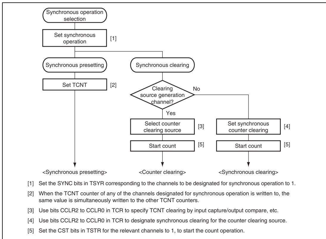
Figure 13.11 Example of Synchronous Operation Setting Procedure
