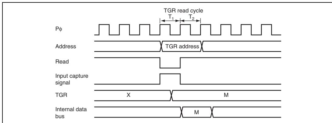
Figure 13.51 Conflict between TGR Read and Input Capture
