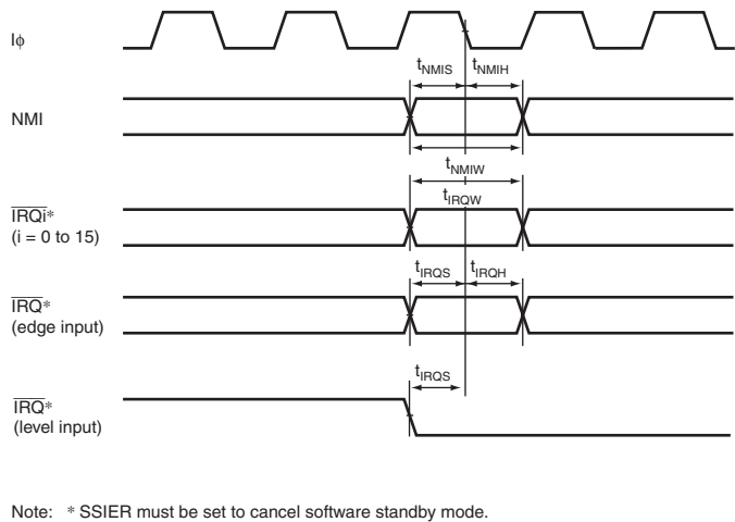
Figure 27.7 Interrupt Input Timing
