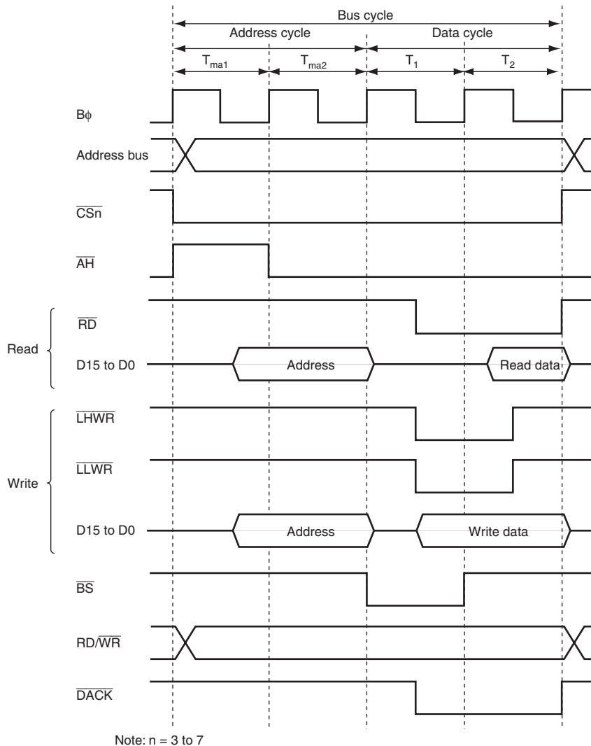
Figure 9.31 16-Bit Access Space Access Timing (ABWHn = 0, ABWLn = 1)
