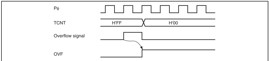
Figure 15.14 Timing of OVF Setting
