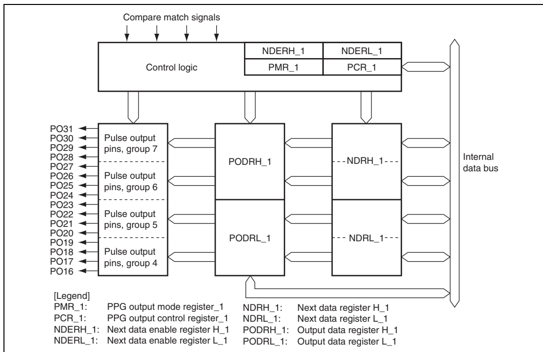
Figure 14.2 Block Diagram of PPG (Unit 1)
