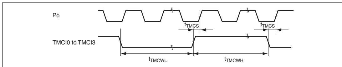
Figure 27.31 8-Bit Timer Clock Input Timing
