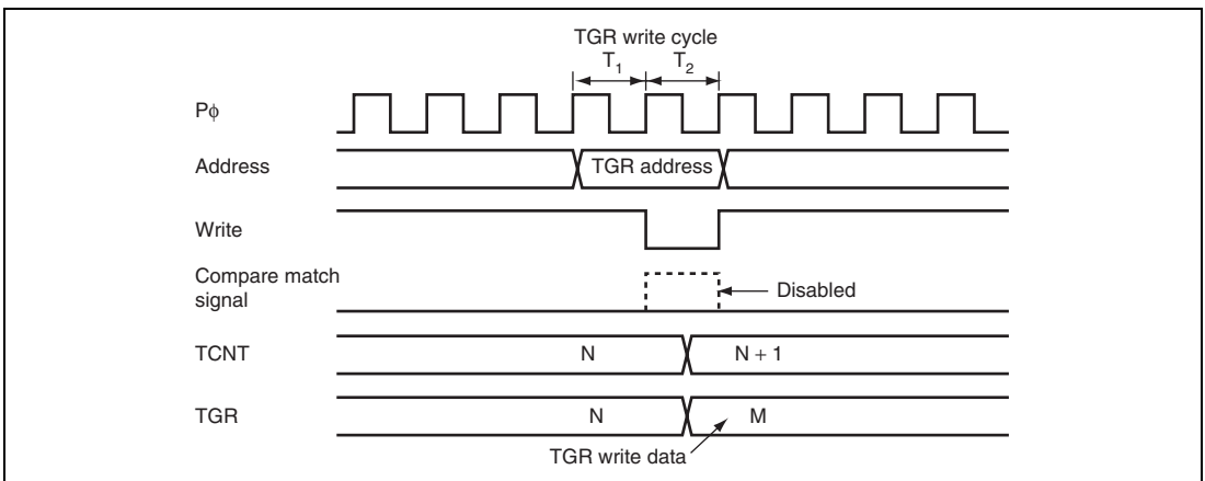
Figure 13.49 Conflict between TGR Write and Compare Match
