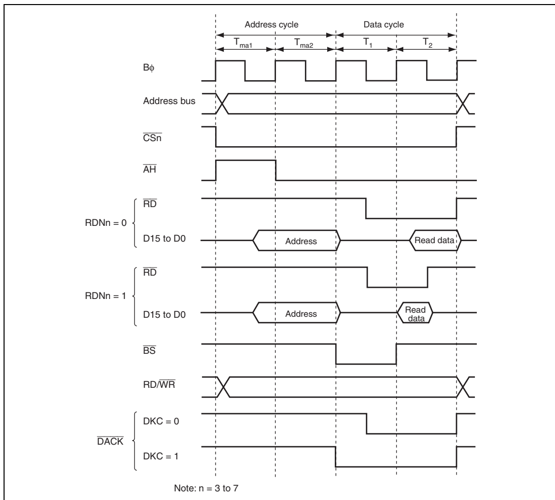
Figure 9.36 \overline{\text{DACK}} Signal Output Timing
