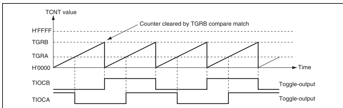
Figure 13.8 Example of Toggle Output Operation
