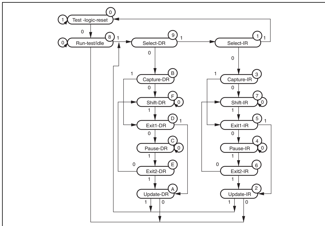
Figure 23.2 State Transition of TAP Controller
