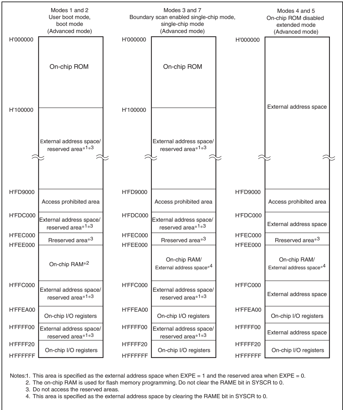
Figure 3.1 Address Map in Each Operating Mode of H8SX/1638 and H8SX/1638L (1)
