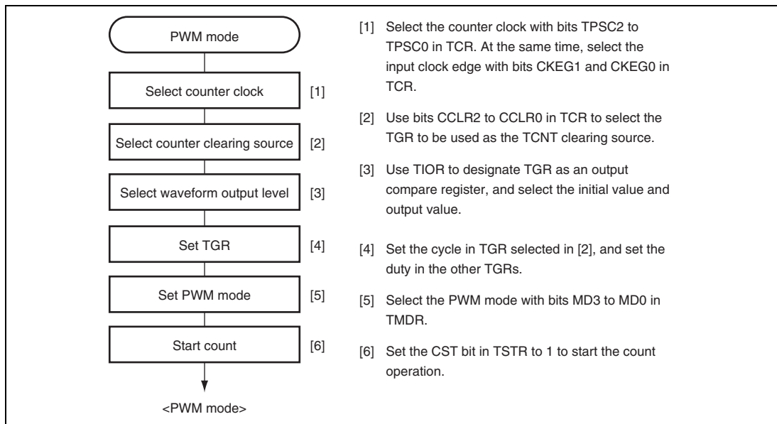
Figure 13.21 Example of PWM Mode Setting Procedure
