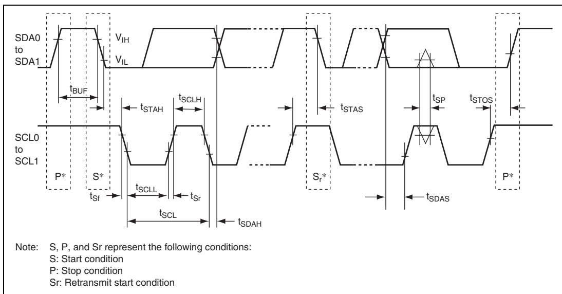
Figure 27.36 I²C Bus Interface 2 Input/Output Timing (Option)
