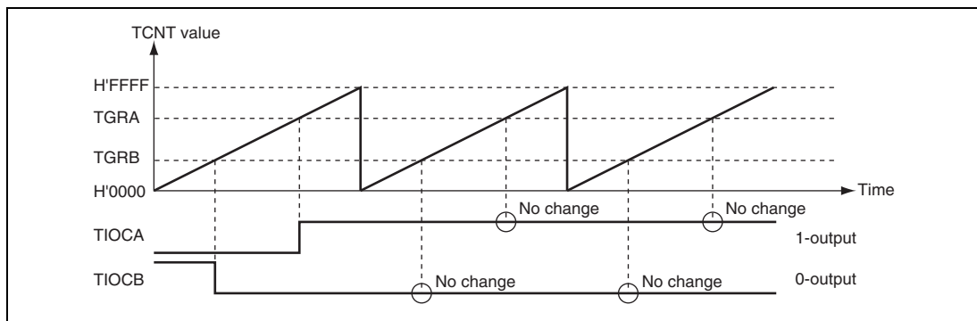
Figure 13.7 Example of 0-Output/1-Output Operation
