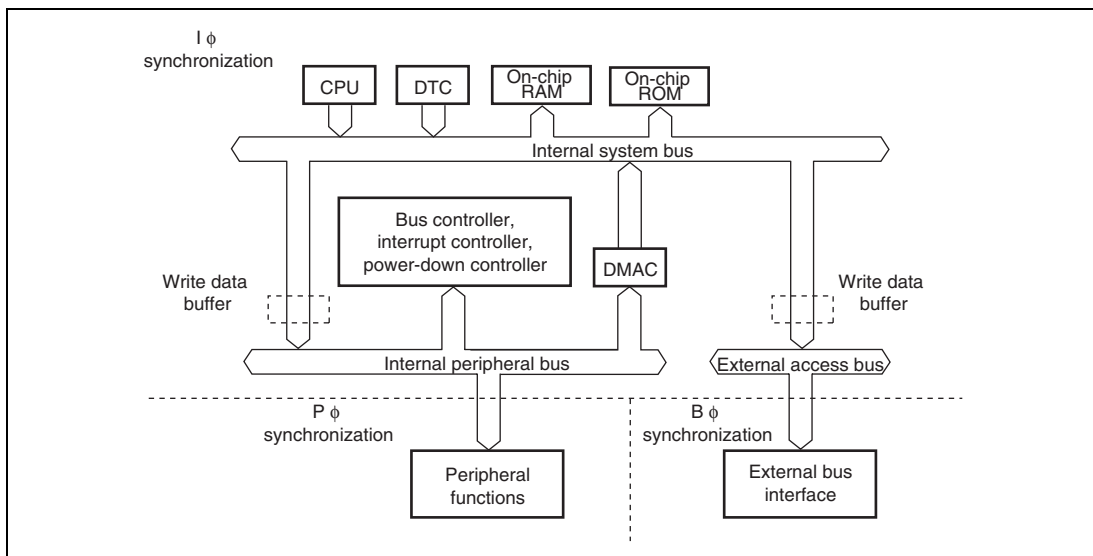
Figure 9.4 Internal Bus Configuration
