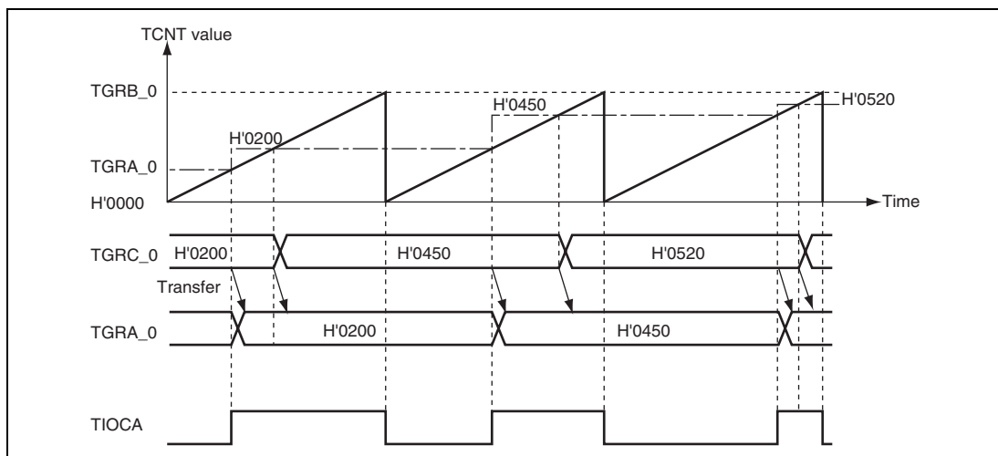
Figure 13.16 Example of Buffer Operation (1)
