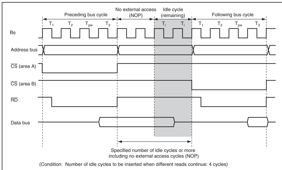
Figure 9.41 Idle Cycle Insertion Example
