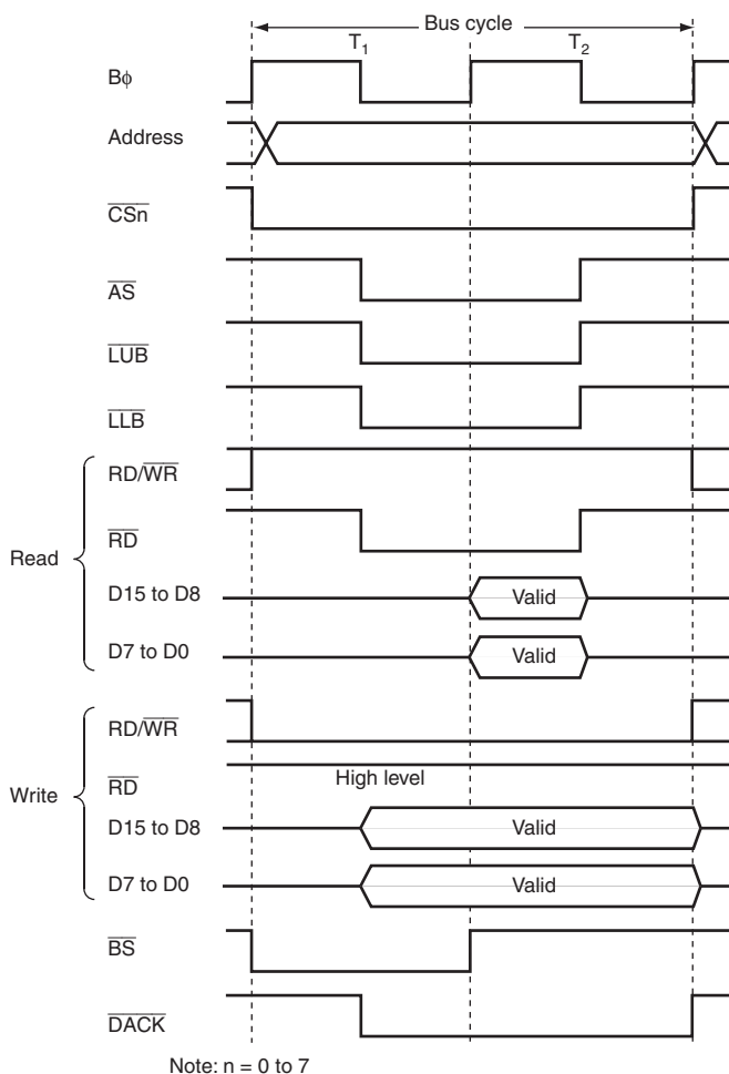
Figure 9.24 16-Bit 2-State Access Space Bus Timing
