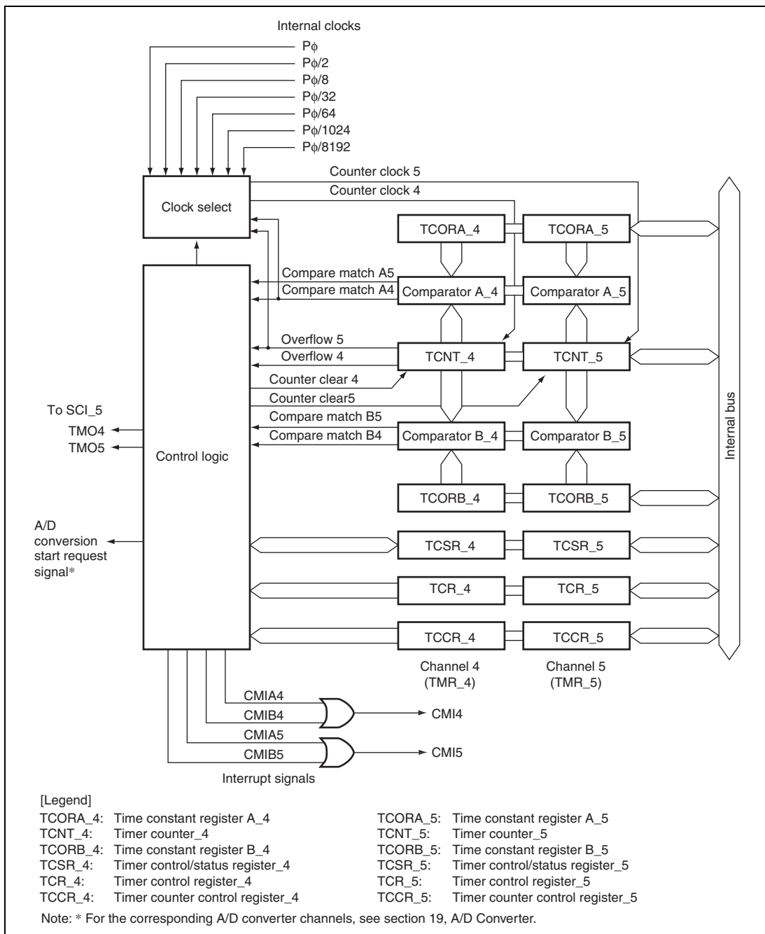
Figure 15.3 Block Diagram of 8-Bit Timer Module (Unit 2)
