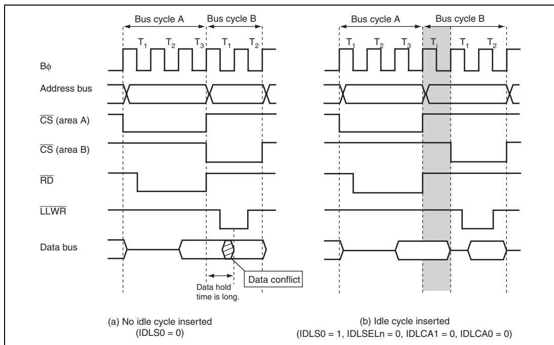
Figure 9.38 Example of Idle Cycle Operation (Write after Read)
