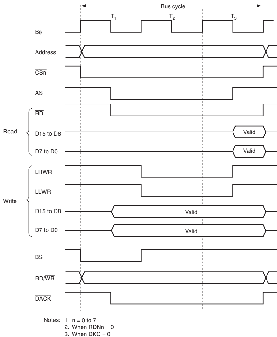
Figure 9.19 16-Bit 3-State Access Space Bus Timing (Word Access for Even Address)
