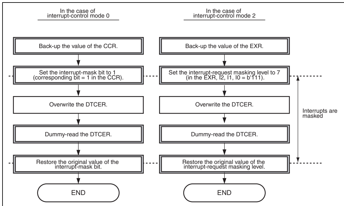
Figure 11.17 Example of Procedures for Overwriting the DTCER
