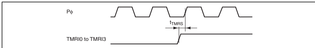
Figure 27.30 8-Bit Timer Reset Input Timing
