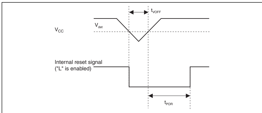
Figure 29.58 Voltage Detection Circuit Timing
