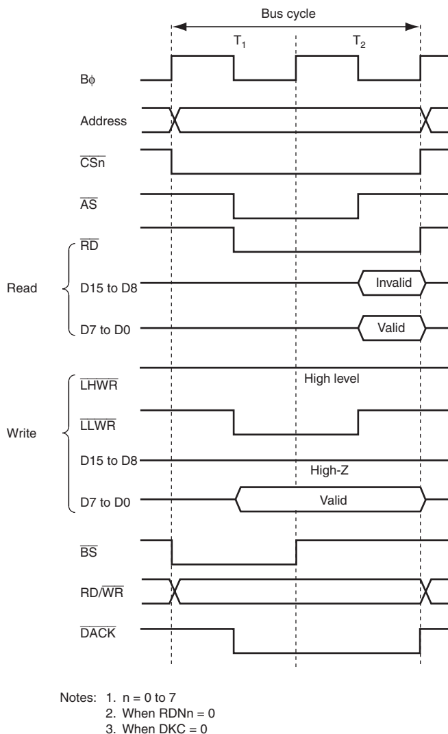
Figure 9.15 16-Bit 2-State Access Space Bus Timing (Byte Access for Odd Address)
