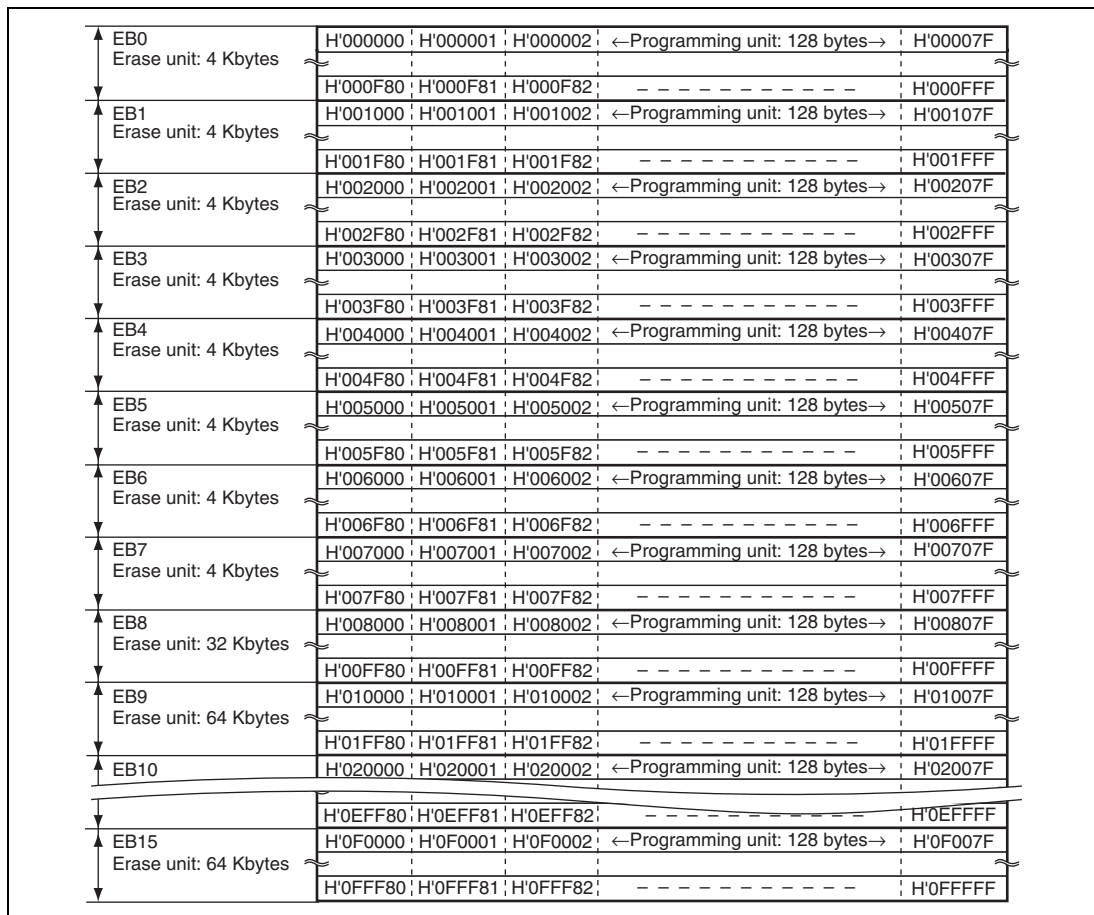
Figure 22.4 (2) User MAT Block Structure of H8SX/1634
