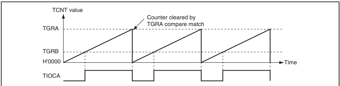
Figure 13.22 Example of PWM Mode Operation (1)
