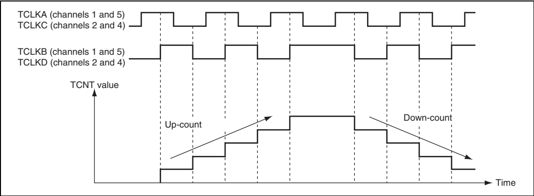
Figure 13.29 Example of Phase Counting Mode 4 Operation
