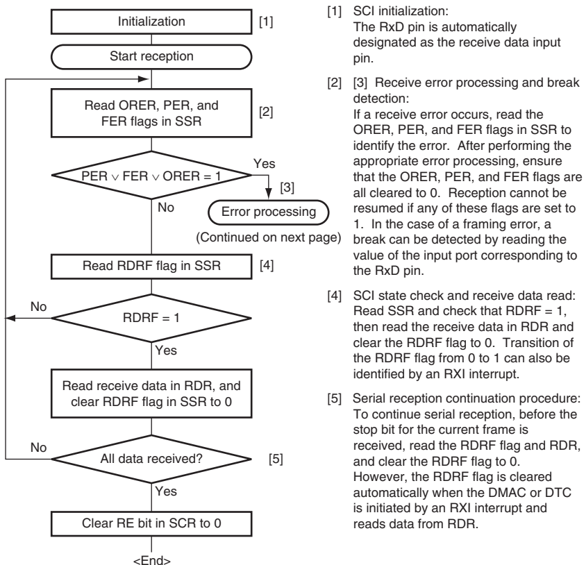
Figure 17.12 Sample Serial Reception Flowchart (1)
