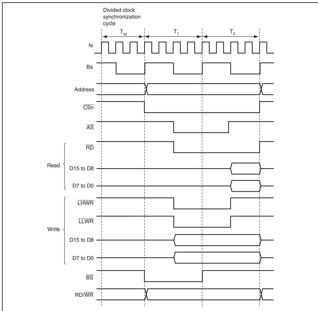
Figure 9.5 System Clock: External Bus Clock = 4:1, External 2-State Access
