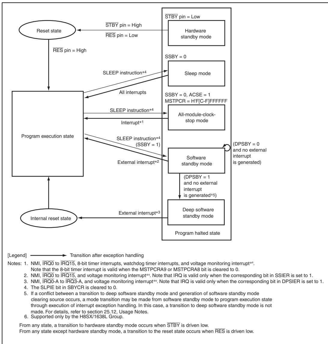
Figure 25.1 Mode Transitions
