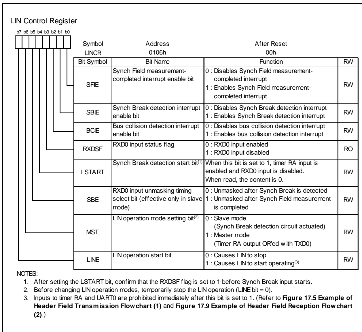
Figure 17.2 LINCX Register
