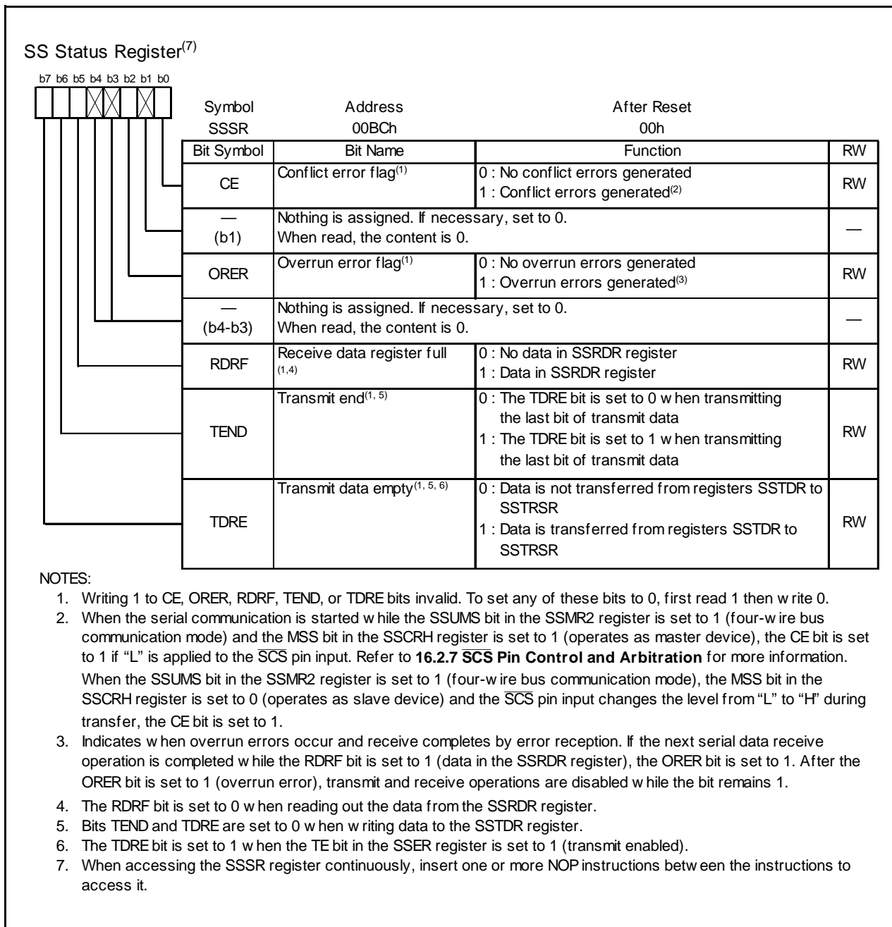
Figure 16.6 SSSR Register
