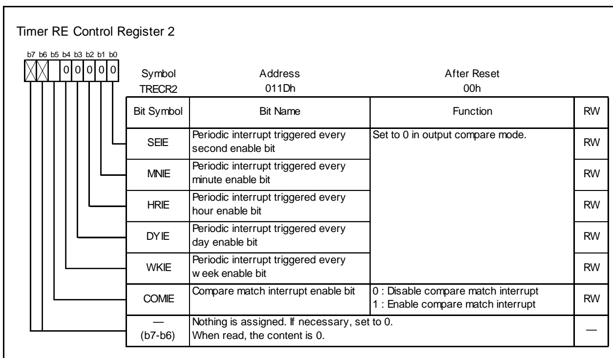
Figure 14.75 TREC2 Register in Output Compare Mode
