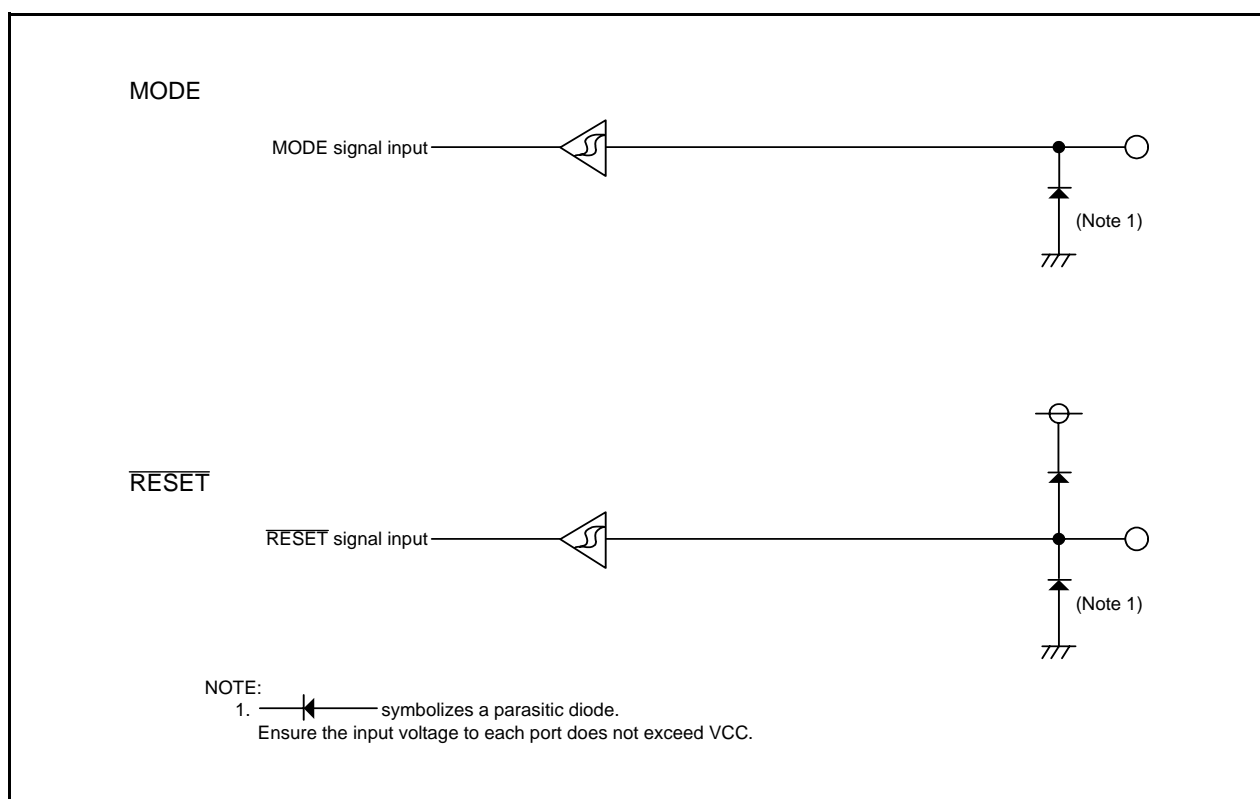
Figure 7.5 Configuration of I/O Pins
