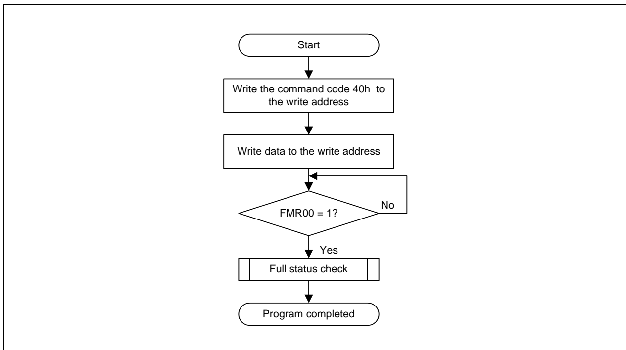
Figure 19.12 Program Command (When Suspend Function Disabled)
