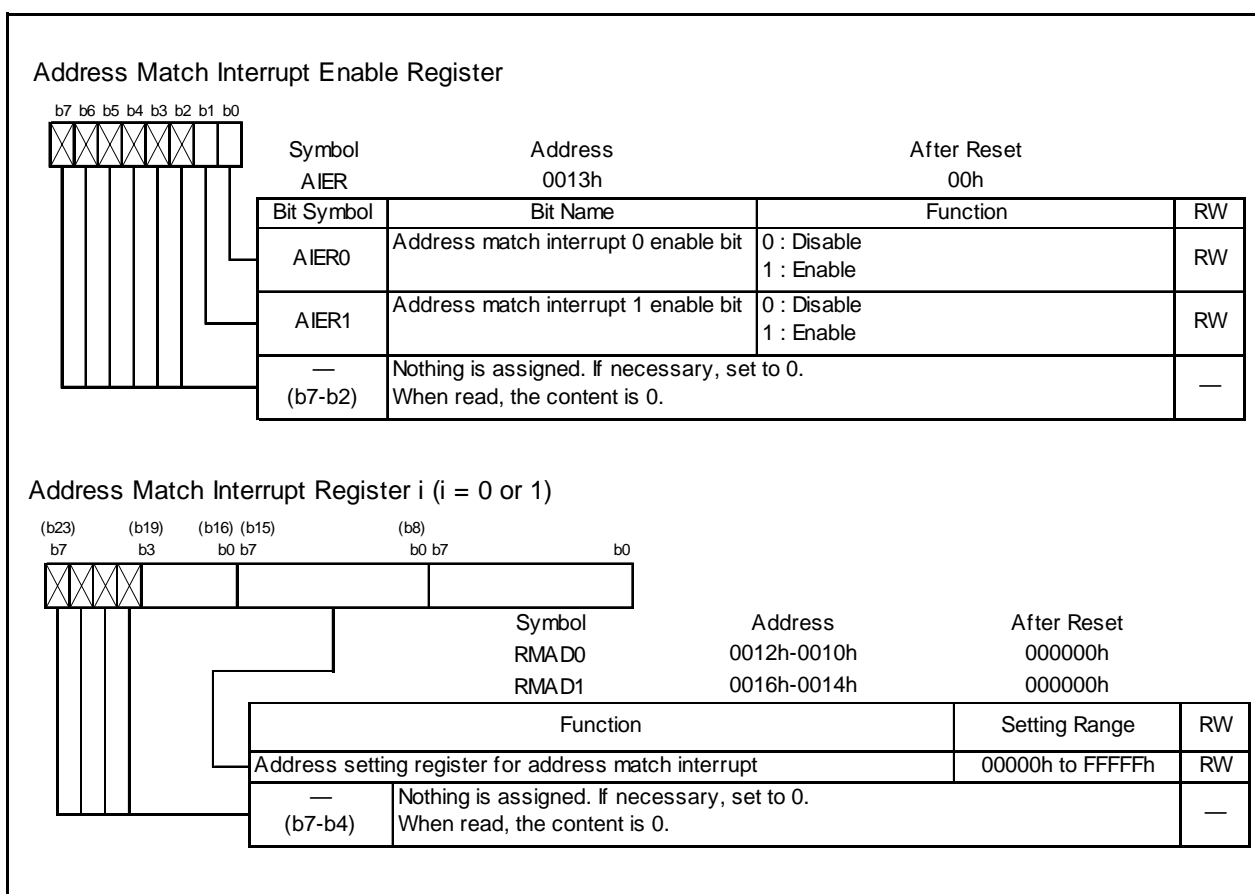
Figure 12.18 Registers AIER and RMAD0 to RMAD1
