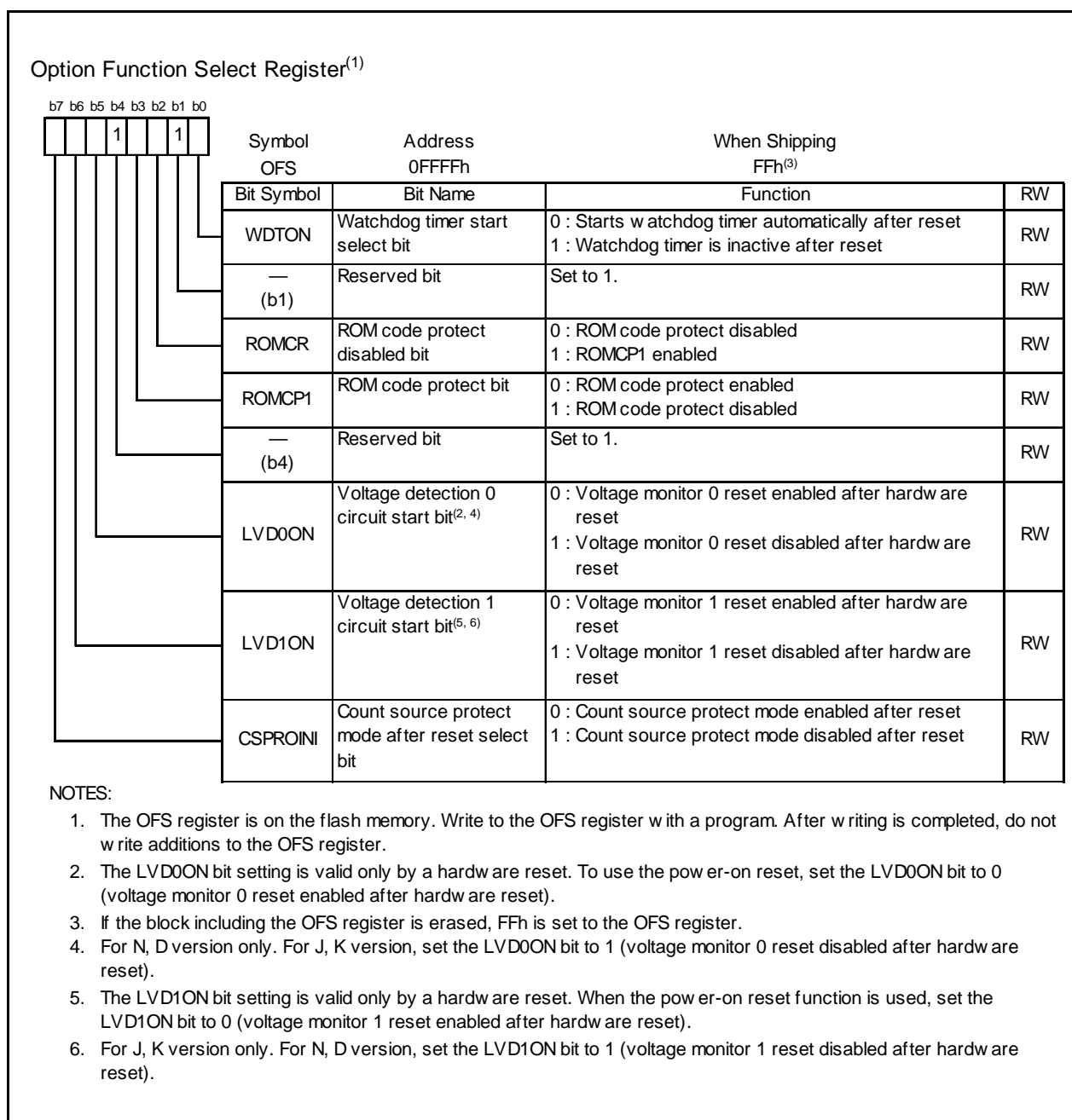
Figure 19.4 OFS Register
