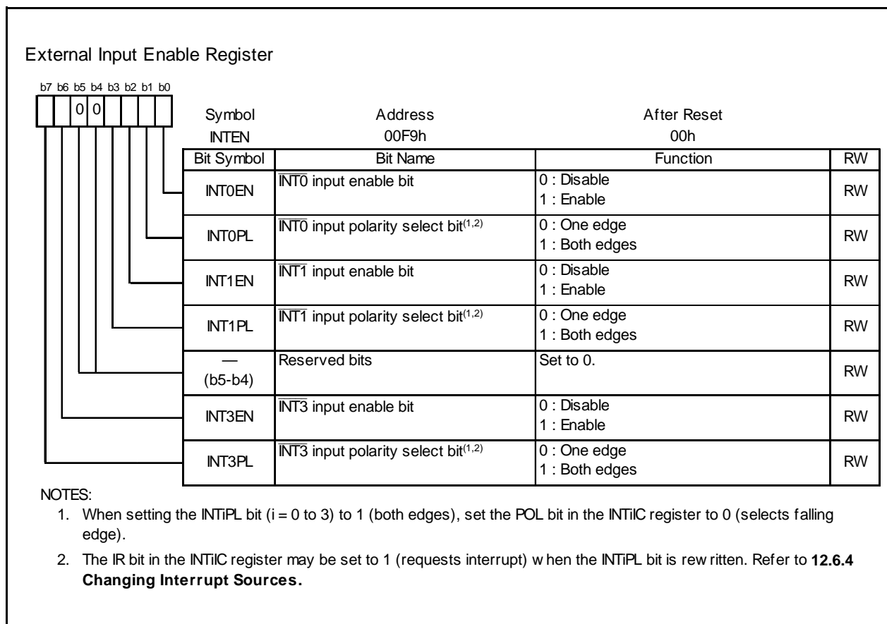
Figure 12.12 \text{INTEN} Register
