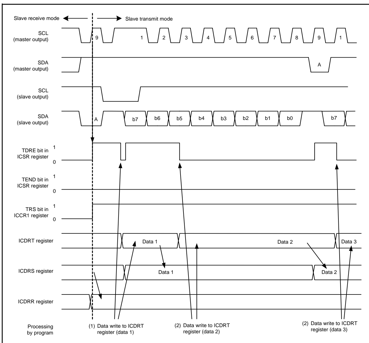
Figure 16.36 Operating Timing in Slave Transmit Mode (I 2 C bus Interface Mode) (1)
