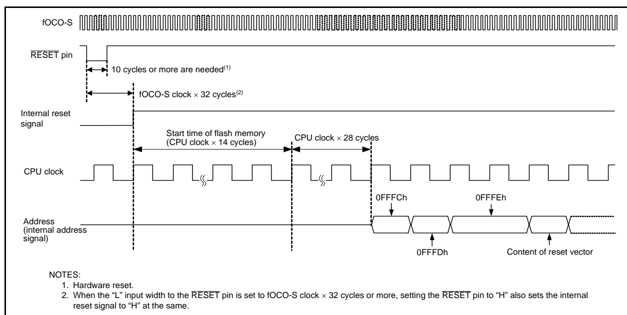
Figure 5.4 Reset Sequence
