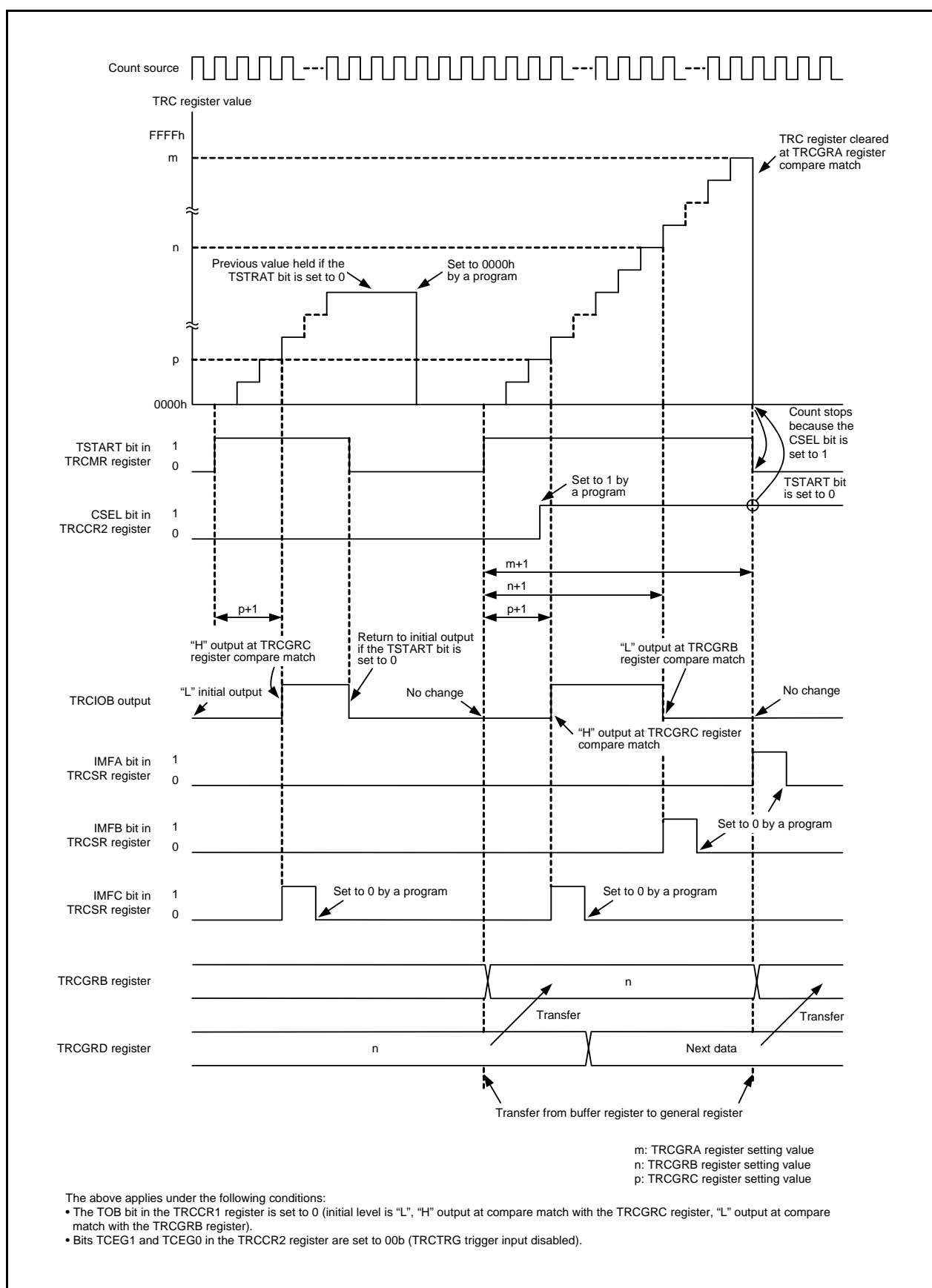
Figure 14.57 Operating Example of PWM2 Mode (TRCTRG Trigger Input Disabled)
