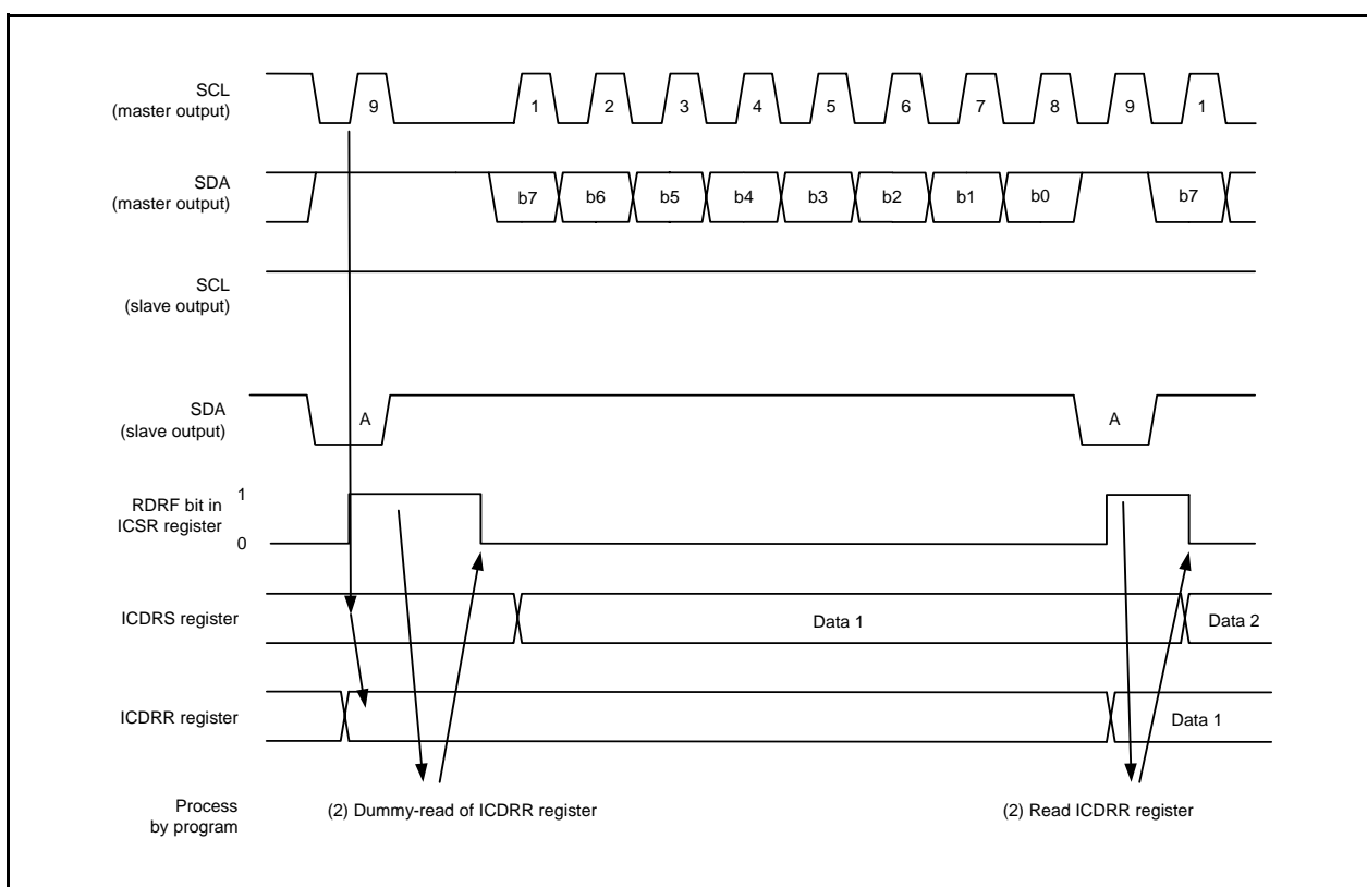
Figure 16.39 Operating Timing in Slave Receive Mode (I²C Bus Interface Mode) (1)
