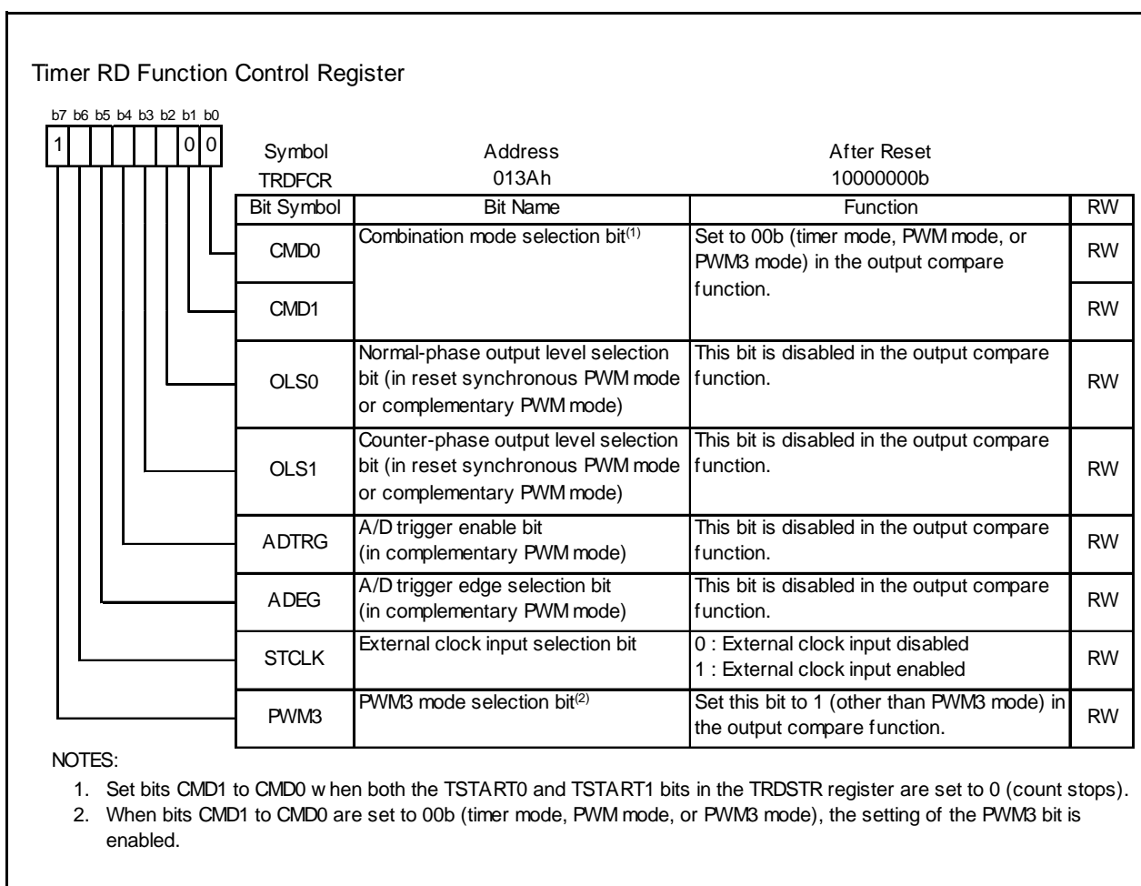
Figure 14.50 TRDFCR Register in Output Compare Function
