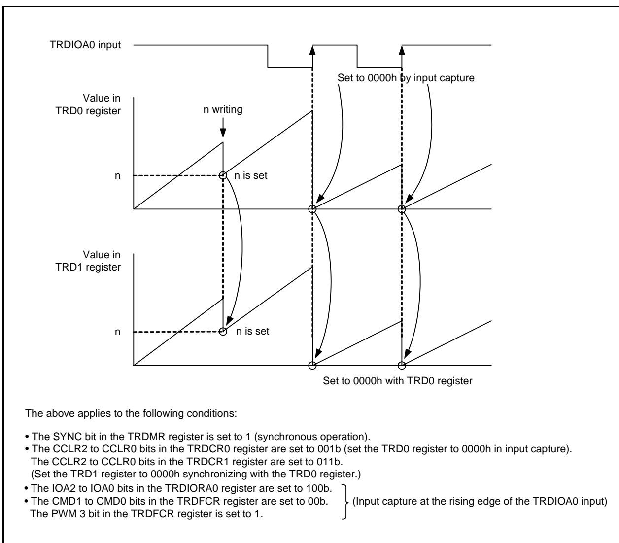
Figure 14.31 Synchronous Operation
