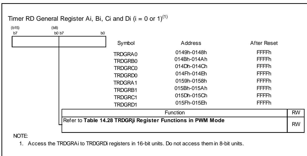
Figure 14.73 Registers TRDGRAi, TRDGRBi, TRDGRCi and TRDGRDi in PWM Mode
