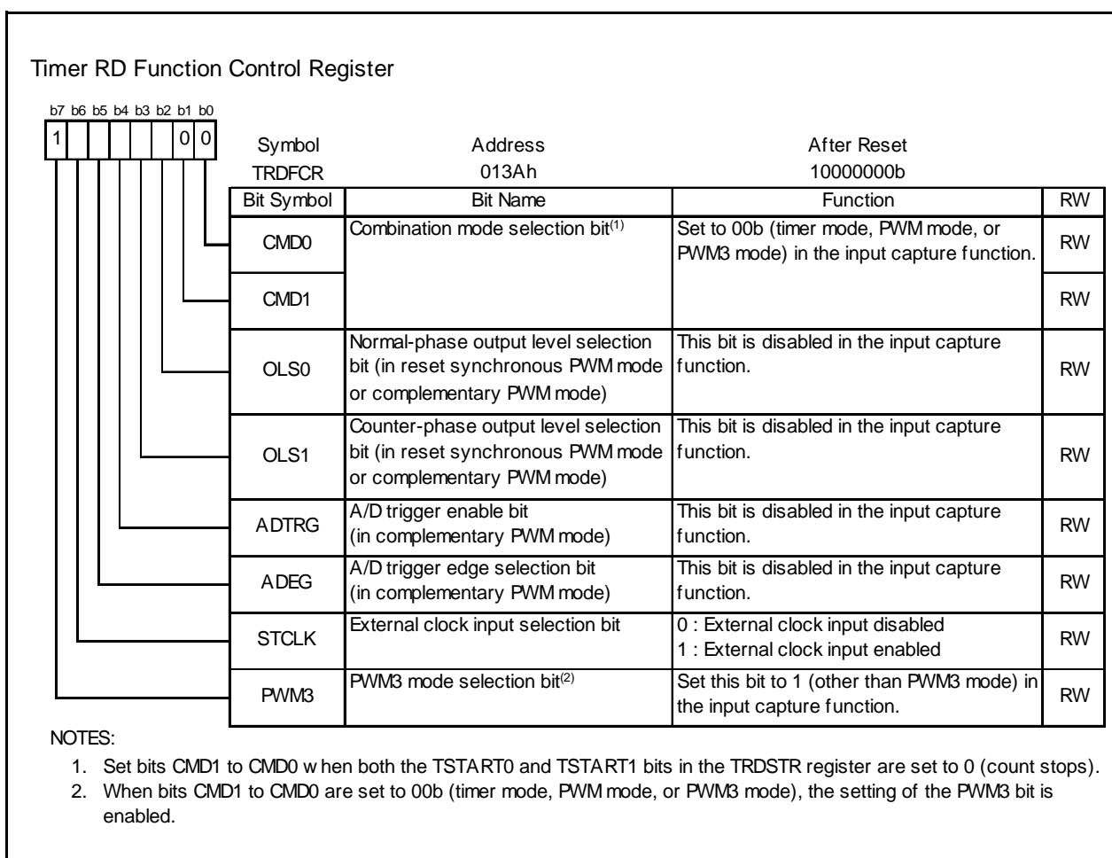
Figure 14.36 TRDFCR Register in Input Capture Function
