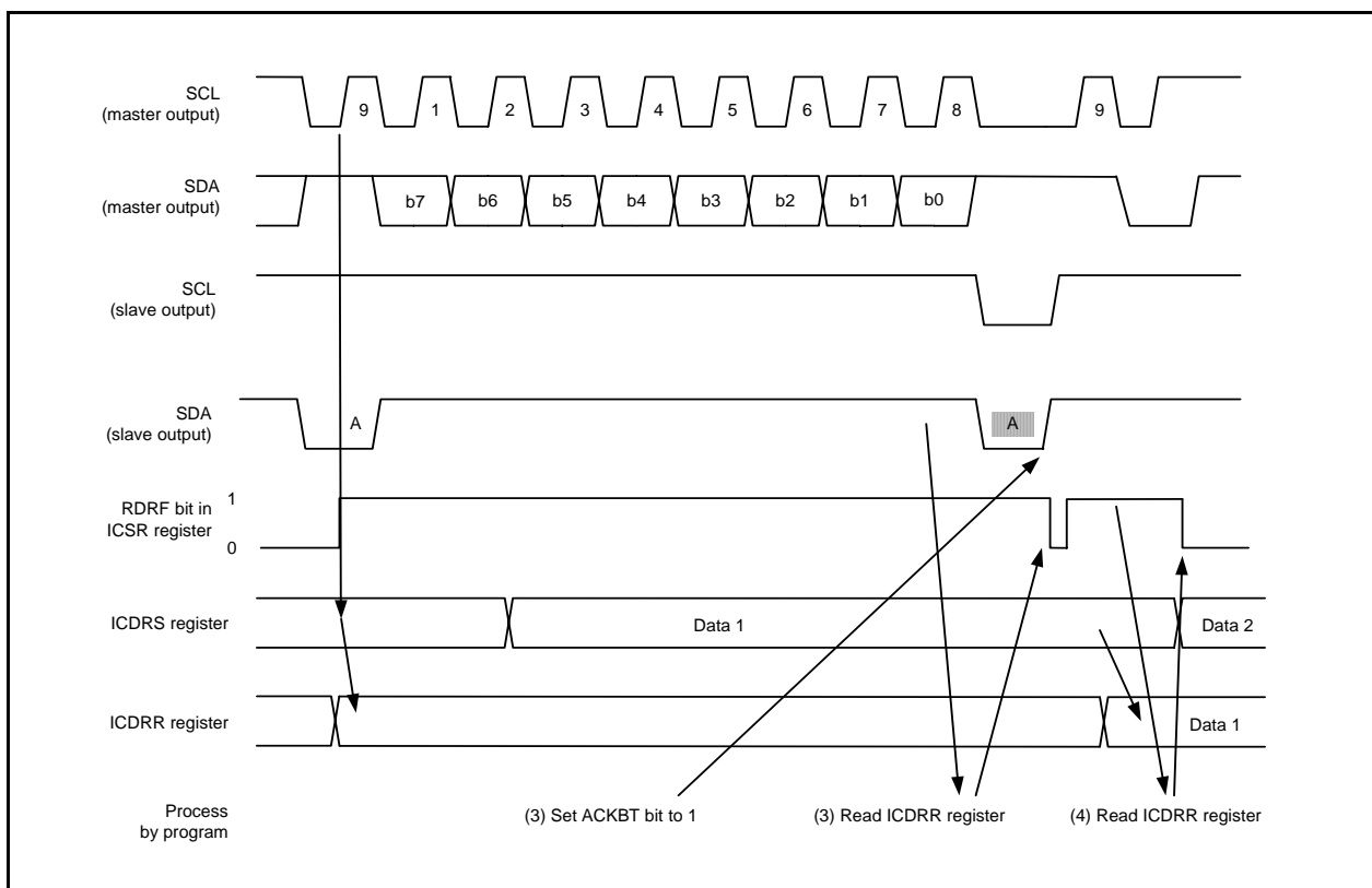
Figure 16.40 Operating Timing in Slave Receive Mode (I²C Bus Interface Mode) (2)
