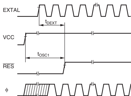
Figure 23.5 Oscillation Stabilization Timing
