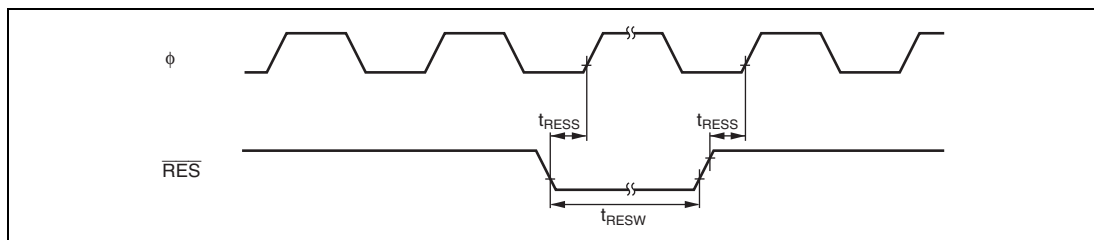
Figure 23.7 Reset Input Timing
