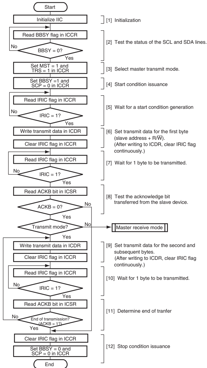
Figure 14.7 Sample Flowchart for Operations in Master Transmit Mode
