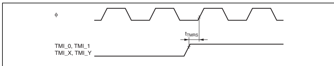
Figure 23.14 8-Bit Timer Reset Input Timing
