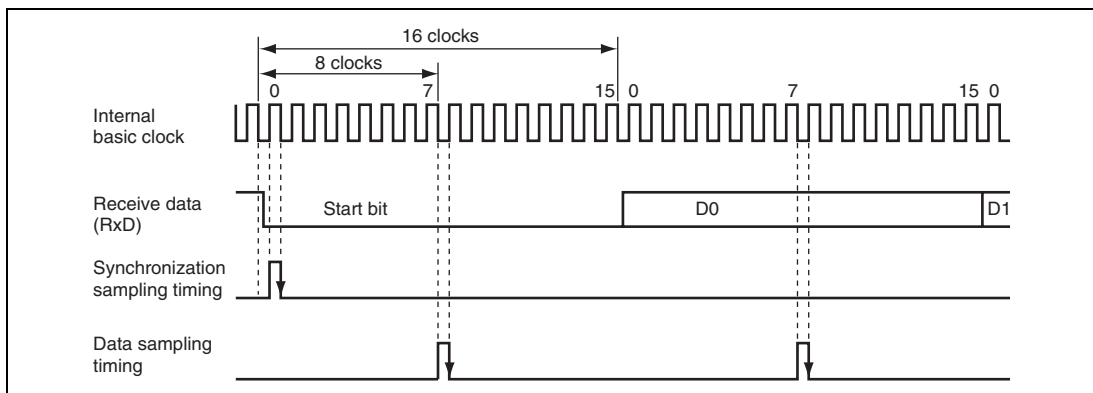
Figure 13.3 Receive Data Sampling Timing in Asynchronous Mode
