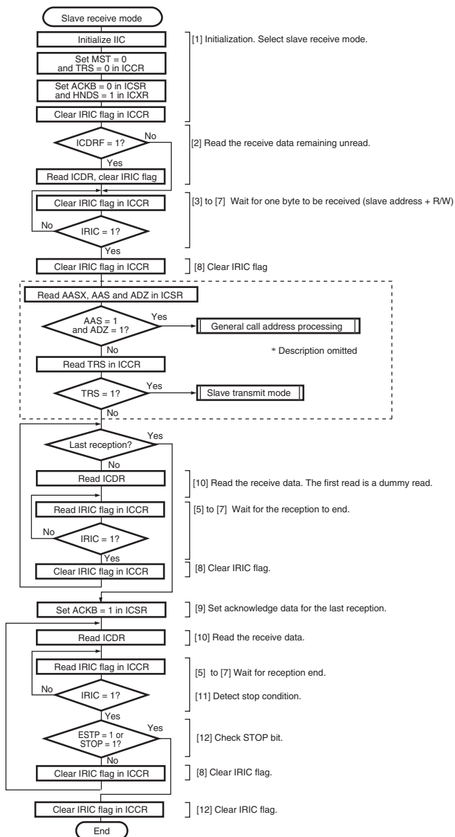
Figure 14.17 Sample Flowchart for Operations in Slave Receive Mode (HNDS = 1)
