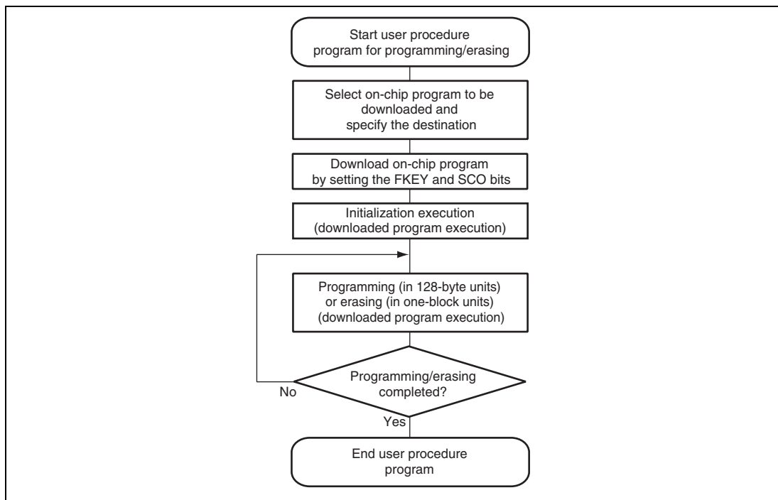
Figure 19.5 Overview of User Procedure Program
