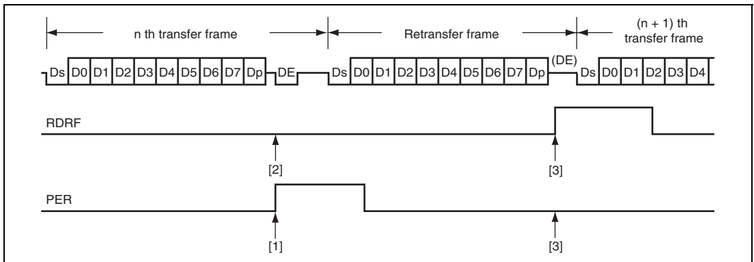
Figure 13.29 Data Re-transfer Operation in SCI Reception Mode
