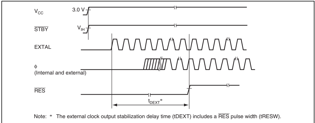
Figure 20.6 Timing of External Clock Output Stabilization Delay Time
