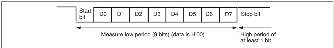
Figure 19.7 Automatic-Bit-Rate Adjustment Operation of SCI
