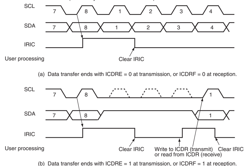
Figure 14.27 IRIC Setting Timing and SCL Control (3)
