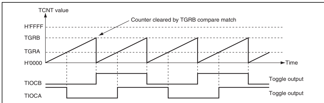
Figure 11.11 Timing of Input Capture Operation
