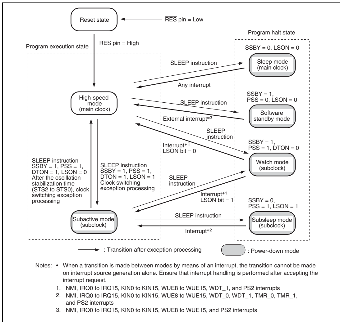
Figure 21.1 Mode Transition Diagram
