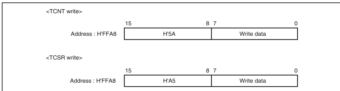
Figure 12.5 Writing to TCNT and TCSR (WDT_0)
