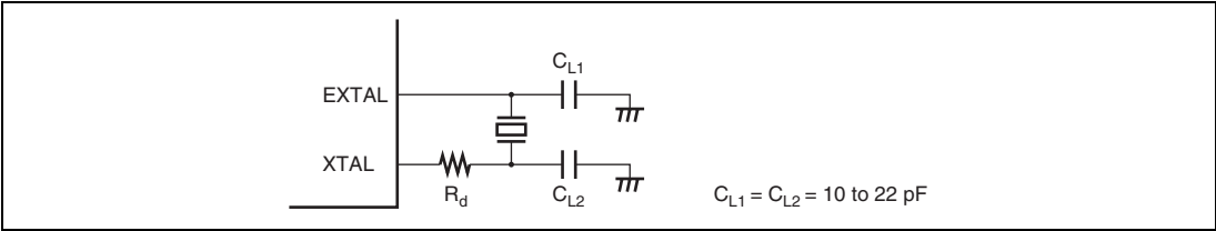
Figure 20.2 Typical Connection to Crystal Resonator
