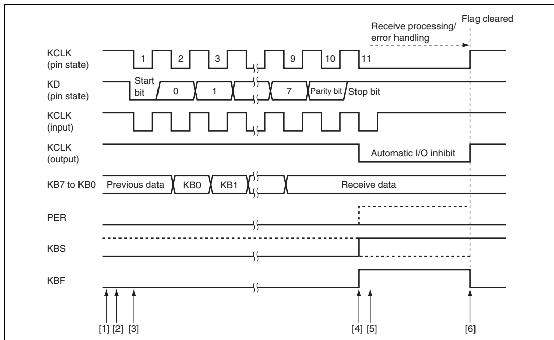
Figure 15.4 Receive Timing
