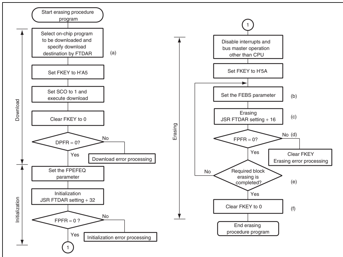
Figure 19.12 Erasing Procedure
