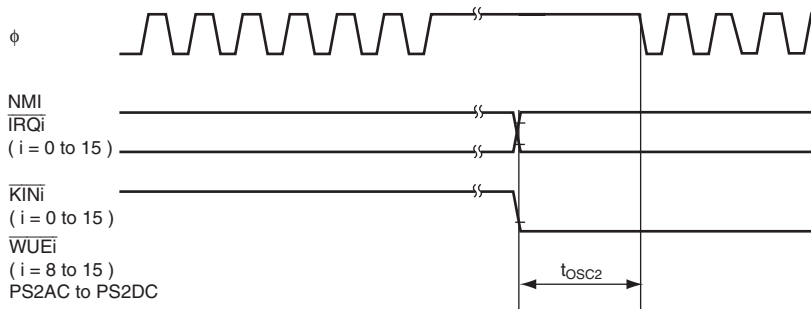
Figure 23.6 Oscillation Stabilization Timing (Exiting Software Standby Mode)
