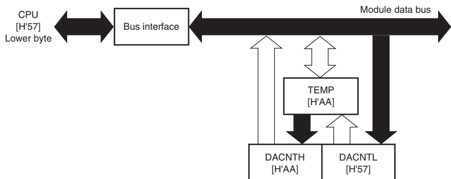
Figure 9.2 DACNT Access Operation (1) [CPU → DACNT (H'AA57) Writing]
