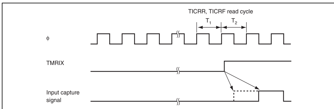
Figure 11.12 Timing of Input Capture Signal (Input capture signal is input during TICRR and TICRF read)
