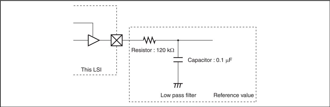
Figure 8.5 Example Circuit when Using PWM as D/A
