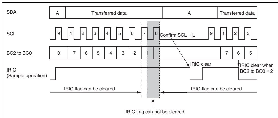
Figure 14.36 IRIC Flag Clearing Timing in Wait Operation
