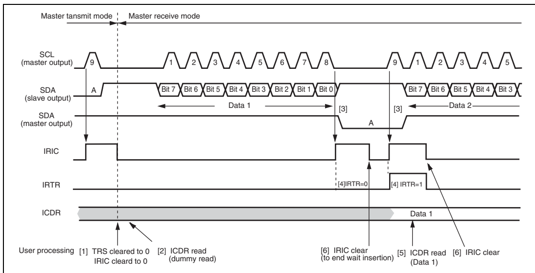
Figure 14.15 Example of Master Receive Mode Operation Timing (MLS = ACKB = 0, WAIT = 1)
