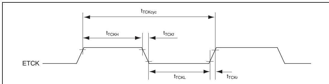
Figure 23.22 JTAG ETCK Timing
