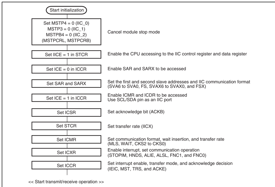
Figure 14.6 Sample Flowchart for IIC Initialization
