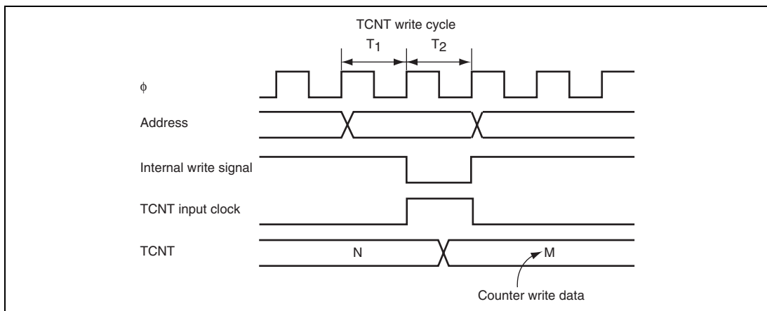
Figure 12.6 Conflict between TCNT Write and Increment
