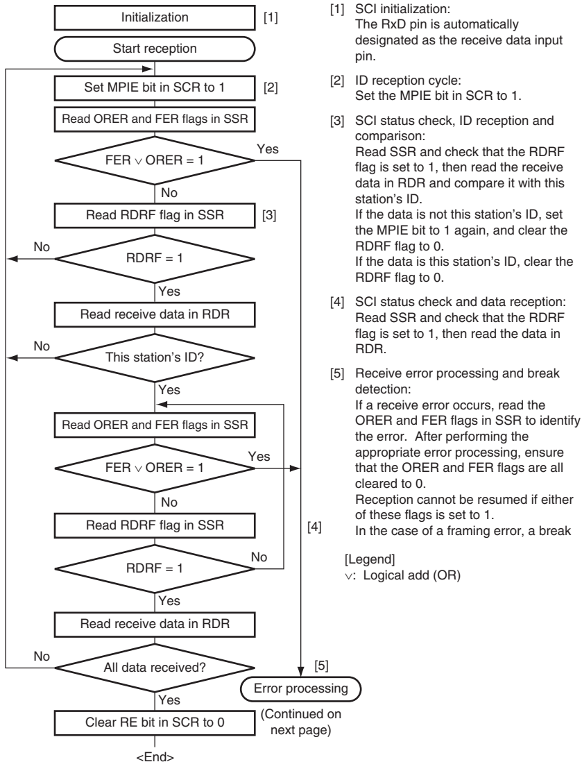
Figure 13.13 Sample Multiprocessor Serial Reception Flowchart (1)
