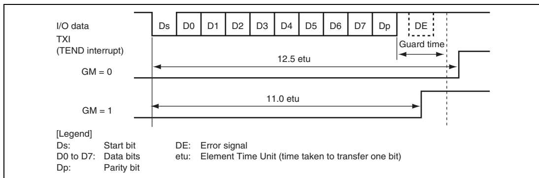
Figure 13.27 TEND Flag Set Timings during Transmission
