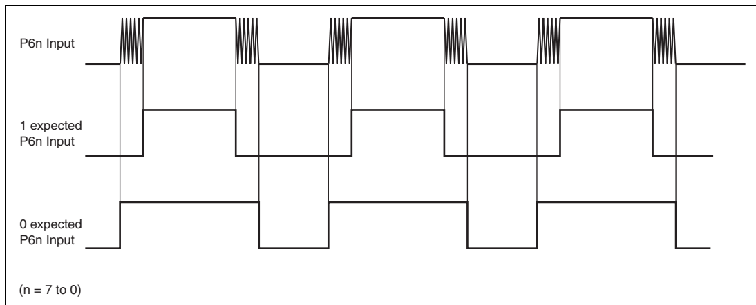
Figure 7.2 Noise Cancel Operation
