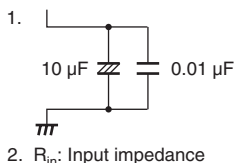
Figure 17.6 Example of Analog Input Protection Circuit
