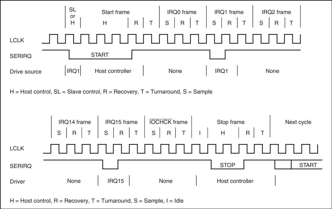
Figure 16.6 SERIRQ Timing
