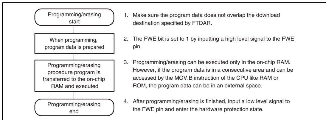
Figure 19.9 Programming/Erasing Overview Flow
