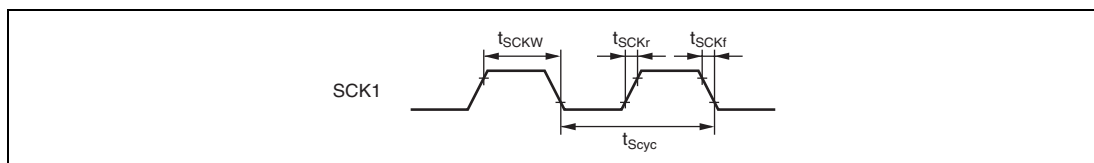
Figure 23.16 SCK Clock Input Timing
