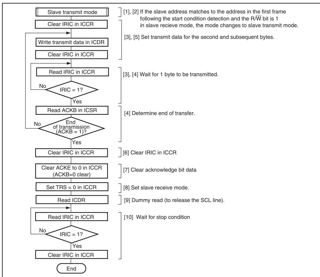
Figure 14.23 Sample Flowchart for Slave Transmit Mode
