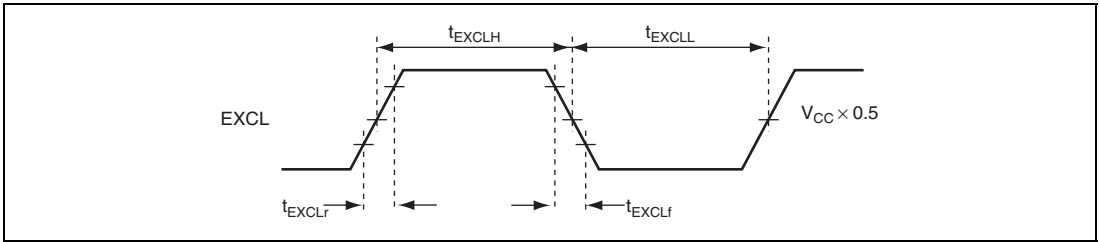
Figure 20.8 Subclock Input Timing
