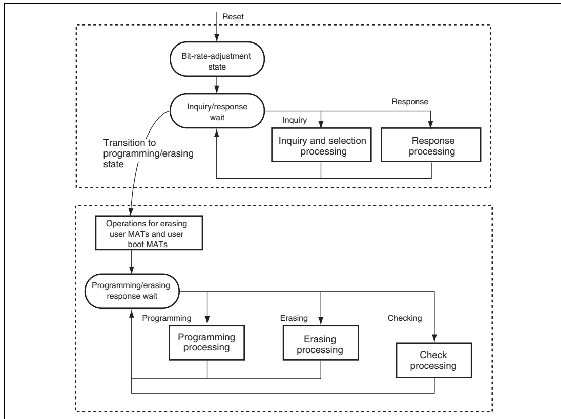
Figure 19.19 Boot Program States
