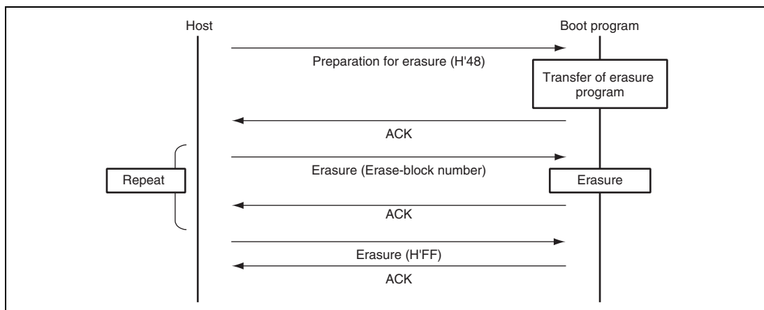
Figure 19.24 Erasure Sequence
