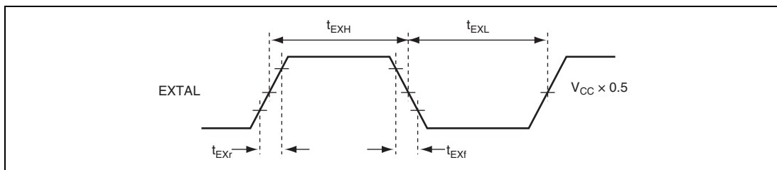
Figure 20.5 External Clock Input Timing
