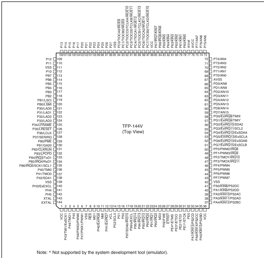
Figure 1.2 H8S/2116 Group Pin Arrangement (TFP-144V)
