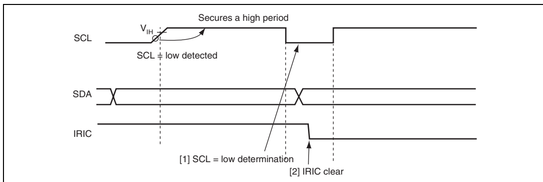
Figure 14.32 IRIC Flag Clearing Timing when WAIT = 1
