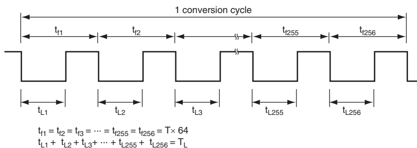
(a) CFS = 0 [base cycle = resolution ( T \times 64 )]
