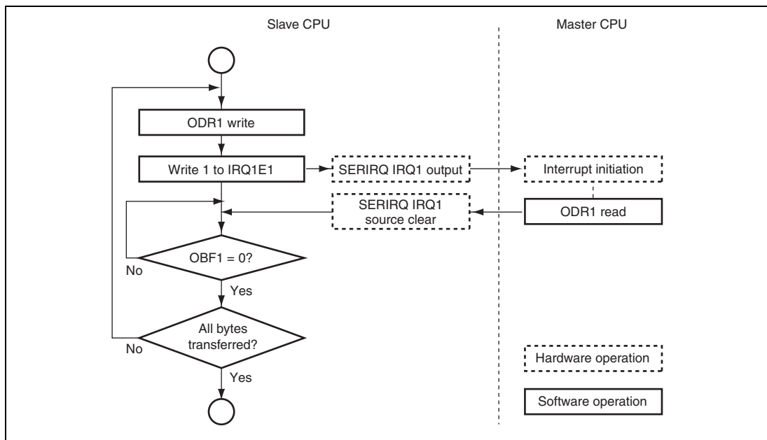
Figure 16.8 HIRQ Flowchart (Example of Channel 1)
