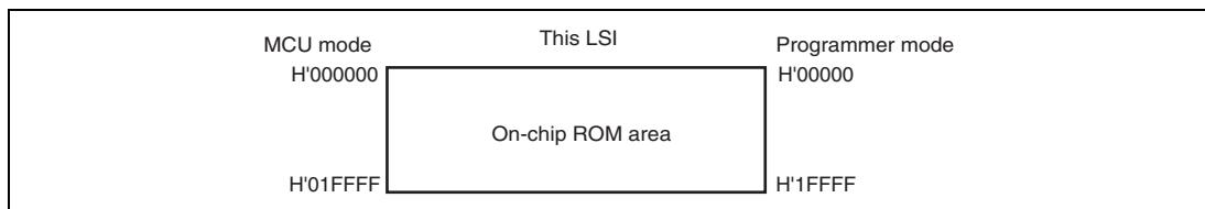
Figure 19.18 Memory Map in Programmer Mode
