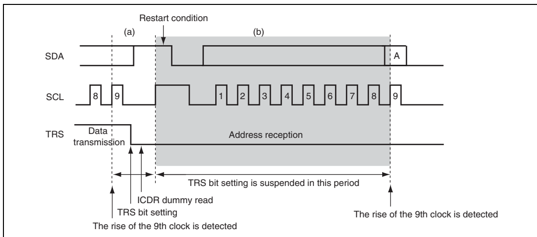
Figure 14.34 TRS Bit Set Timing in Slave Mode
