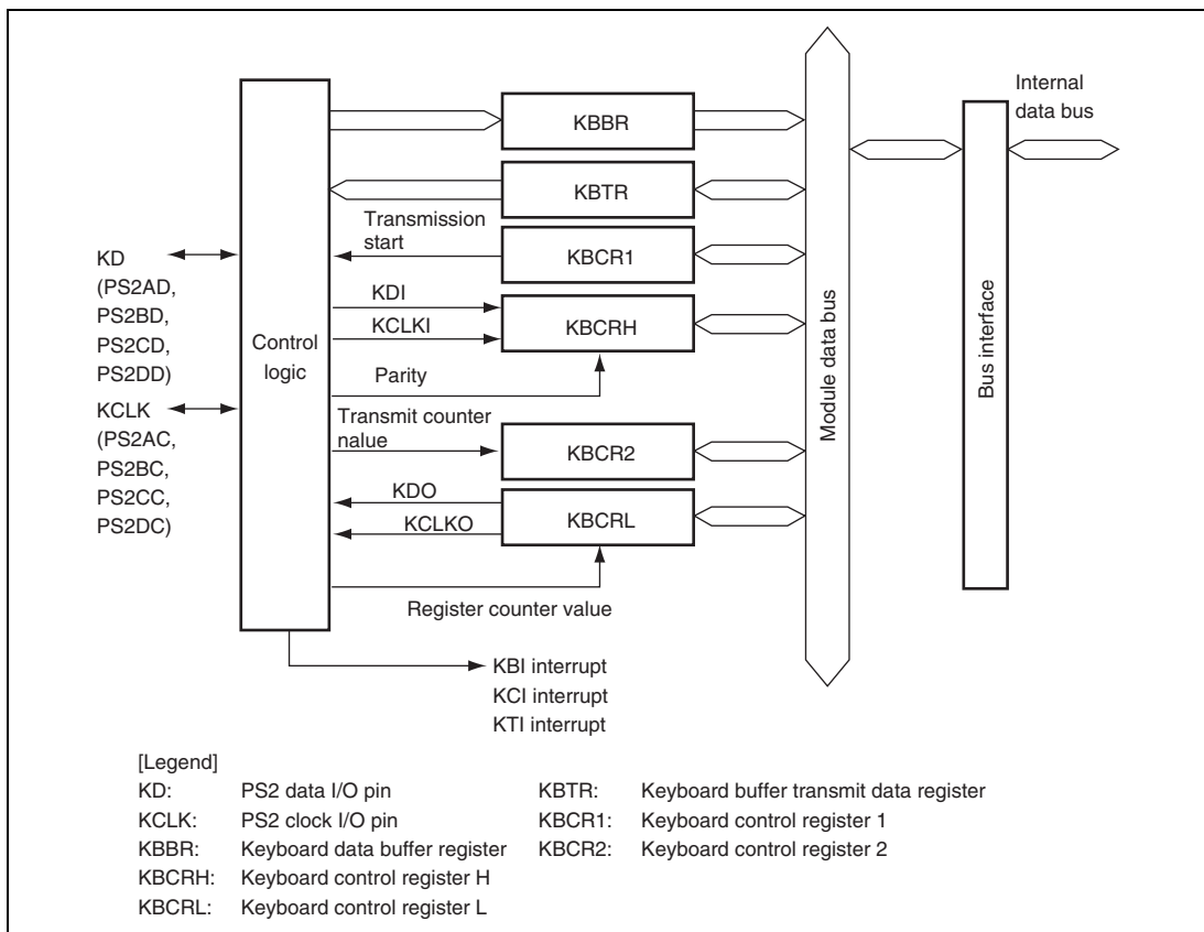
Figure 15.1 Block Diagram of PS2
