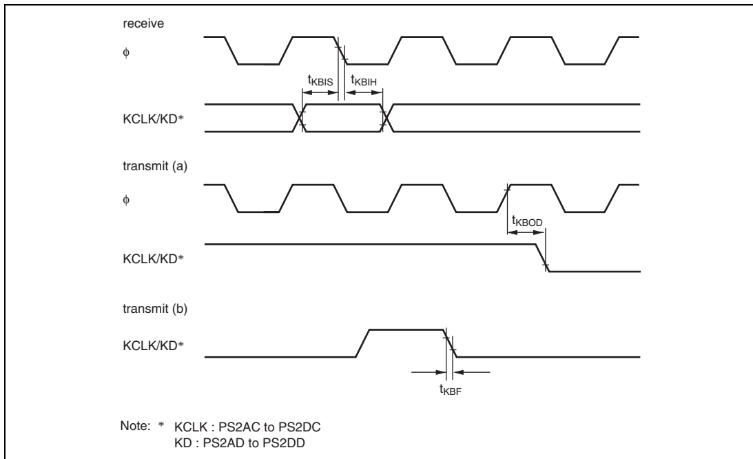
Figure 23.18 PS2 Timing
