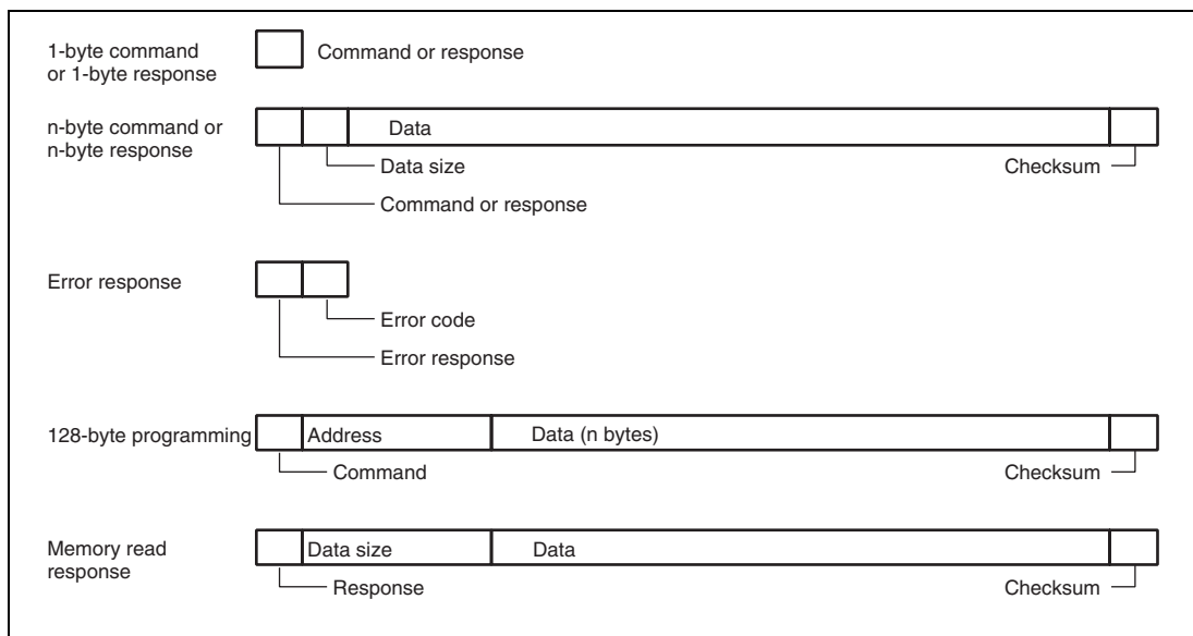
Figure 19.21 Communication Protocol Format
