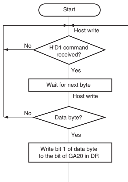
Figure 16.4 GA20 Output
