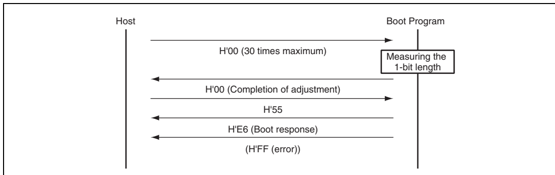
Figure 19.20 Bit-Rate-Adjustment Sequence
