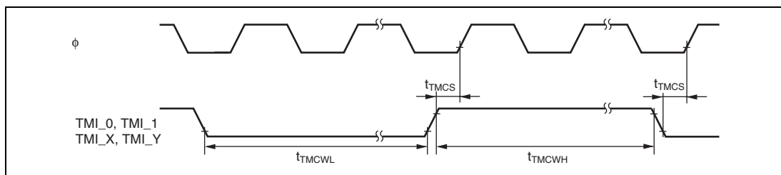
Figure 23.13 8-Bit Timer Clock Input Timing
