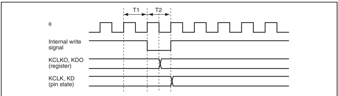
Figure 15.10 KCLKO and KDO Write Timing
