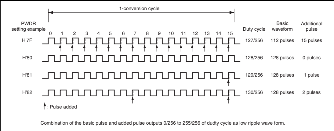
Figure 8.4 Example of PWM Setting
