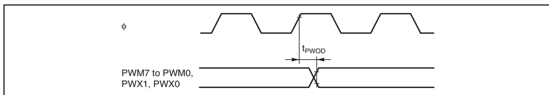
Figure 23.15 PWM, PWMX Output Timing
