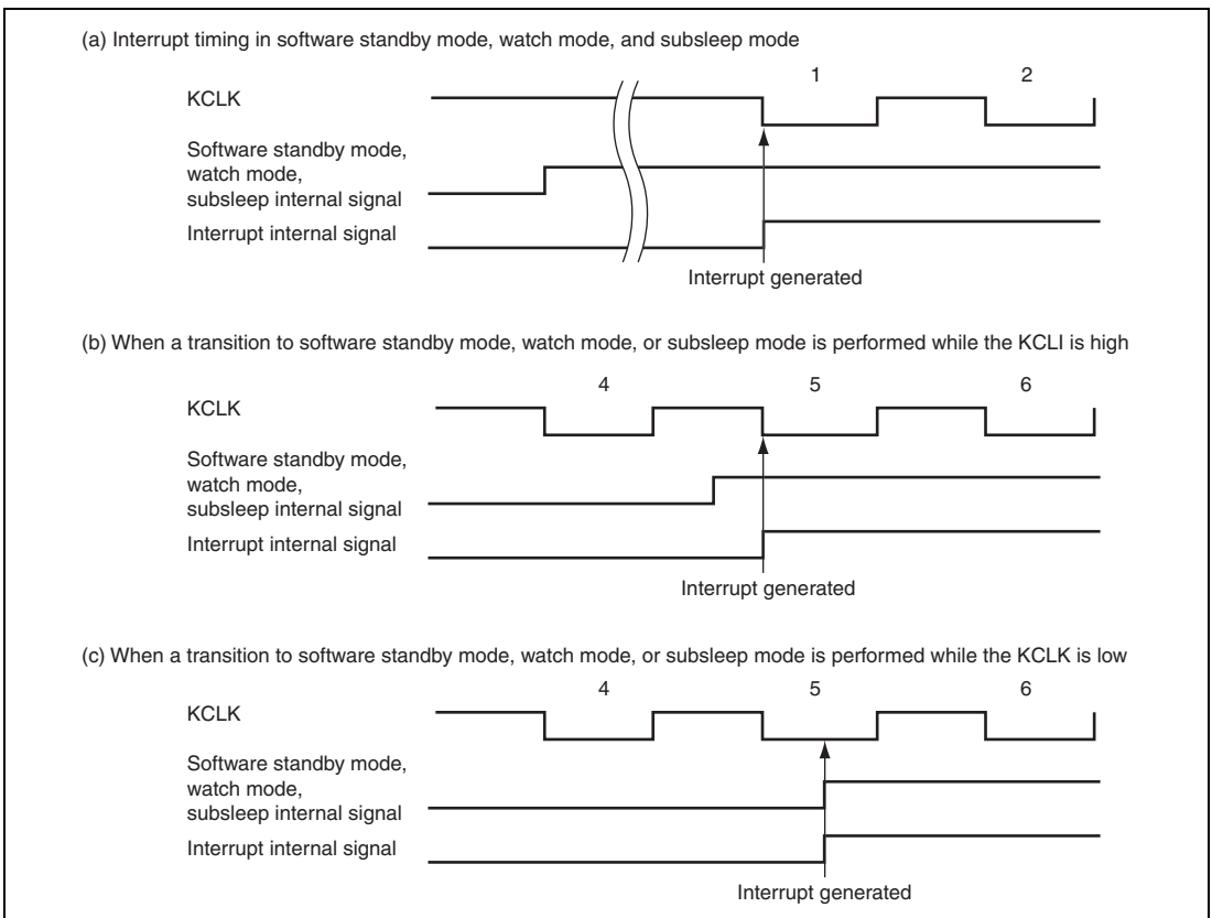
Figure 15.17 Interrupt Timing in Software Standby Mode, Watch Mode, and Subsleep Mode
