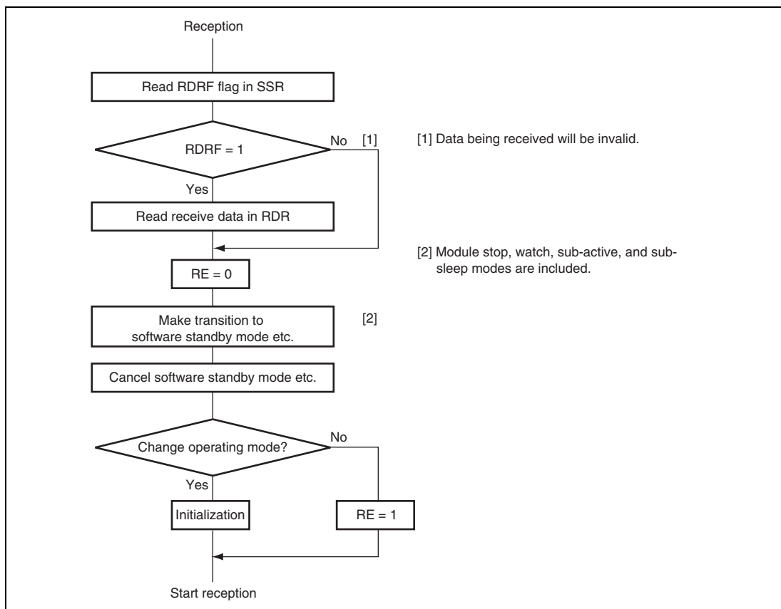
Figure 13.36 Sample Flowchart for Mode Transition during Reception
