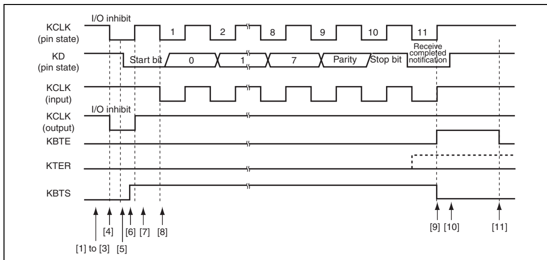
Figure 15.6 Transmit Timing
