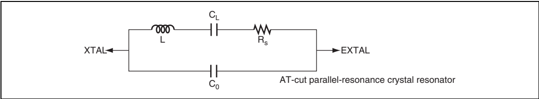
Figure 20.3 Equivalent Circuit of Crystal Resonator
