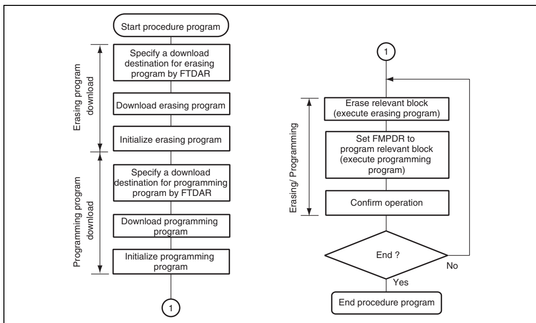
Figure 19.13 Repeating Procedure of Erasing and Programming
