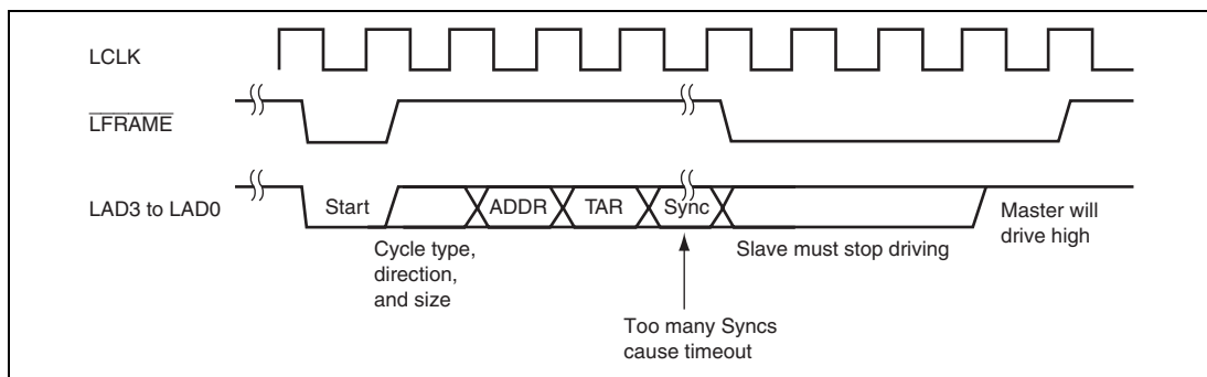
Figure 16.3 Abort Mechanism
