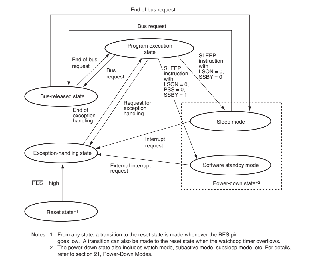
Figure 2.13 State Transitions
