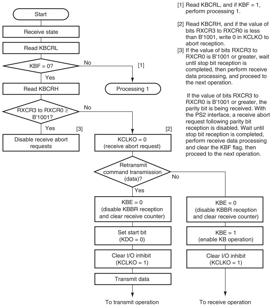
Figure 15.7 Sample Receive Abort Processing Flowchart (1)
