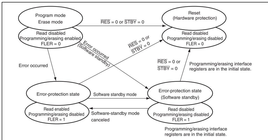
Figure 19.16 Transitions to Error-Protection State
