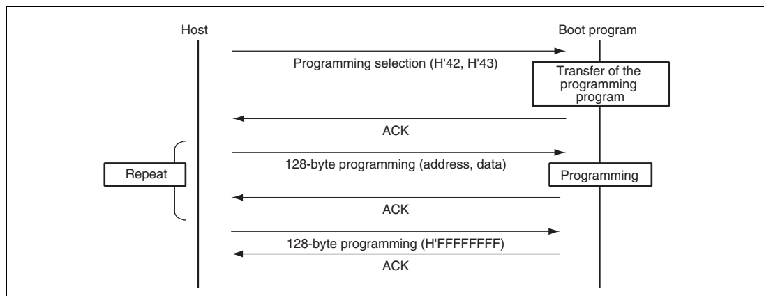
Figure 19.23 Programming Sequence
