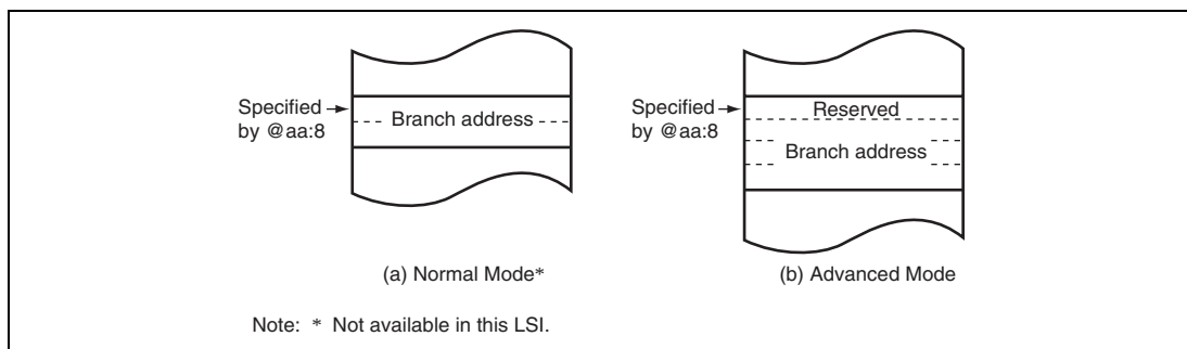
Figure 2.12 Branch Address Specification in Memory Indirect Addressing Mode
