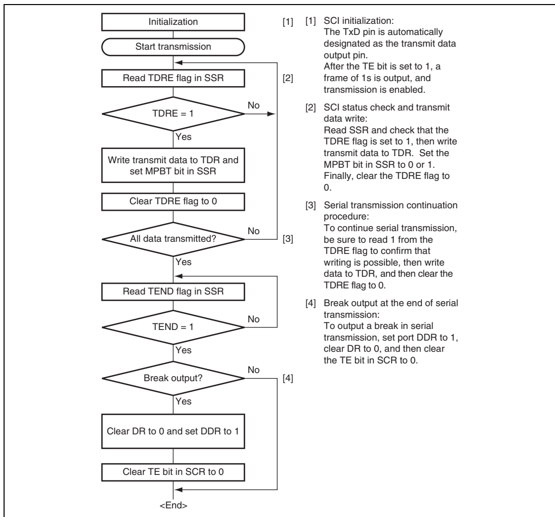
Figure 13.11 Sample Multiprocessor Serial Transmission Flowchart
