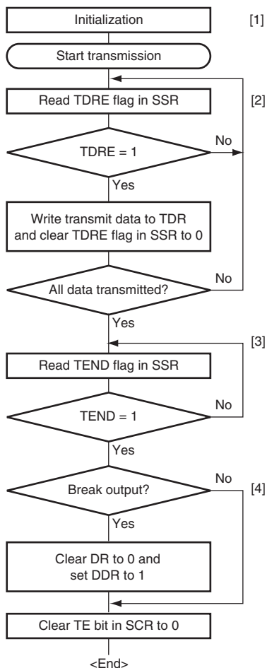
Figure 13.7 Sample Serial Transmission Flowchart
