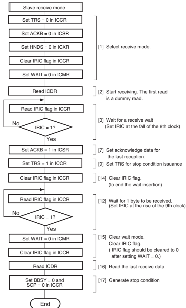
Figure 14.14 Sample Flowchart for Operations in Master Receive Mode (receiving a single byte) (WAIT = 1)
