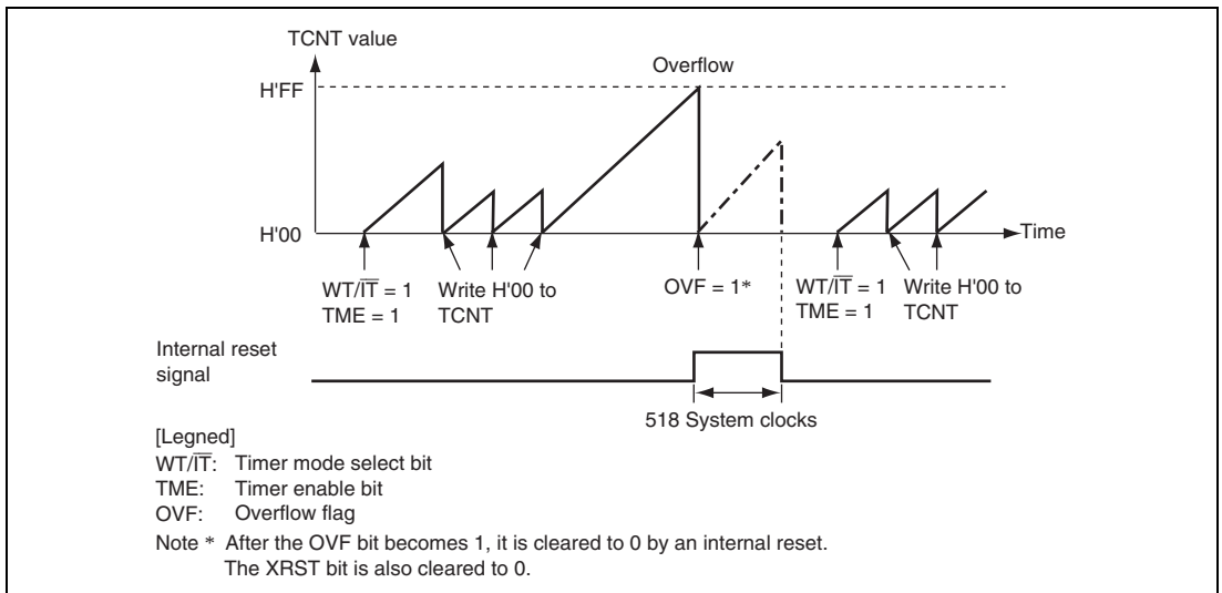
Figure 12.2 Watchdog Timer Mode ( \text{RST}/\overline{\text{NMI}} = 1 ) Operation
