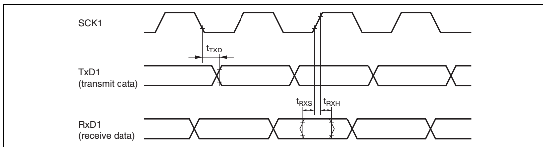
Figure 23.17 SCI Input/Output Timing (Clock Synchronous Mode)
