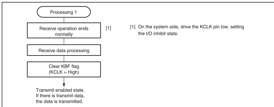
Figure 15.7 Sample Receive Abort Processing Flowchart (2)
