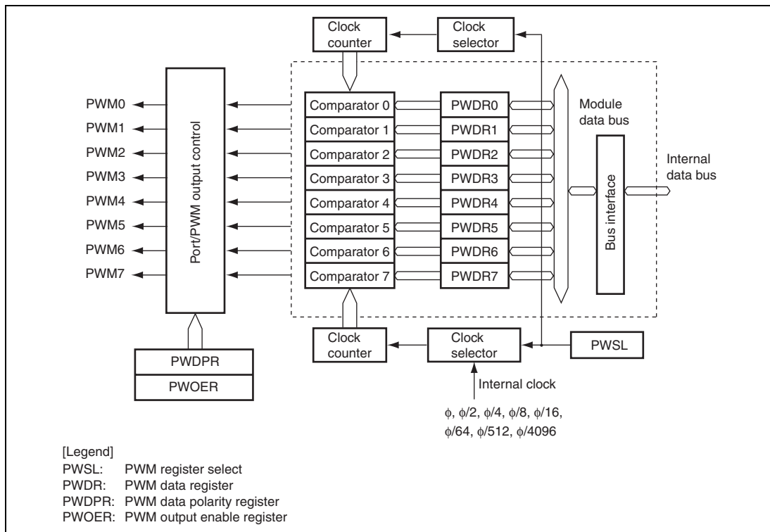
Figure 8.1 Block Diagram of PWM Timer
