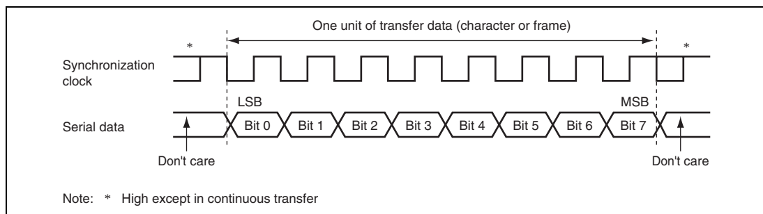
Figure 13.14 Data Format in Synchronous Communication (LSB-First)
