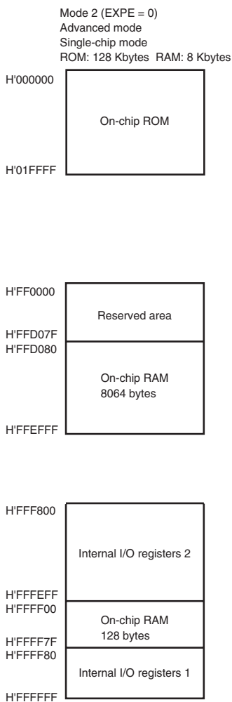
Figure 3.1 Address Map
