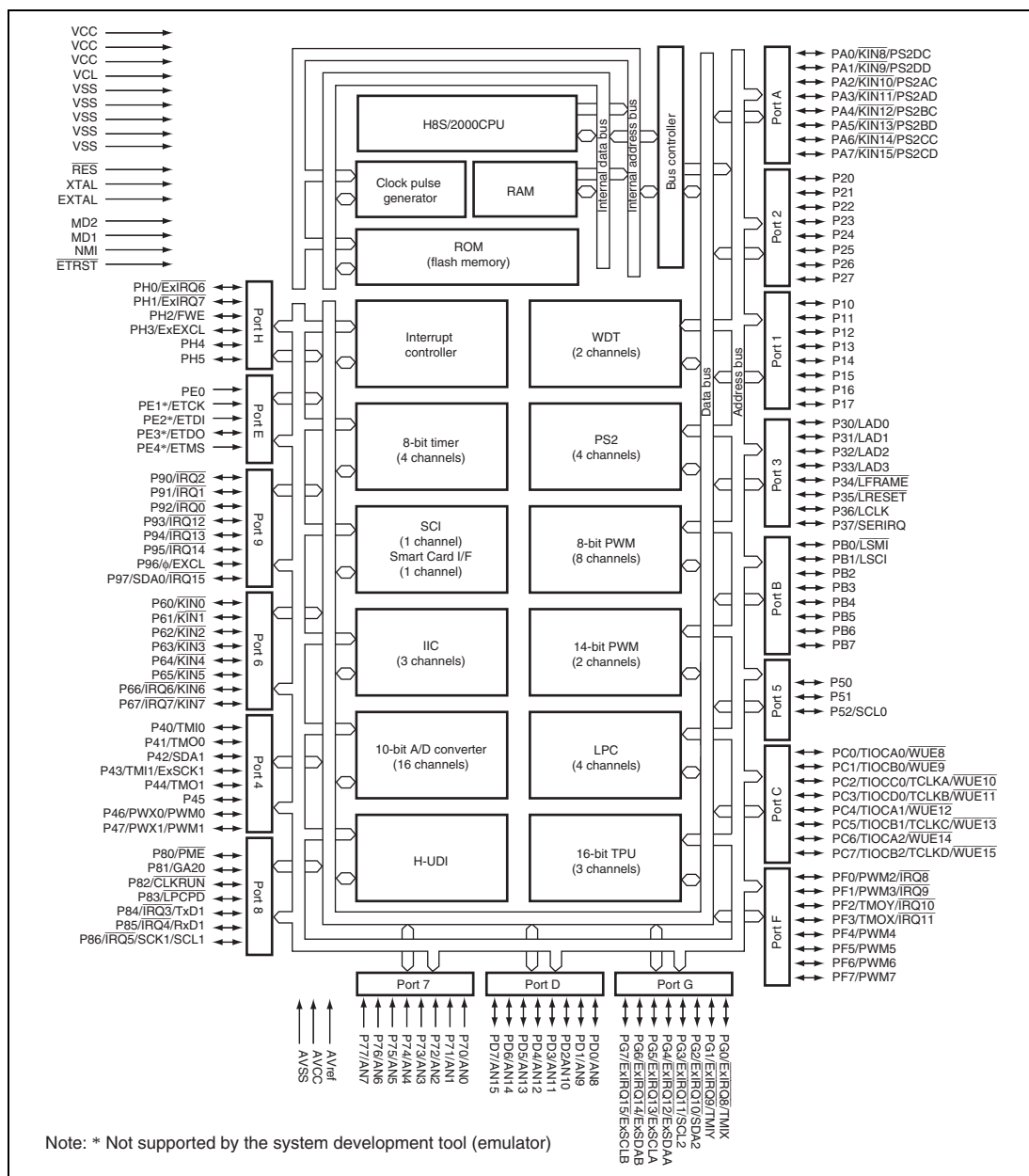
Figure 1.1 H8S/2116 Group Internal Block Diagram
