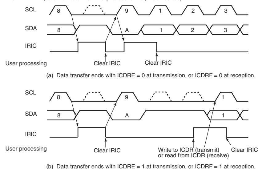
Figure 14.26 IRIC Setting Timing and SCL Control (2)
