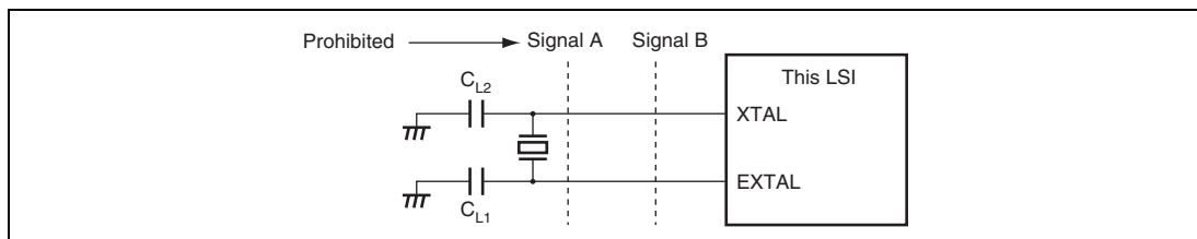
Figure 20.9 Note on Board Design of Oscillator Section
