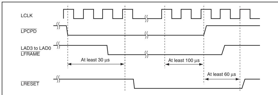
Figure 16.5 Power-Down State Termination Timing
