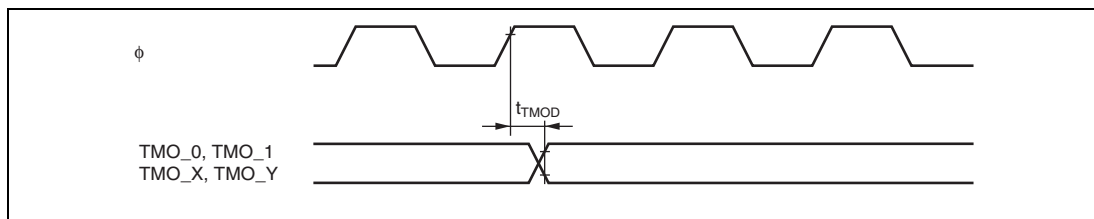
Figure 23.12 8-Bit Timer Output Timing
