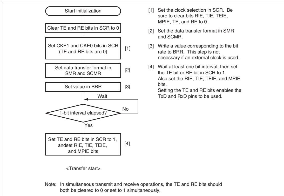
Figure 13.15 Sample SCI Initialization Flowchart
