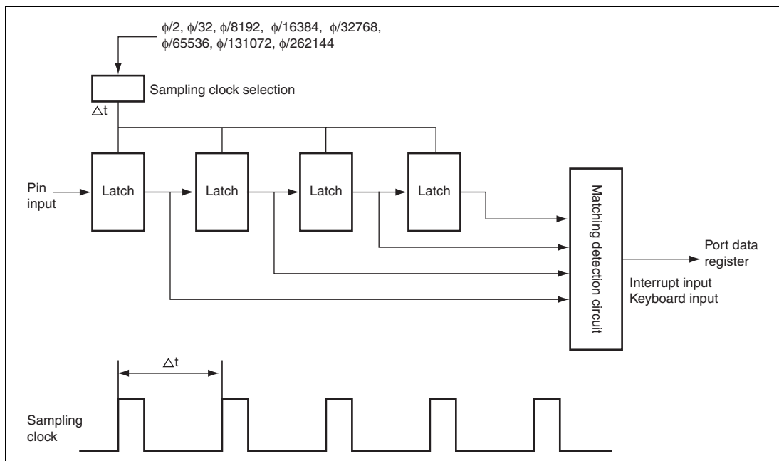
Figure 7.1 Noise Cancel Circuit
