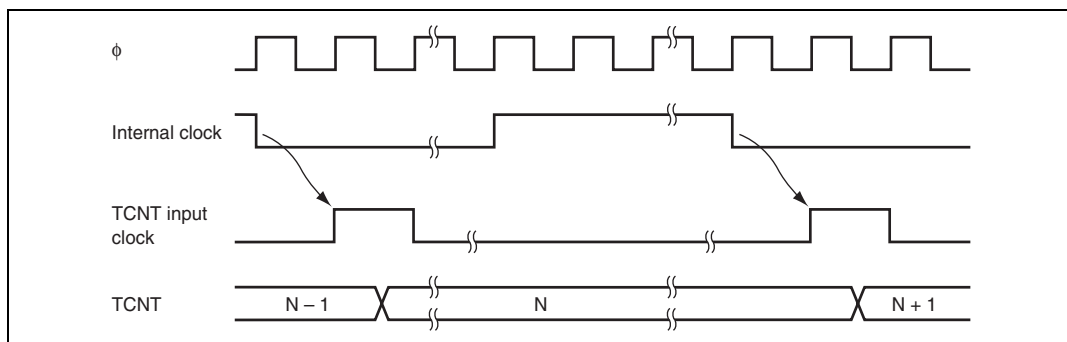
Figure 11.4 Count Timing for Internal Clock Input
