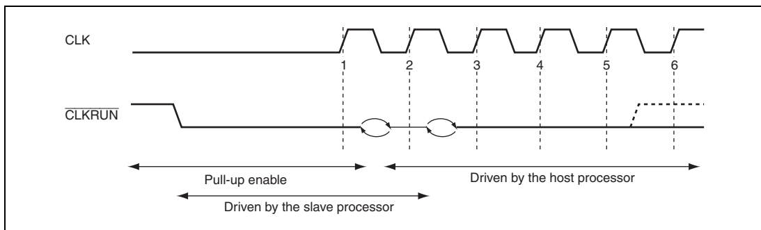
Figure 16.7 Clock Start Request Timing
