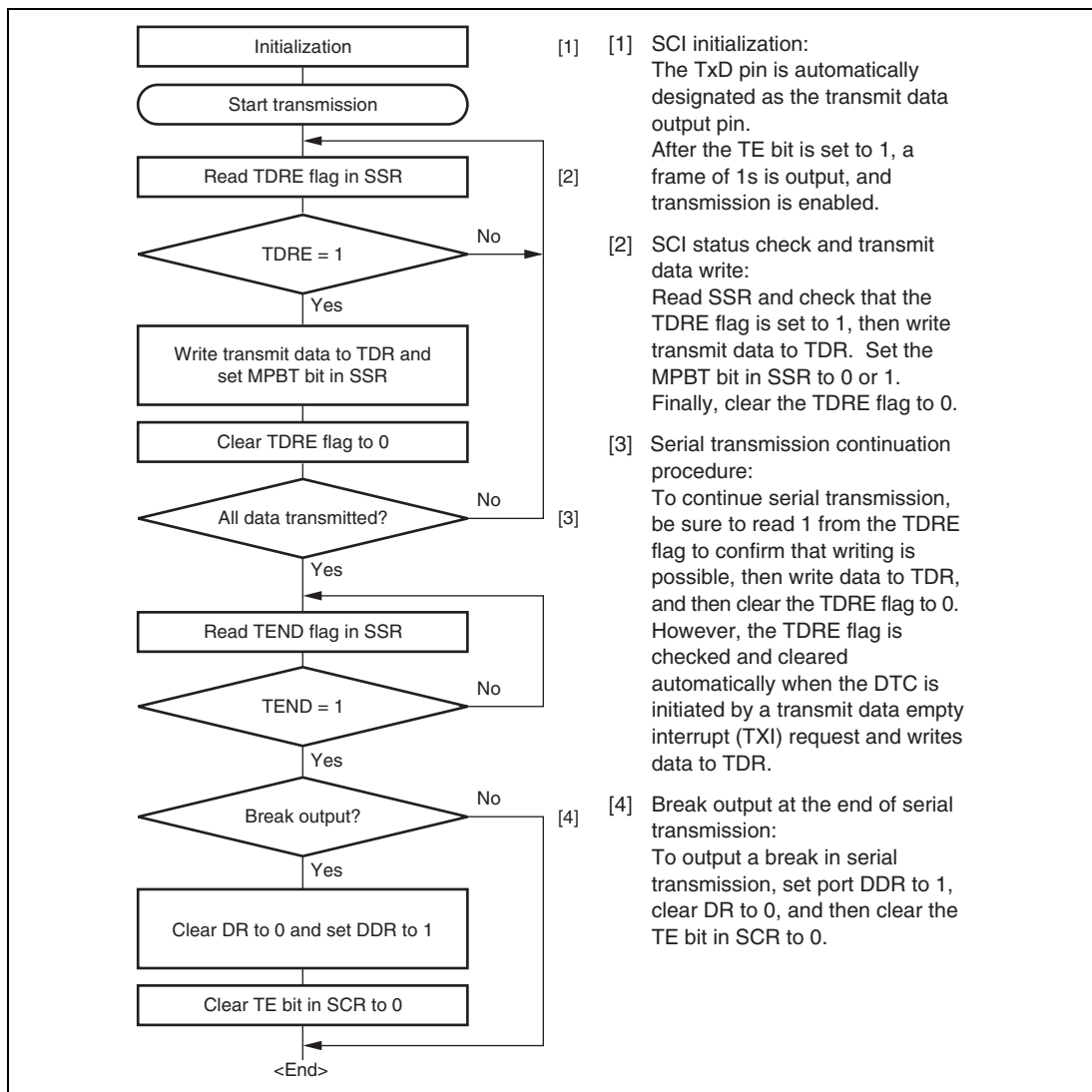
Figure 15.11 Sample Multiprocessor Serial Transmission Flowchart
