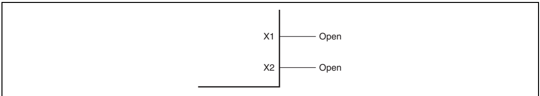
Figure 23.9 Handling of X1 and X2 Pins
