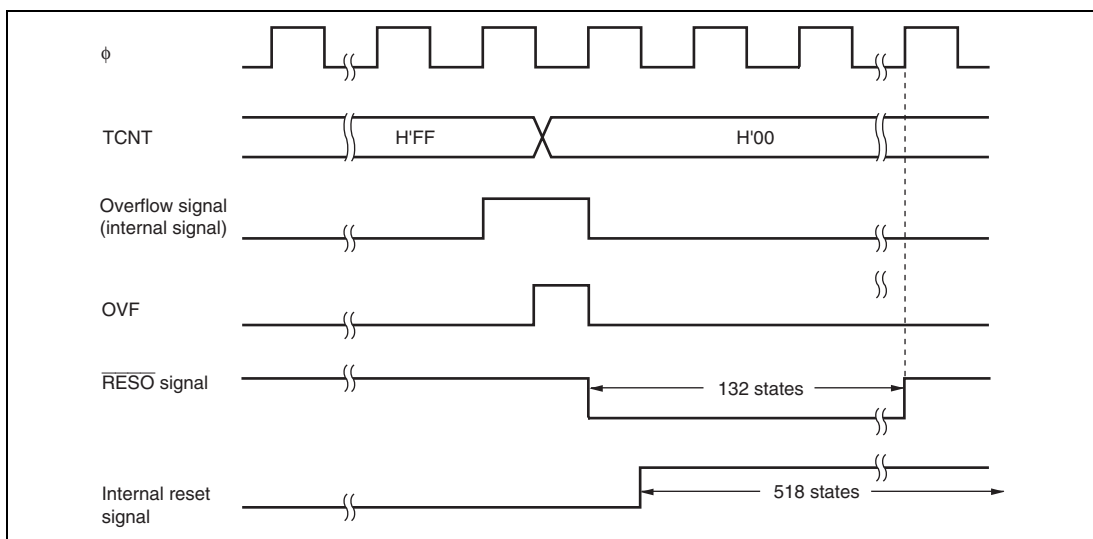
Figure 14.5 Output Timing of \overline{\text{RESO}} signal
