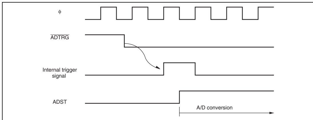
Figure 19.3 External Trigger Input Timing
