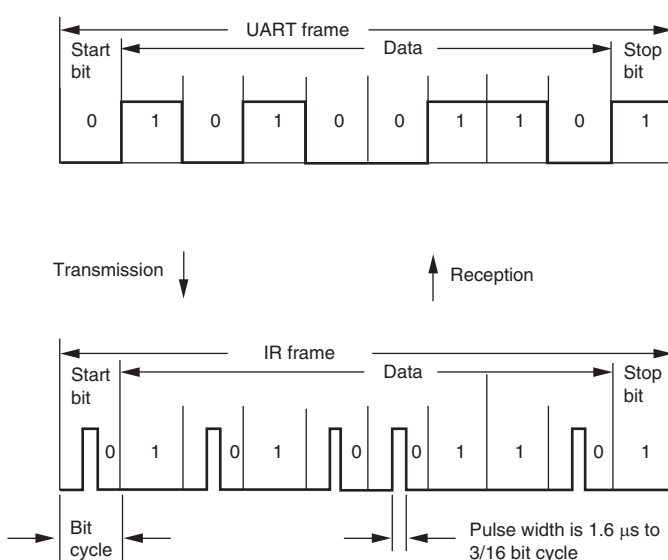
Figure 15.34 IrDA Transmission and Reception
