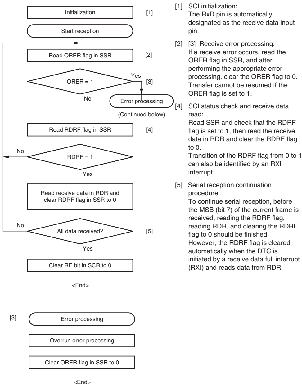
Figure 15.19 Sample Serial Reception Flowchart
