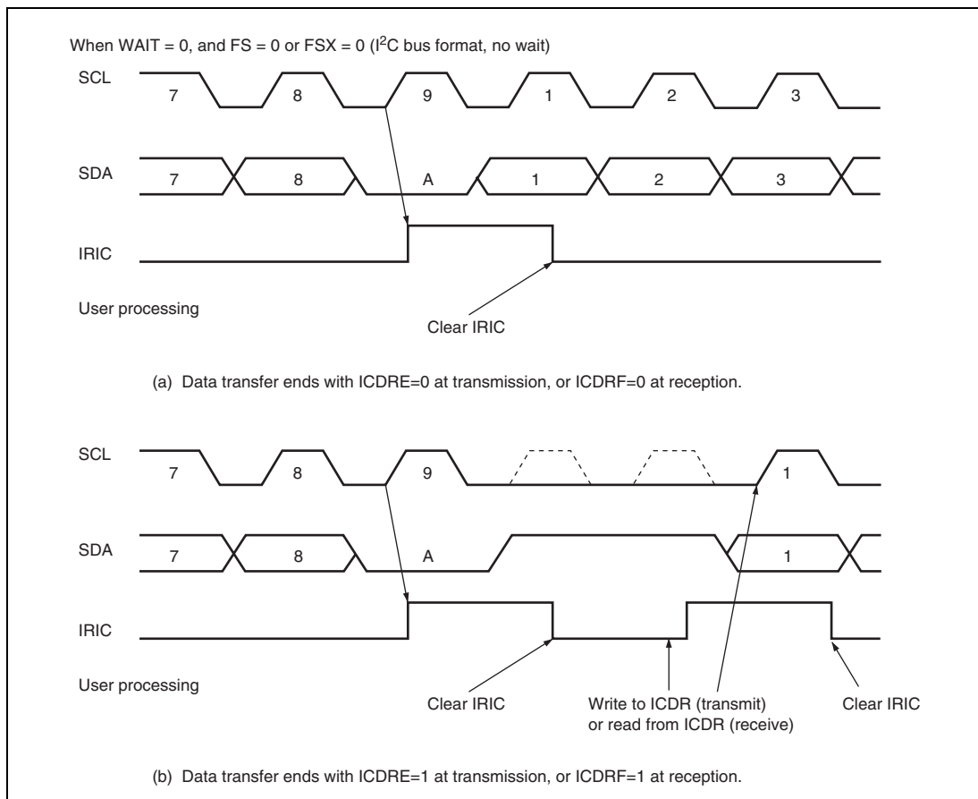
Figure 16.25 IRIC Setting Timing and SCL Control (1)
