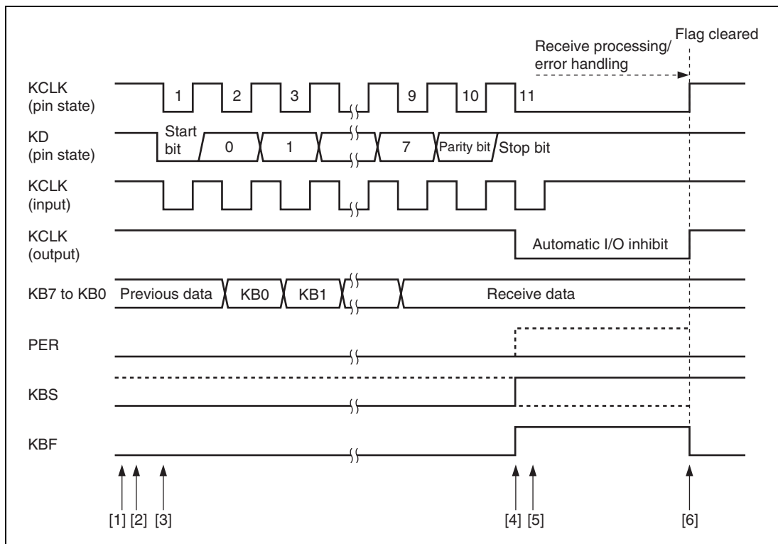
Figure 17.4 Receive Timing
