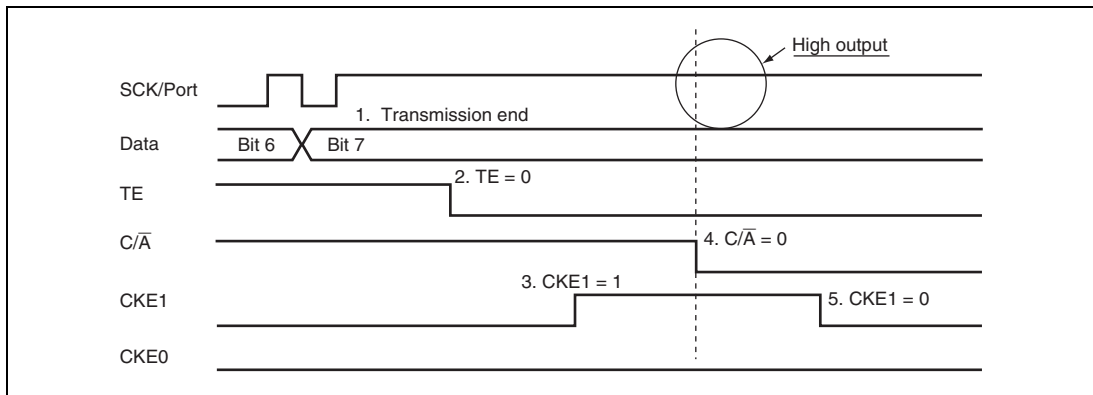
Figure 15.41 Prevention of Low Pulse Output at Switching from SCK Pins to Port Pins
