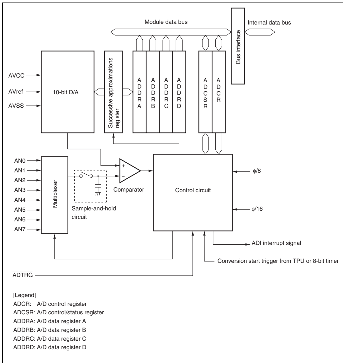
Figure 19.1 Block Diagram of A/D Converter
