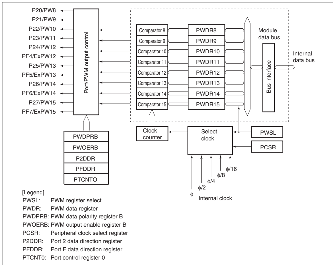
Figure 9.1 Block Diagram of PWM Timer
