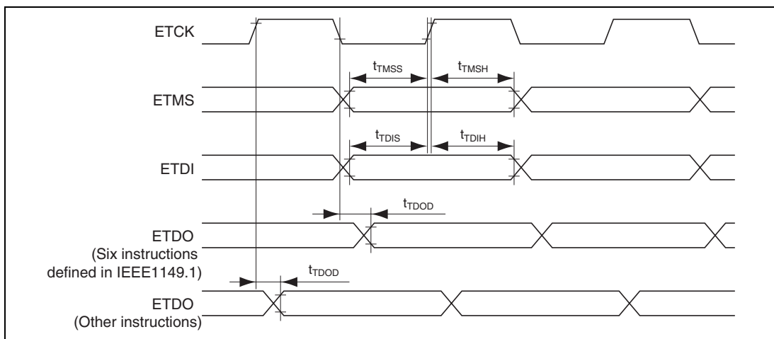
Figure 26.28 JTAG Input/Output Timing
