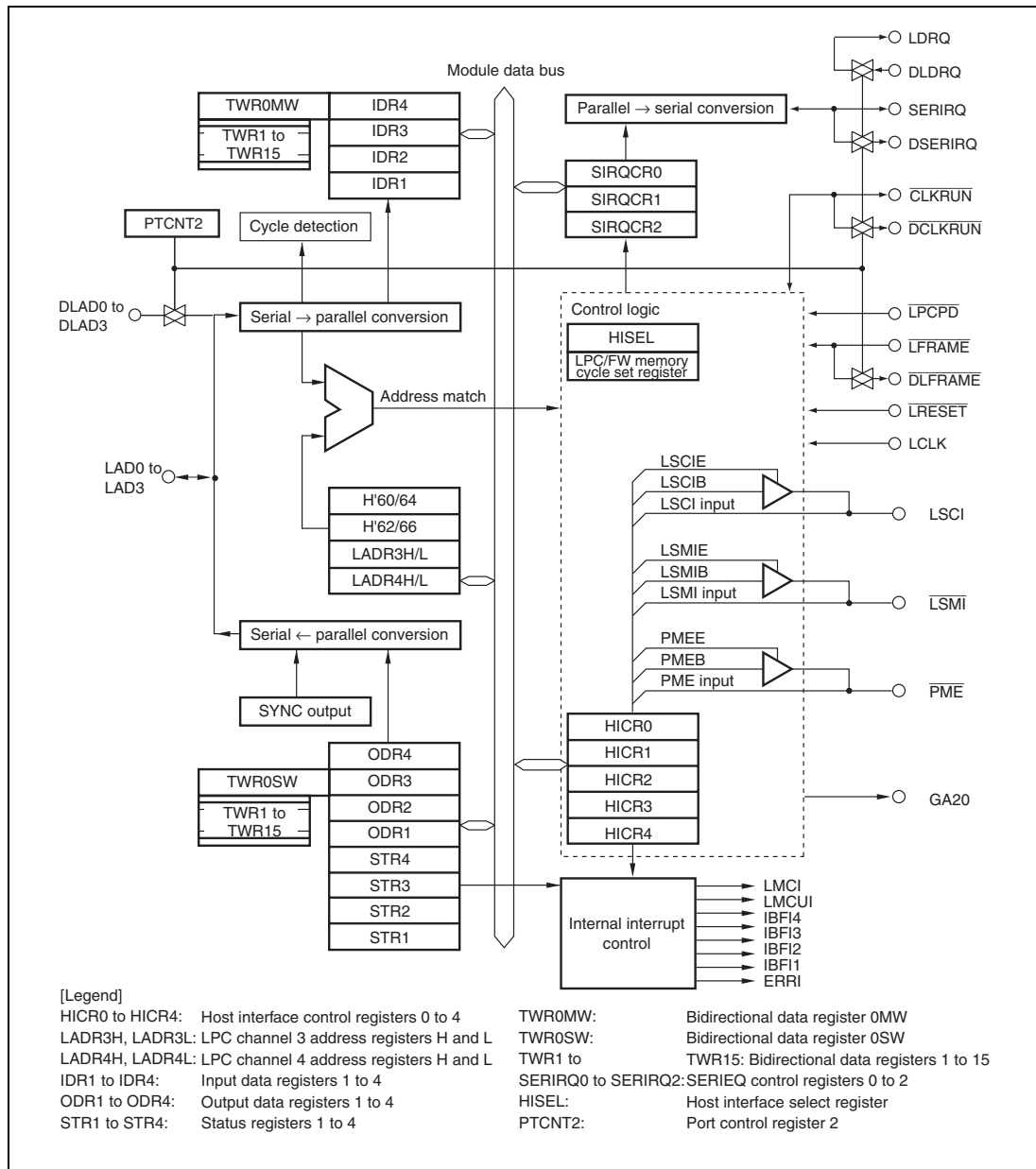
Figure 18.1 Block Diagram of LPC
