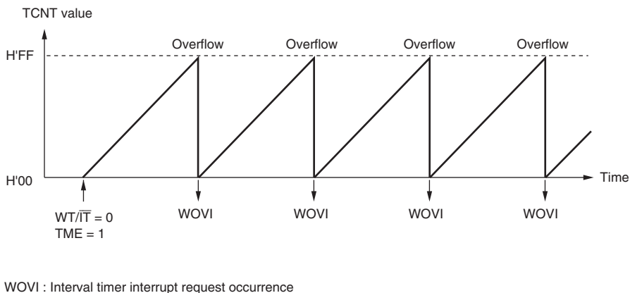
Figure 14.3 Interval Timer Mode Operation
