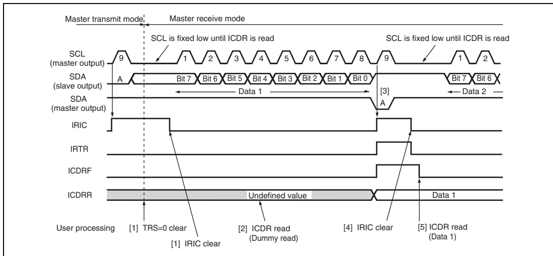
Figure 16.11 Example of Operation Timing in Master Receive Mode (MLS = WAIT = 0, HNDS = 1)
