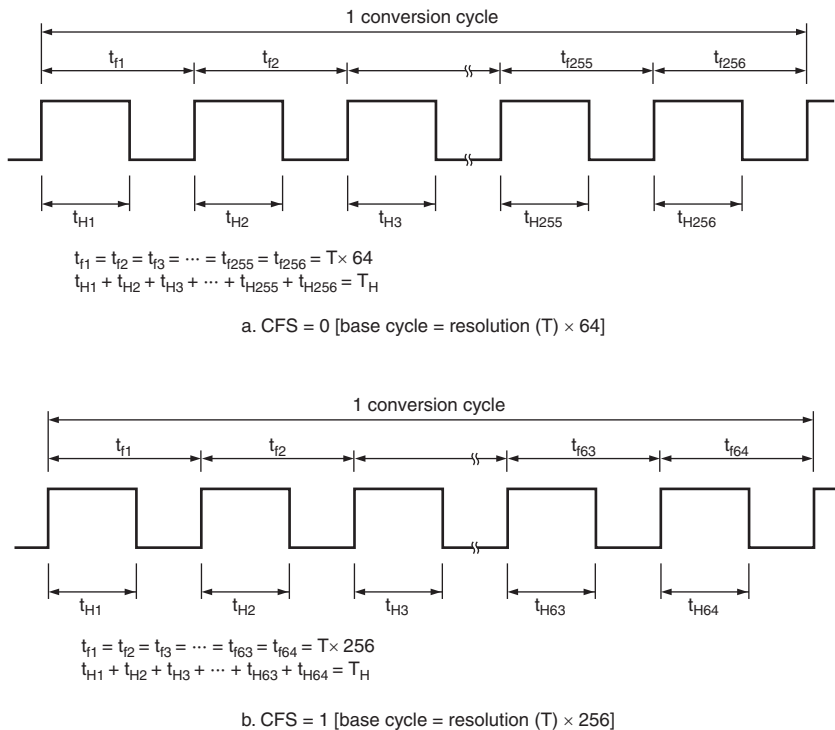
Figure 10.5 Output Waveform (OS = 1, DADR corresponds to T_H )
