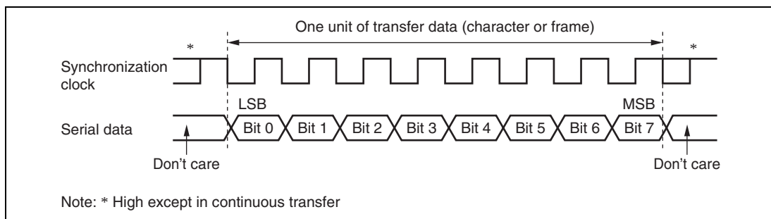
Figure 15.14 Data Format in Synchronous Communication (LSB-First)
