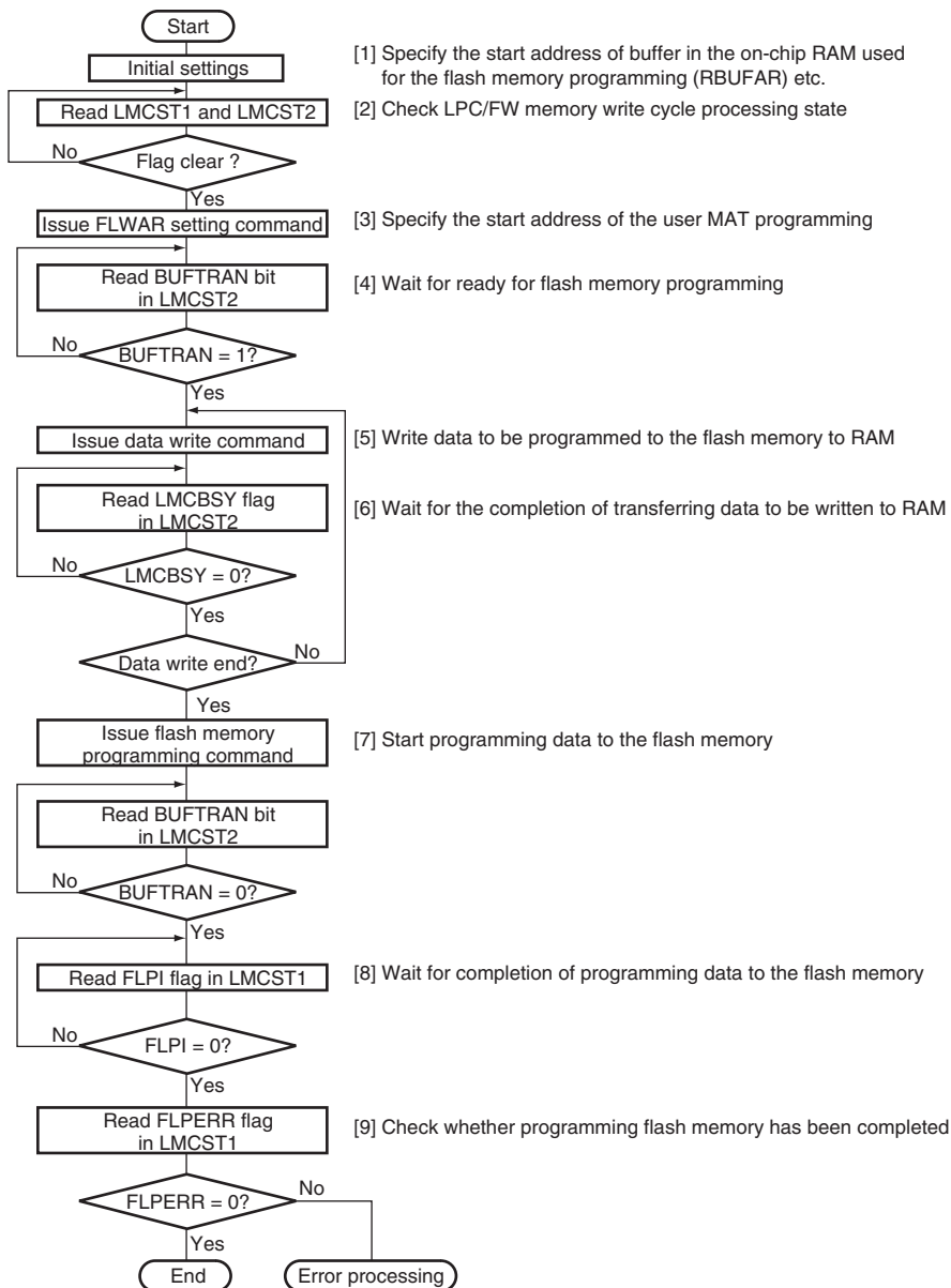
Figure 18.15 Example of Programming Flash Memory
