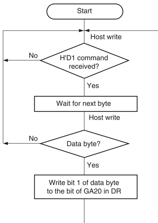
Figure 18.4 GA20 Output
