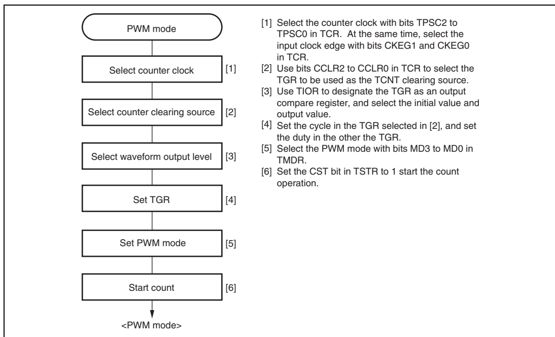
Figure 12.21 Example of PWM Mode Setting Procedure
