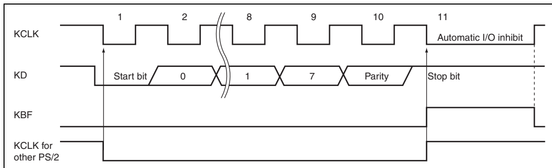
Figure 17.13 Receive Timing and KCLK
