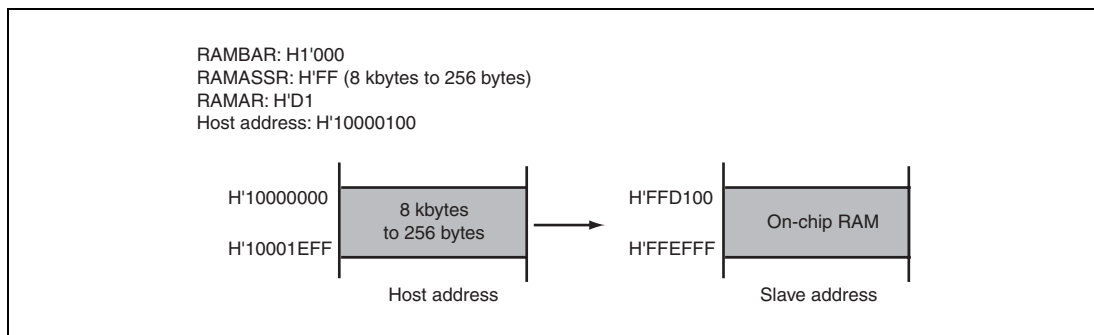
Figure 18.10 Example of On-Chip RAM Address Translation
