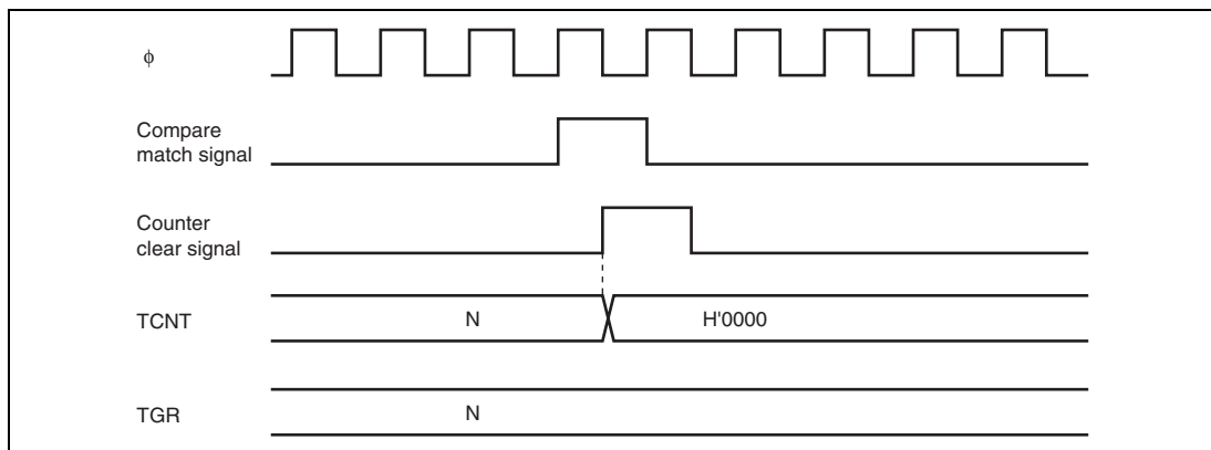
Figure 12.34 Counter Clear Timing (Compare Match)
