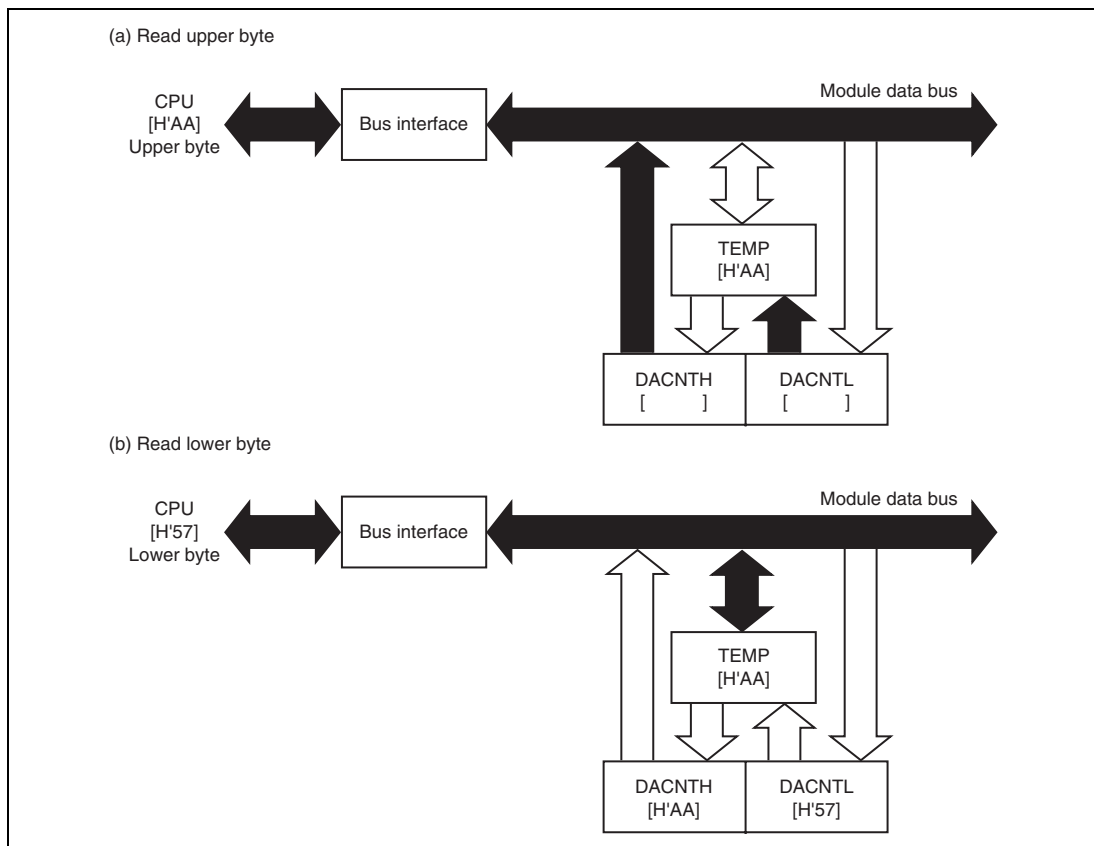
Figure 10.2 (2) DACNT Access Operation (2) [DACNT → CPU(H'AA57) Reading]
