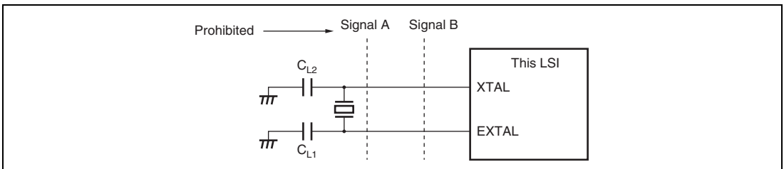
Figure 23.10 Note on Board Design of Oscillator Section
