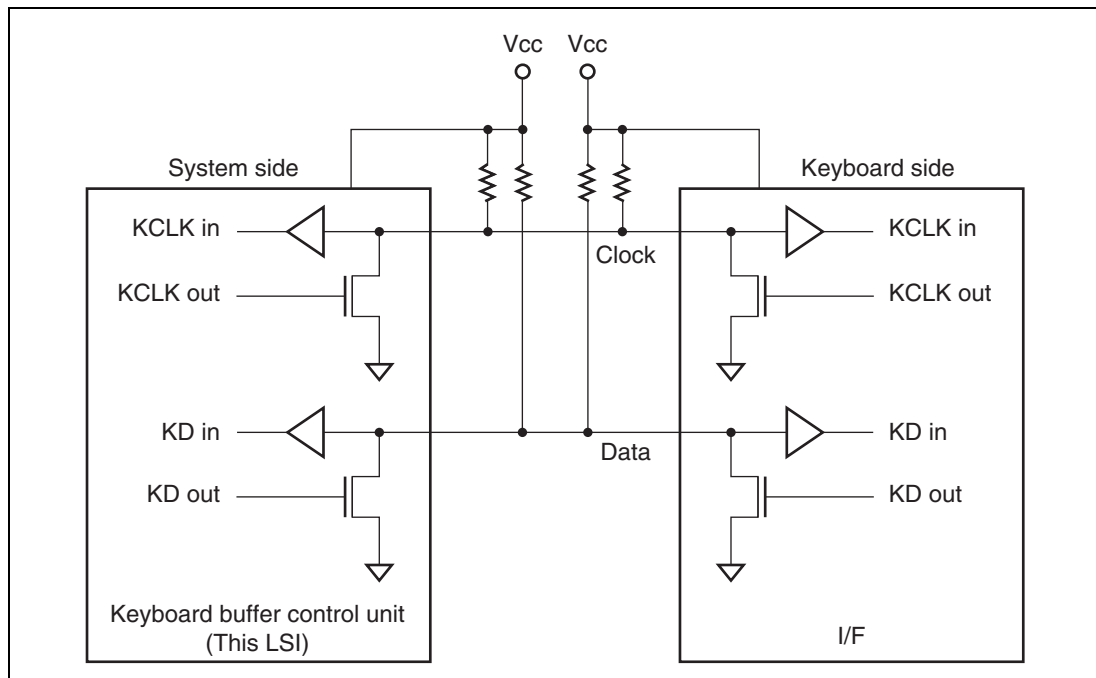
Figure 17.2 KBU Connection
