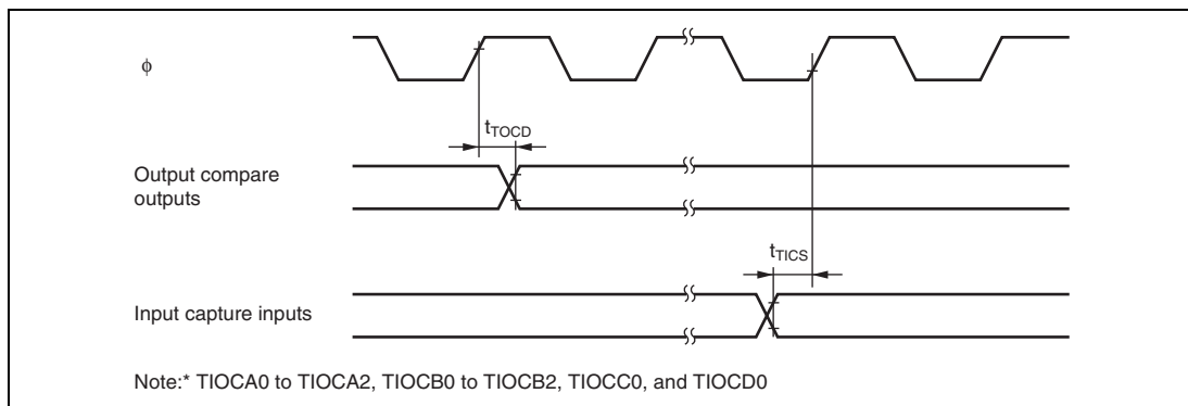
Figure 26.12 TPU Input/Output Timing
