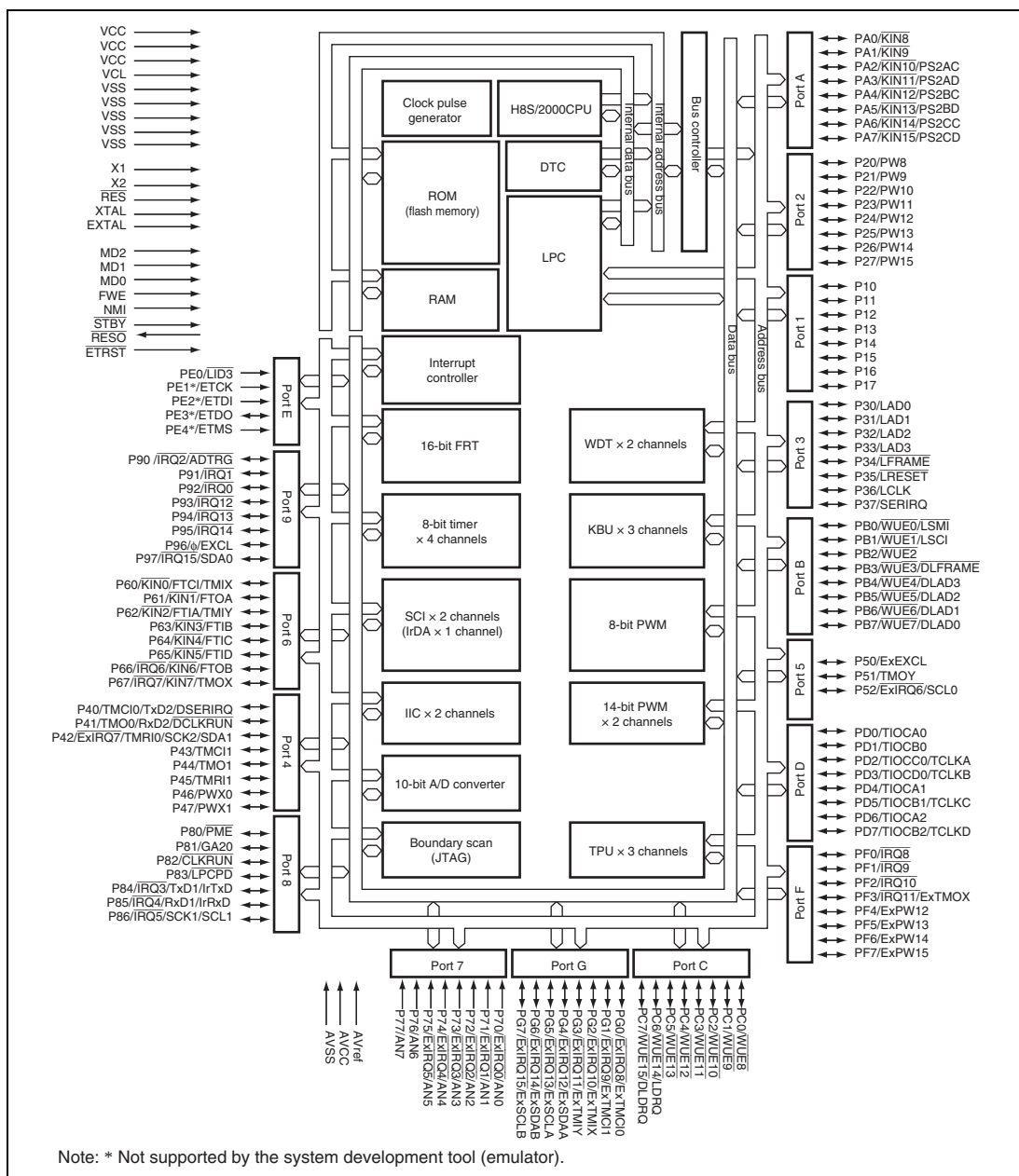
Figure 1.1 H8S/2114R Group Internal Block Diagram
