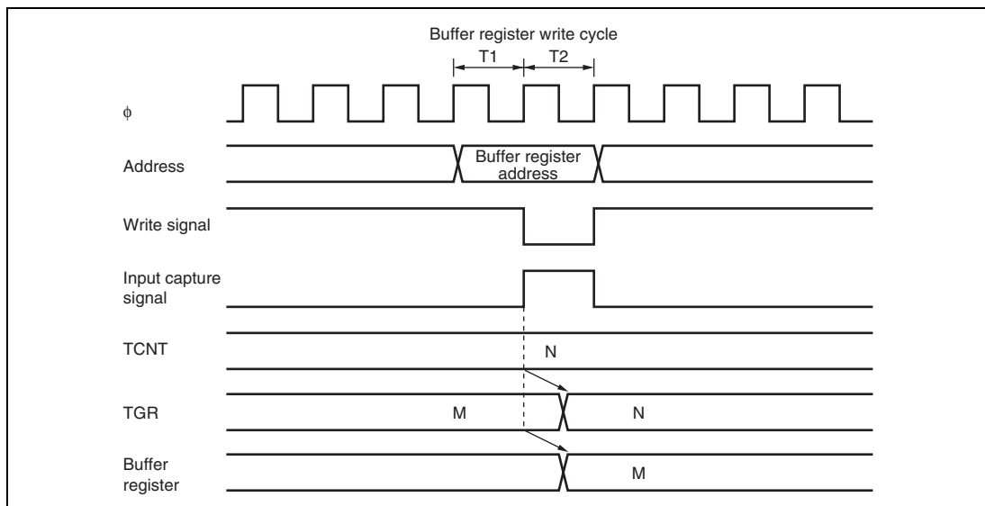
Figure 12.51 Conflict between Buffer Register Write and Input Capture
