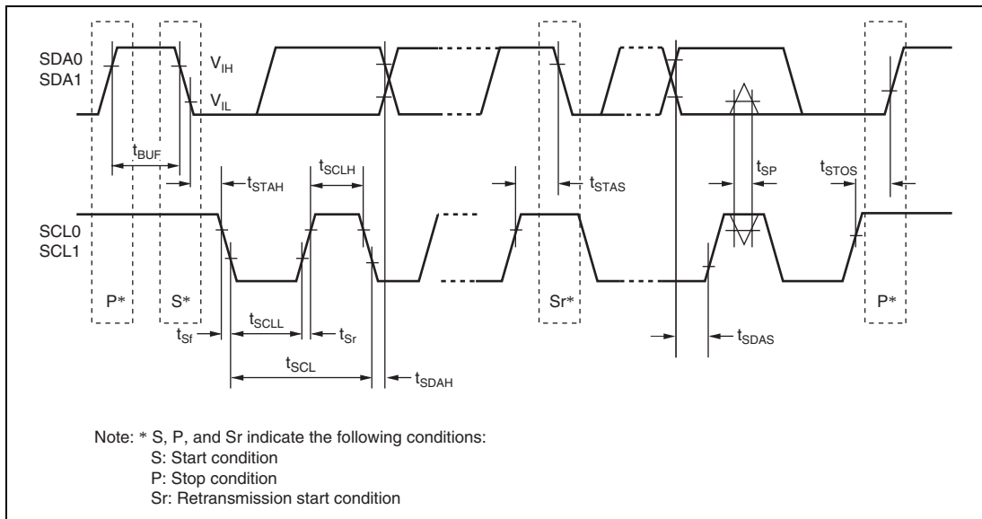
Figure 26.23 I²C Bus Interface Input/Output Timing
