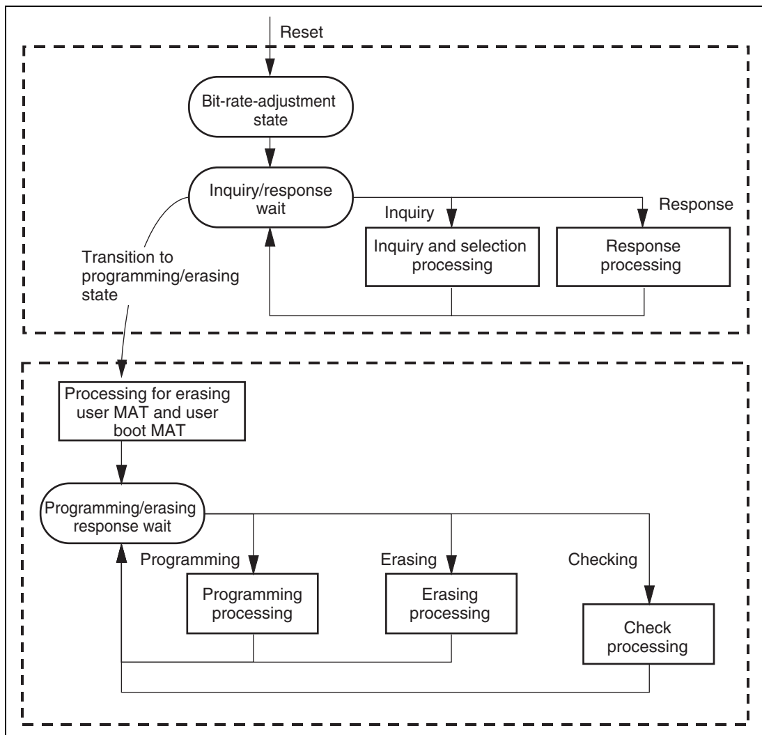
Figure 21.19 Boot Program States
