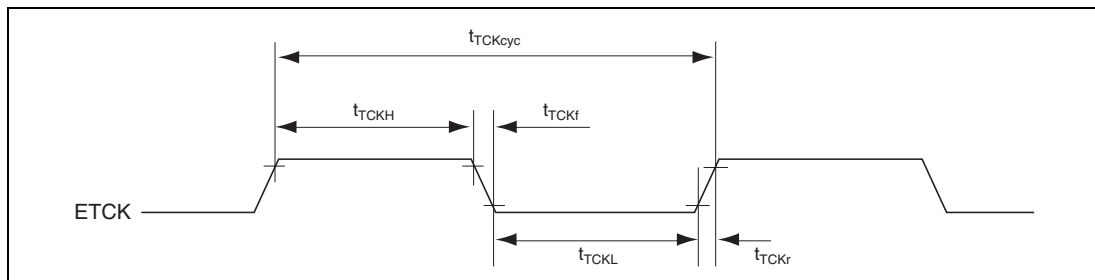
Figure 26.26 JTAG ETCK Timing
