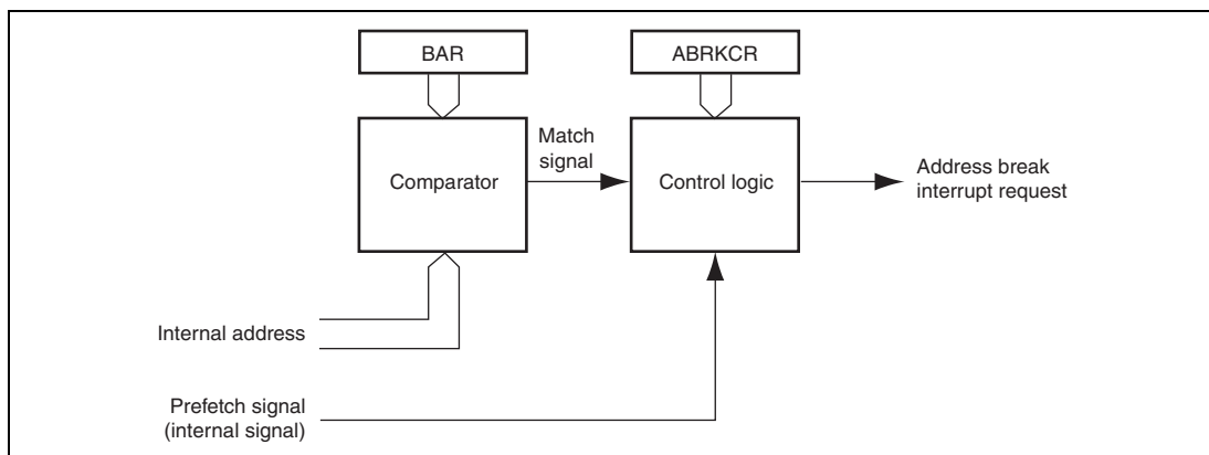
Figure 5.12 Block Diagram of Address Break Function
