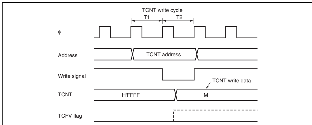
Figure 12.53 Conflict between TCNT Write and Overflow
