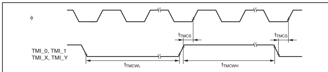
Figure 26.15 8-Bit Timer Clock Input Timing
