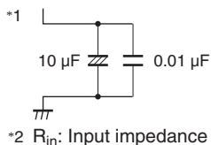
Figure 19.7 Example of Analog Input Protection Circuit
