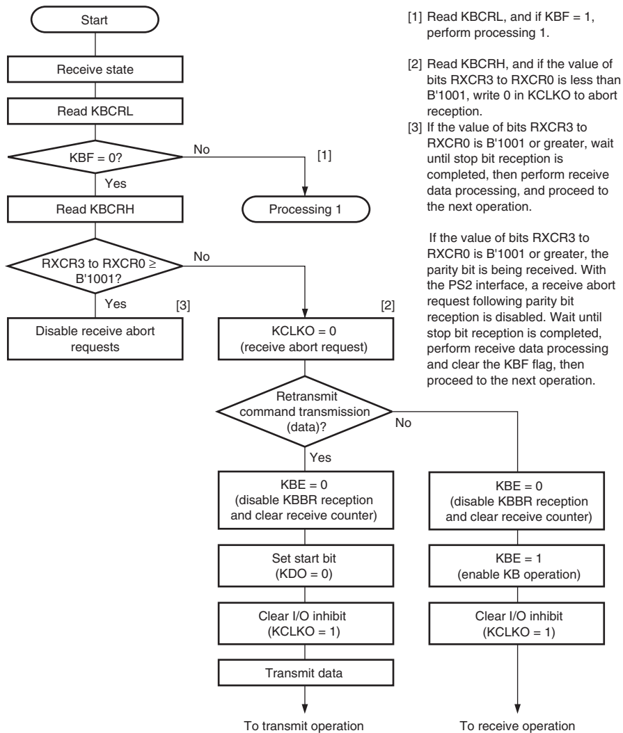
Figure 17.7 (1) Sample Receive Abort Processing Flowchart
