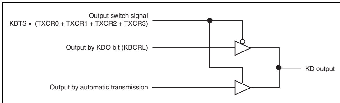
Figure 17.20 KD Output
