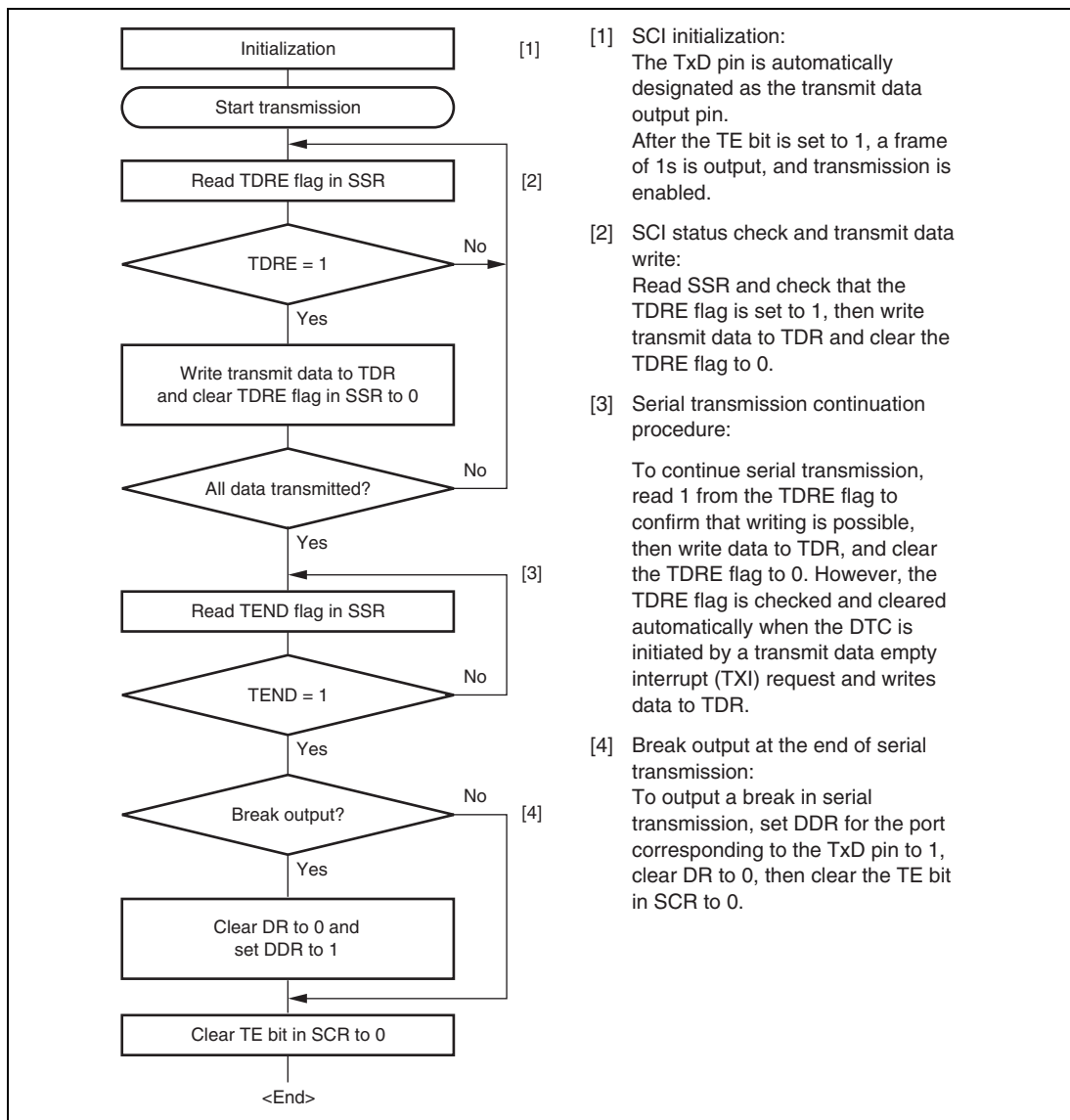
Figure 15.7 Sample Serial Transmission Flowchart
