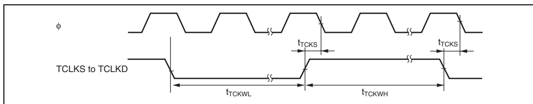
Figure 26.13 TPU Clock Input Timing
