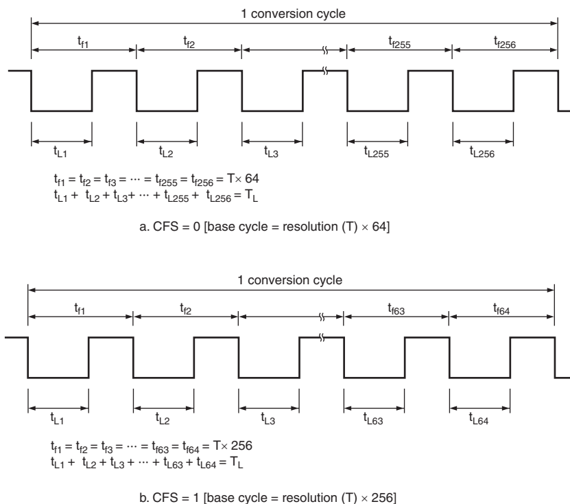
Figure 10.4 Output Waveform (OS = 0, DADR corresponds to T_L )
