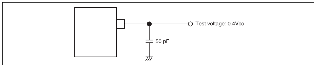
Figure 26.25 Test Conditions for Tester
