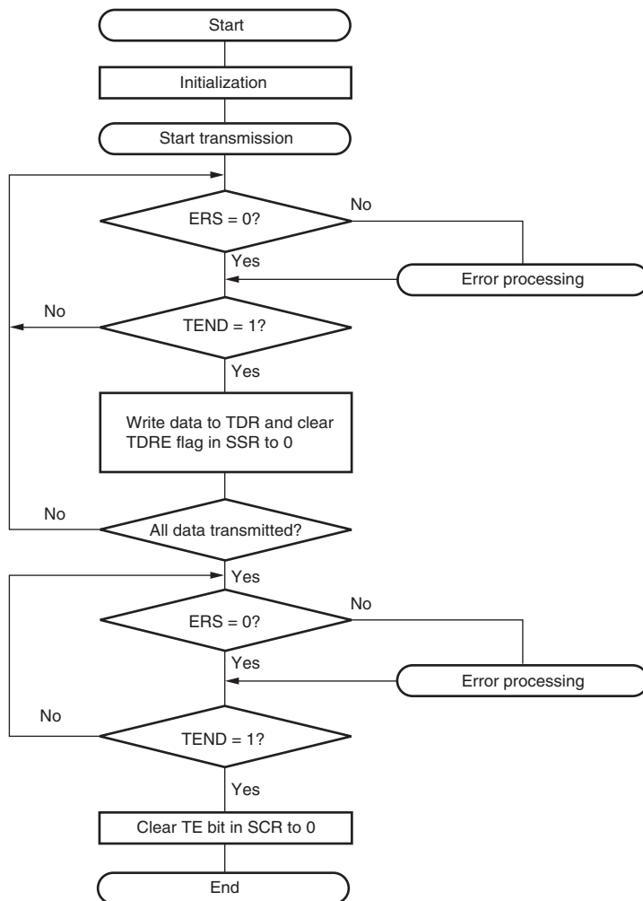
Figure 15.28 Sample Transmission Flowchart
