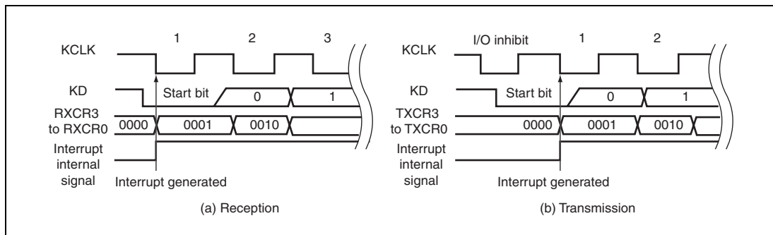
Figure 17.15 Timing of First KCLK Interrupt
