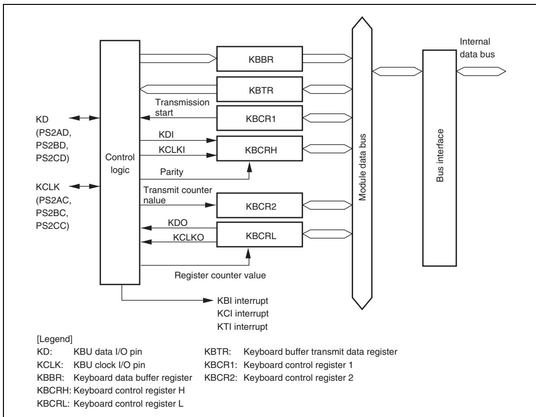
Figure 17.1 Block Diagram of KBU
