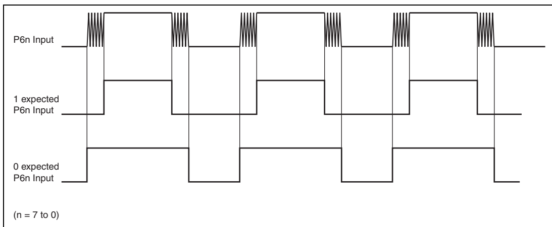
Figure 8.2 Noise Cancel Operation
