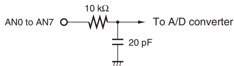
Figure 19.7 Example of Analog Input Protection Circuit
