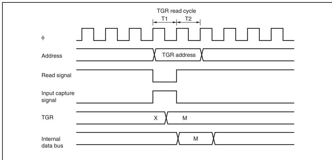
Figure 12.49 Conflict between TGR Read and Input Capture
