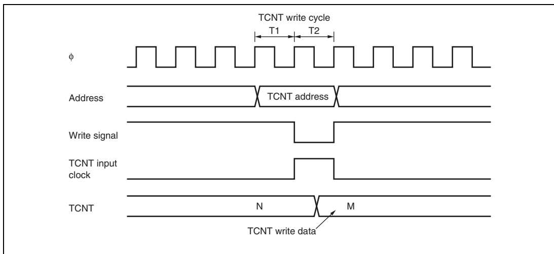
Figure 12.46 Conflict between TCNT Write and Increment Operations
