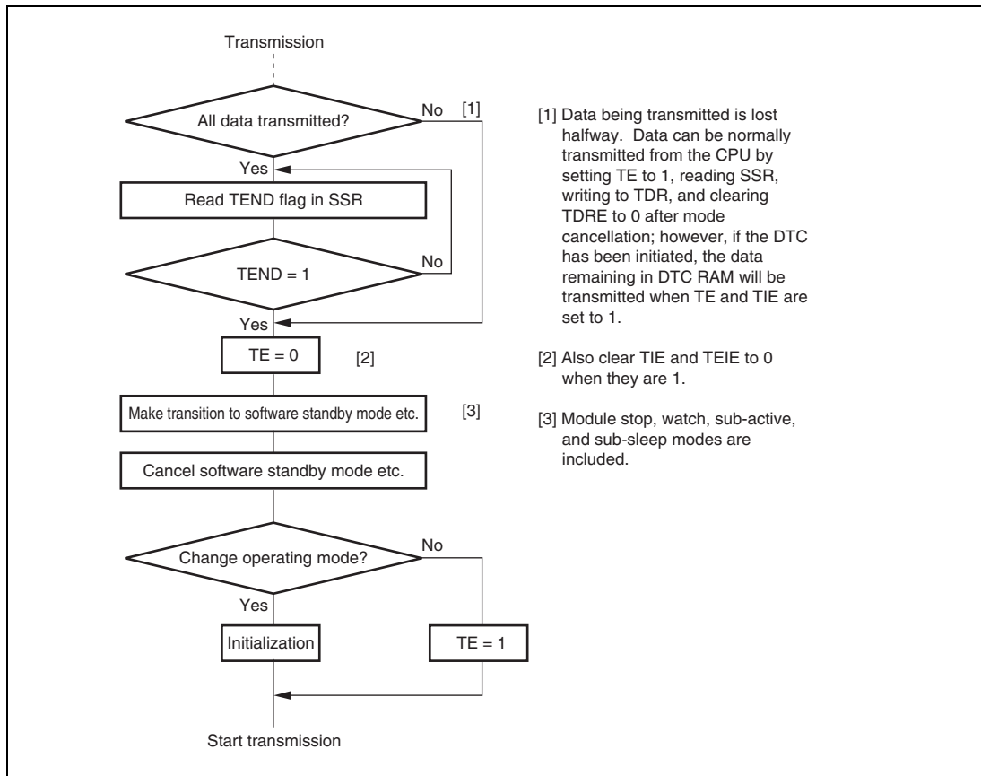
Figure 15.36 Sample Flowchart for Mode Transition during Transmission
