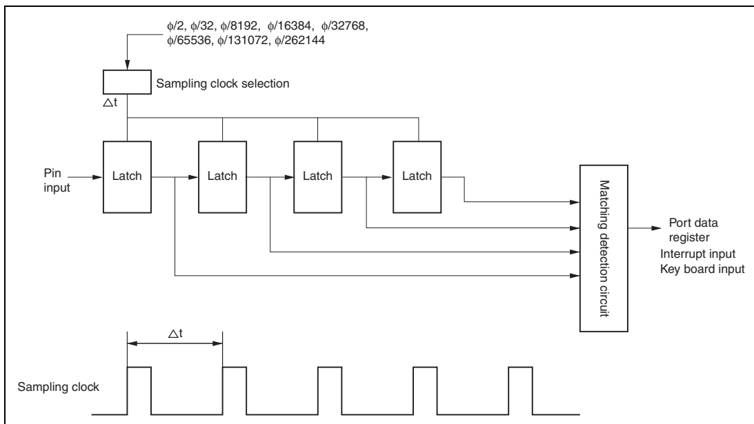
Figure 8.1 Noise Cancel Circuit
