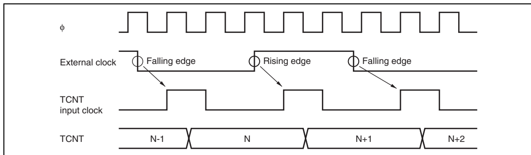
Figure 12.31 Count Timing in External Clock Operation
