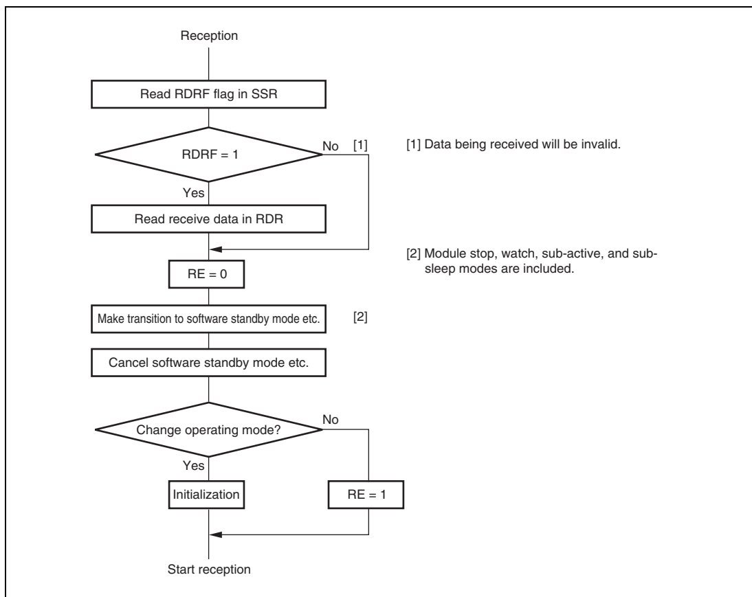
Figure 15.39 Sample Flowchart for Mode Transition during Reception
