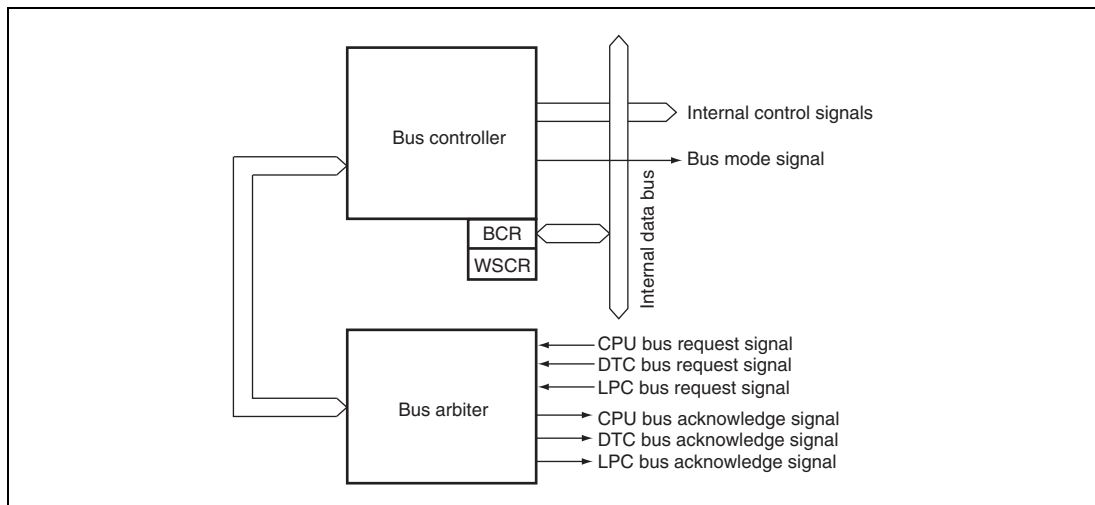
Figure 6.1 Block Diagram of BSC
