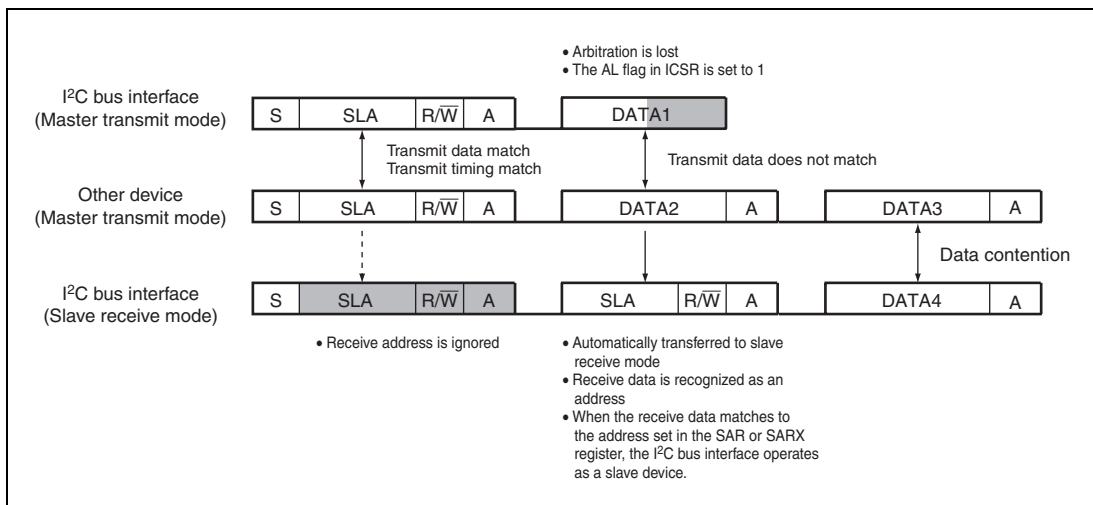
Figure 16.35 Diagram of Erroneous Operation when Arbitration is Lost
