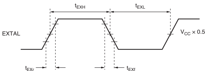
Figure 23.5 External Clock Input Timing
