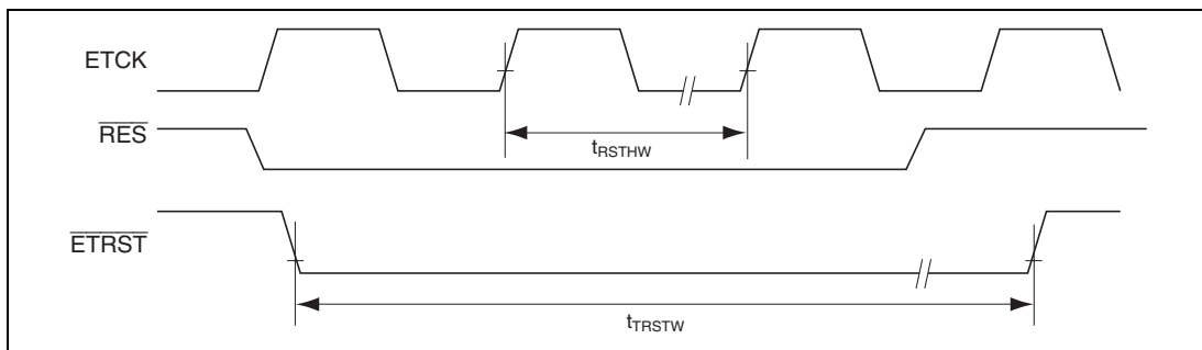
Figure 26.27 Reset Hold Timing
