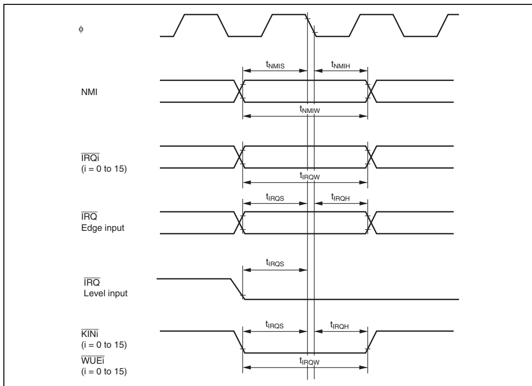
Figure 26.8 Interrupt Input Timing
