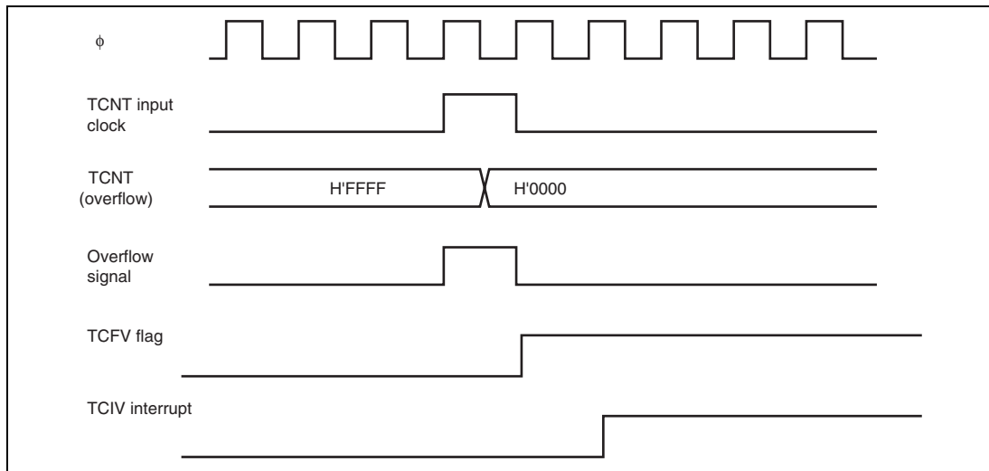
Figure 12.40 TCIV Interrupt Setting Timing
