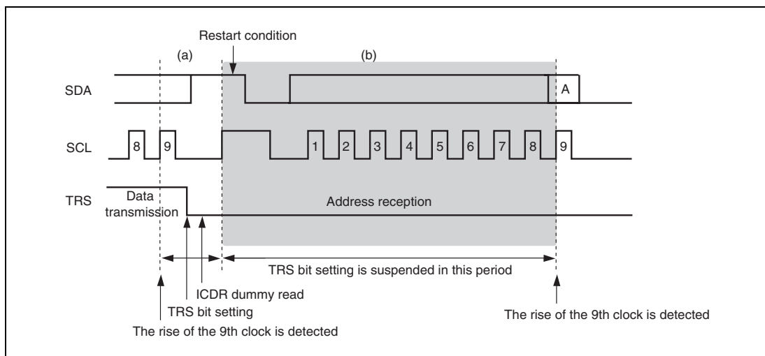
Figure 16.34 TRS Bit Set Timing in Slave Mode
