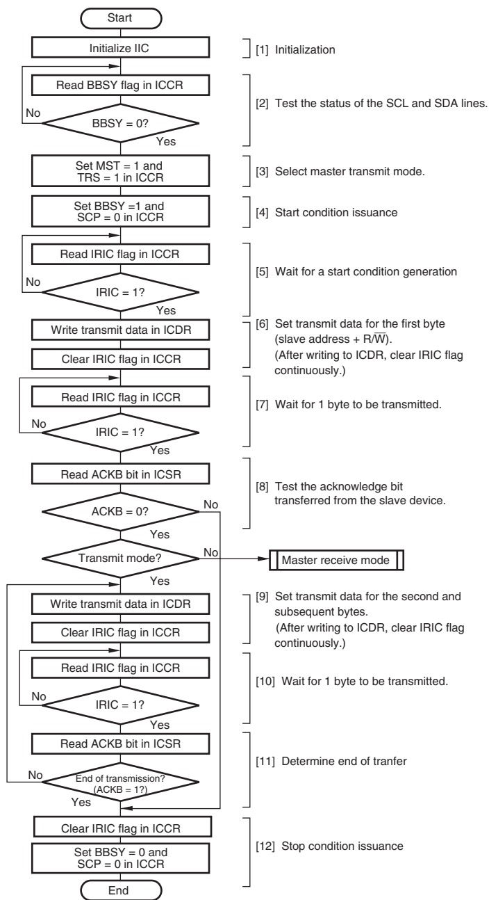
Figure 16.7 Sample Flowchart for Operations in Master Transmit Mode
