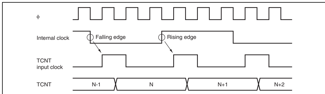
Figure 12.30 Count Timing in Internal Clock Operation
