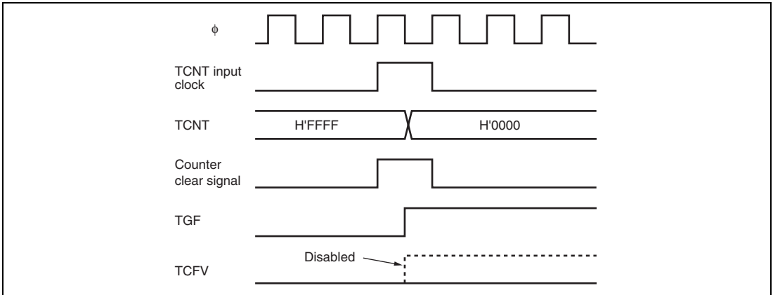
Figure 12.52 Conflict between Overflow and Counter Clearing
