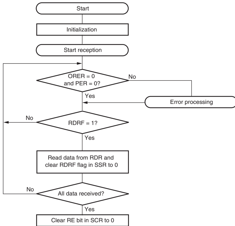
Figure 15.30 Sample Reception Flowchart
