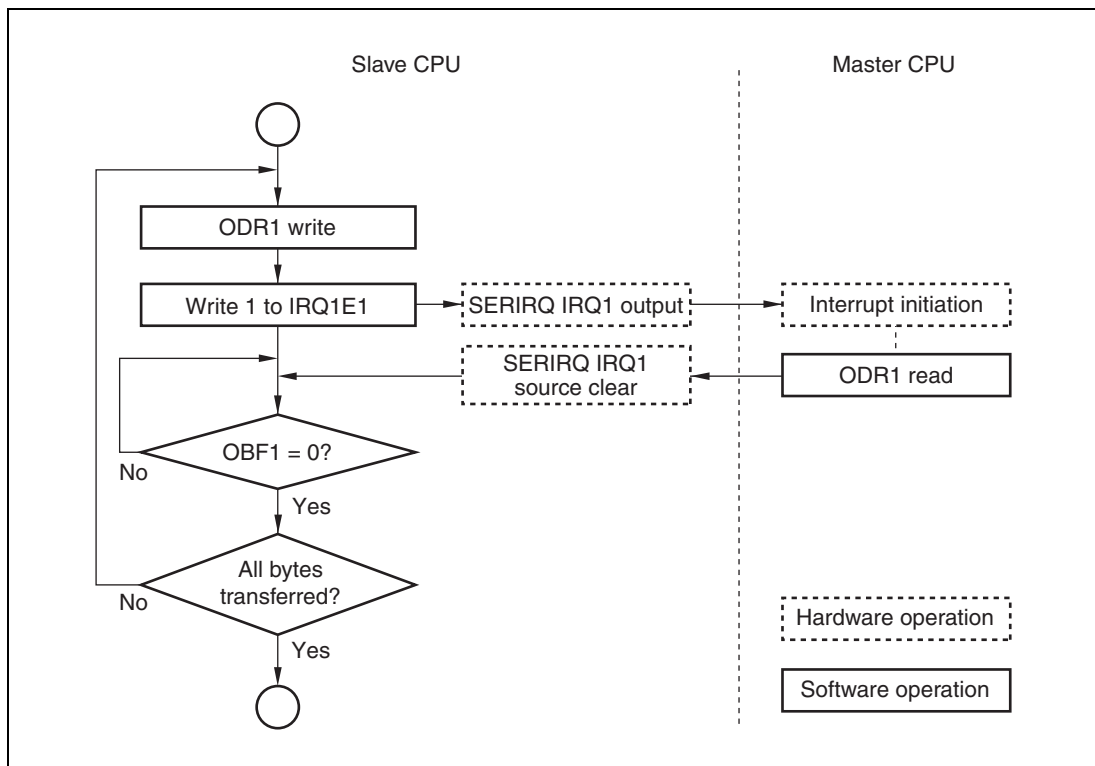
Figure 18.17 HIRQ Flowchart (Example of Channel 1)
