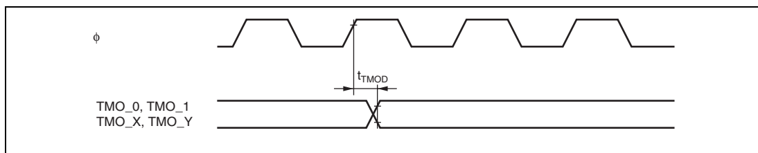
Figure 26.14 8-Bit Timer Output Timing
