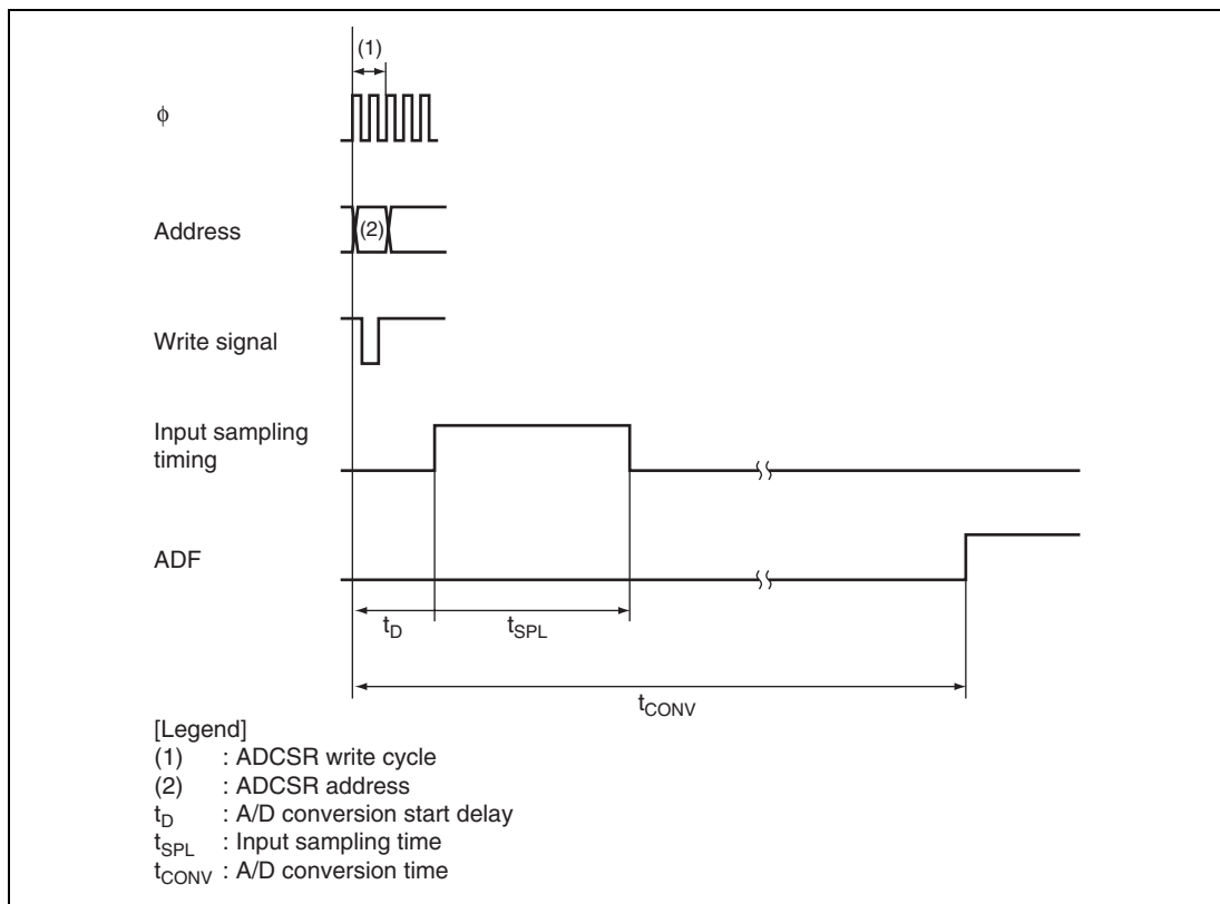
Figure 19.2 A/D Conversion Timing
