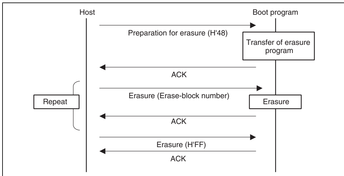
Figure 21.24 Erasure Sequence
