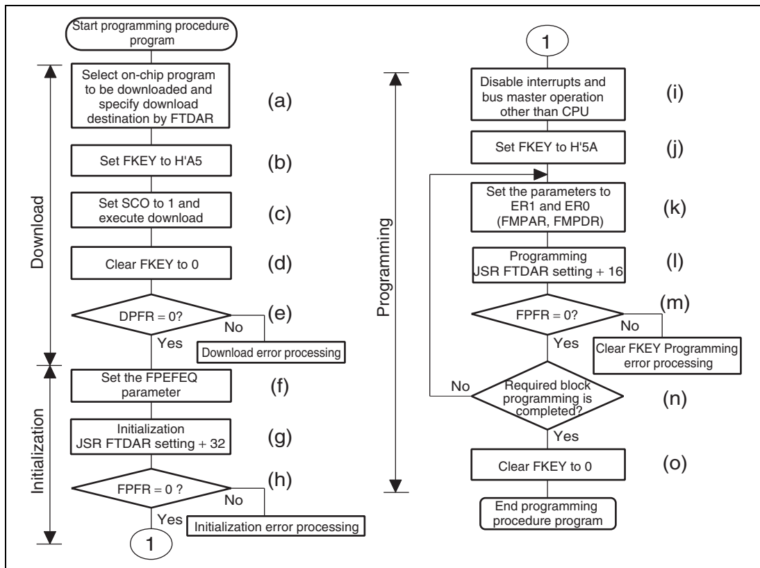
Figure 21.11 Programming Procedure
