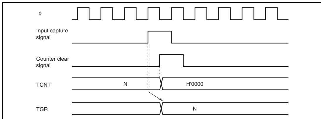
Figure 12.35 Counter Clear Timing (Input Capture)
