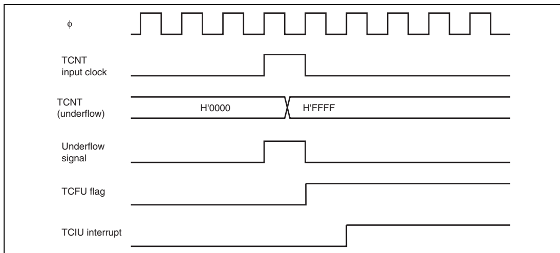
Figure 12.41 TCIU Interrupt Setting Timing
