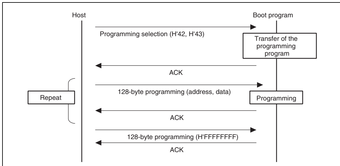
Figure 21.23 Programming Sequence
