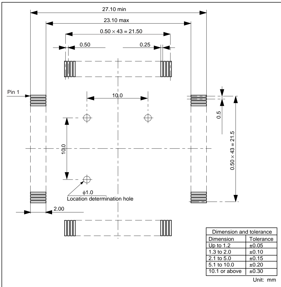
Figure 4 Recommended Dimensions for Mount Pad
