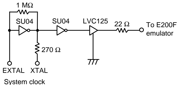
Figure 10 Clock Oscillator
