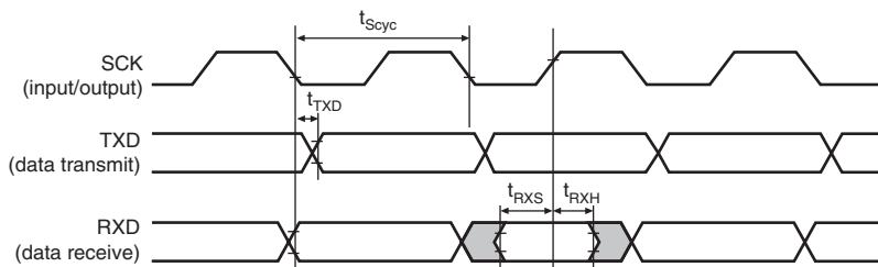
Figure 27.47 SCIF Input/Output Timing in Clocked Synchronous Mode
